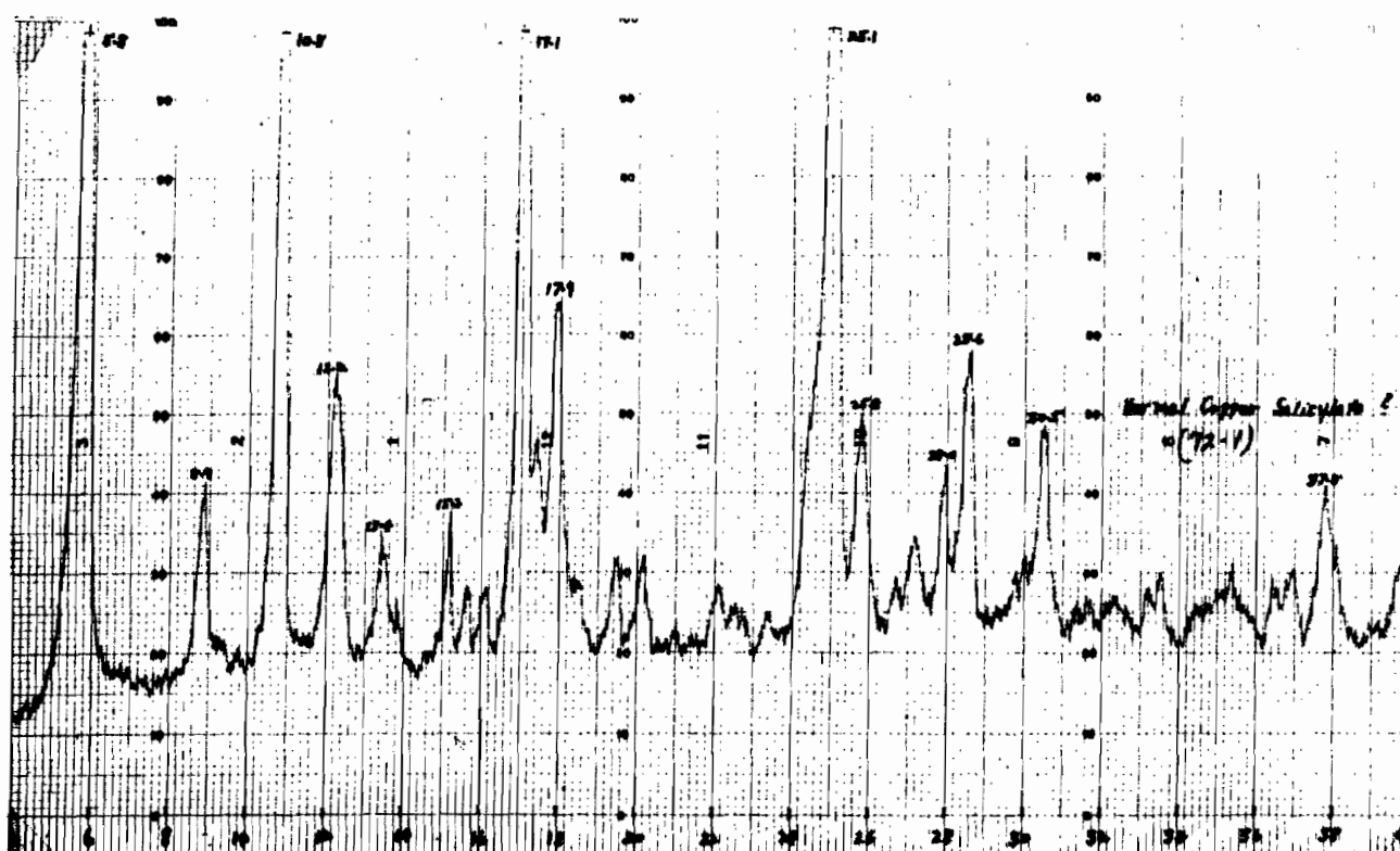
Figure 4 X-ray Diffraction Pattern of Sample 72-1
