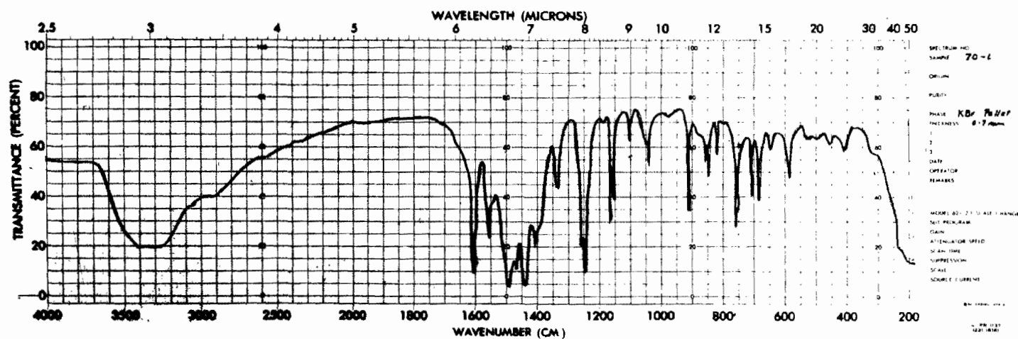
Figure 14 Infrared Spectrum of Sample 70-1
