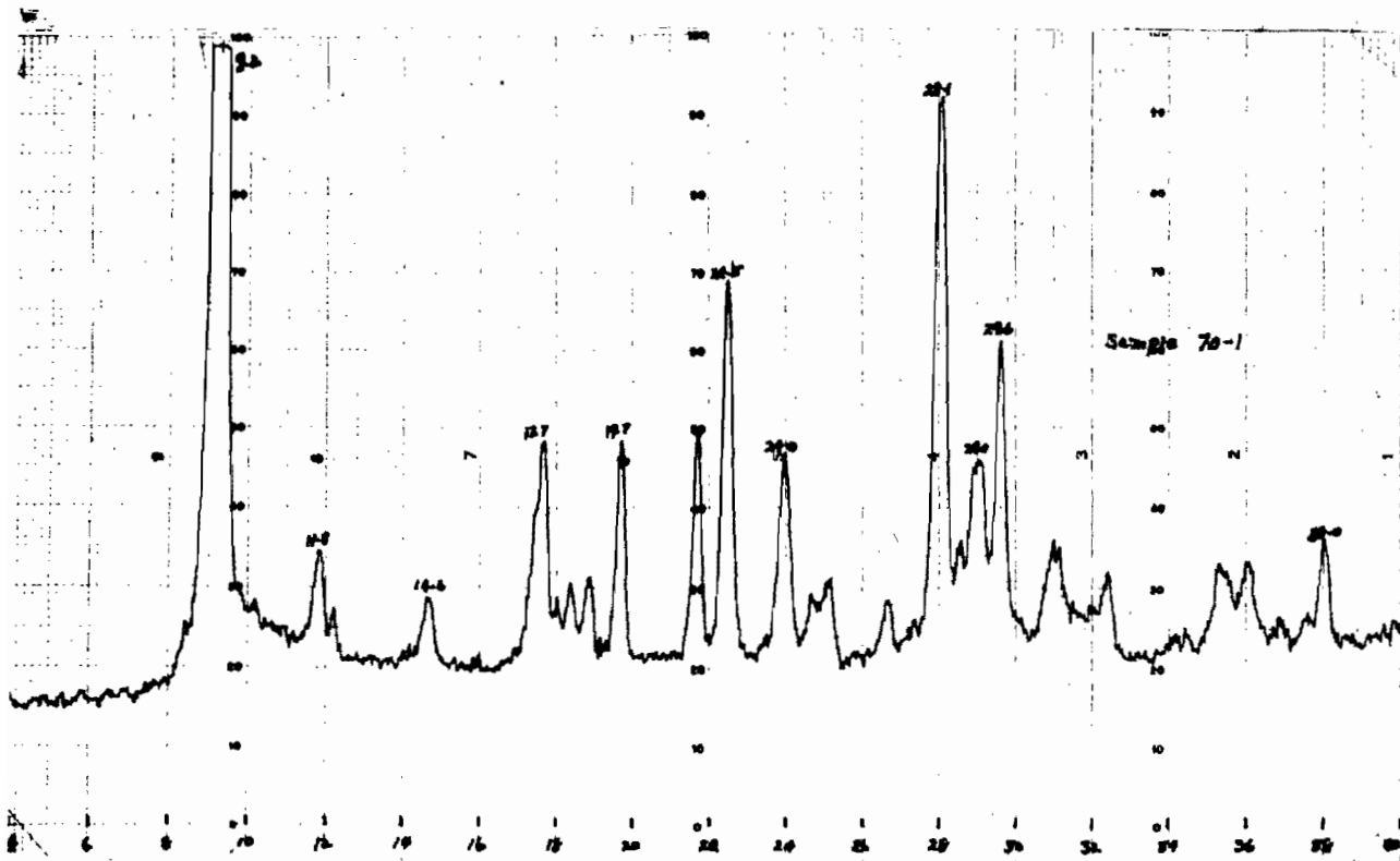
Figure 2 X-ray Diffraction Pattern of Sample 70-1
