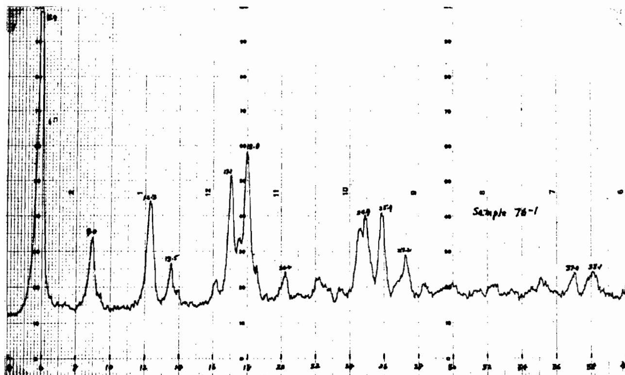
Figure 6 X-ray Diffraction Pattern of Sample 76-1
