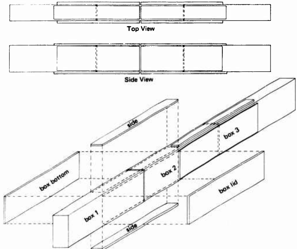
Figure 3. Construction plan for beam made from three 106-mm ammunition boxes (10-foot clear span).
