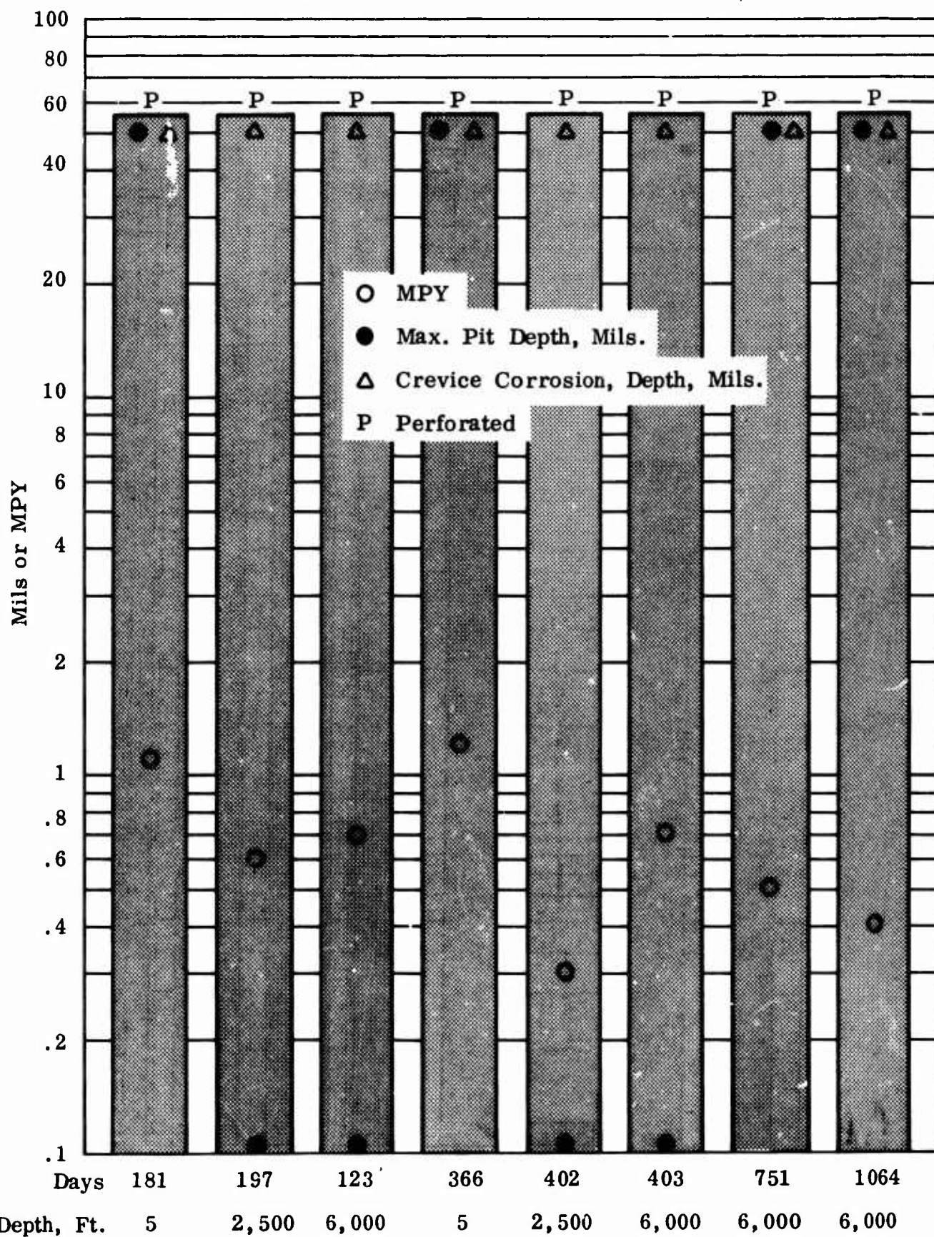
Figure 11. Corrosion rates, maximum pit depths and crevice corrosion of AISI Type 304 (sensitized) stainless steel in seawater at the surface and at depth.
