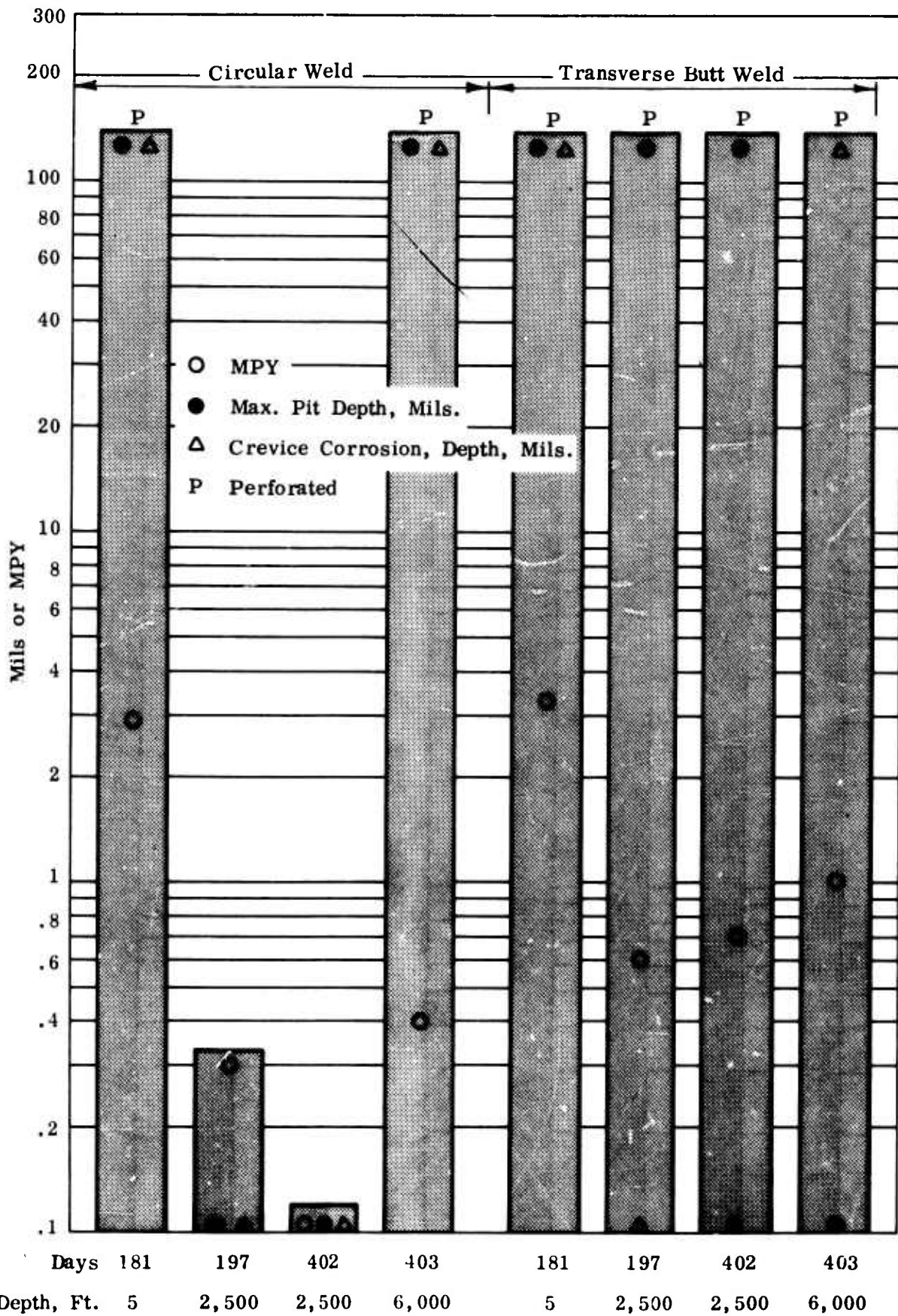
Figure 30. Corrosion rates, maximum pit depths and crevice corrosion of welded AISI Type 631-RH1050 precipitation hardening stainless steel in seawater at the surface and at depth.
