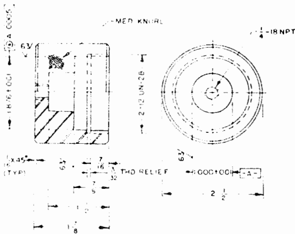
Figure B1. Test device end cap
