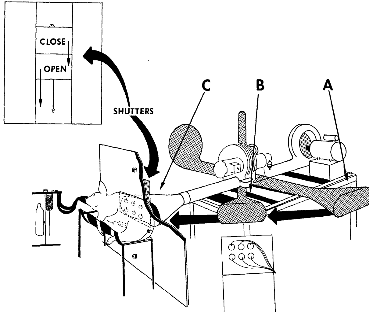
FIGURE 1. Experimental apparatus showing the flame gun, thermal barrier with shutter system, pig in transporting device, and thermocouples for steady-state temperature data. Position A is for warm-up, position B is for steady-state flame temperature determinations, and C is the position of the flame gun during an experiment.
