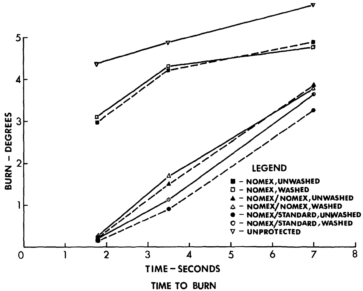
FIGURE 4. Average degree of burn (gross evaluation) vs exposure time.
