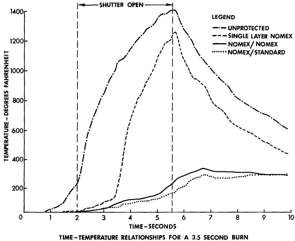
FIGURE 7. These representative temperatures were measured by a thermocouple placed between the fabric and the skin at the center of each test site. The temperature rise which occurred before the shutter opened is due to the heating of the shutter by the flame gun.
