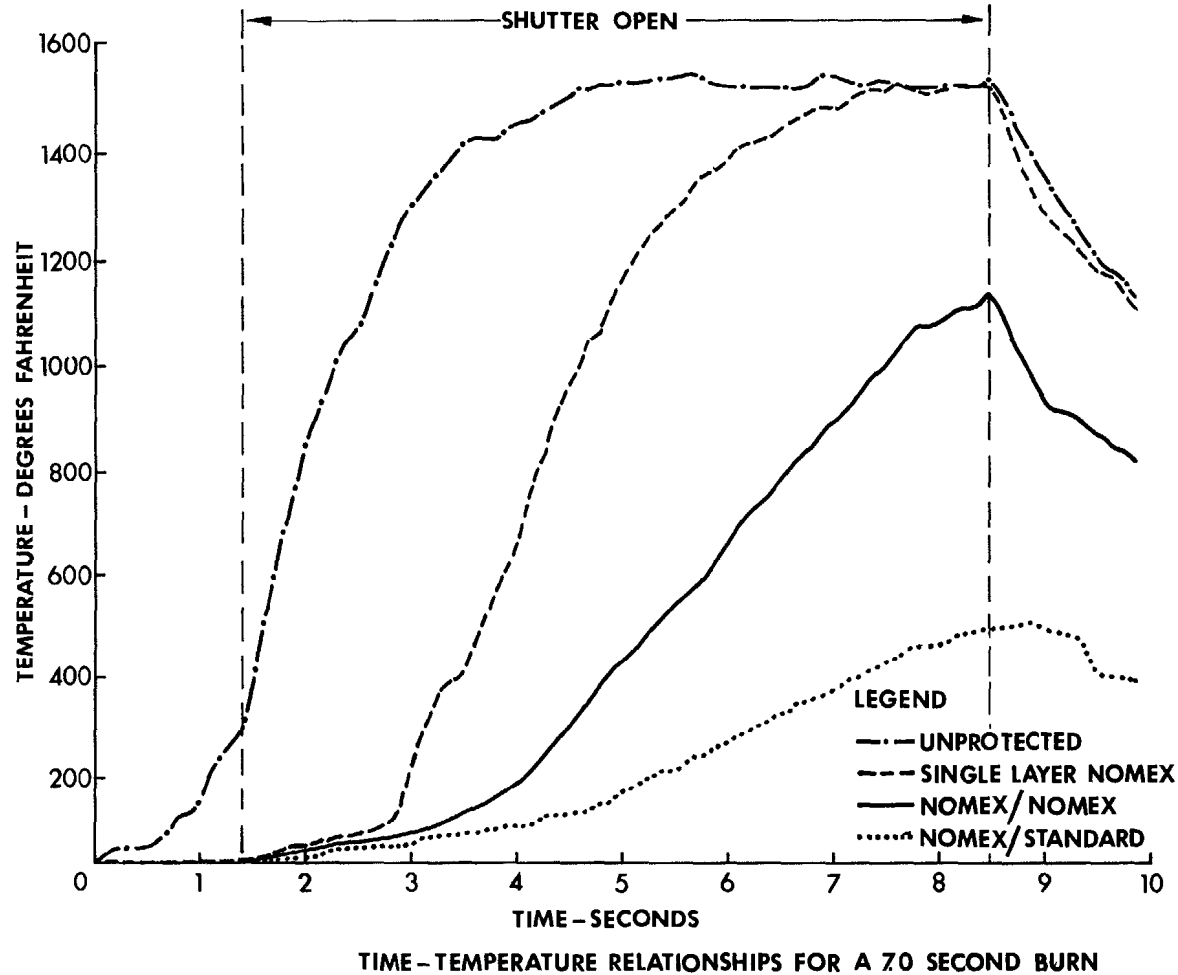
FIGURE 8. These representative temperatures were measured by a thermocouple placed between the fabric and the skin at the center of each test site. The temperature rise which occurred before the shutter opened is due to the heating of the shutter by the flame gun.
