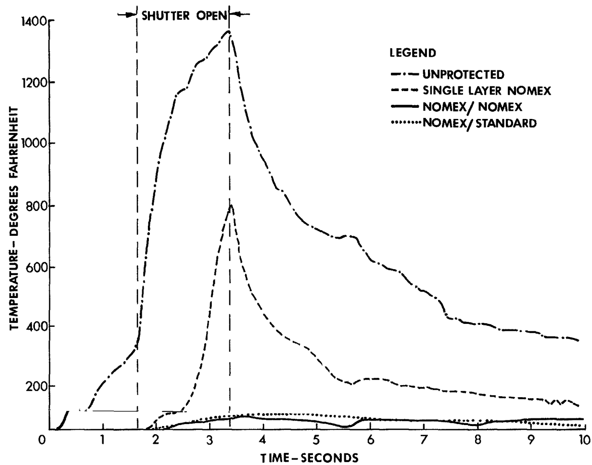
TIME-TEMPERATURE RELATIONSHIPS FOR A 1.75 SECOND BURN
