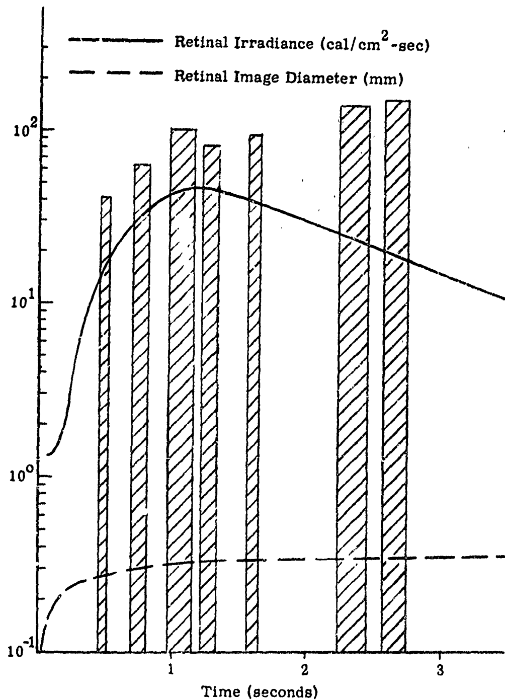
Figure 13 - Retinal irradiance as a function of time for primate exposed to high yield, low altitude detonation. Cross-hatched areas indicate periods when monkey's eyes were closed, open areas indicate periods when retinal exposure occurred (43a).
