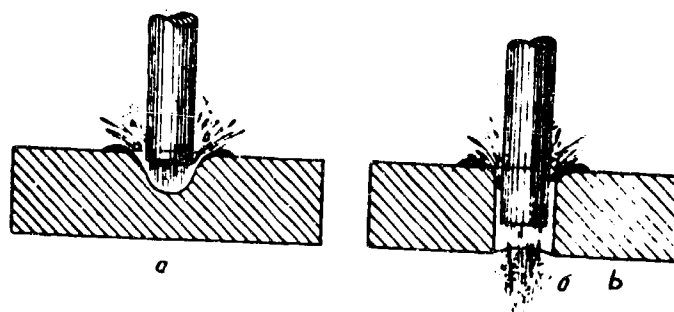
Fig. 86. Burning a Hole Through Metal with an Arc.: a - beginning of cut; and b - completion of the cut.
