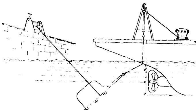
Fig. 45. Pulling a Vertical Rudder from Under the Stern Overhang.
