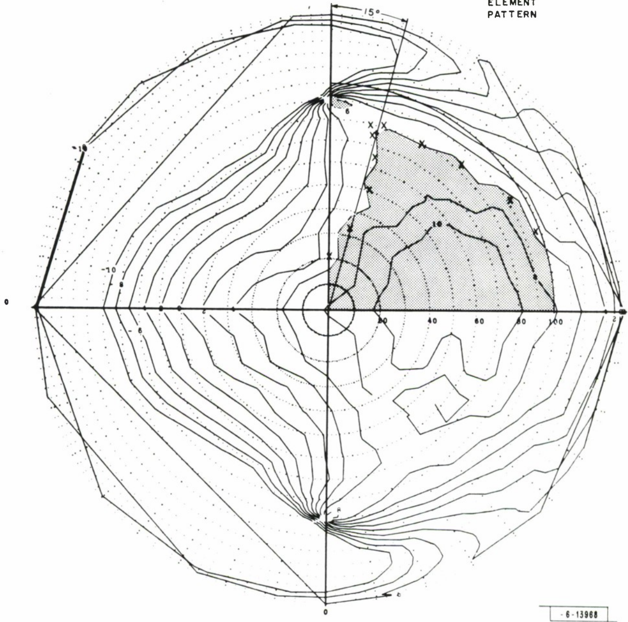
Fig. 5. Contour plot in the (\theta, \phi) plane, 400 MHz, 50^\circ depression angle.
