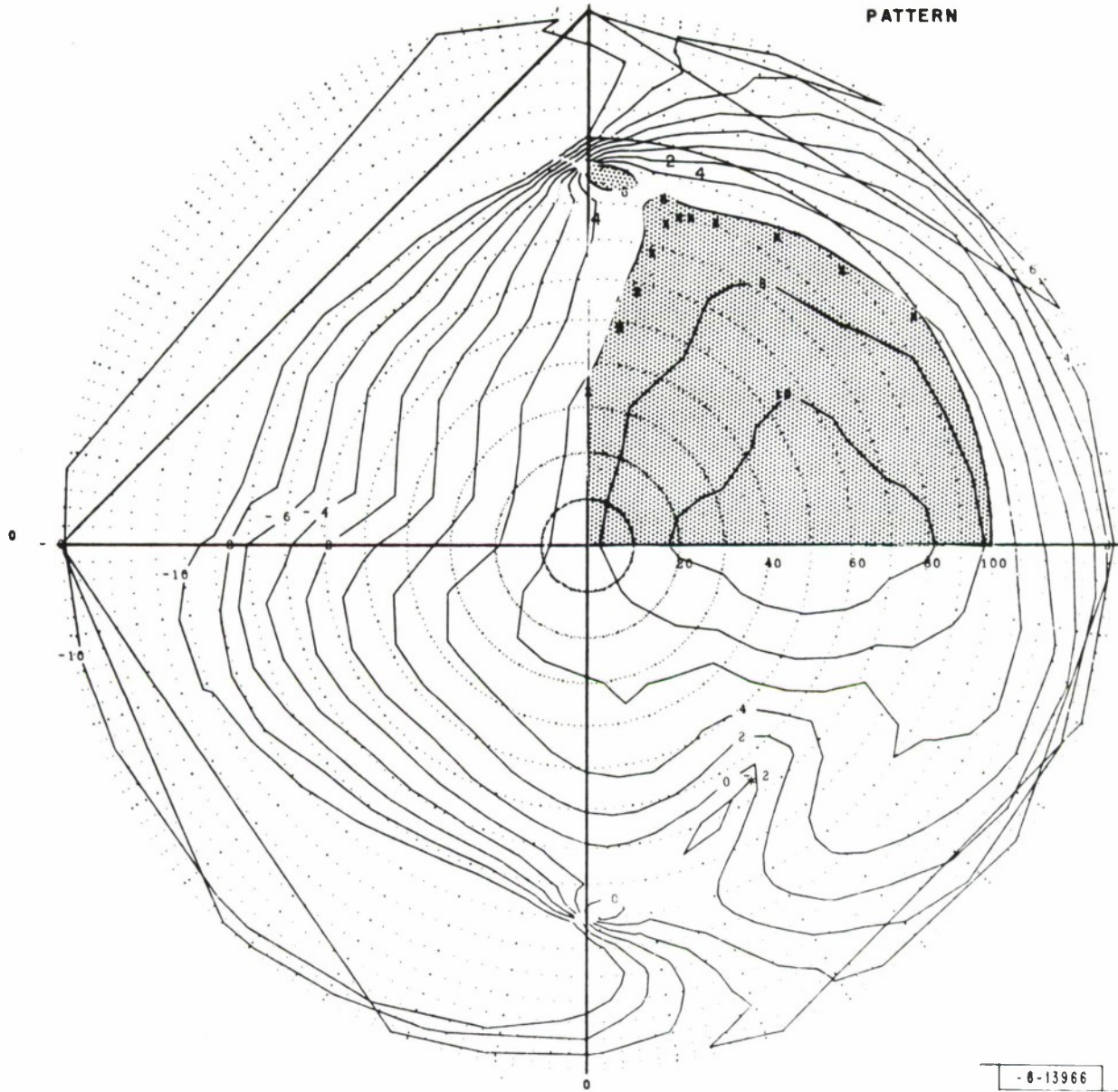
Fig. 3. Contour plot in the (\theta, \varphi) plane, 250 MHz, 50^\circ depression angle.
