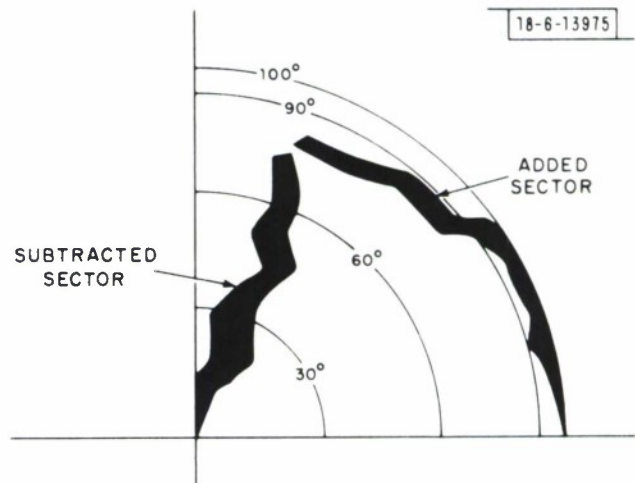
Fig. 12. Change in coverage with change in depression angle from 50^\circ - 60^\circ , 400 MHz.
