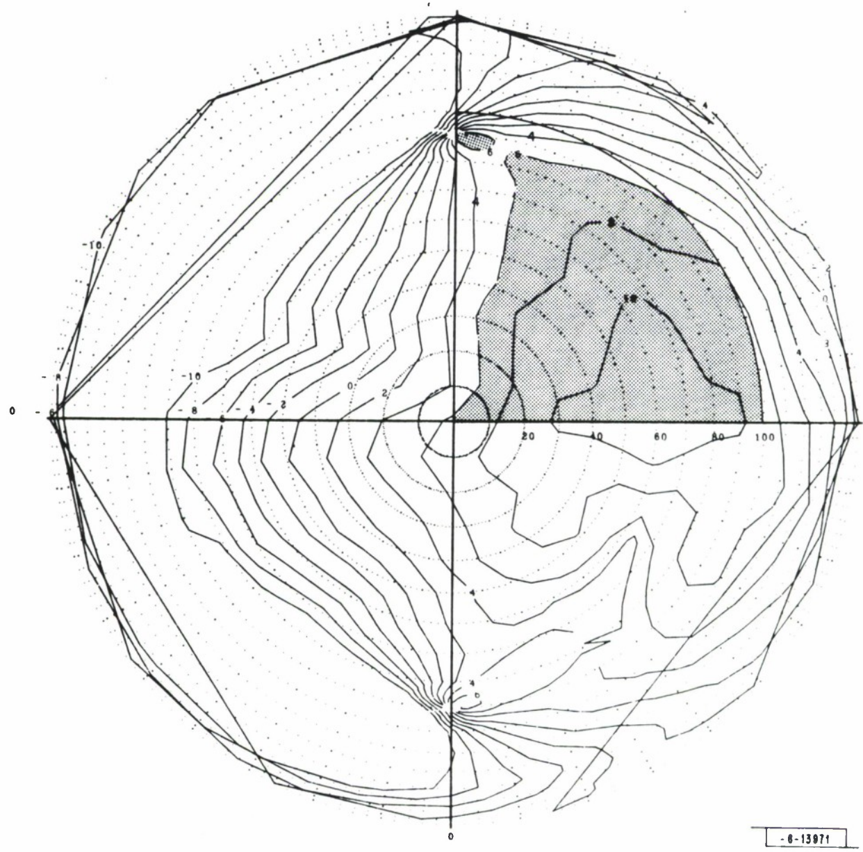
Fig. 8. Contour plot in the (\theta, \phi) plane, 300 MHz, 60^\circ depression angle.
