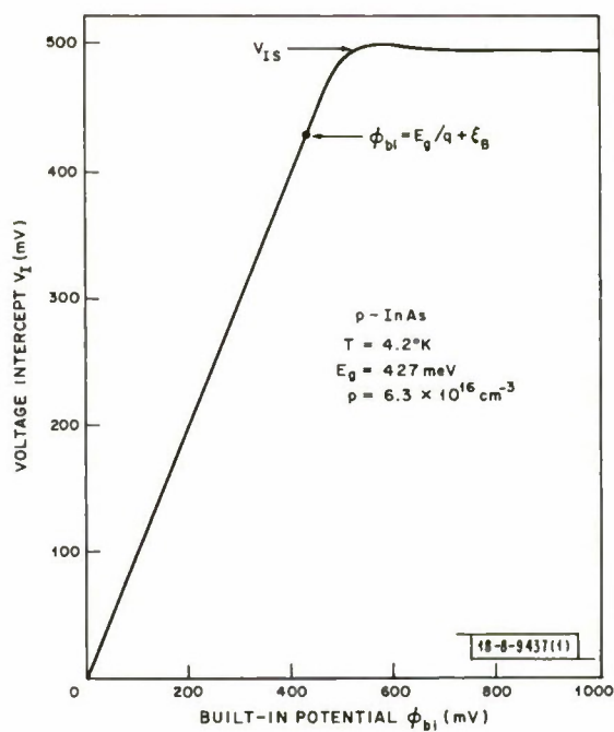
Fig. III-2. Calculated variation of the C^{-2} -V voltage intercept V_I with built-in potential for p-InAs illustrating saturation at V_{IS} .
