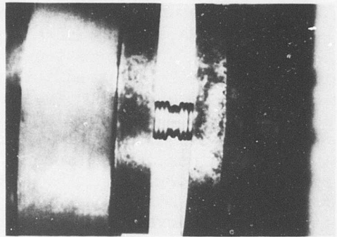
Figure 4. Development of Ring Buckles.
