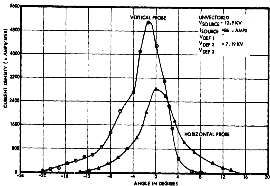
Figure 49. Run 710501, Vertical and Horizontal Current Densities for Unvectored Beam After 26 Hours
