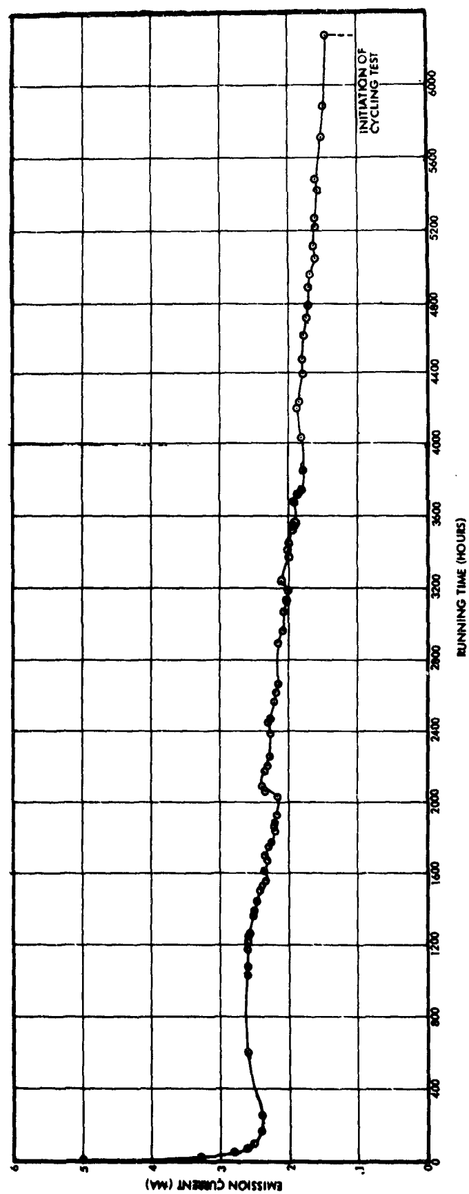
Figure 137. Single Neutralizer Life Test Performance Data
