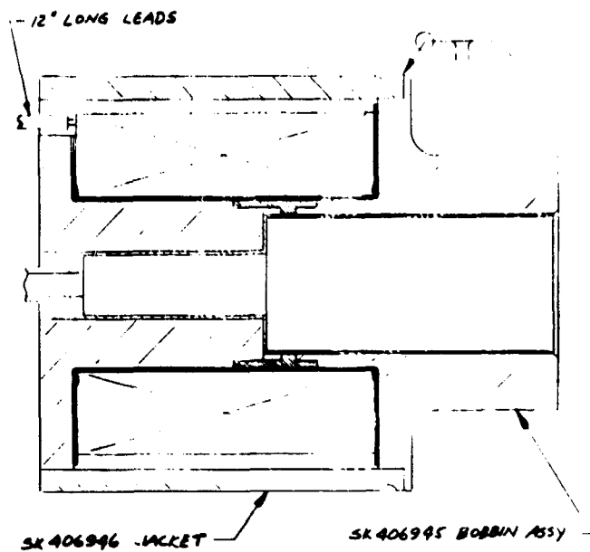
Figure 116. Solenoid Assembly
