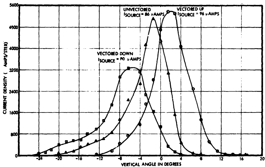
Figure 48. Run 710501, Vertical Vectoring Data at 26 Hours
