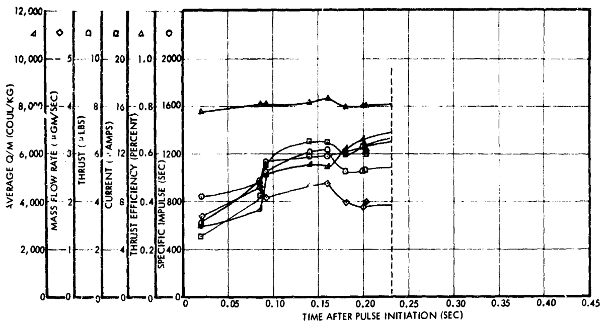
Figure 98. On-Time Profile of Time-of-Flight Parameters at V_N = 14.7 kv, 0.95 in. Hg, 0.6 second total period, 0.23 second on time
