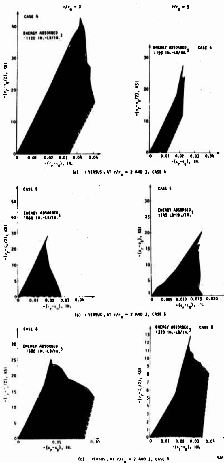
FIGURE 4-7. SHEAR STRESS/STRAIN CURVES AT r/r_0 = 2 AND r/r_0 = 3 FOR CASES 4, 5 AND 8
