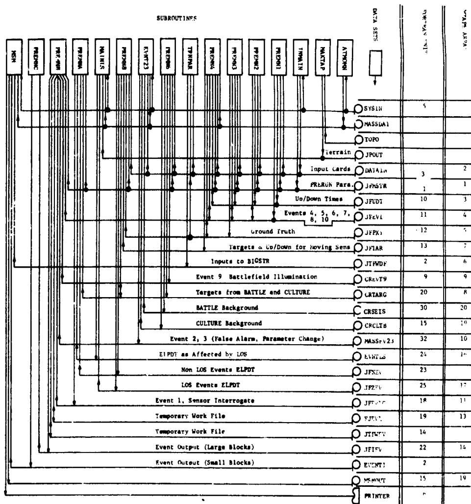
FIGURE 6.1-2 SUBROUTINE/DATA SET LINKAGES
