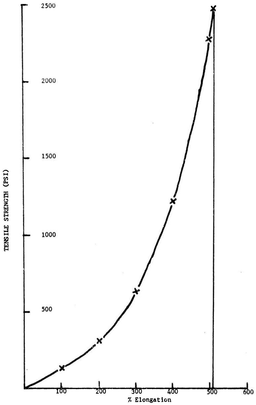
FIGURE 6 TOUGHNESS CURVE FOR NATURAL RUBBER OUTER SKIN
