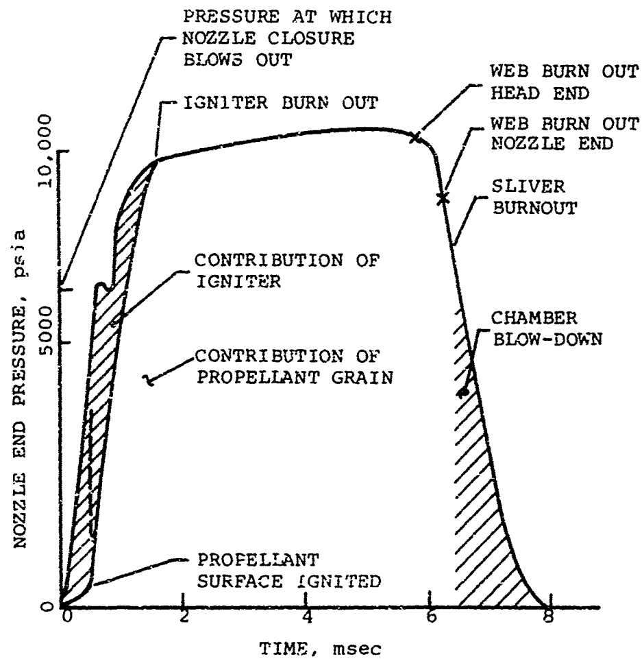
Fig. 1 Events that occur during the operation of an impulsive thruster (representative of Hit type of application),
