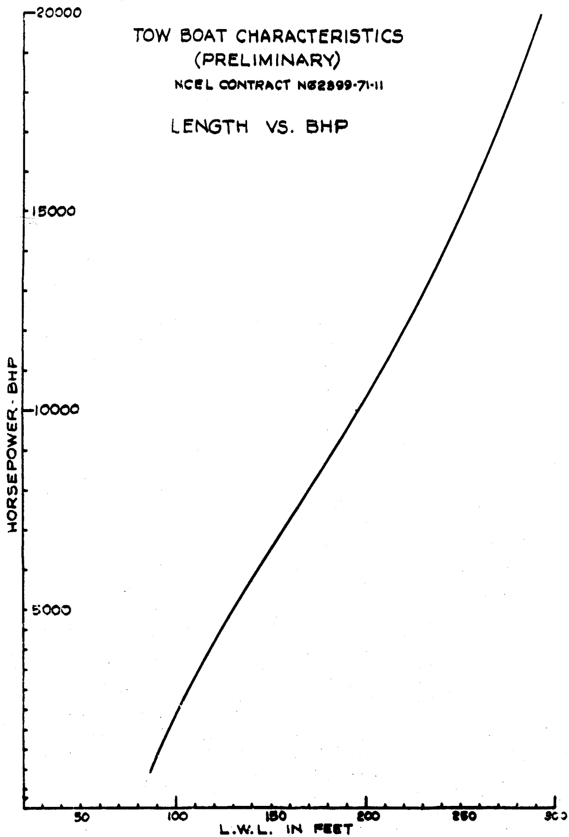
HP VS LENGTH FOR TUGS CONSIDERED FIGURE 1-14H
