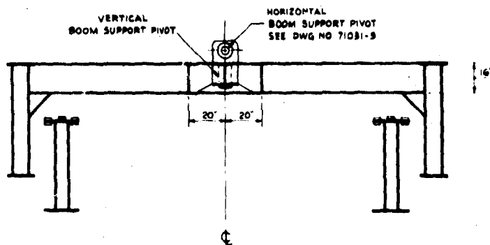
SECT 2-C
