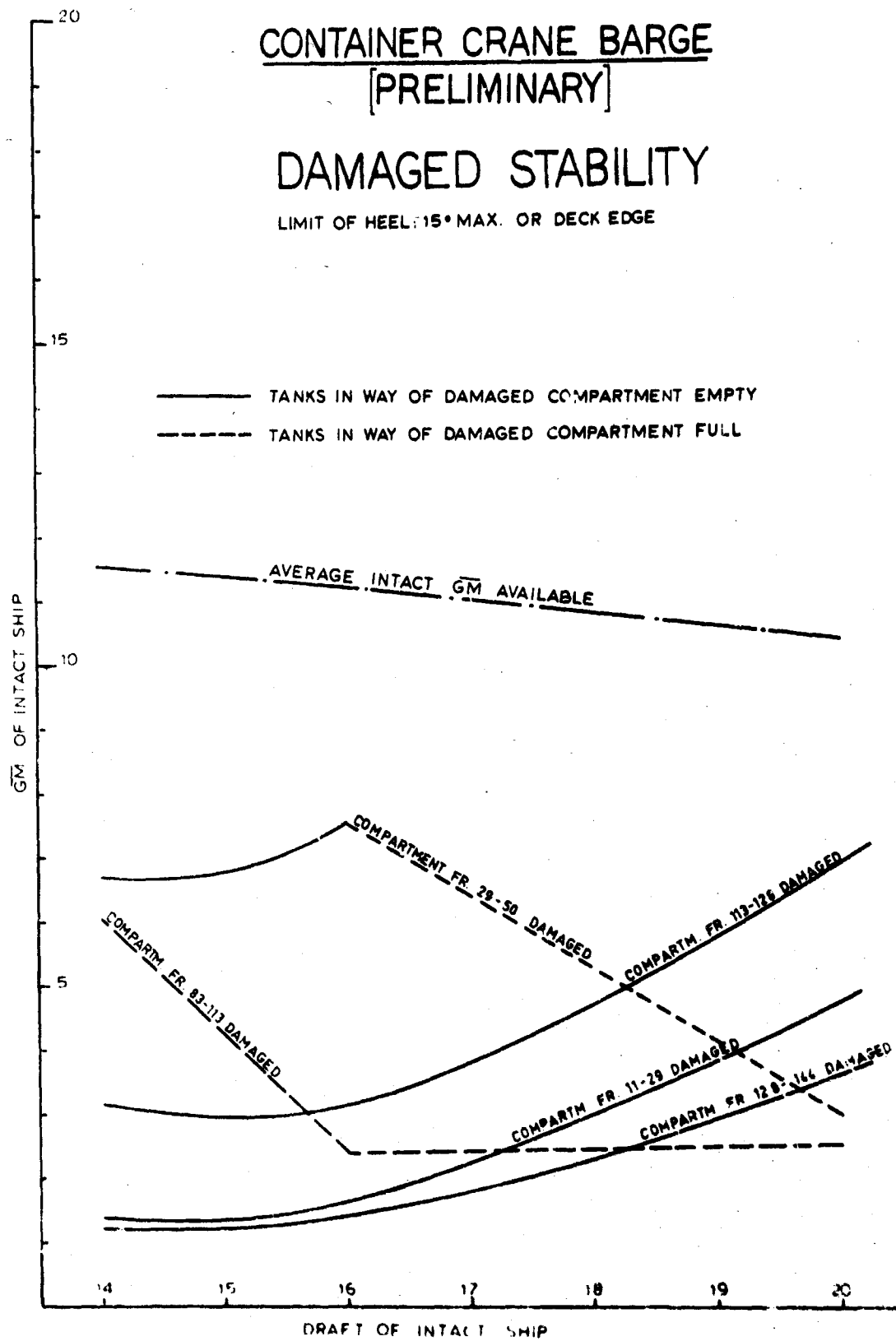
DAMAGED STABILITY FIGURE 1-4
