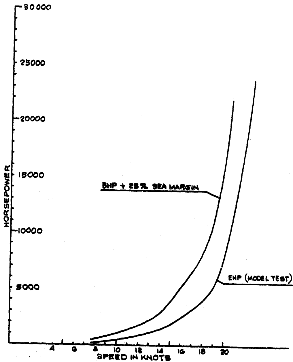
SPEED VS HP - TUG FOR 16 KNOT TOWING FIGURE 1-14A
