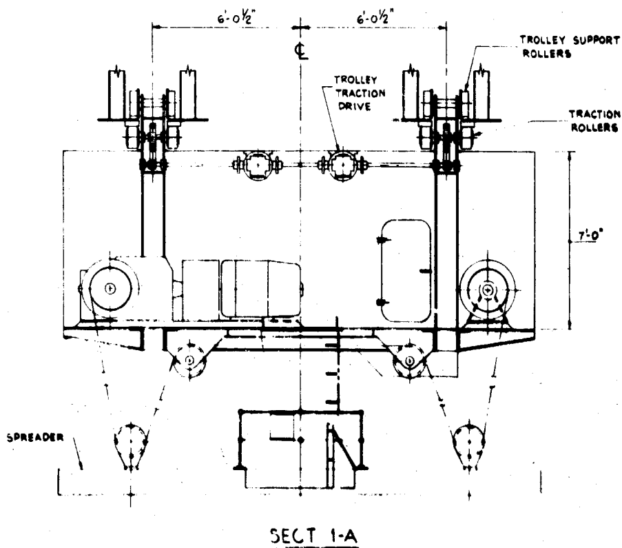
FIGURE 71031-4. BARGE CRANE CONCEPT BOOM CRANE ARRANGEMENT (SCALE 3/8" = 1'0"; DWG. NO. 7103-4)
