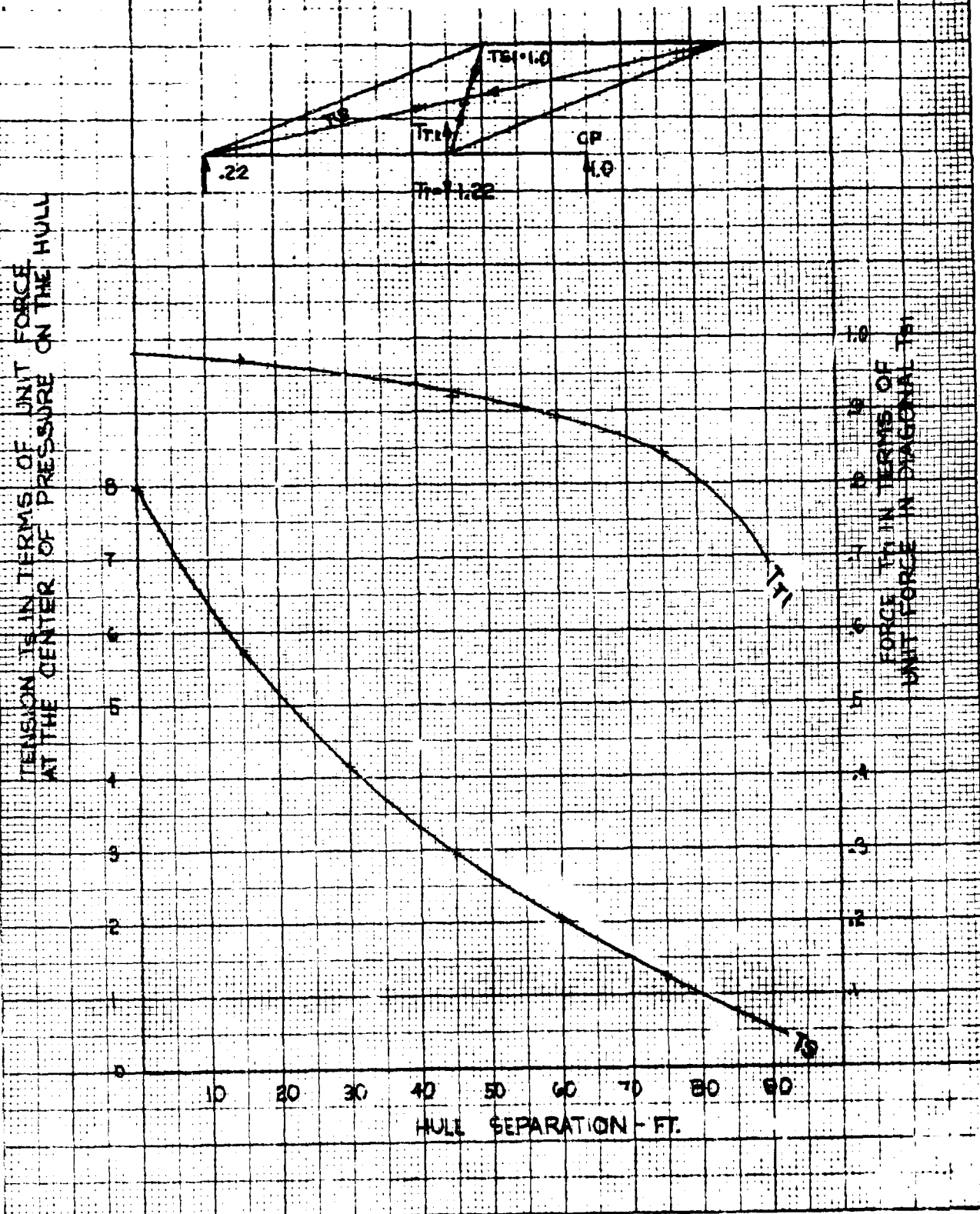
DIAGONAL TENSIONS FIGURE 2-9
