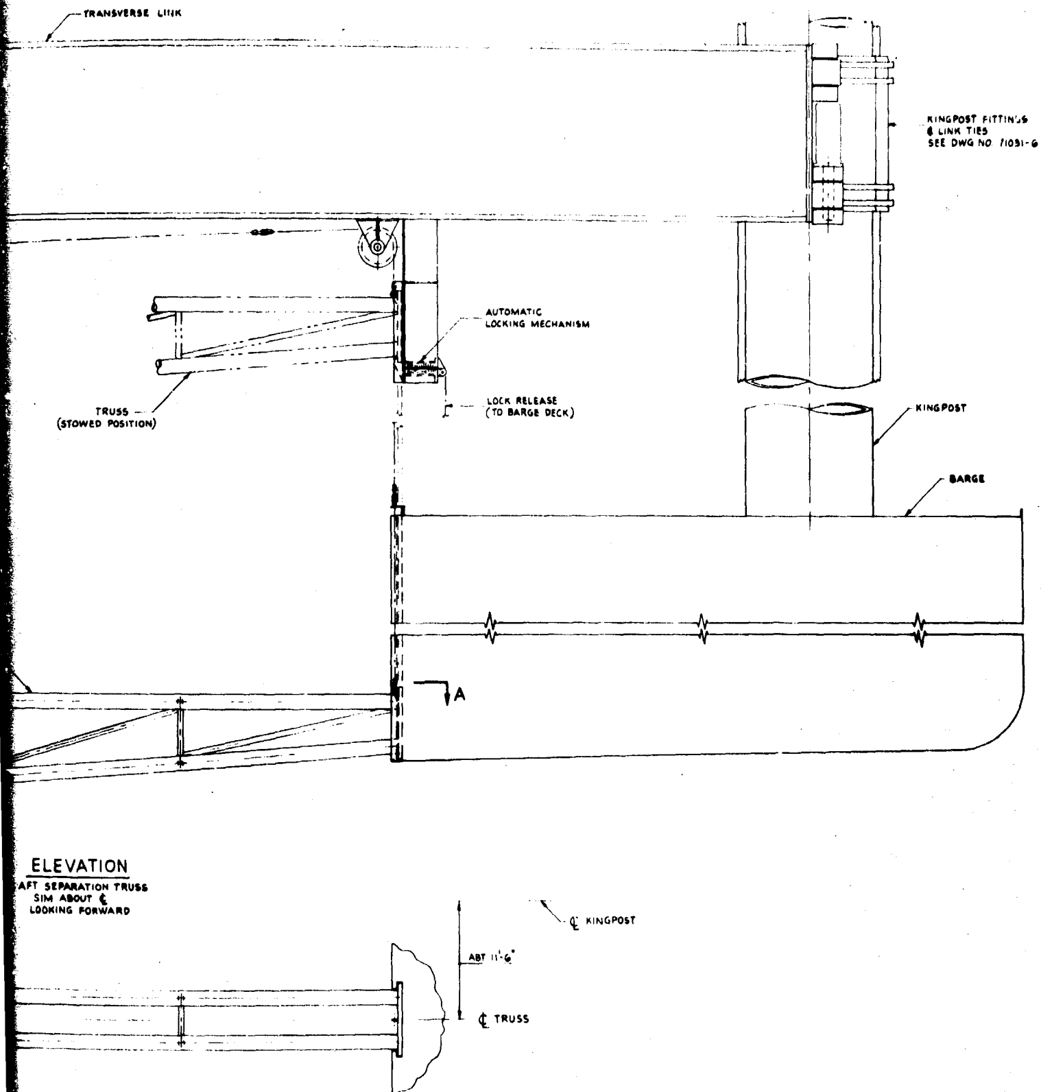
FIGURE 71031-8. BARGE CRANE DESIGN BOOM CRANE ARRANGEMENT (SCALE 3/8" = 1'0"; DWG. NO. 71031-8)
