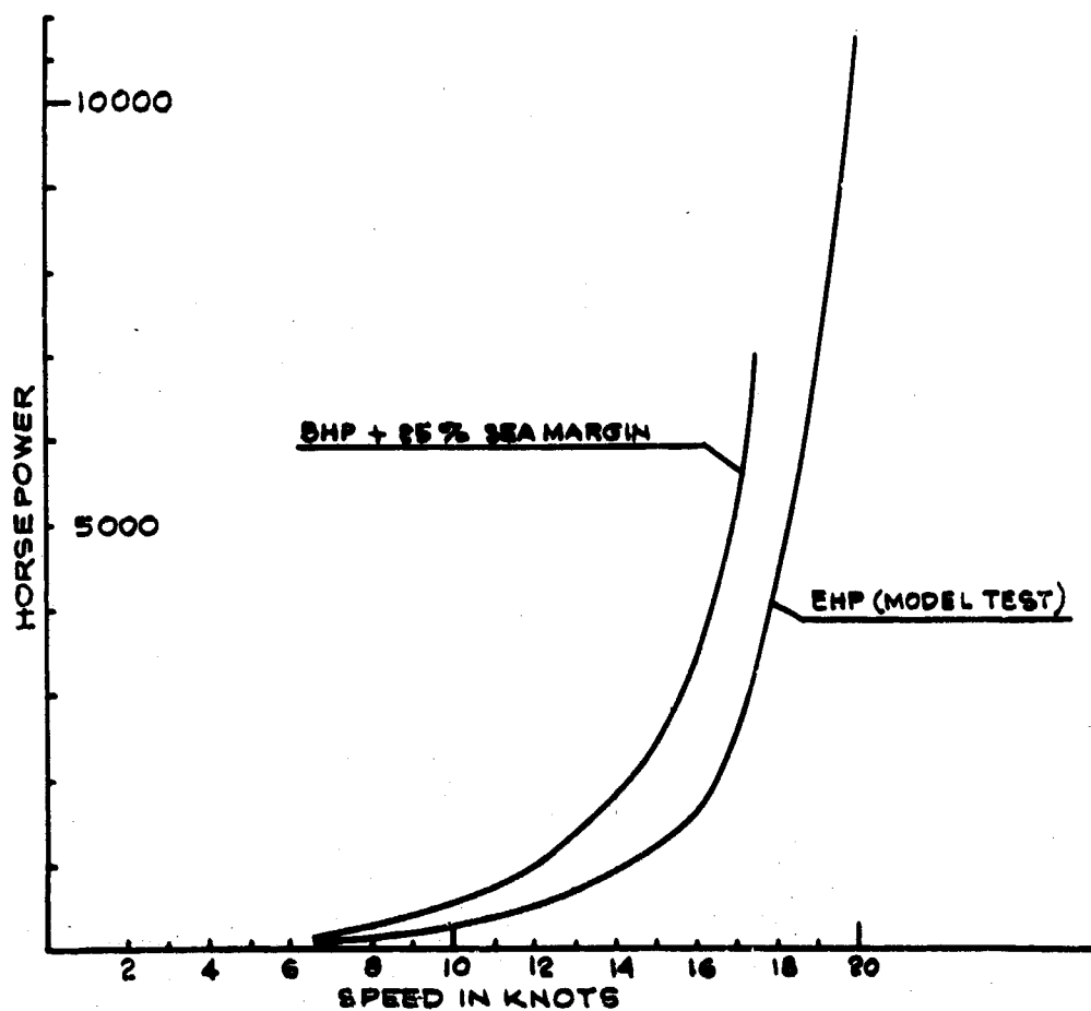
SPEED VS HP - TUG FOR 14 KNOT TOWING FIGURE 1-14C
