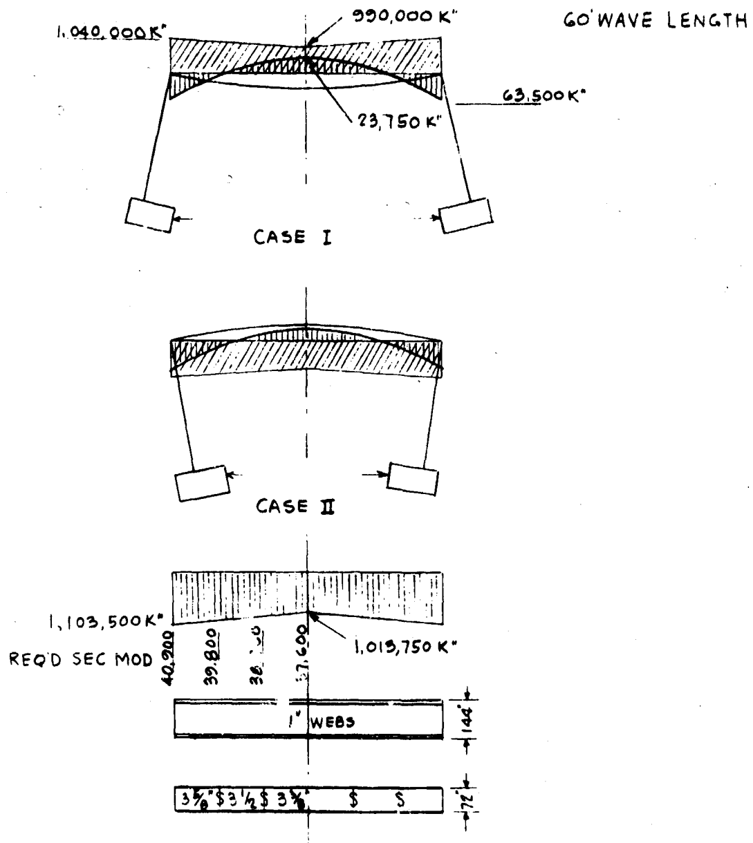
BENDING MOMENTS FOR 60' WAVE LENGTH
