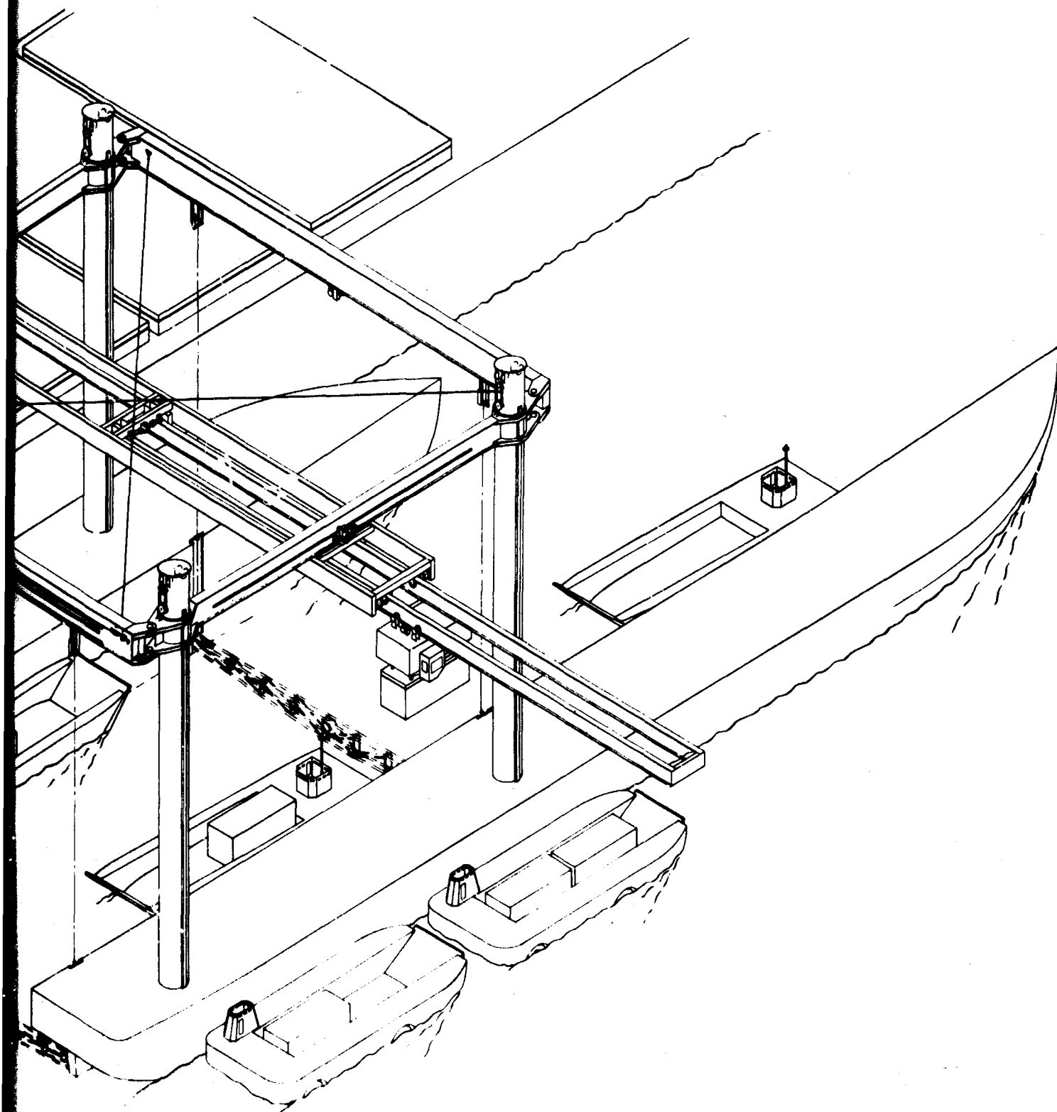
FIGURE 71031-9. BARGE CRANE DESIGN BOOM CRANE ARRANGEMENT (SCALE 1/16" = 1'0"; DWG. NO. 71031-9)
