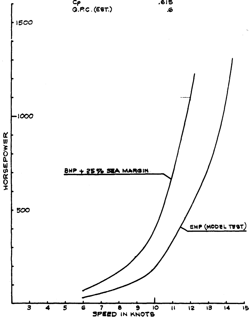
SPEED VS HP - TUG FOR 12 KNOT TOWING FIGURE 1-14E
