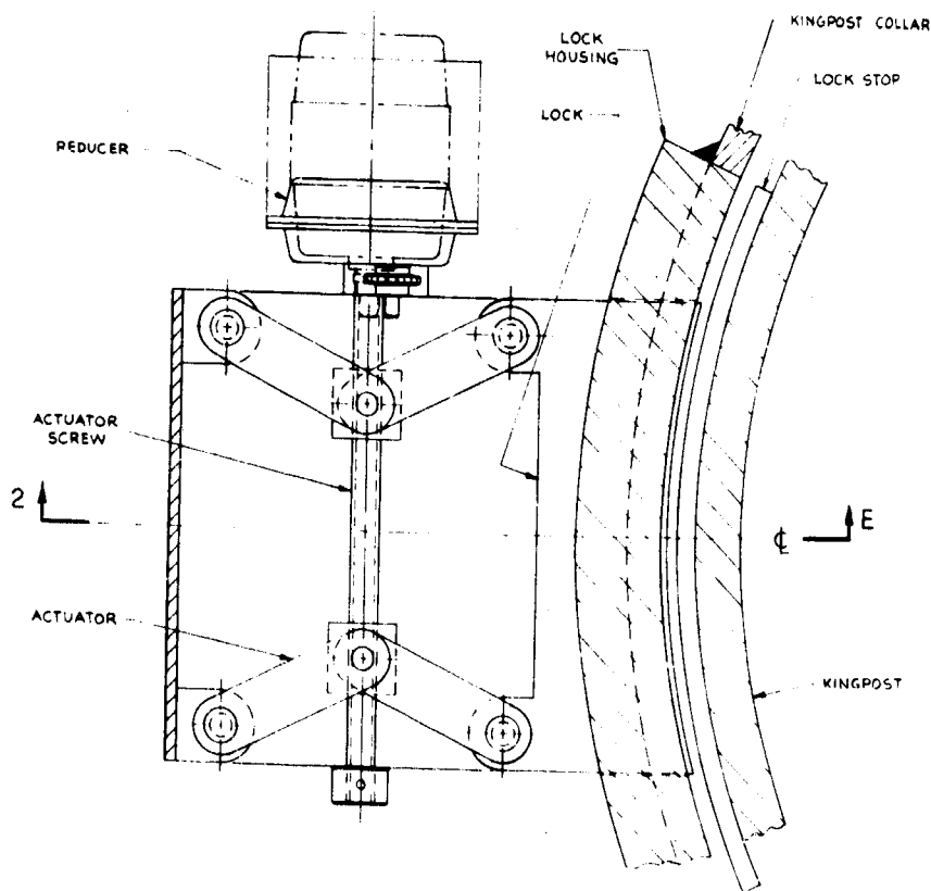
SECT 2-D VERTICAL LOCK ACTUATORS SCALE: 3"=1'-0"
