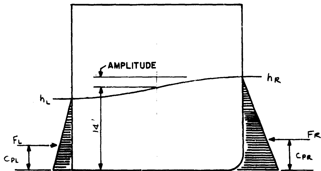
WAVE POSITION FOR WAVE LENGTHS GREATER THAN 60 FEET FIGURE 2-11
