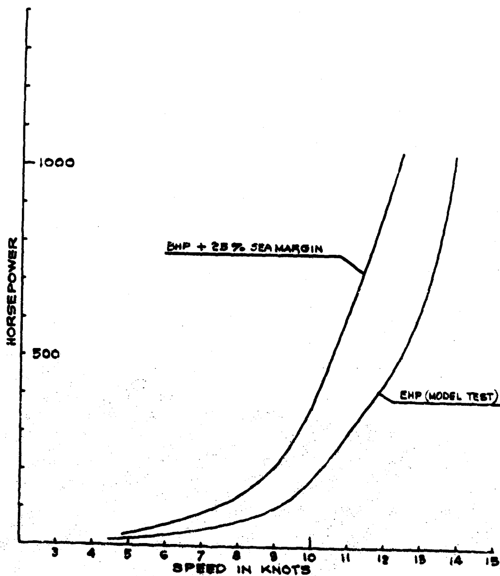
SPEED VS HP - TUG FOR 10 KNOT TOWING FIGURE 1-14C
