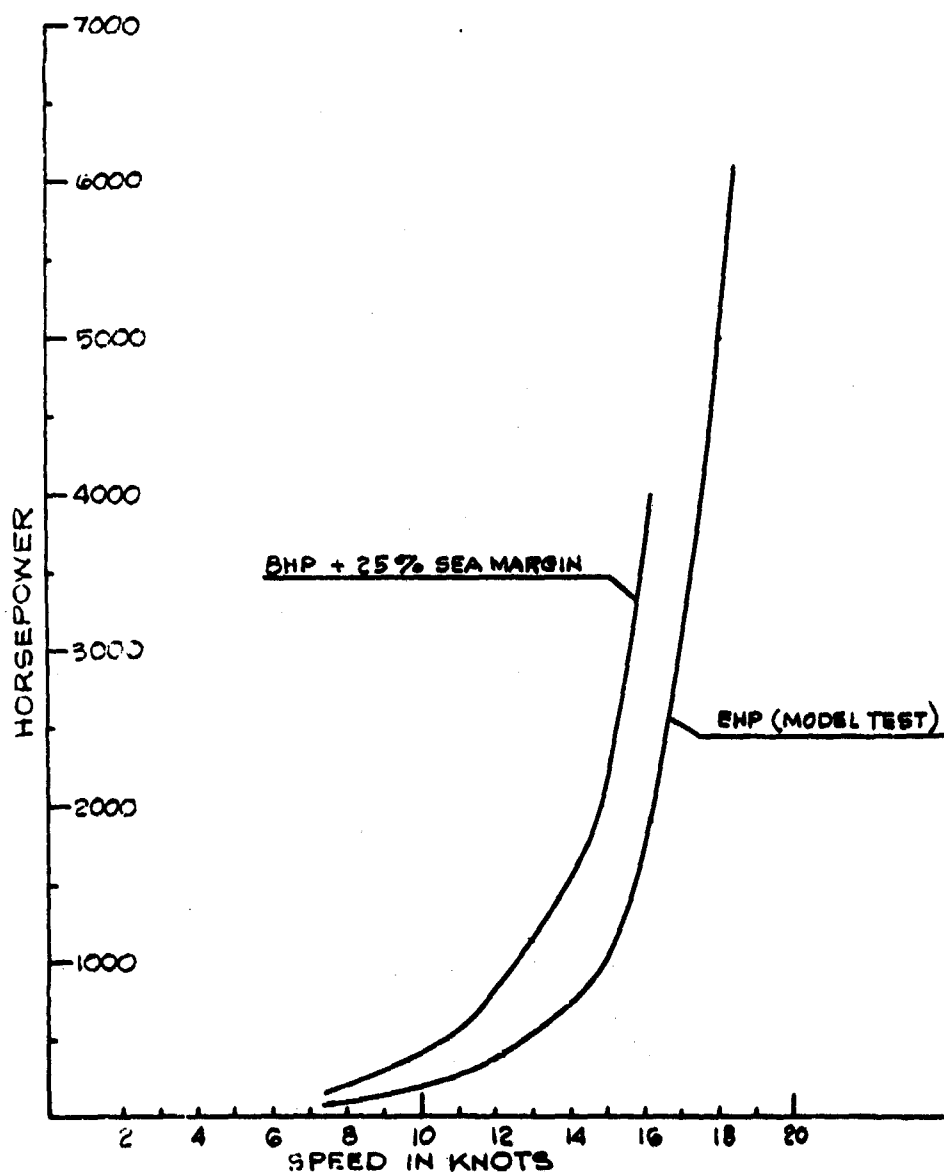
SPEED VS HP - TUG FOR 13 KNOT TOWING FIGURE 1-14D
