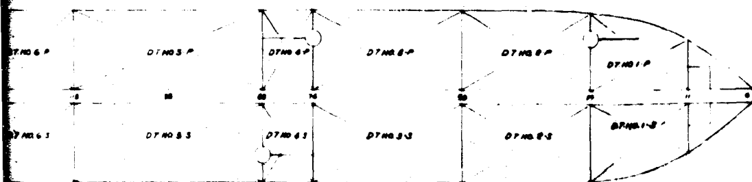
SECOND DECK 1/16" = 1'-0"
