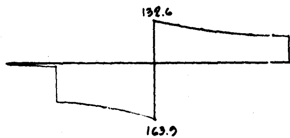
SHEAR DIAGRAM (ONE MEMBER)
