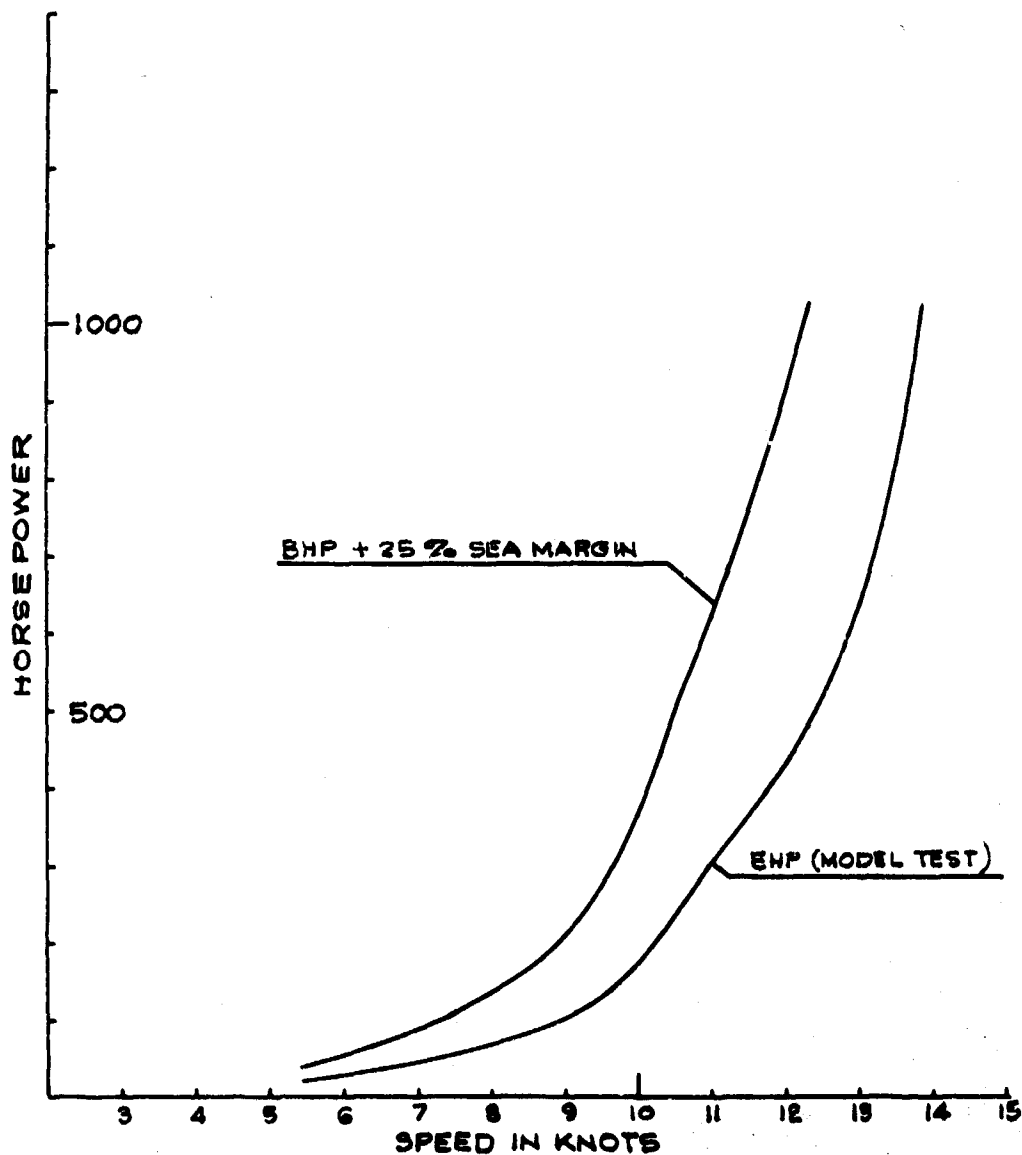
SPEED VS HP - TUG FOR 11 KNOT TOWING FIGURE 1-14F
