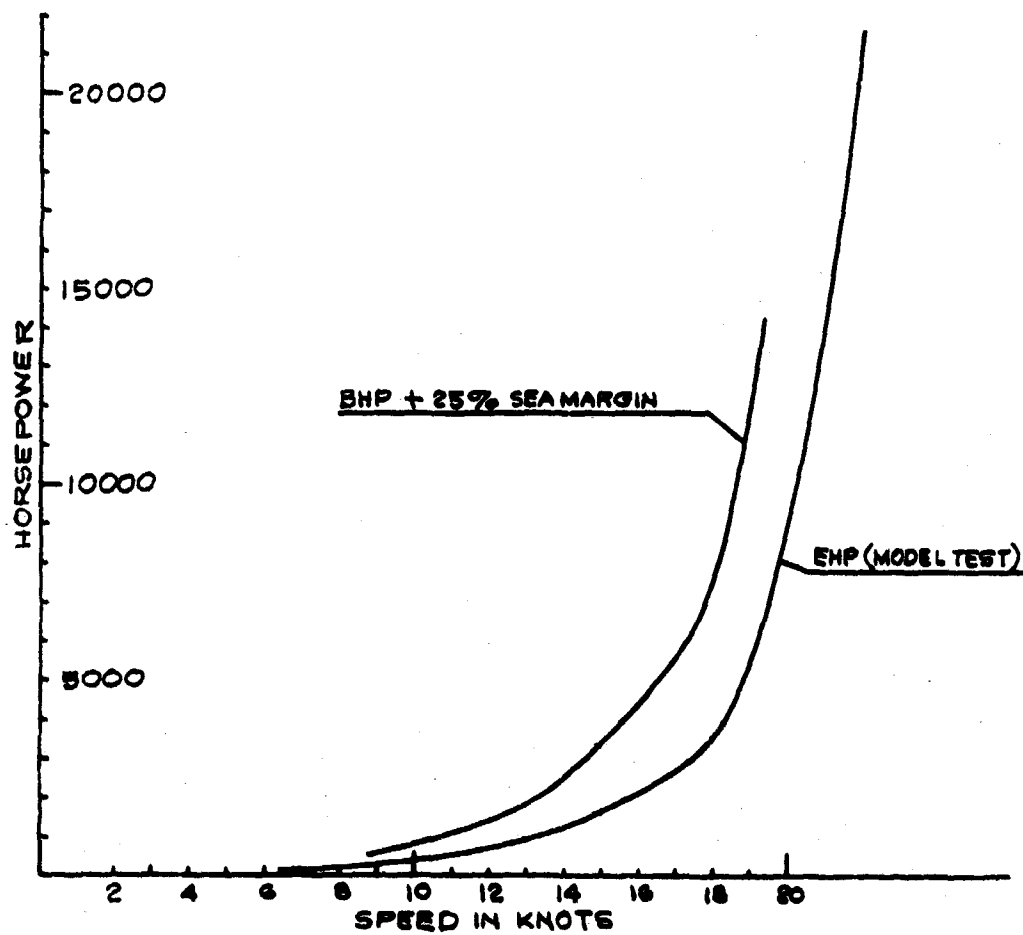
SPEED VS HP - TUG FOR 15 KNOT TOWING FIGURE 1-14B
