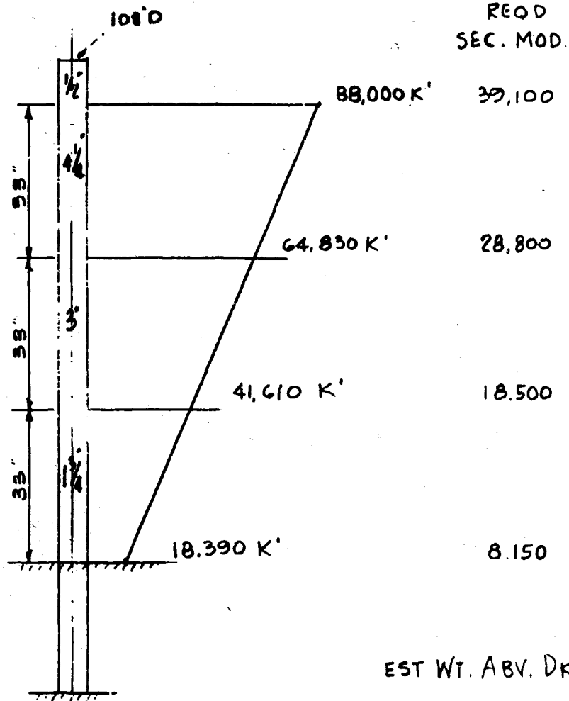
MOMENT DIAGRAM
