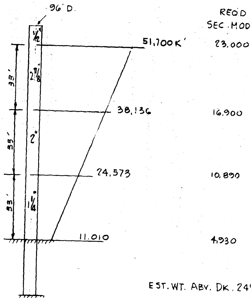
MOMENT DIAGRAM
