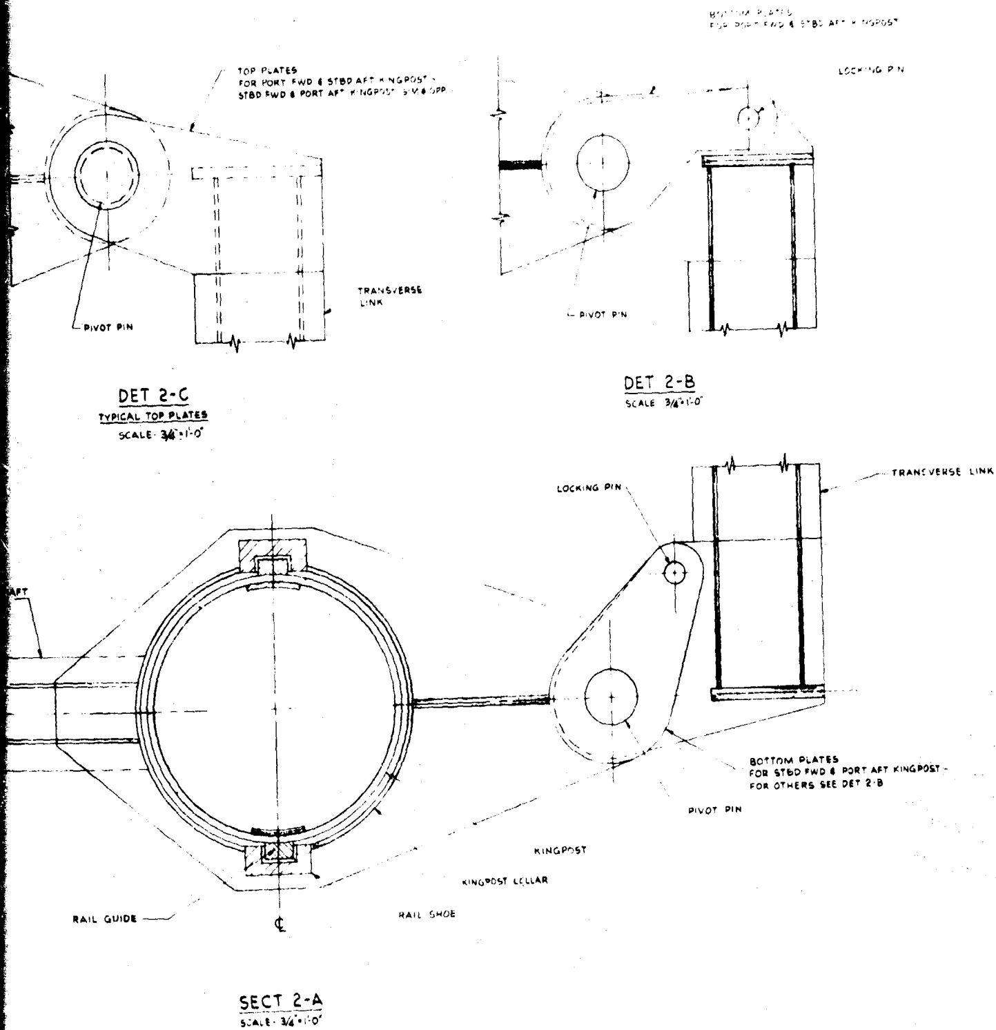
FIGURE 71031-6. BARGE CRANE DESIGN (2 OF 2) BOOM CRANE ARRANGEMENT (SCALE AS NOTED; DWG. NO. 71031-6)
