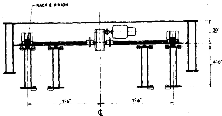
SECT 2-D
