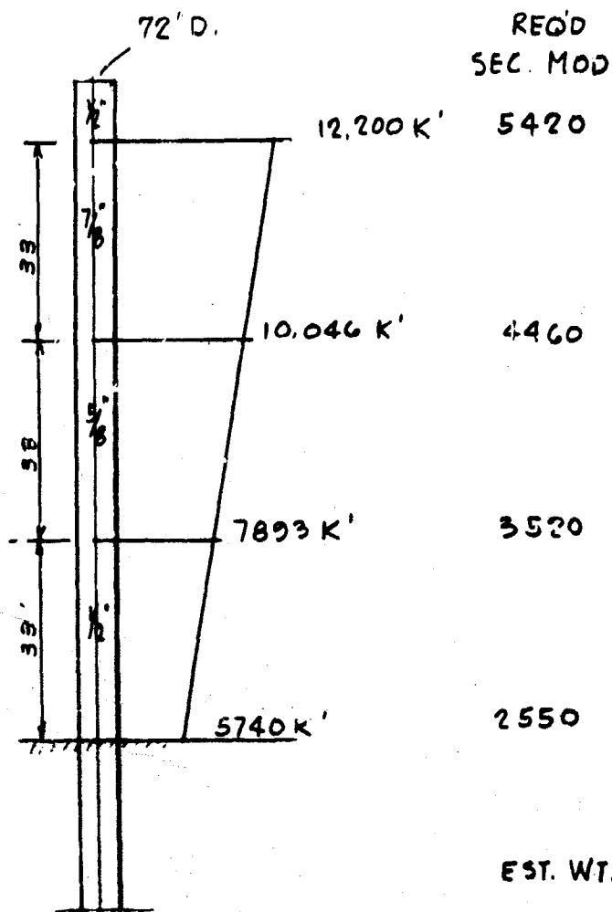
MOMENT DIAGRAM
