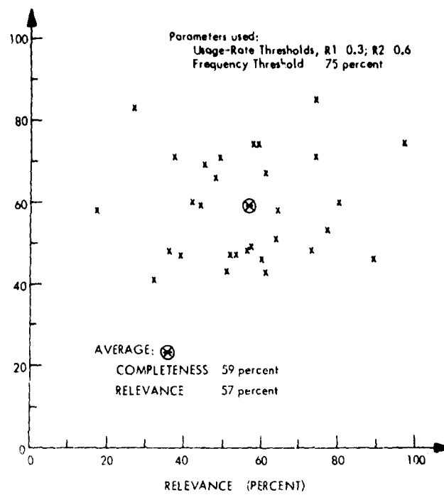
Fig. 16 Results of Method III for 30 Documents
