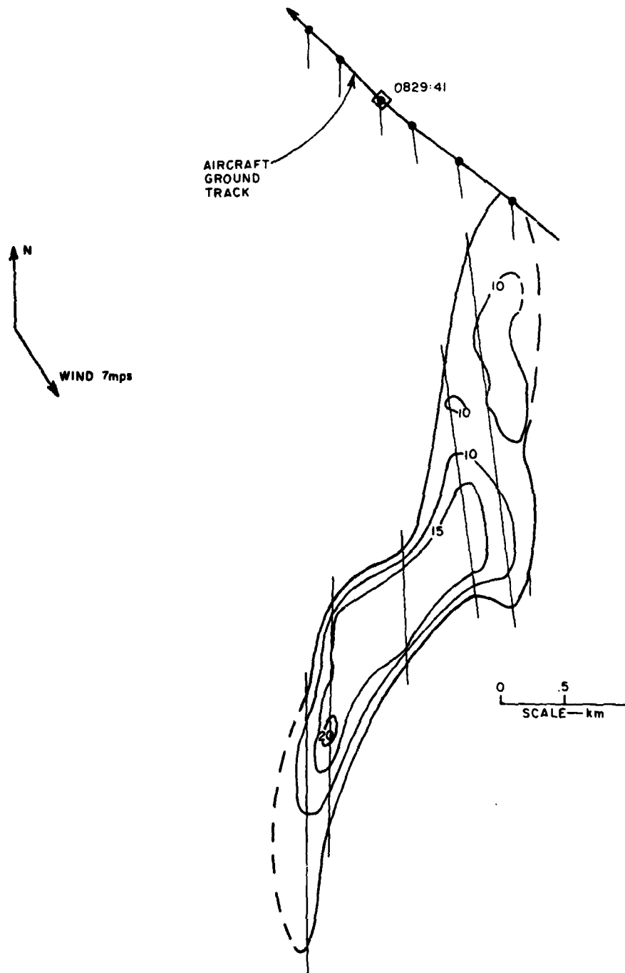
FIG.10 RELATIVE DENSITY VARIATION OF THE SUB-VISIBLE CLOUD RUN 5 12.8km FROM GZ IN DB ABOVE BACKGROUND
