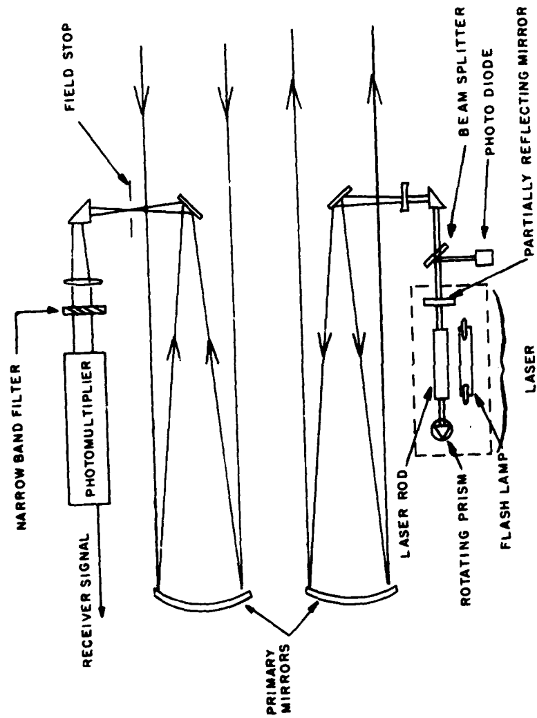
FIG. 3 MARK V LIDAR OPTICAL DIAGRAM
