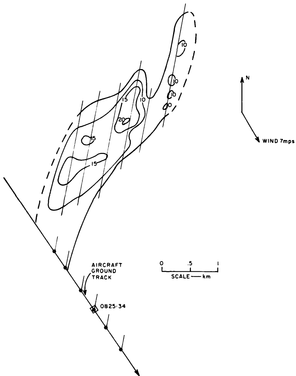
FIG 9 RELATIVE DENSITY VARIATIONS OF THE SUB-VISIBLE CLOUD RUN 4 11.5 km FROM GZ IN DB ABOVE BACKGROUND
