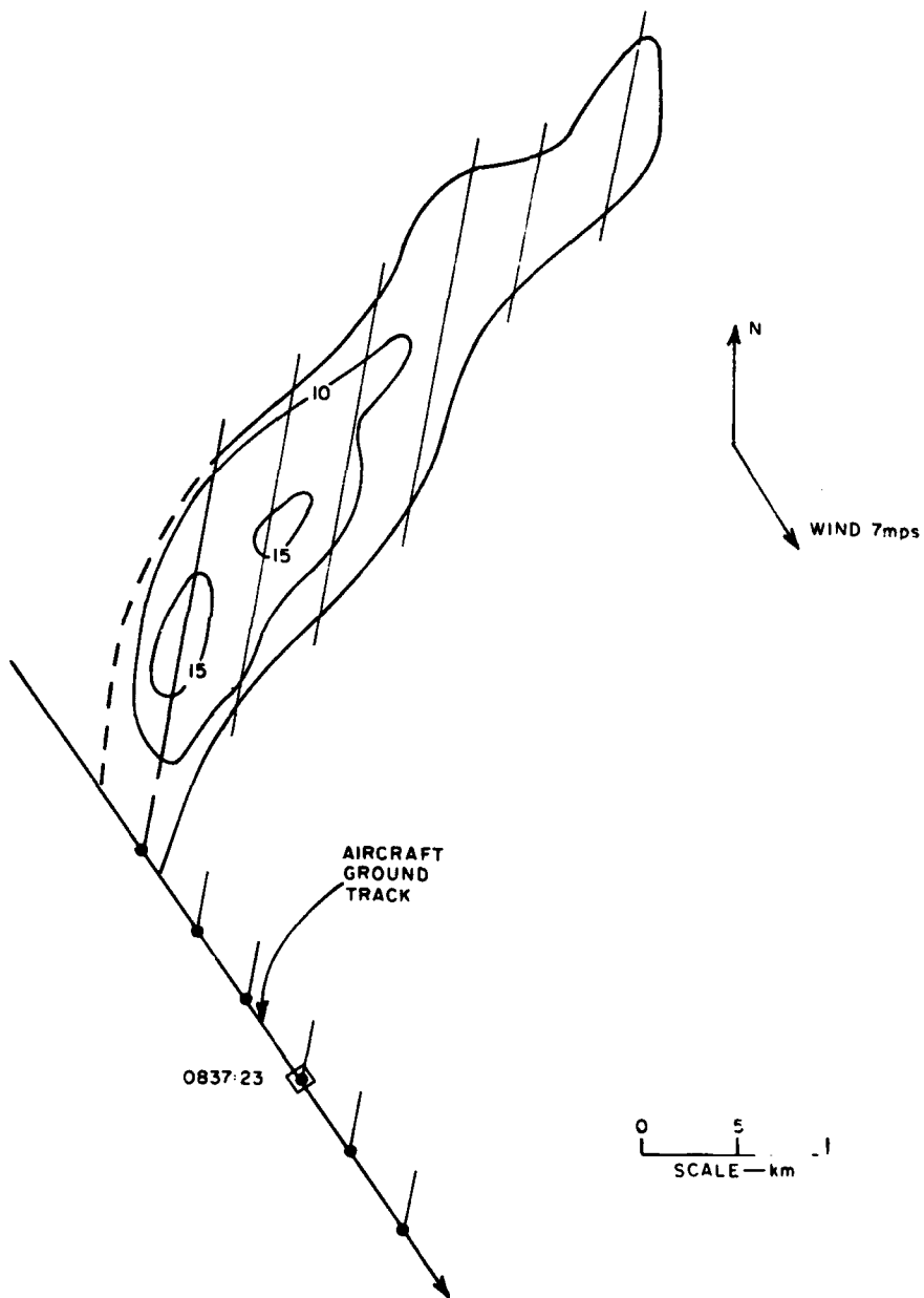
FIG II RELATIVE DENSITY VARIATION OF THE SUB-VISIBLE CLOUD RUN 6 15.6 km FROM GZ IN DB ABOVE BACKGROUND
