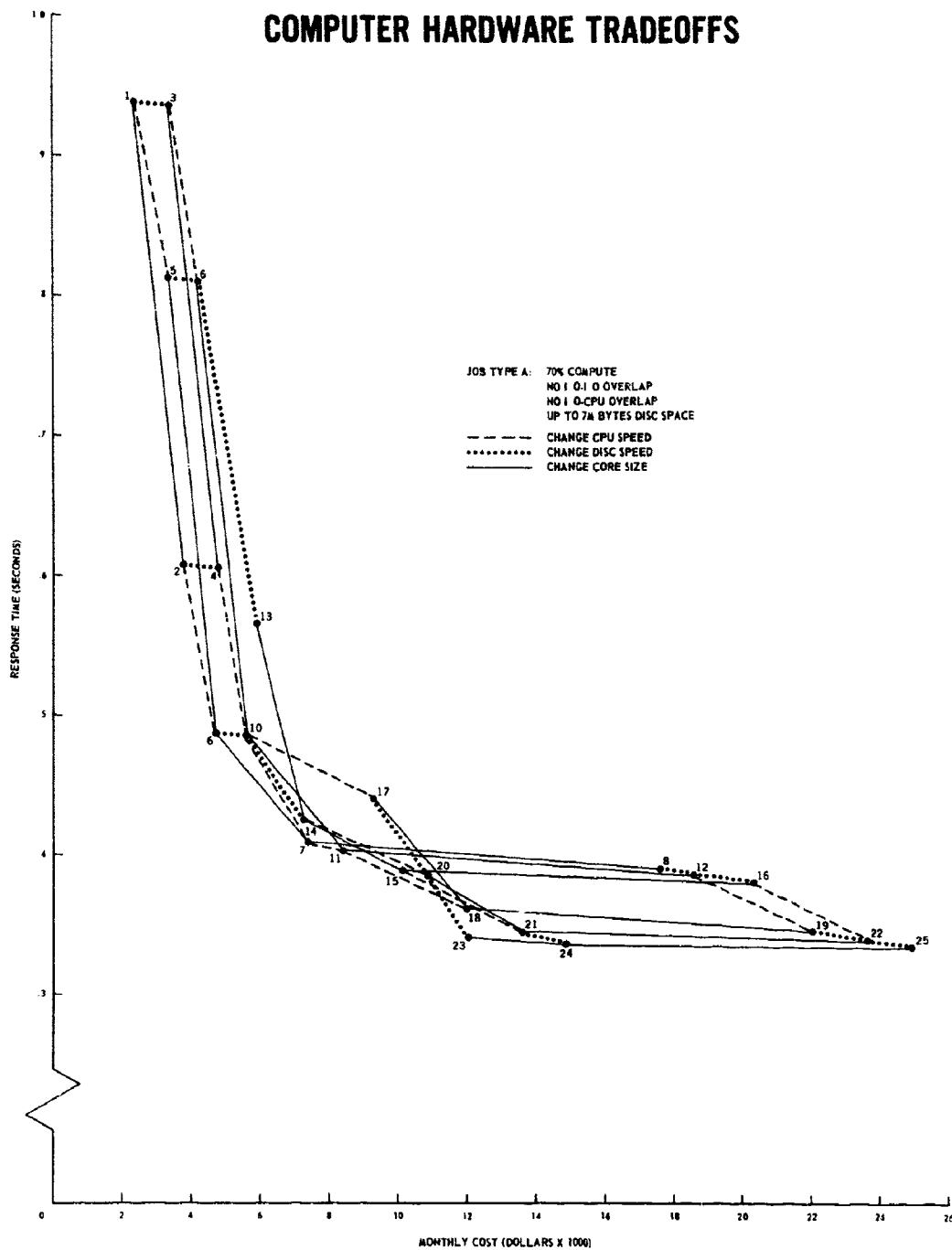
Figure 2-2. Computer Hardware Tradeoffs: Job Type A
