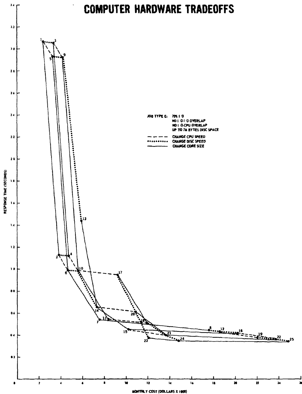
Figure 2-3. Computer Hardware Tradeoffs: Job Type B
