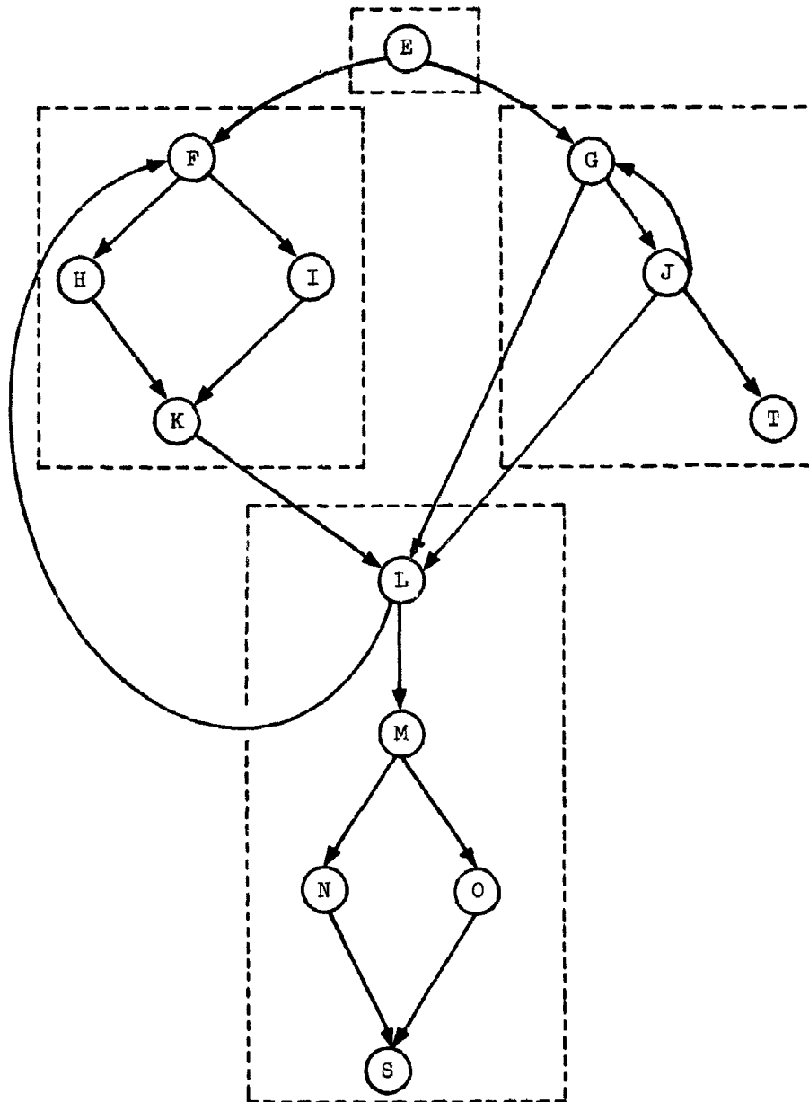
Figure 4-1. Program Control Flow Graph
