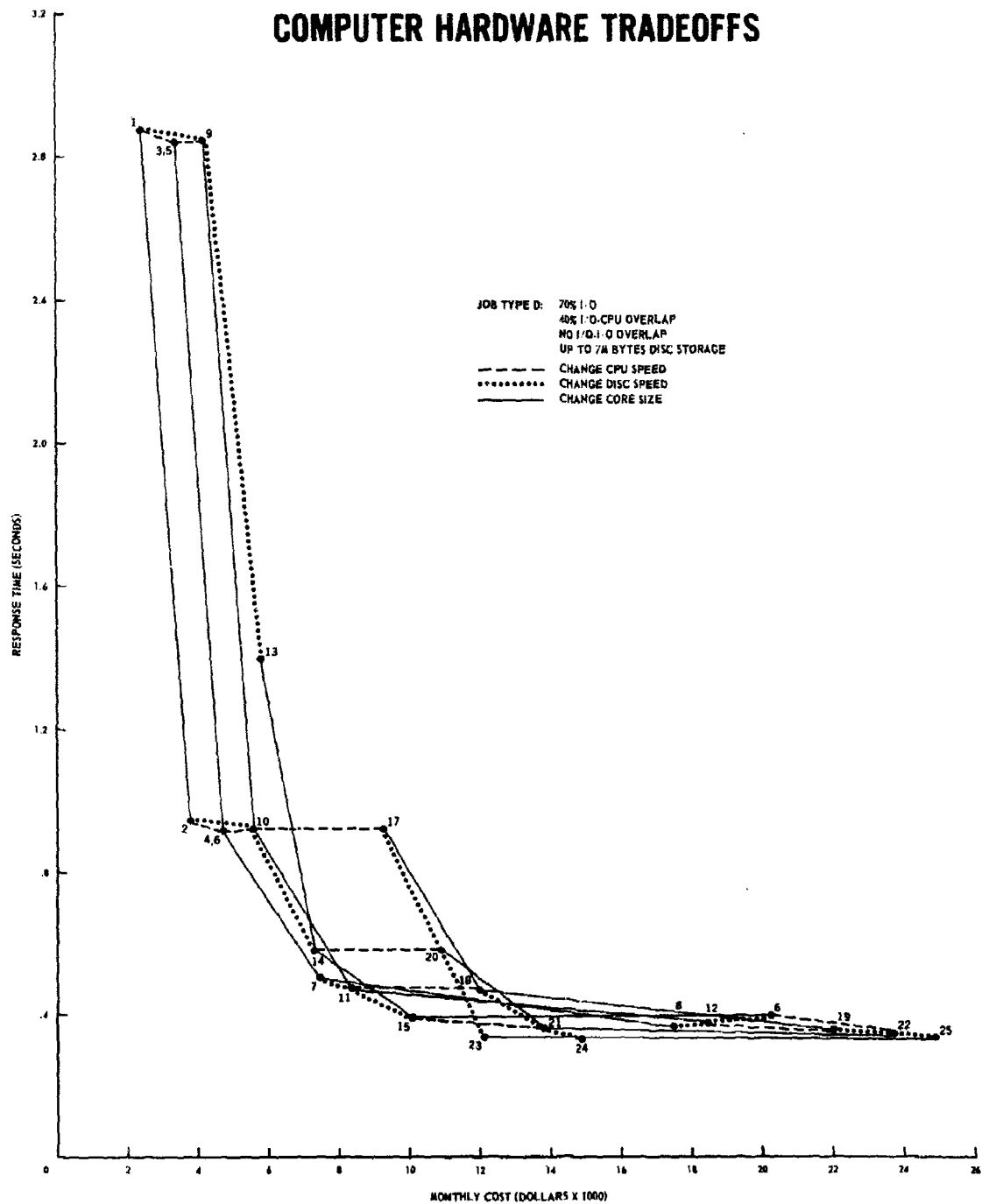
Figure 2-5. Computer Hardware Tradeoffs: Job Type D
