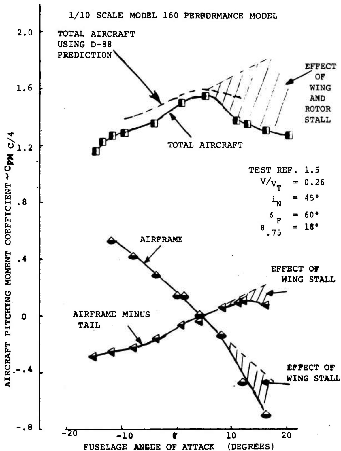
FIGURE 5.28: TOTAL AIRCRAFT LONGITUDINAL STABILITY CORRELATION - MID-TRANSITION
