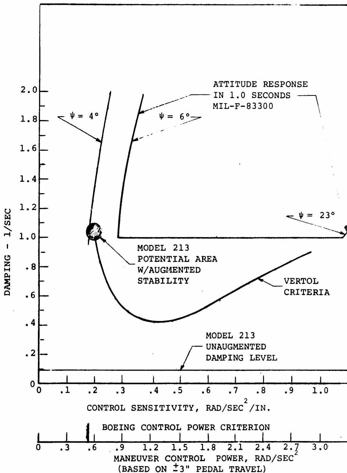
FIGURE 5.9. YAW CONTROLLABILITY IN HOVER
