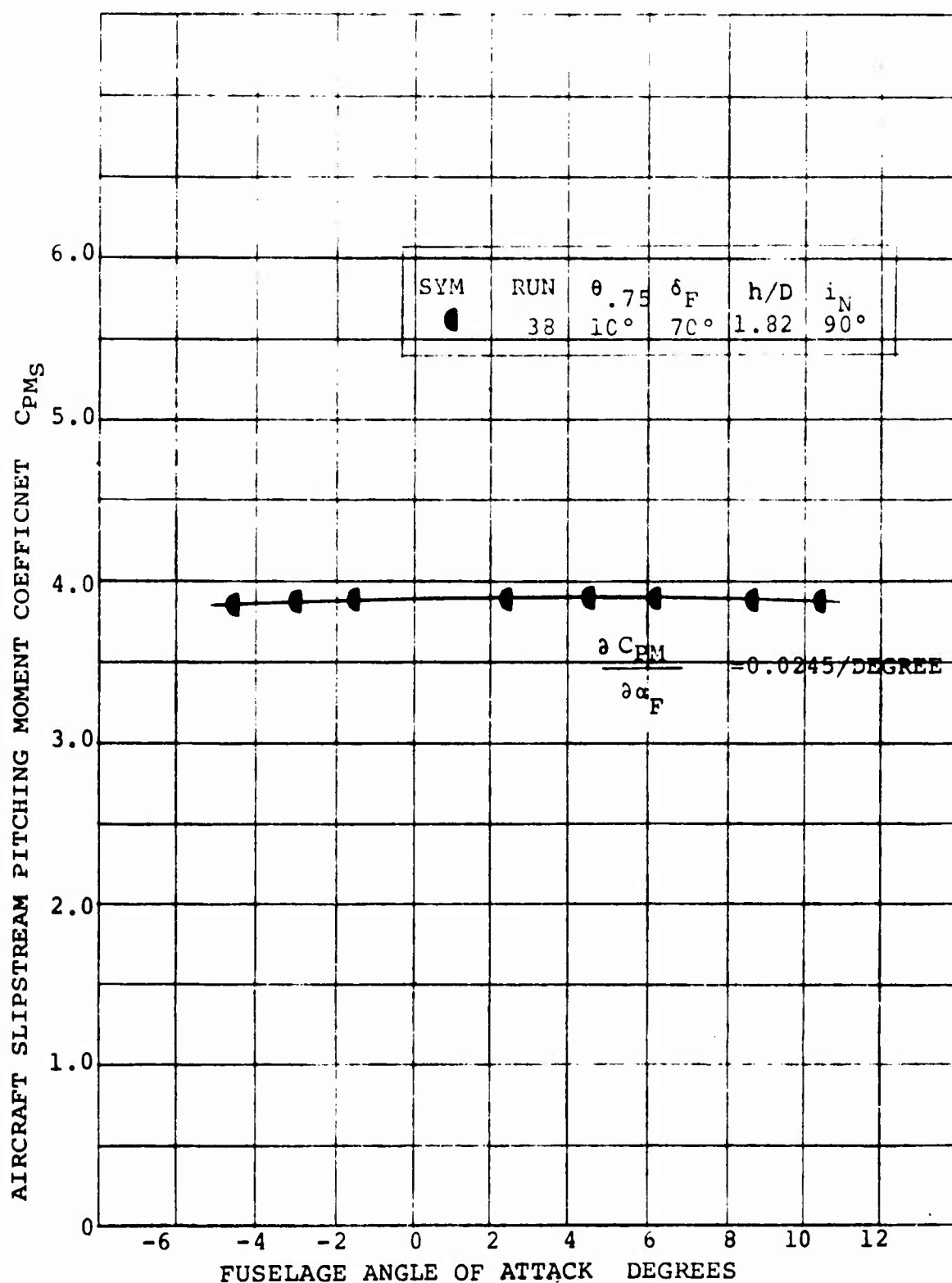
FIGURE 5.14: EFFECT OF ANGLE OF ATTACK ON AIRCRAFT PITCHING MOMENT IN THE NEAR HOVER MODE AT q = 4 PSF
