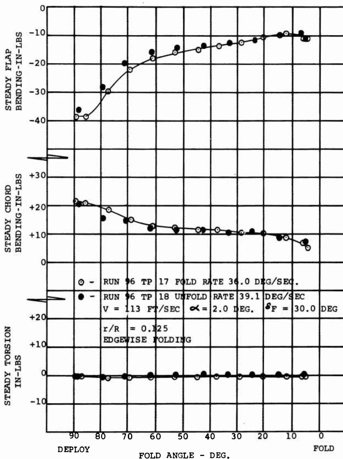
FIGURE 3.17 STEADY BLADE LOADS DURING DYNAMIC FOLD AND DEPLOYMENT, EDGEWISE FOLDING
