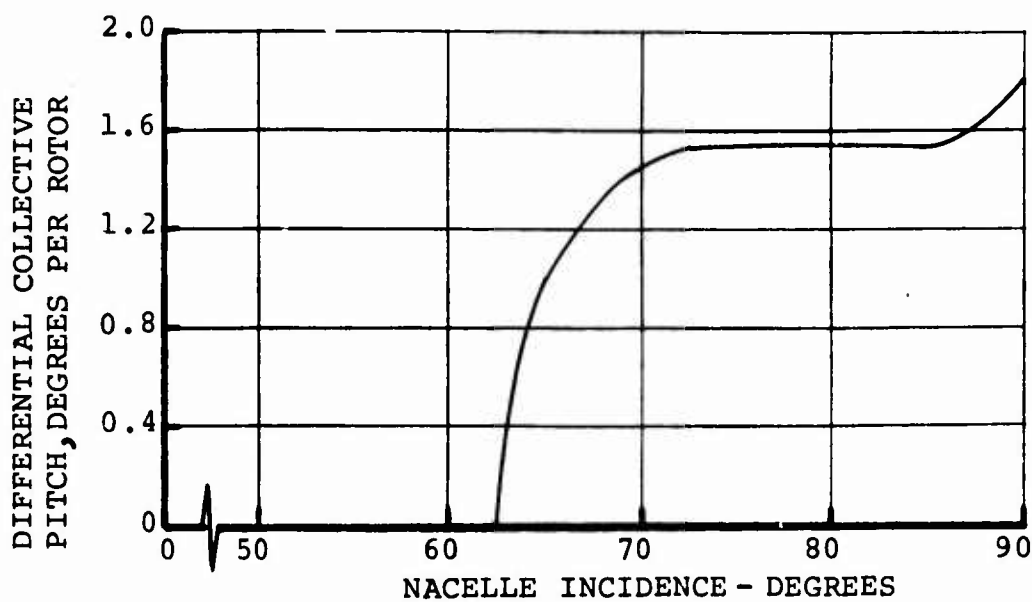
FIGURE 5.31: ROLL CONTROL PHASING THROUGH TRANSITION
