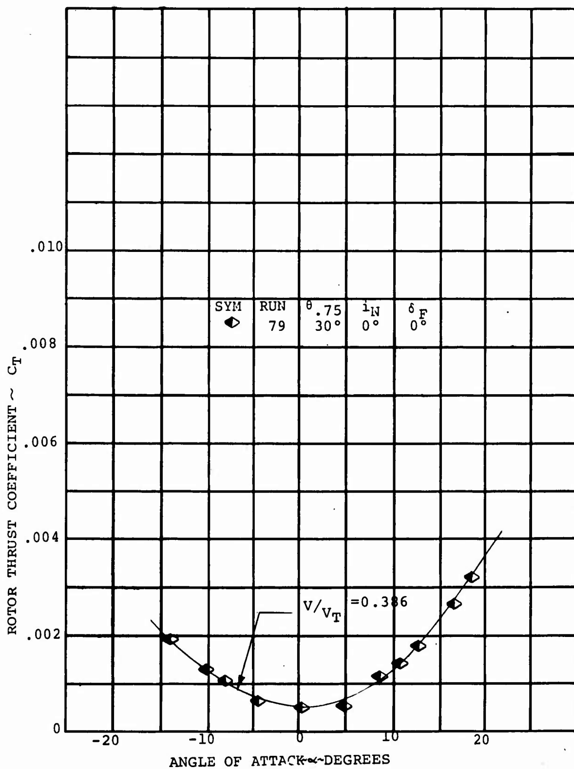
FIGURE 4.21: ROTOR THRUST/ANGLE OF ATTACK VARIATION IN CRUISE
