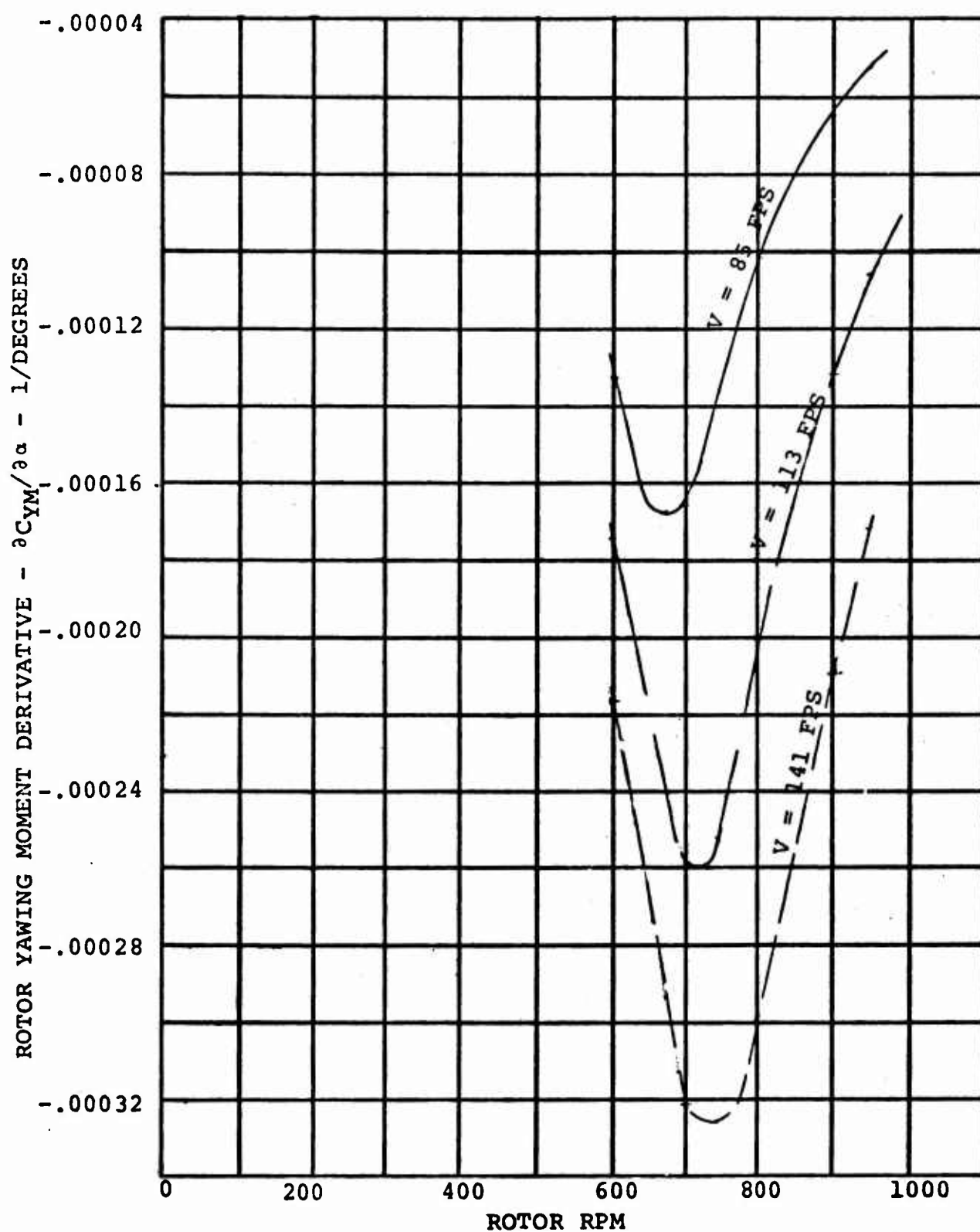
FIGURE 5.44. ROTOR YAWING MOMENT DERIVATIVE VARIATION WITH ROTOR RPM, \delta_F = 0.^\circ
