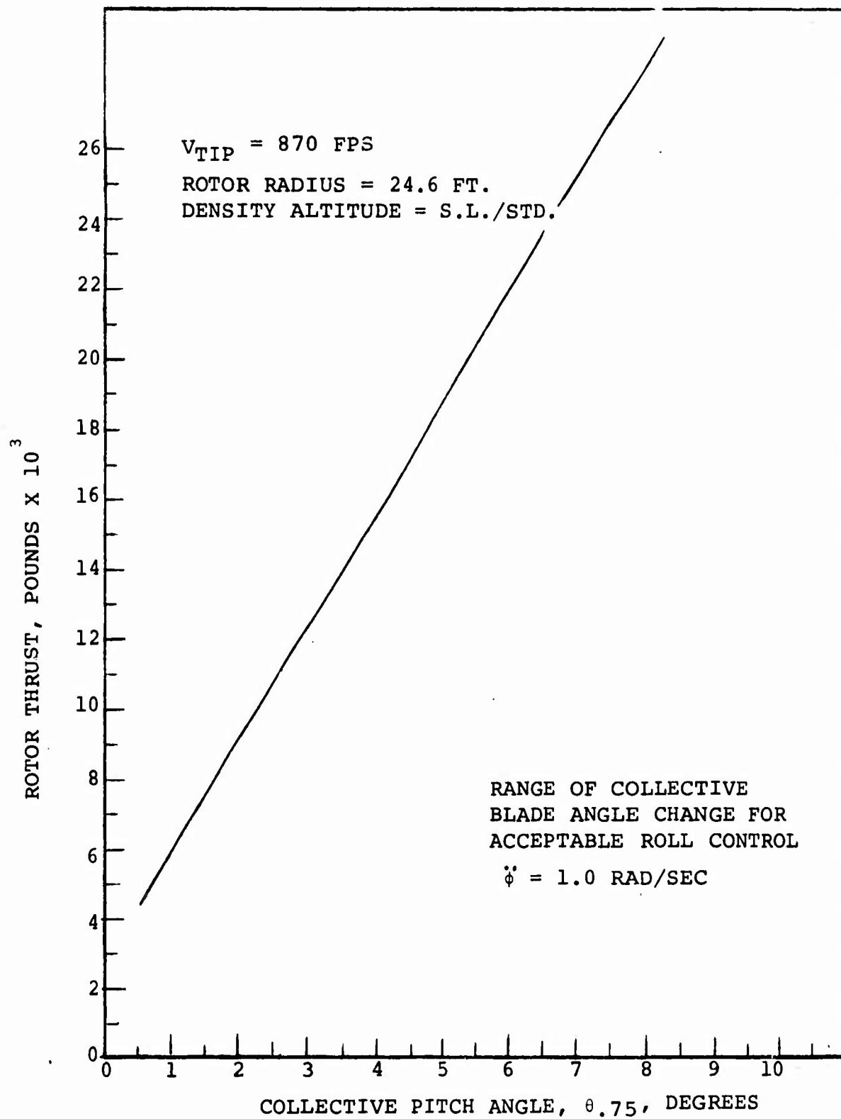
FIGURE 5.18 COLLECTIVE PITCH EFFECTIVENESS
