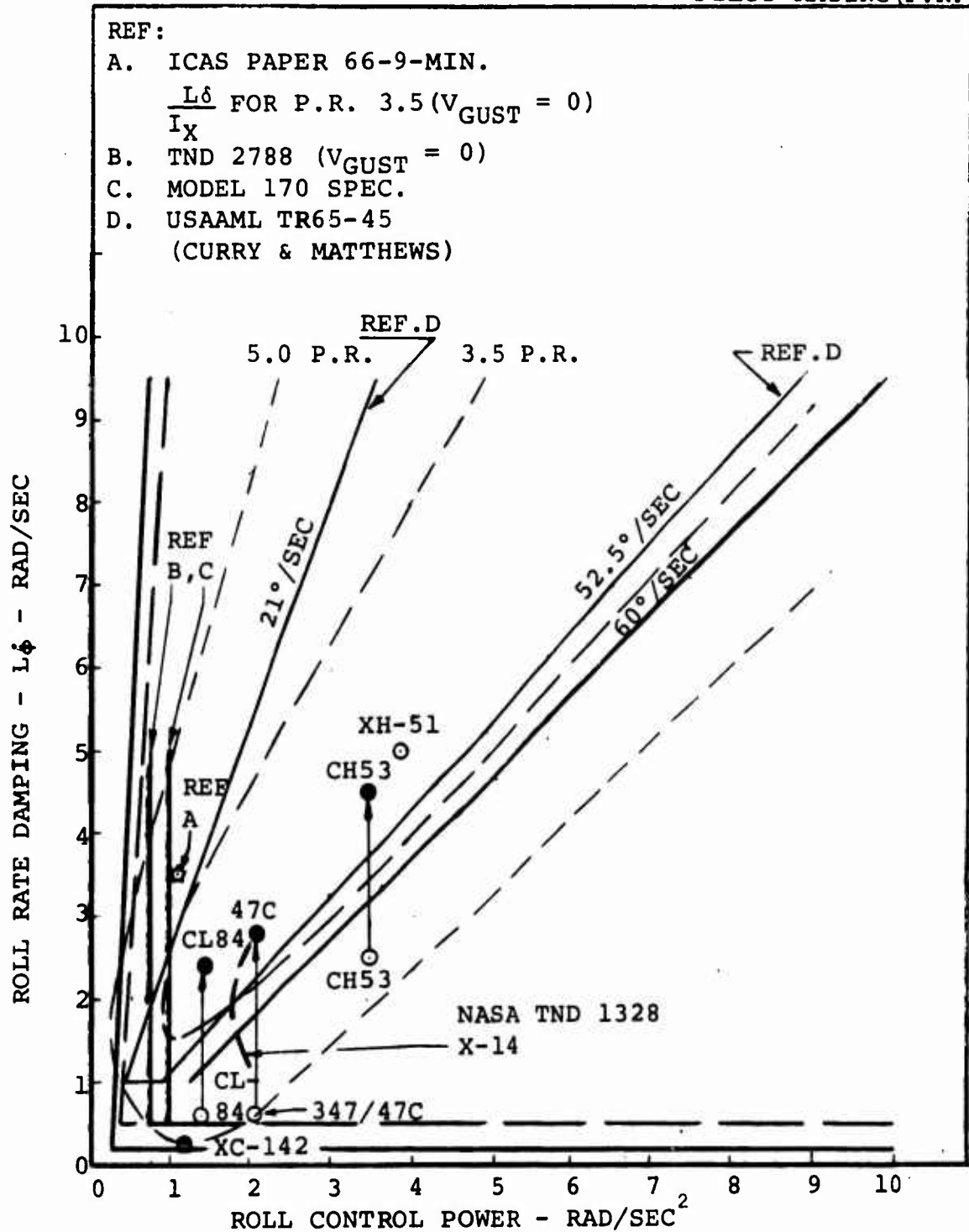
FIGURE 5.19. ROLL CONTROL POWER
