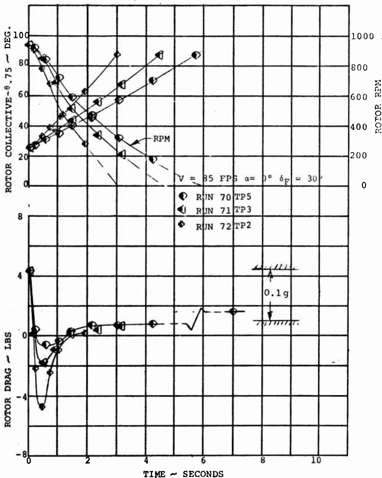
FIGURE 5.70. EFFECT OF COLLECTIVE RATE ON ROTOR DRAG DURING FEATHER AT V=85 \text{ FPS } \alpha=0^\circ \delta_F=30^\circ (LINEAR COLLECTIVE RATE)
