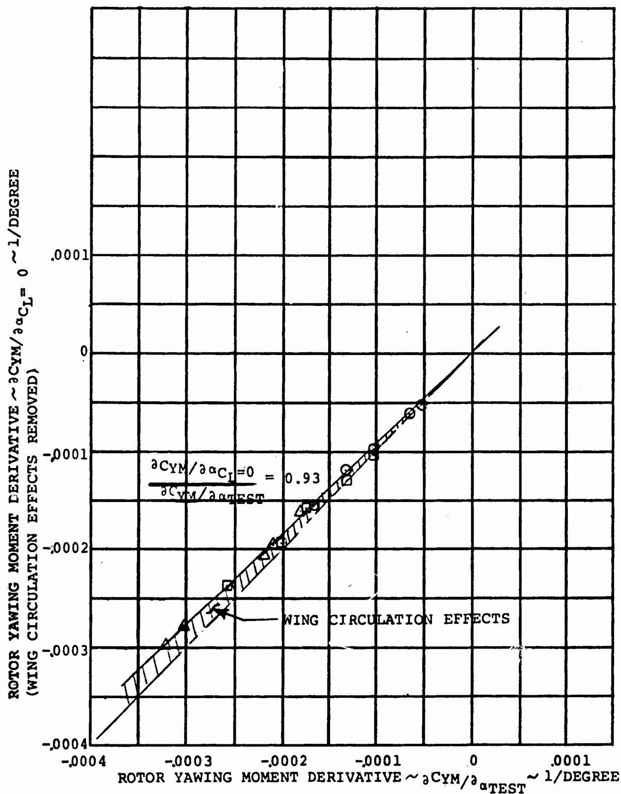
FIGURE 5.50. COMPARISON OF ROTOR YAWING MOMENT DERIVATIVE WITH AND WITHOUT WING CIRCULATION EFFECTS
