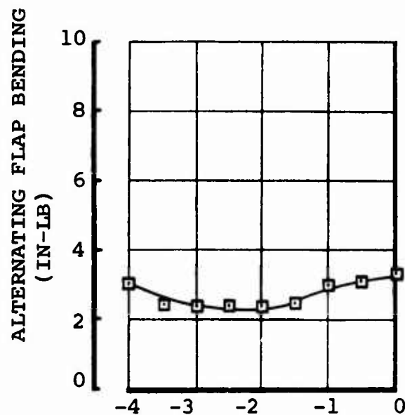
FIGURE 3.12 EFFECT OF AIRCRAFT PITCH ON BLADE ROOT BENDING MOMENTS IN CRUISE FLIGHT
