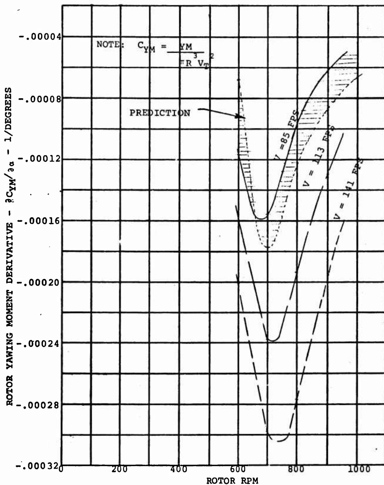
FIGURE 5.54. ROTOR YAWING MOMENT DERIVATIVE VARIATION WITH ROTOR RPM (WING CIRCULATION EFFECTS REMOVED)
