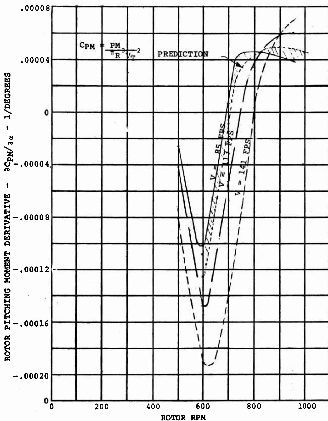
FIGURE 5.52. ROTOR PITCHING MOMENT DERIVATIVE VARIATION WITH ROTOR RPM (WING CIRCULATION EFFECTS REMOVED)
