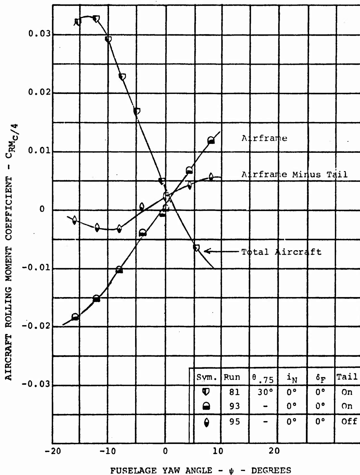
FIGURE 5.63. CONTRIBUTION OF PROP/ROTOR AND VERTICAL TAIL TO AIRCRAFT ROLLING MOMENT, \delta_F = 0 , V/V_T = 0.382
