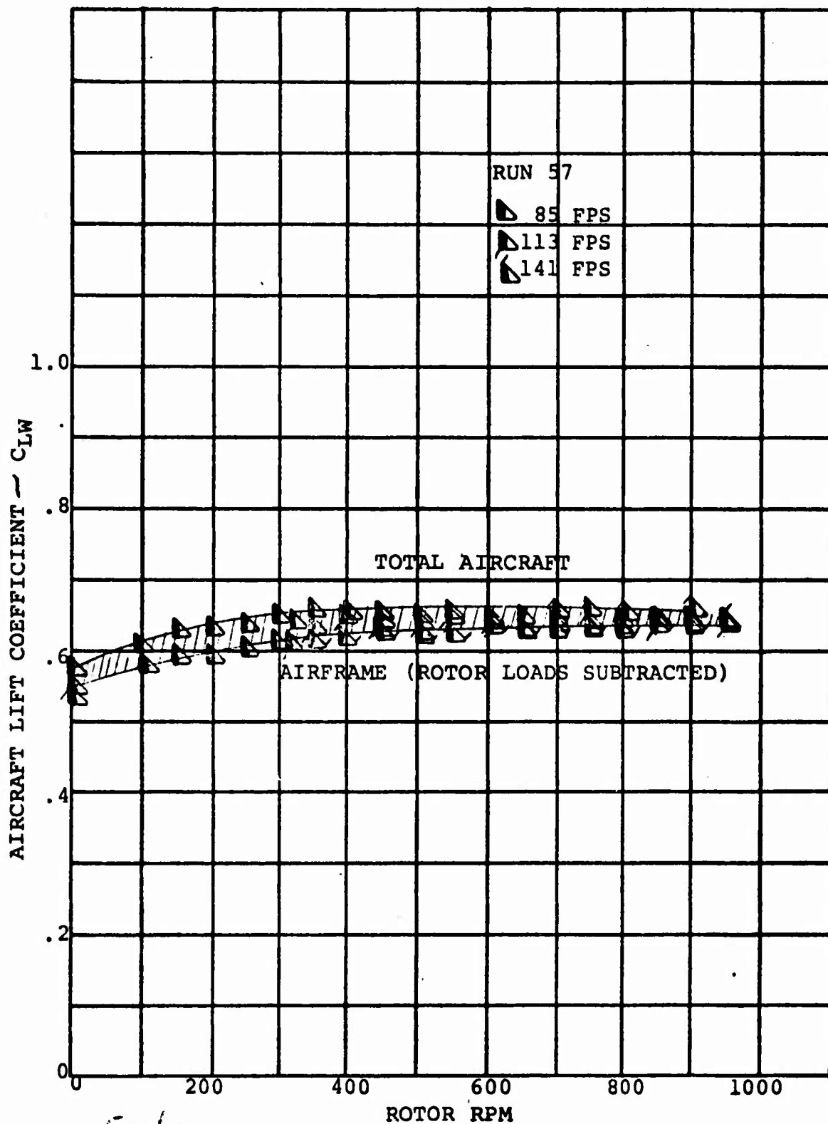
FIGURE 5.66. EFFECT OF ROTOR RPM AND FORWARD SPEED ON AIRCRAFT LIFT \alpha=0^\circ \delta_F=30^\circ (STEADY WINDMILLING)
