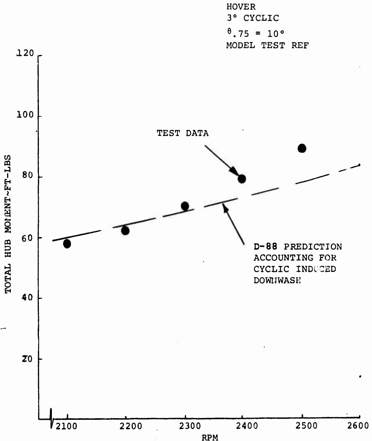
FIGURE 5.5: CORRELATION OF ROTOR HUB MOMENT DUE TO 3° CYCLIC IN HOVER WITH PREDICTION
