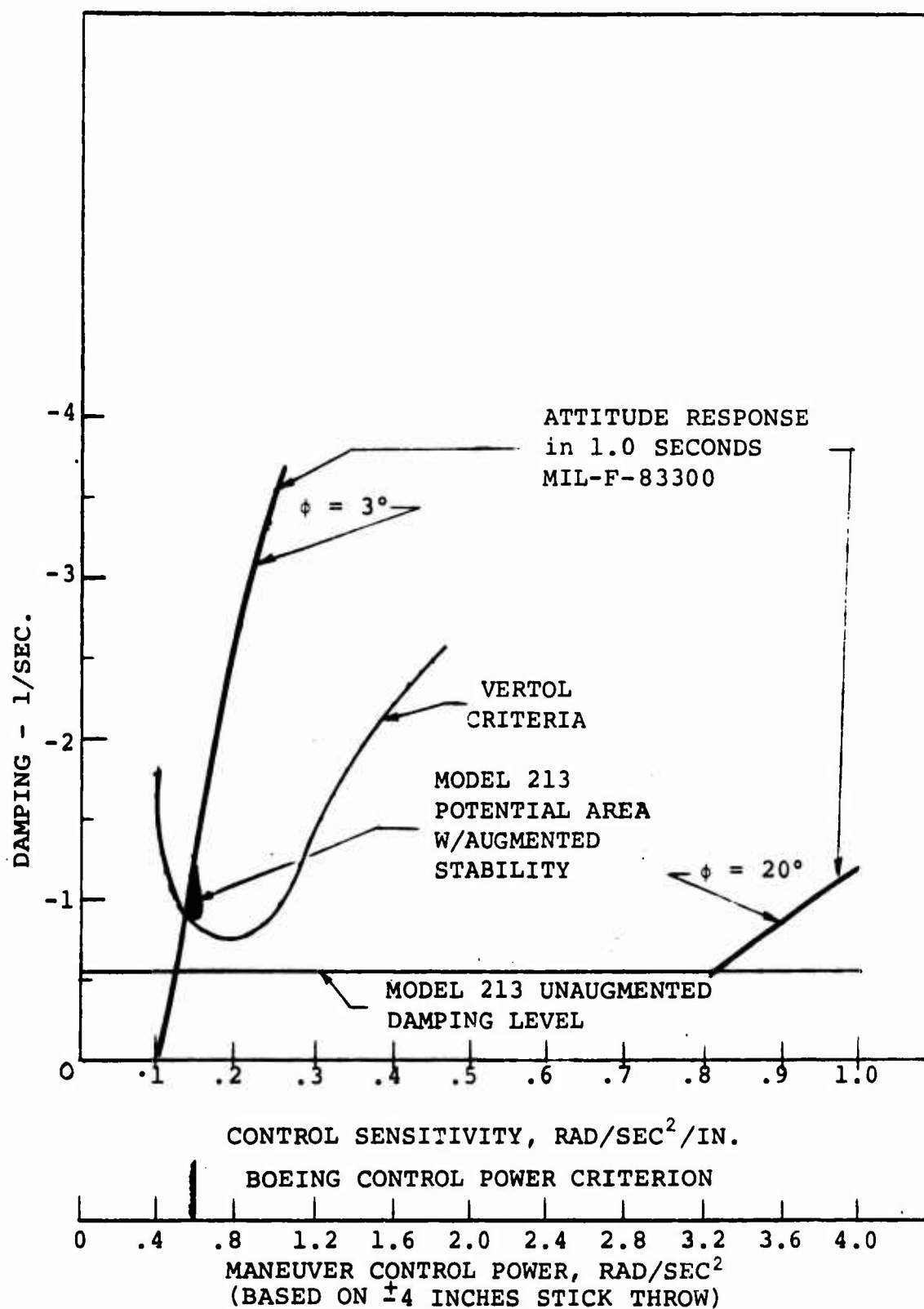
FIGURE 5.15. PITCH CONTROLLABILITY IN HOVER
