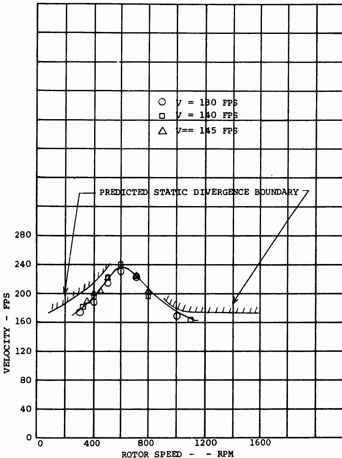
FIGURE 3.46 STATIC DIVERGENCY BOUNDARY EXTRACTED FROM TEST DATA - RUN 126 - REDUCED TORSION STIFFNESS SPAR - 1/9 SCALE CONVERSION MODEL
