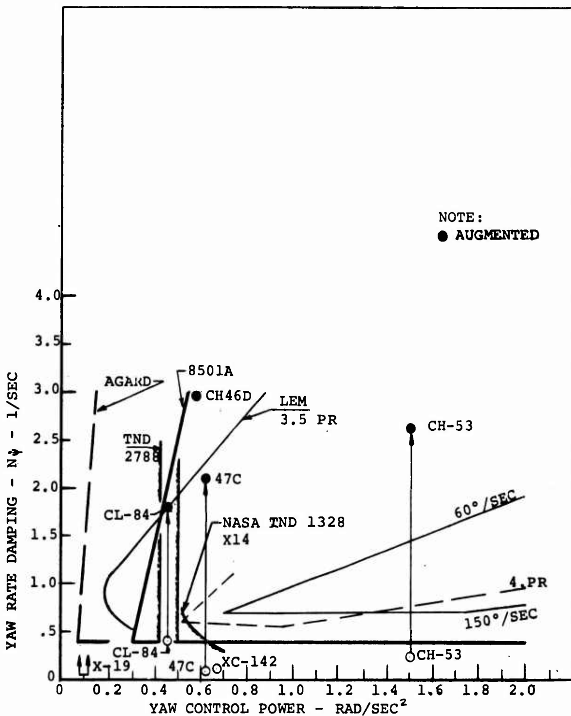
FIGURE 5.10. YAW CONTROL POWER
