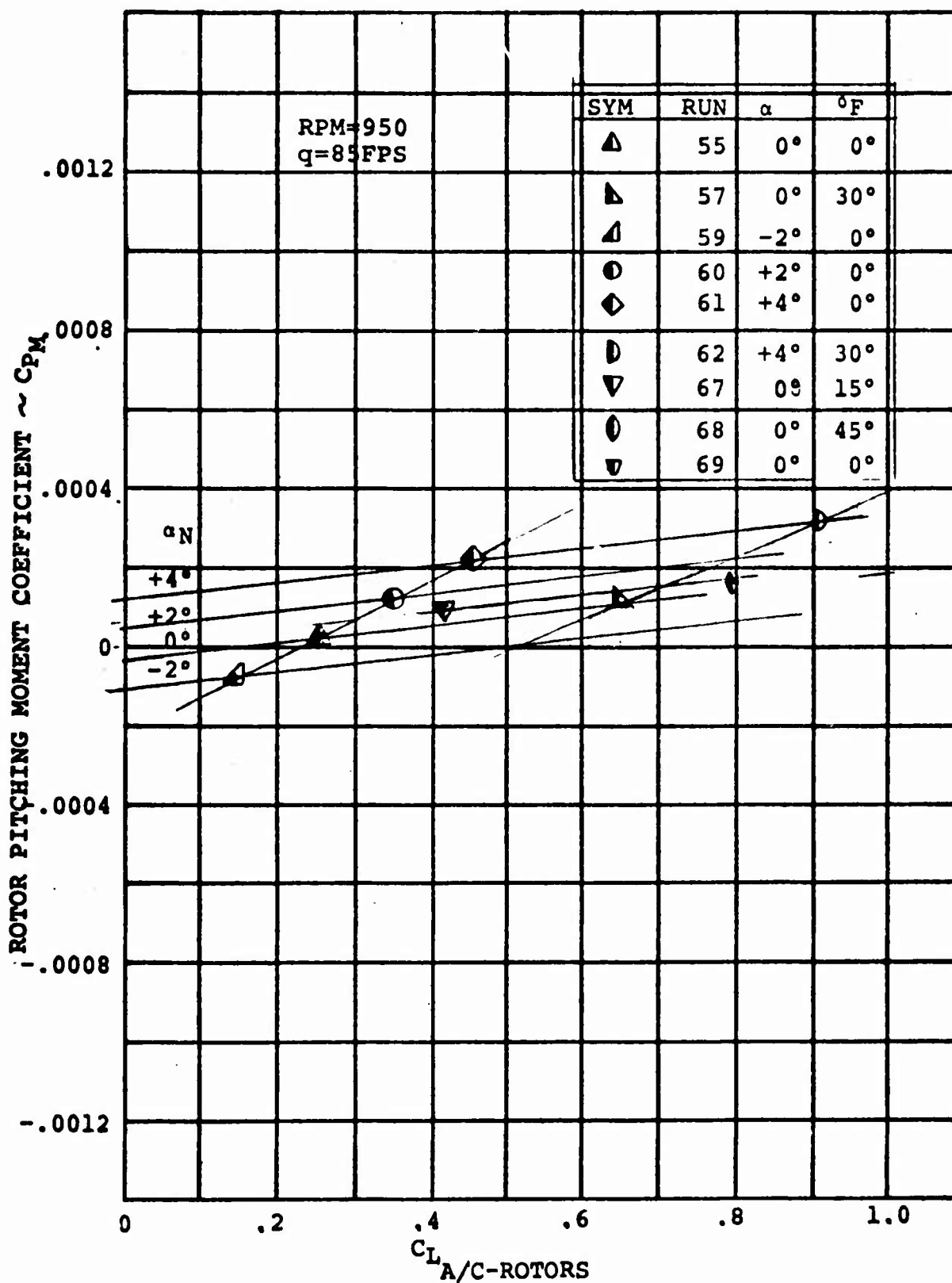
FIGURE 5.47. EFFECT OF WING LIFT ON ROTOR PITCHING MOMENT (V = 85 FPS, RPM = 950)
