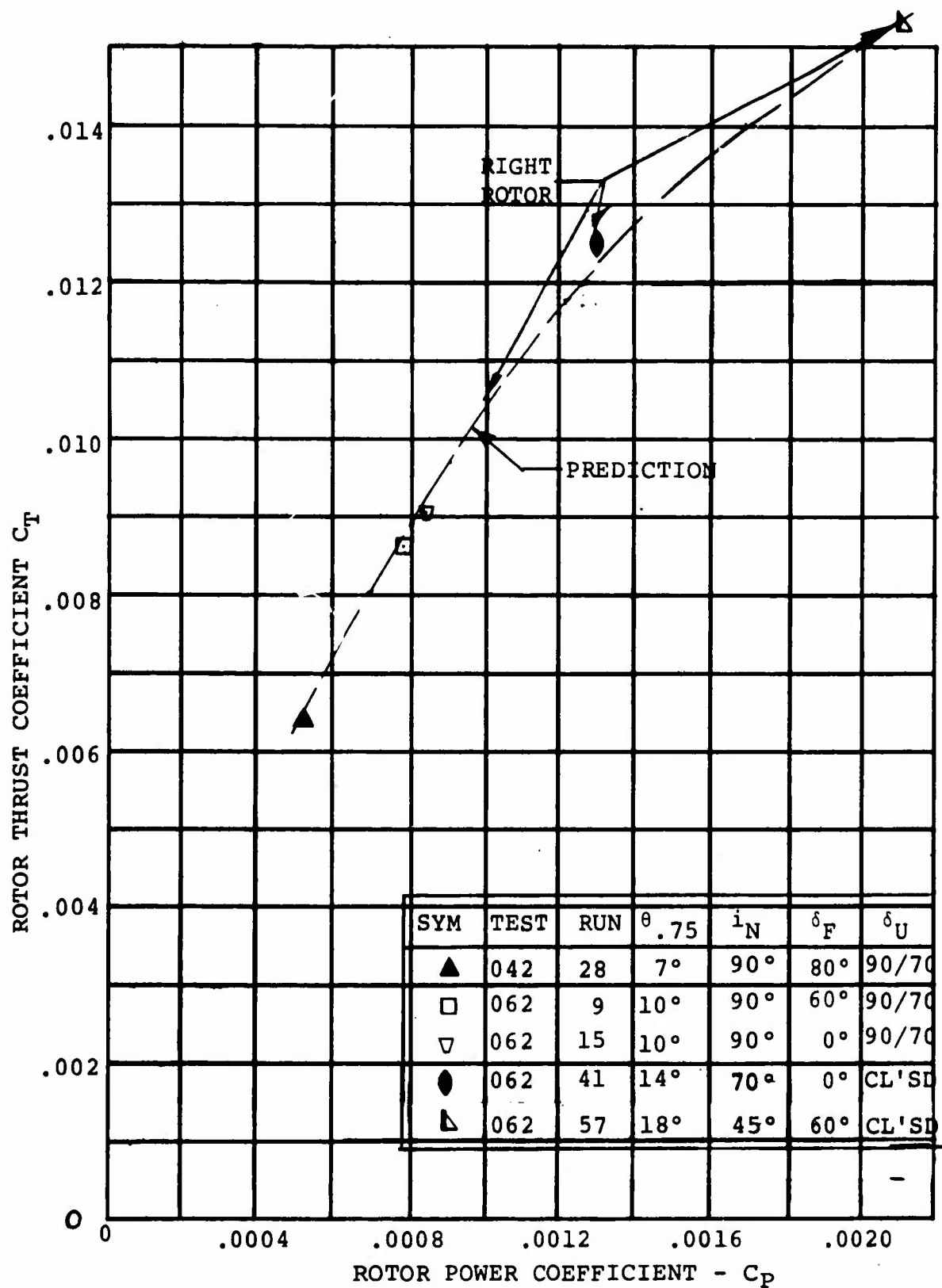
FIGURE 4.1: COMPARISON OF TEST DATA AND PREDICTION OF ROTOR THRUST/POWER COEFFICIENT VARIATION IN HOVER OUT-OF-GROUND EFFECT, 2000 RPM (ISOLATED ROTOR)
