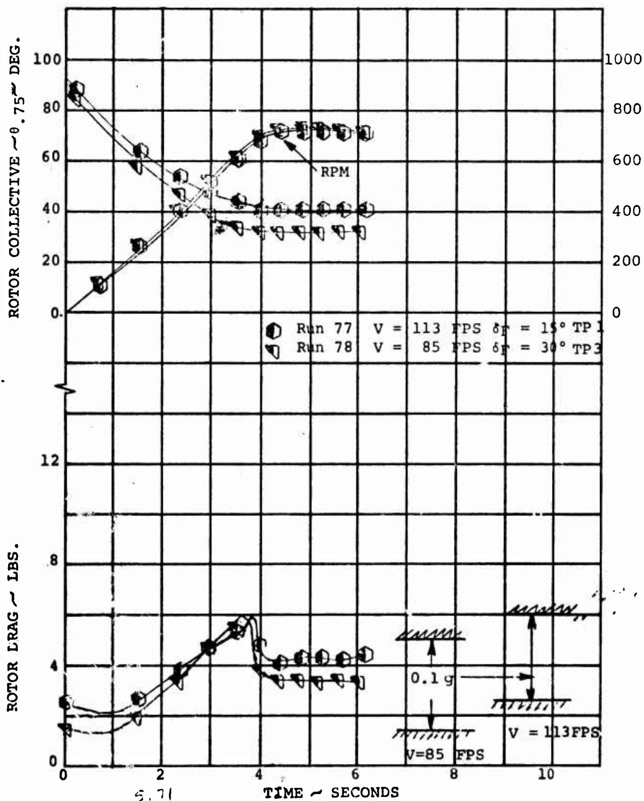
FIGURE E5.71. EFFECT OF FORWARD SPEED ON ROTOR DRAG DURING SPINUP FOR 4.5 SECOND LINEAR COLLECTIVE RATE, FINAL RPM = 715
