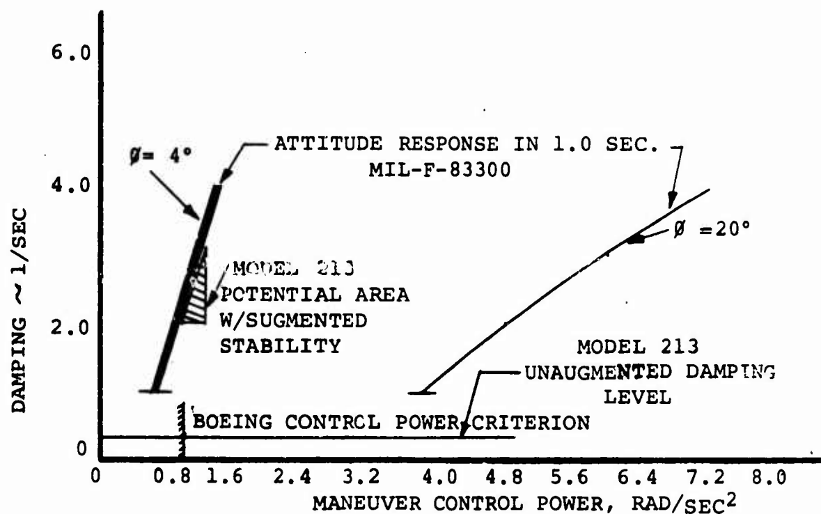
FIGURE 5.17: ROLL CONTROLLABILITY
