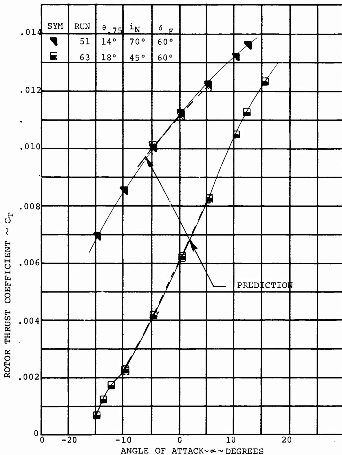
FIGURE 4.13: COMPARISON OF TEST AND PREDICTION FOR ROTOR THRUST COEFFICIENT/ANGLE OF ATTACK VARIATION IN TRANSITION
