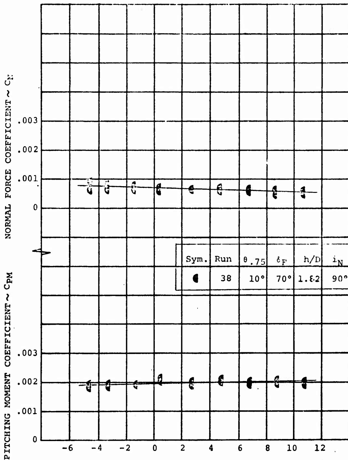
FIGURE 5.12 EFFECT OF ANGLE OF ATTACK ON ROTOR NORMAL FORCE AND PITCHING MOMENT IN THE NEAR HOVER MODE AT q=4 psf.
