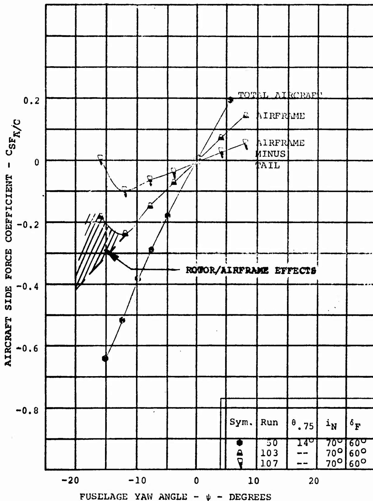
FIGURE 5.35: CONTRIBUTION OF PROP/ROTOR AND VERTICAL TAIL TO AIRCRAFT SIDE FORCE AT V/V_T = 0.206 . WITH i_N = 70^\circ
