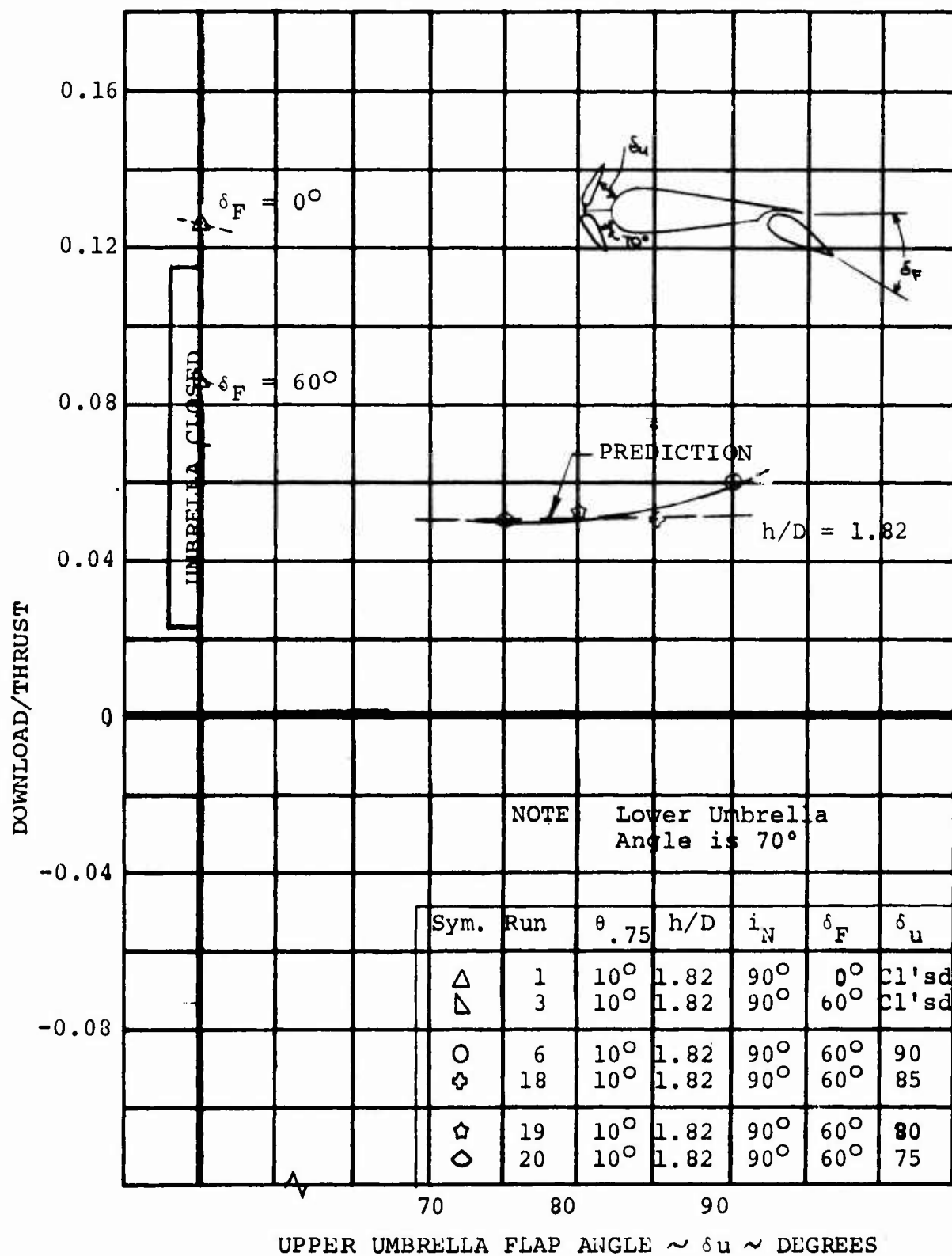
FIGURE 4.10: EFFECT OF UMBRELLA FLAP ANGLE ON AIRCRAFT HOVER DOWNLOAD/THRUST RATIO
