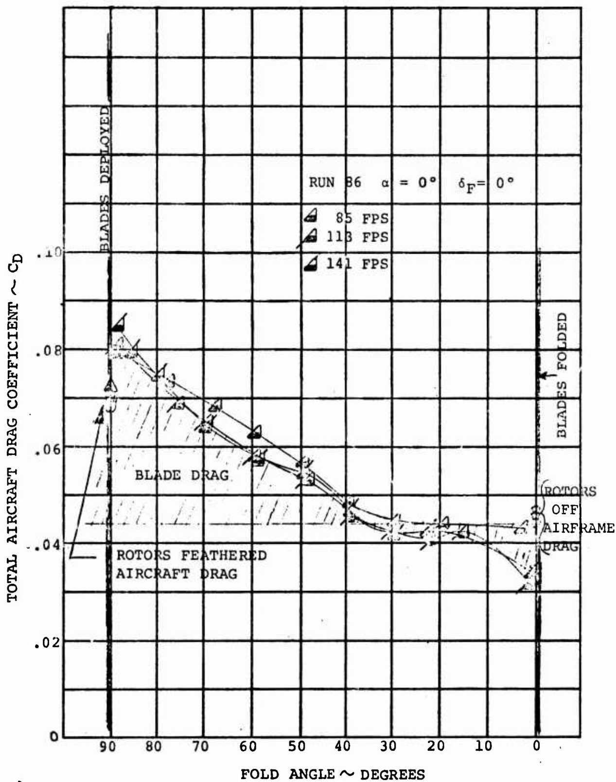
FIGURE 4.38 AIRCRAFT DRAG VARIATION WITH BLADE FOLDING AT \alpha = 0^\circ \delta_F = 0^\circ (FLATWISE FOLD)
