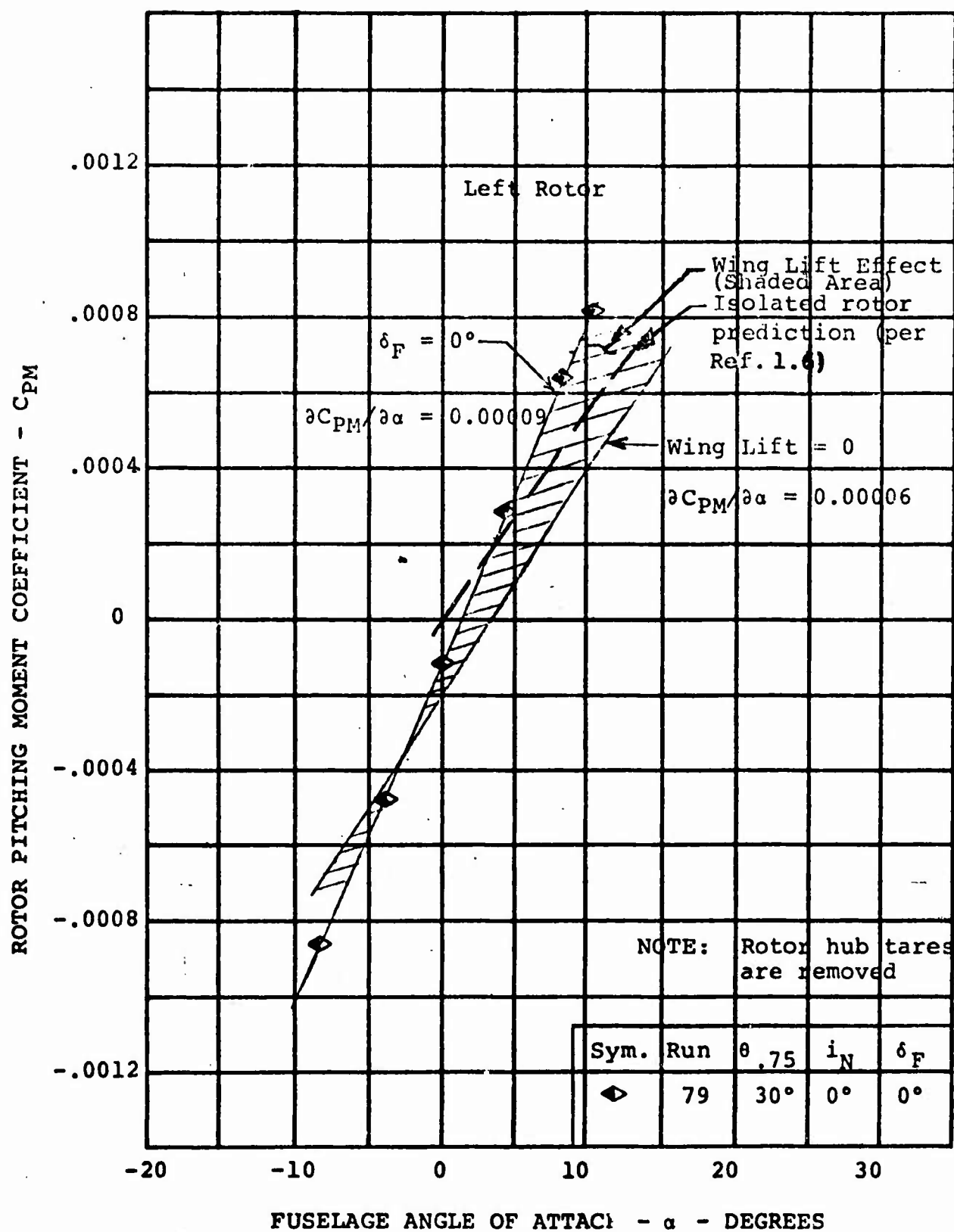
FIGURE 5.36. INFLUENCE OF WING LIFT ON ROTOR PITCHING MOMENT AT V/V_T = 0.386
