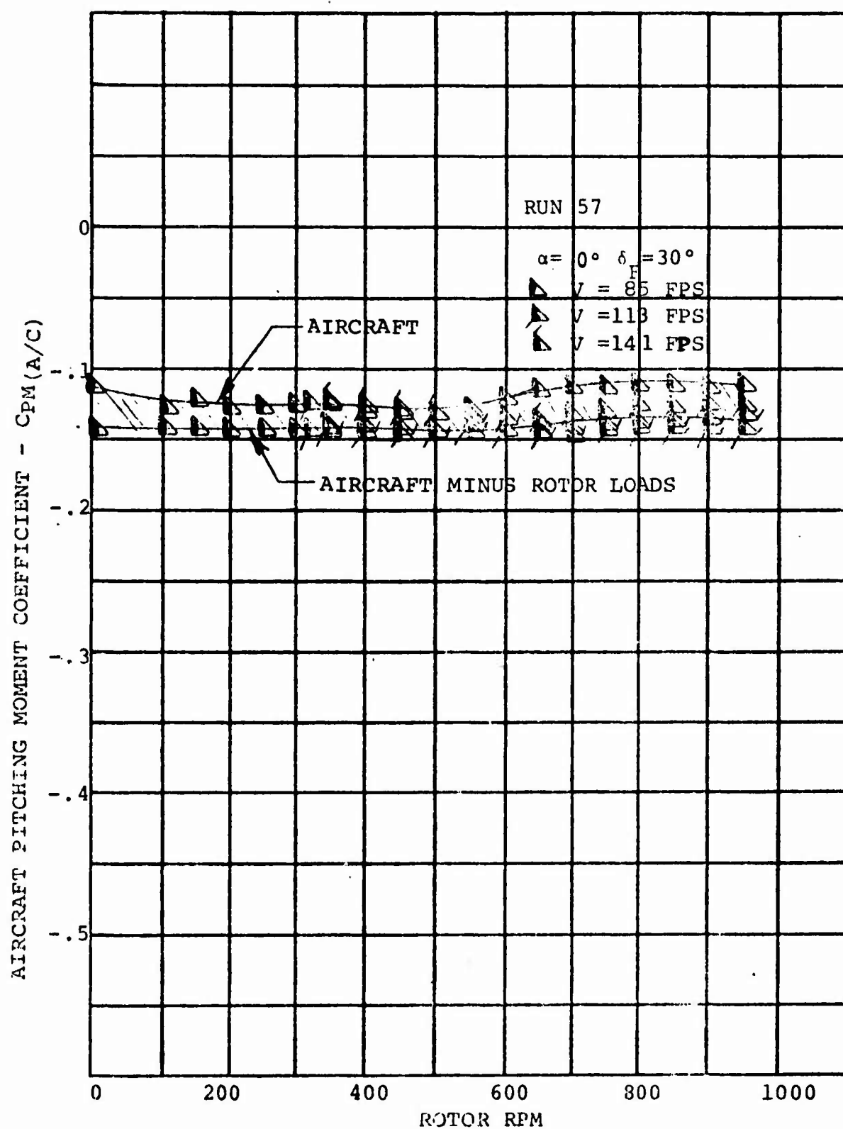
FIGURE 5.67. EFFECT OF ROTOR RPM AND FORWARD SPEED ON AIRCRAFT PITCHING MOMENT \alpha=0^\circ \delta_F=30^\circ (STEADY WINDMILLING)
