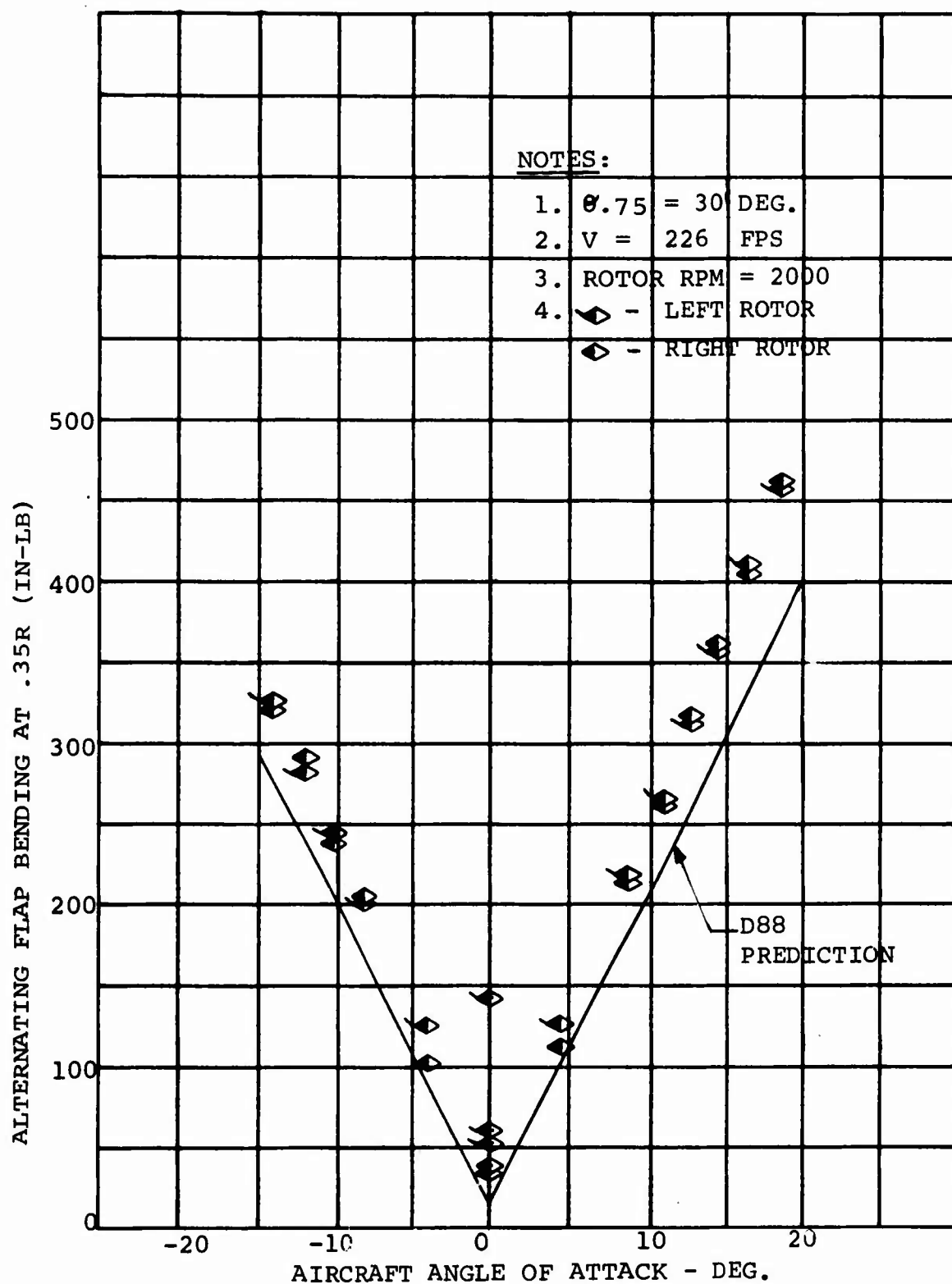
FIGURE 3.32 CORRELATION OF PREDICTED AND MEASURED ALTERNATING BLADE FLAP BENDING MOMENT WITH ANGLE OF ATTACK VARIATION FOR CRUISE FLIGHT, TILT ROTOR PERFORMANCE MODEL.
