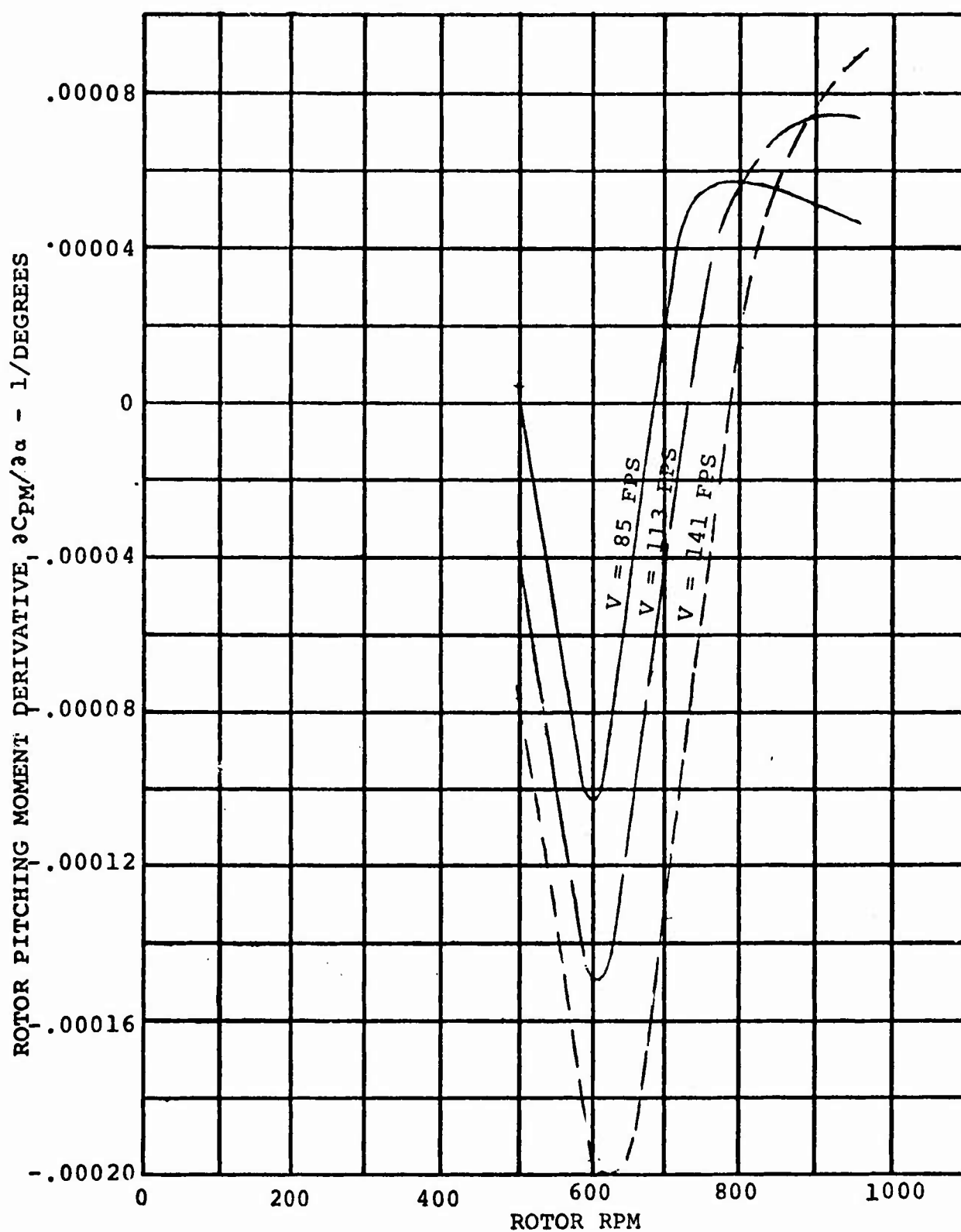
FIGURE 5.42 ROTOR PITCHING MOMENT DERIVATIVE VARIATION WITH ROTOR RPM, \delta F = 0^\circ
