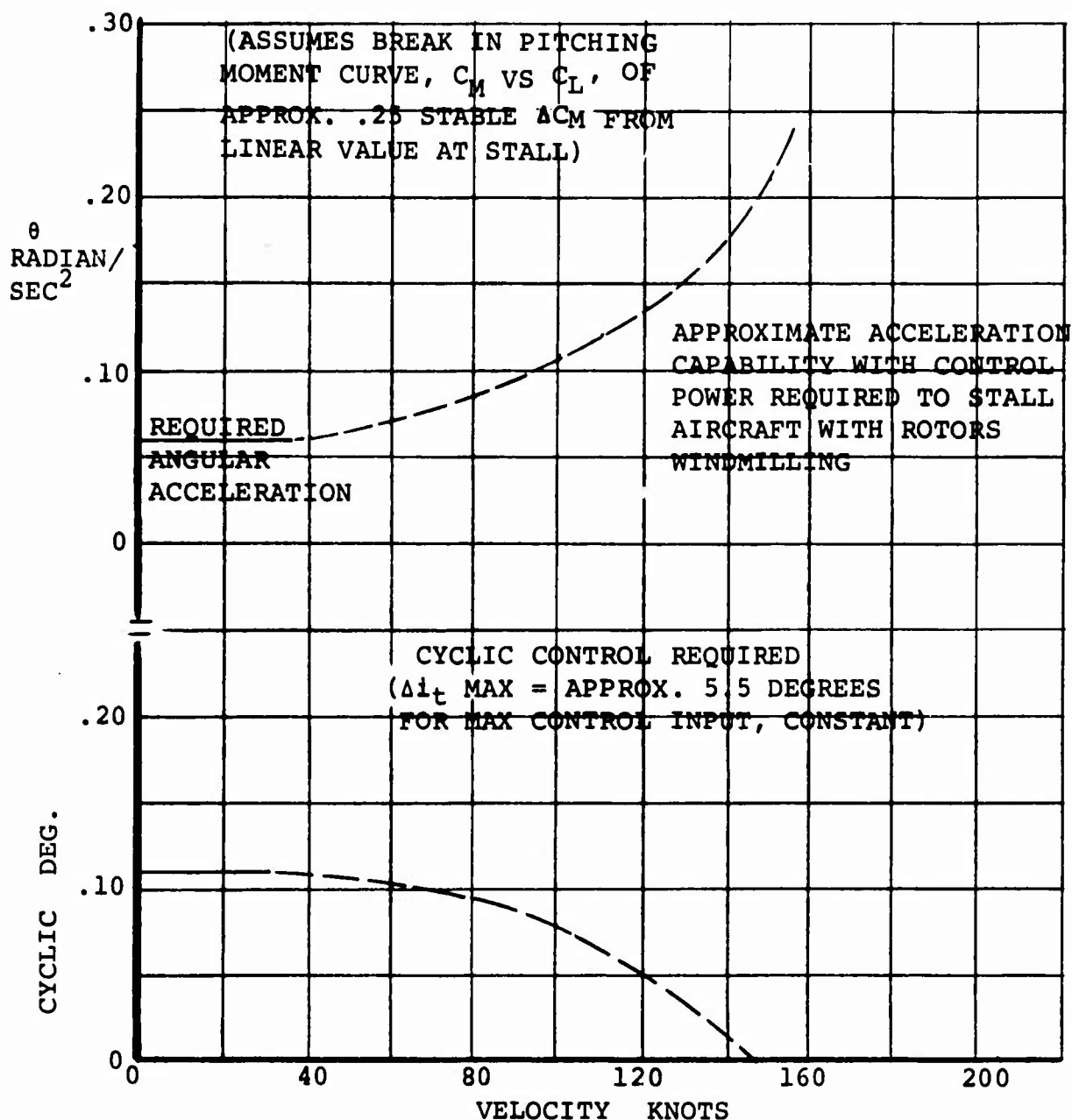
FIGURE 5.34: MODEL 222 LONGITUDINAL CONTROL CAPABILITY AND REQUIREMENT
