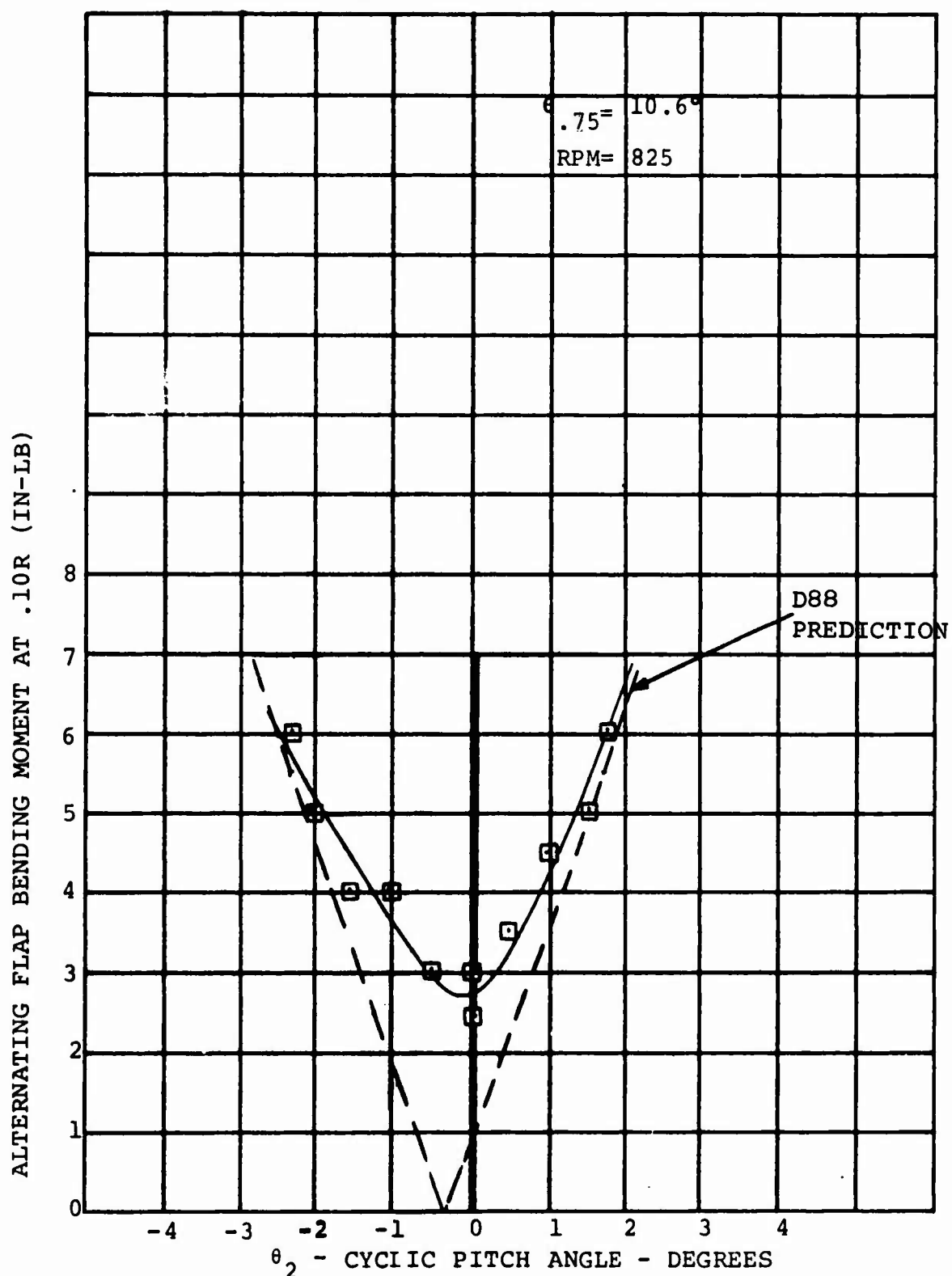
FIGURE 3.18 CORRELATION OF MEASURED AND PREDICTED ROTOR ALTERNATING FLAP BENDING MOMENT IN HOVER WITH CYCLIC PITCH VARIATION-TILT ROTOR DYNAMIC MODEL
