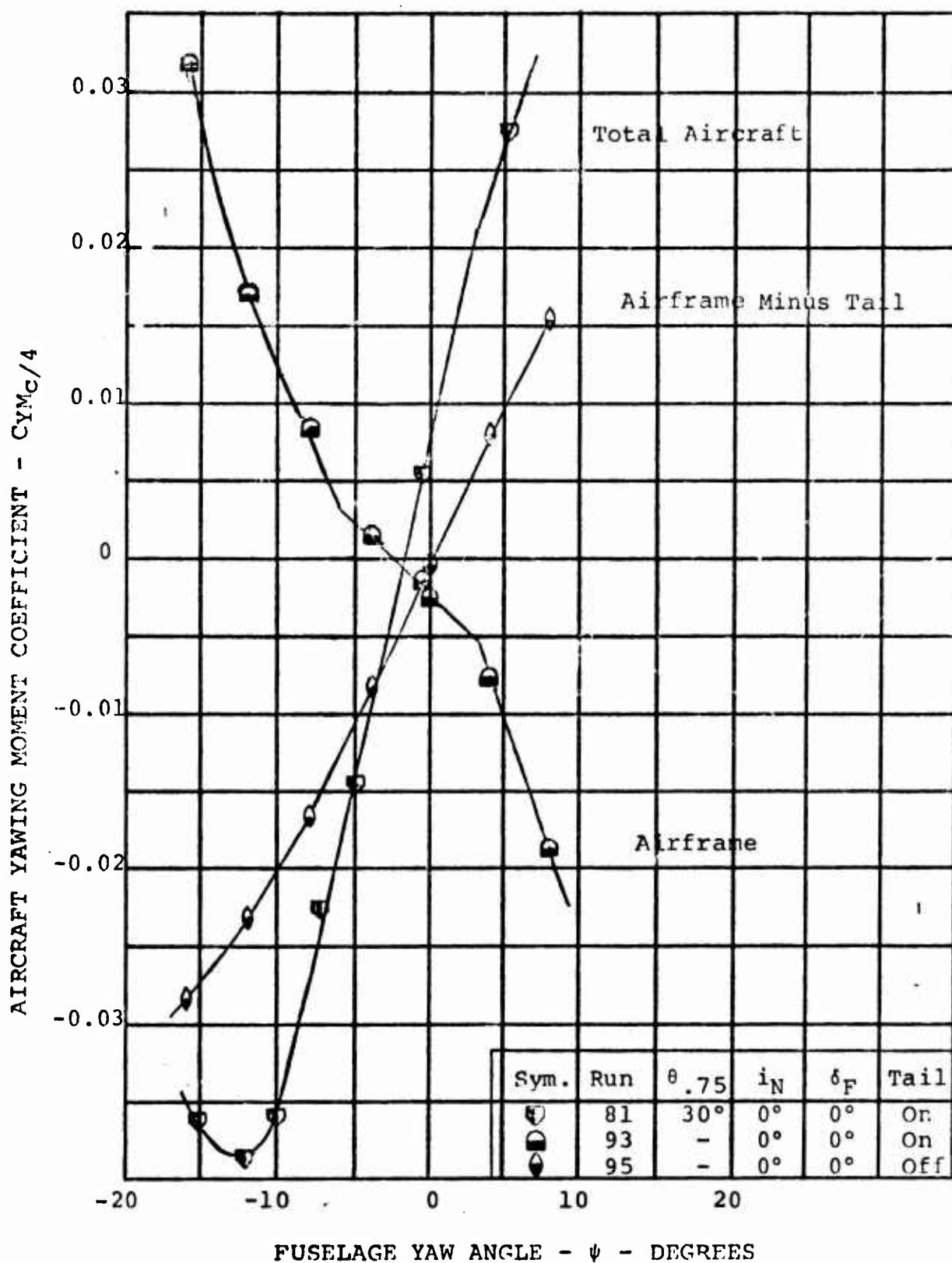
FIGURE 5.62. CONTRIBUTION OF PROP/ROTOR AND VERTICAL TAIL TO AIRCRAFT YAWING MOMENT, \delta_F = 0 , V/V_T = 0.382
