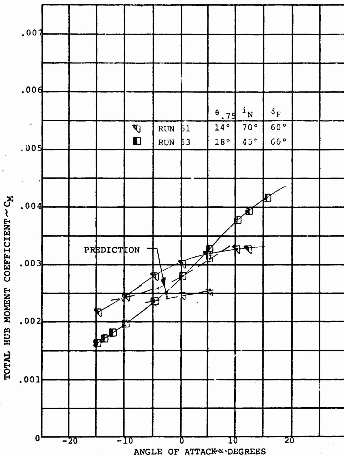
FIGURE 4.15: COMPARISON OF TEST AND PREDICTION FOR TOTAL HUB MOMENT IN TRANSITION
