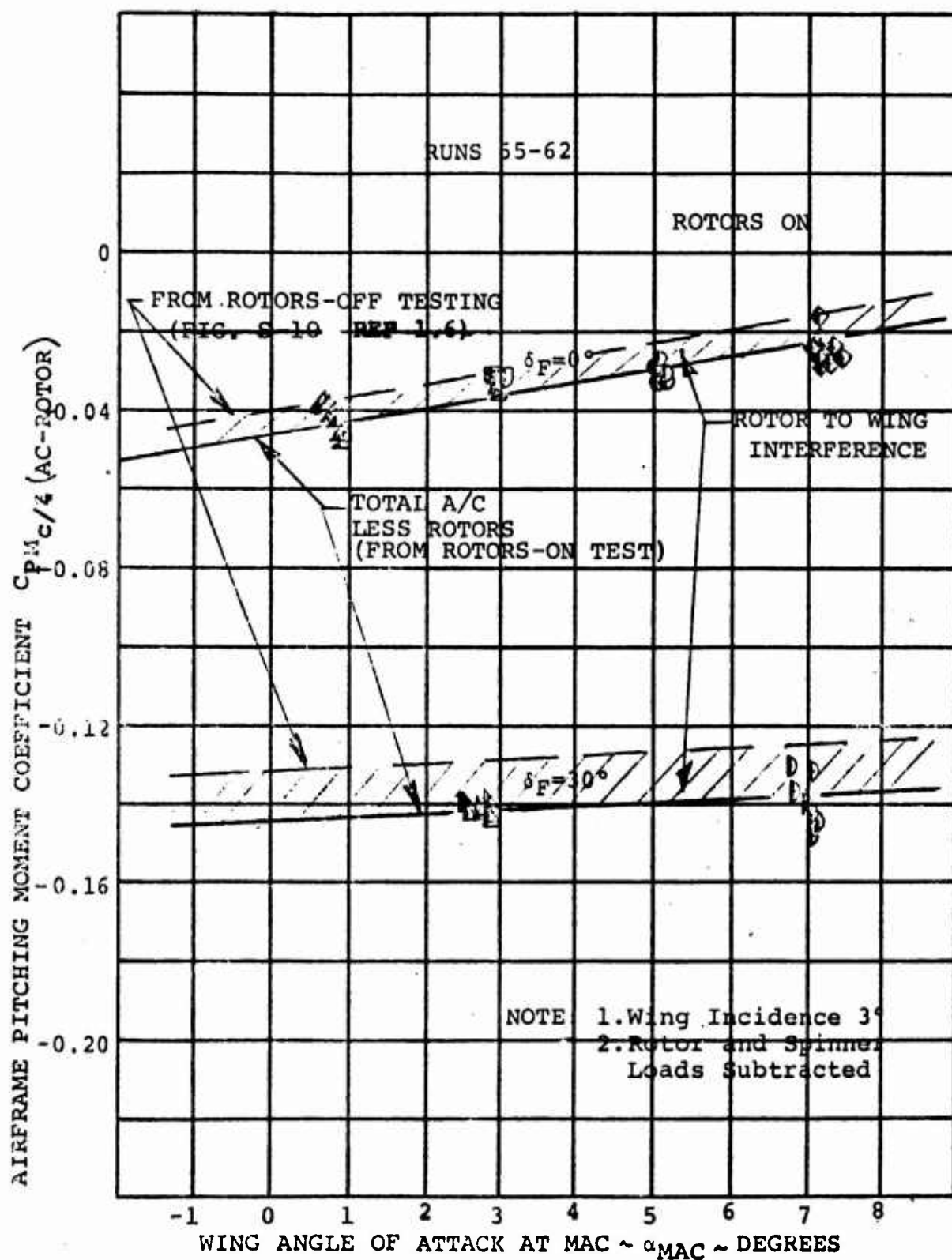
FIGURE 4.34 AIRFRAME PITCHING MOMENT/ANGLE OF ATTACK VARIATION FOR FLAP DEFLECTIONS OF 0^\circ AND 30^\circ
