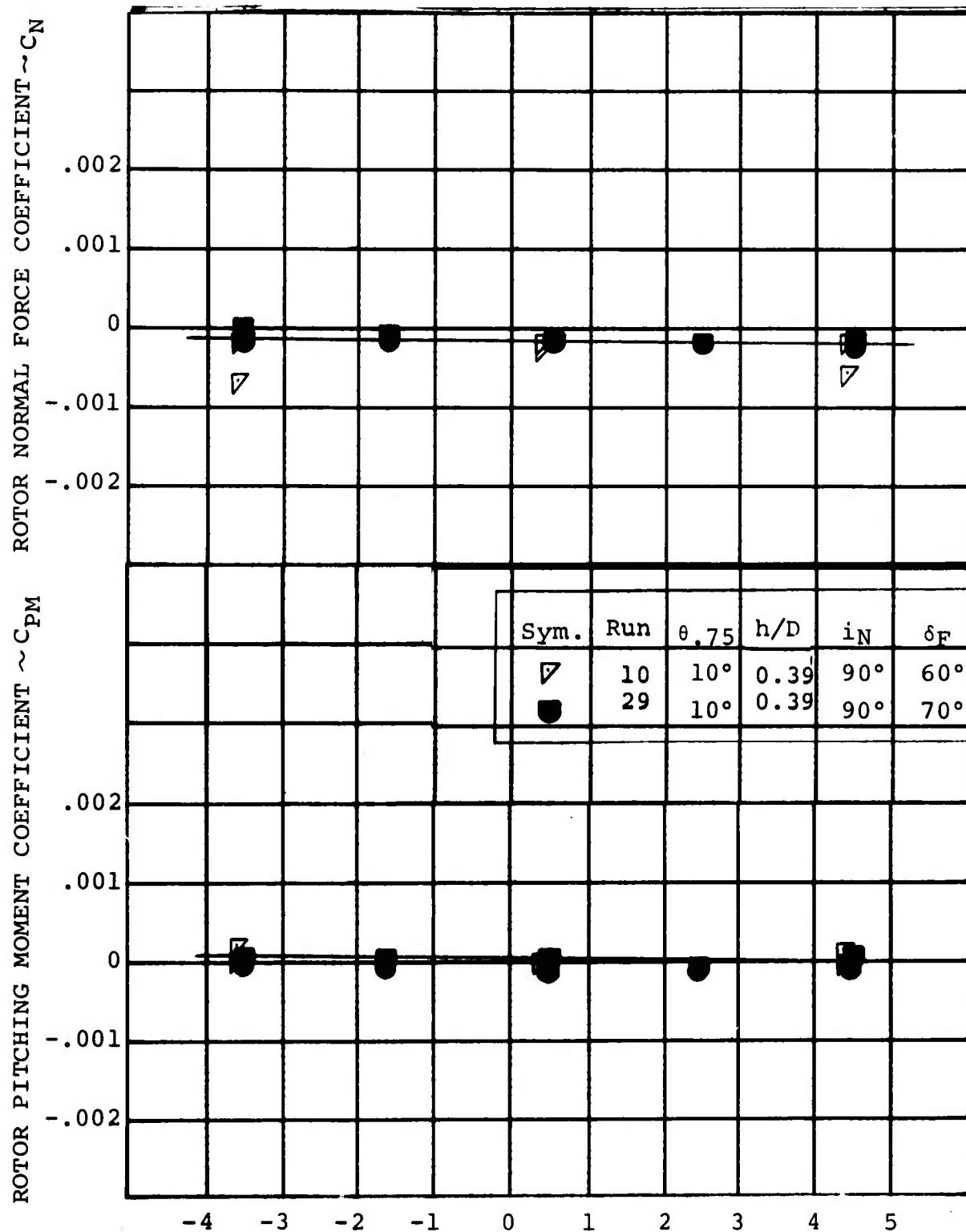
FUSELAGE ANGLE OF ATTACK \sim DEGREES FIGURE 5.11 EFFECT OF ANGLE OF ATTACK ON ROTOR NORMAL FORCE IN HOVER
