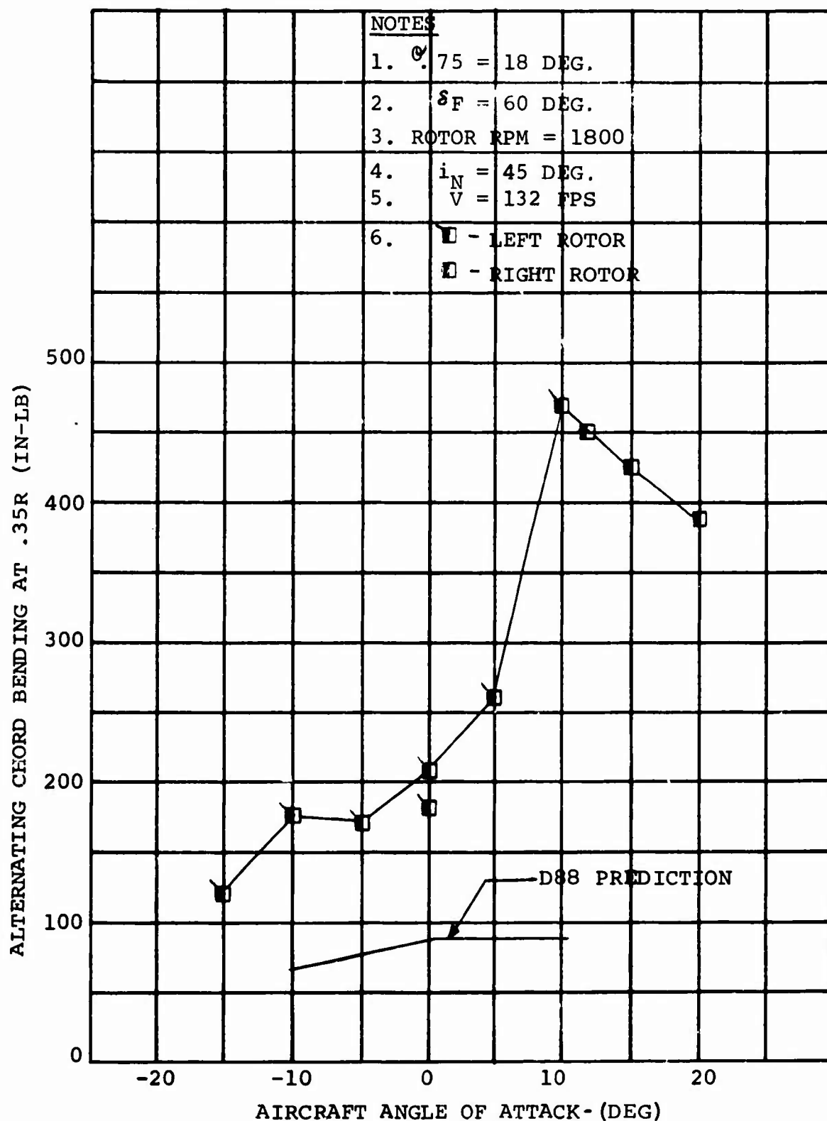
FIGURE 3.27 CORRELATION OF PREDICTED AND MEASURED BLADE ALTERNATING CHORD BENDING MOMENT WITH AIRCRAFT ANGLE OF ATTACK FOR TRANSITION FLIGHT, TILT ROTOR PERFORMANCE MODEL.
