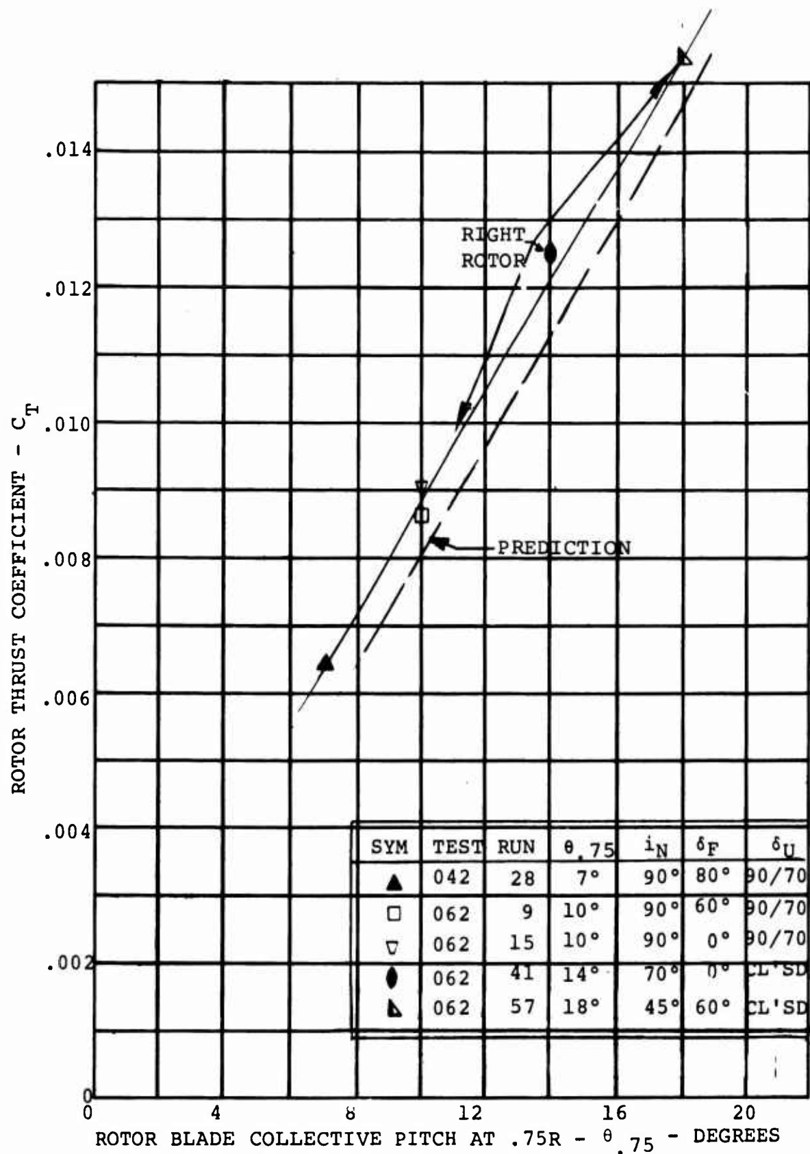
FIGURE 4.2: COMPARISON OF TEST DATA AND PREDICTION OF ROTOR THRUST COEFFICIENT/COLLECTIVE VARIATION IN HOVER OUT-OF-GROUND EFFECT, 2000 RPM (ISOLATED ROTOR)
