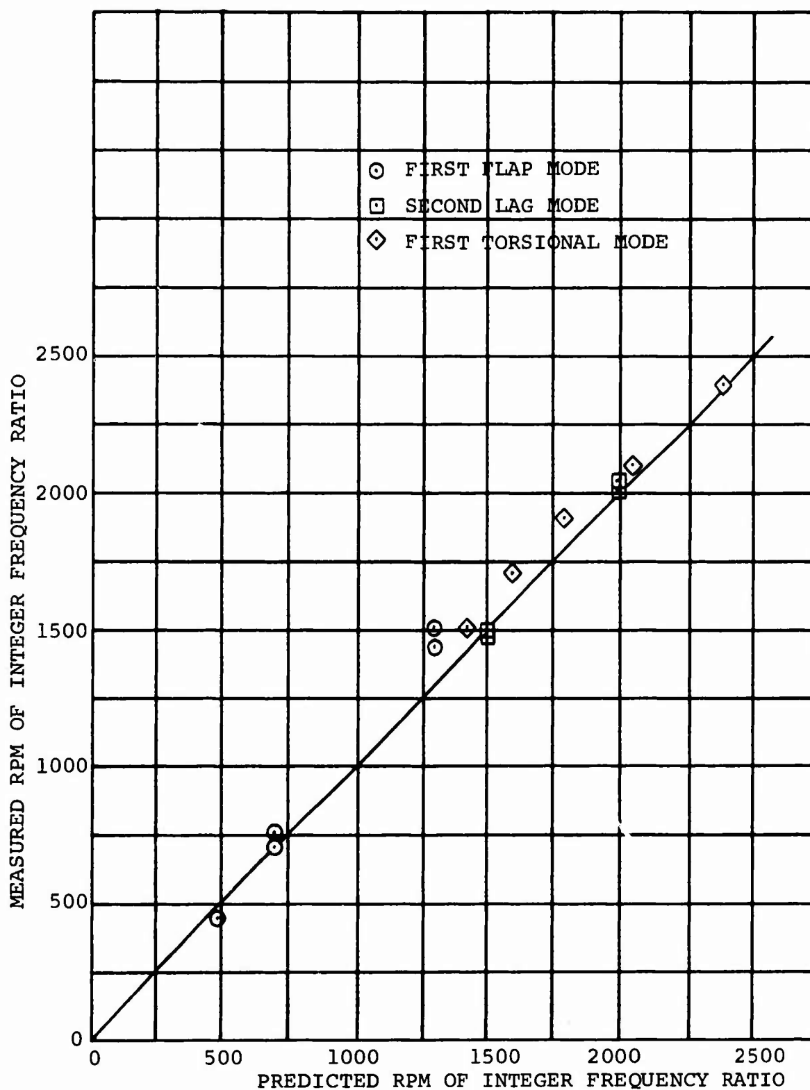
FIGURE 3.7 CORRELATION OF MEASURED AND PREDICTED BLADE FREQUENCIES TILT ROTOR PERFORMANCE MODEL
