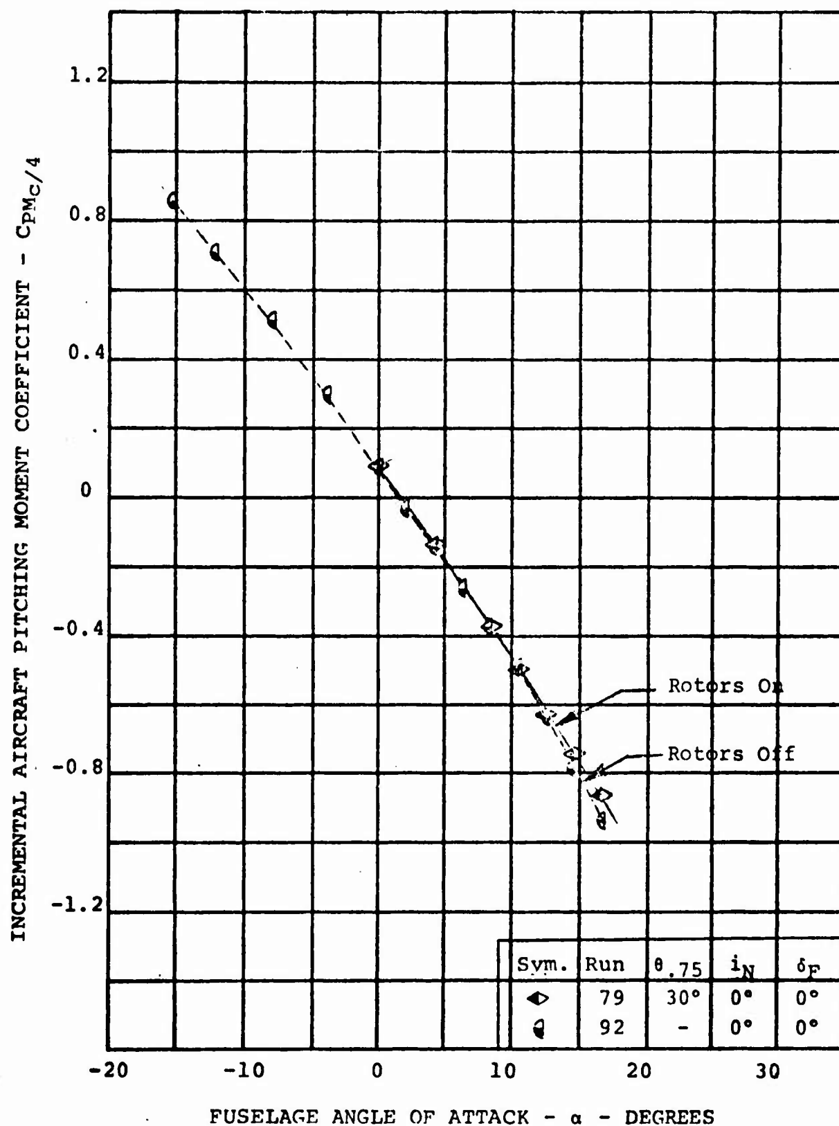
FIGURE 5.58 EFFECT OF ROTORS ON HORIZONTAL TAIL CONTRIBUTION TO AIRCRAFT PITCHING MOMENT
