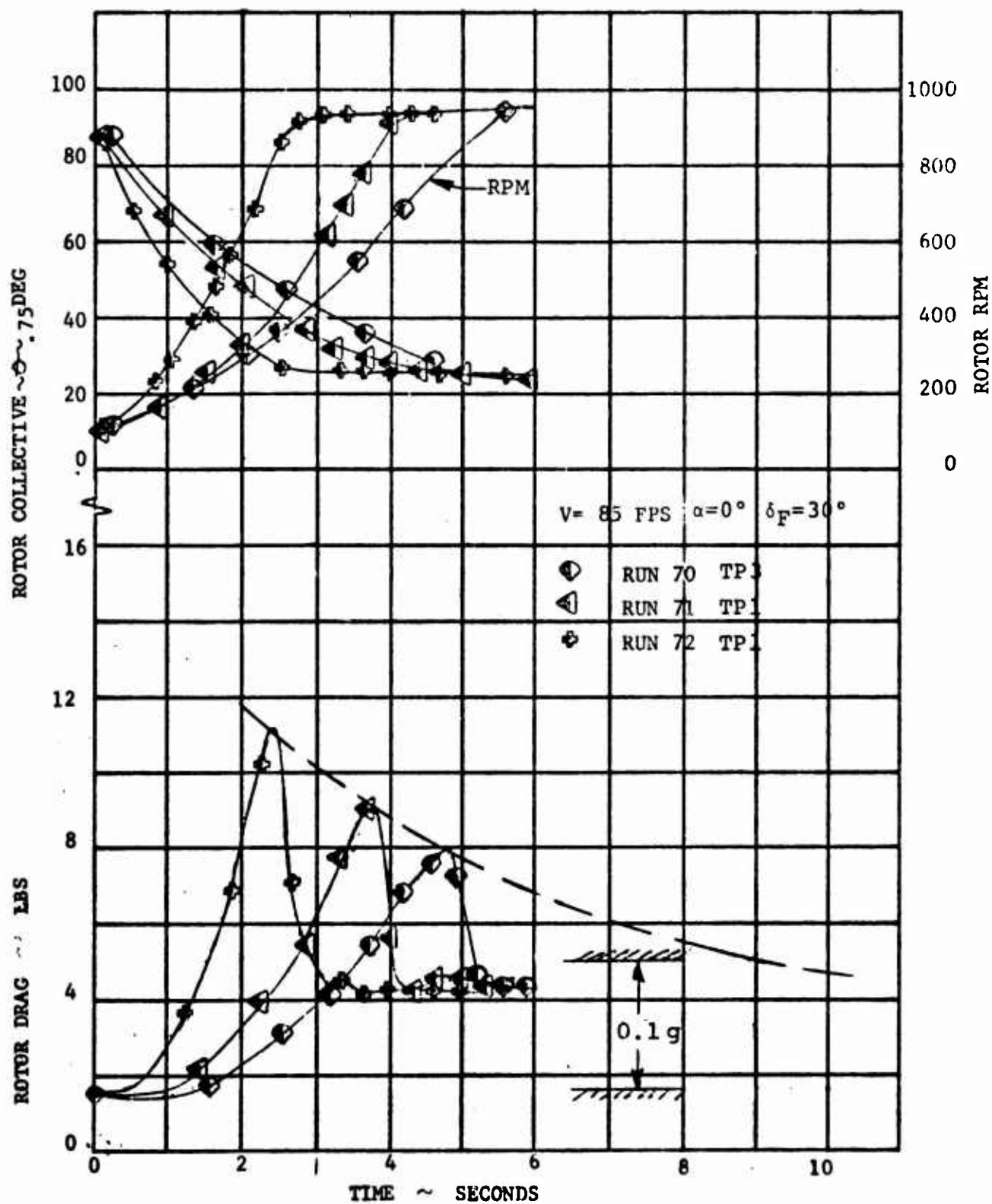
FIGURE 5.69: EFFECT OF COLLECTIVE SCHEDULING ON SPINUP RPM
