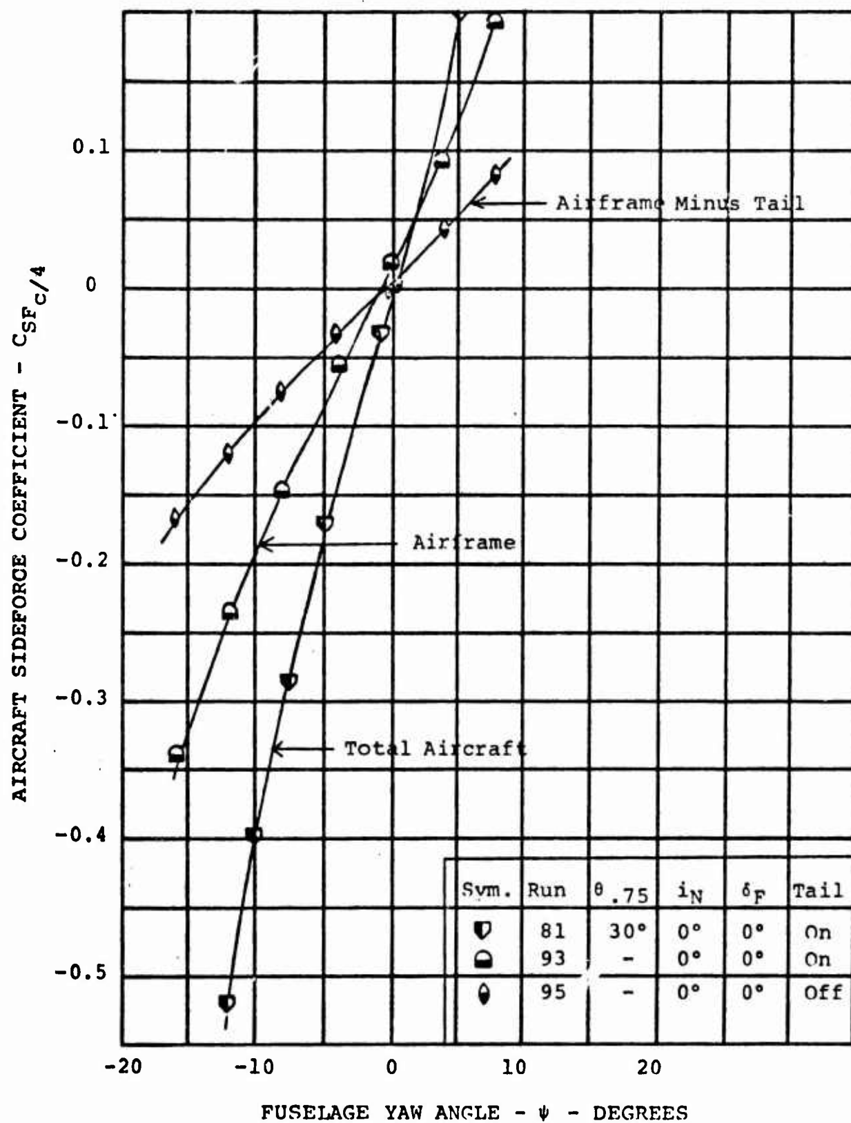
FIGURE 5.61. CONTRIBUTION OF PROP/ROTOR AND VERTICAL TAIL TO AIRCRAFT SIDE FORCE, \delta_F = 0^\circ , V/V_T = 0.382
