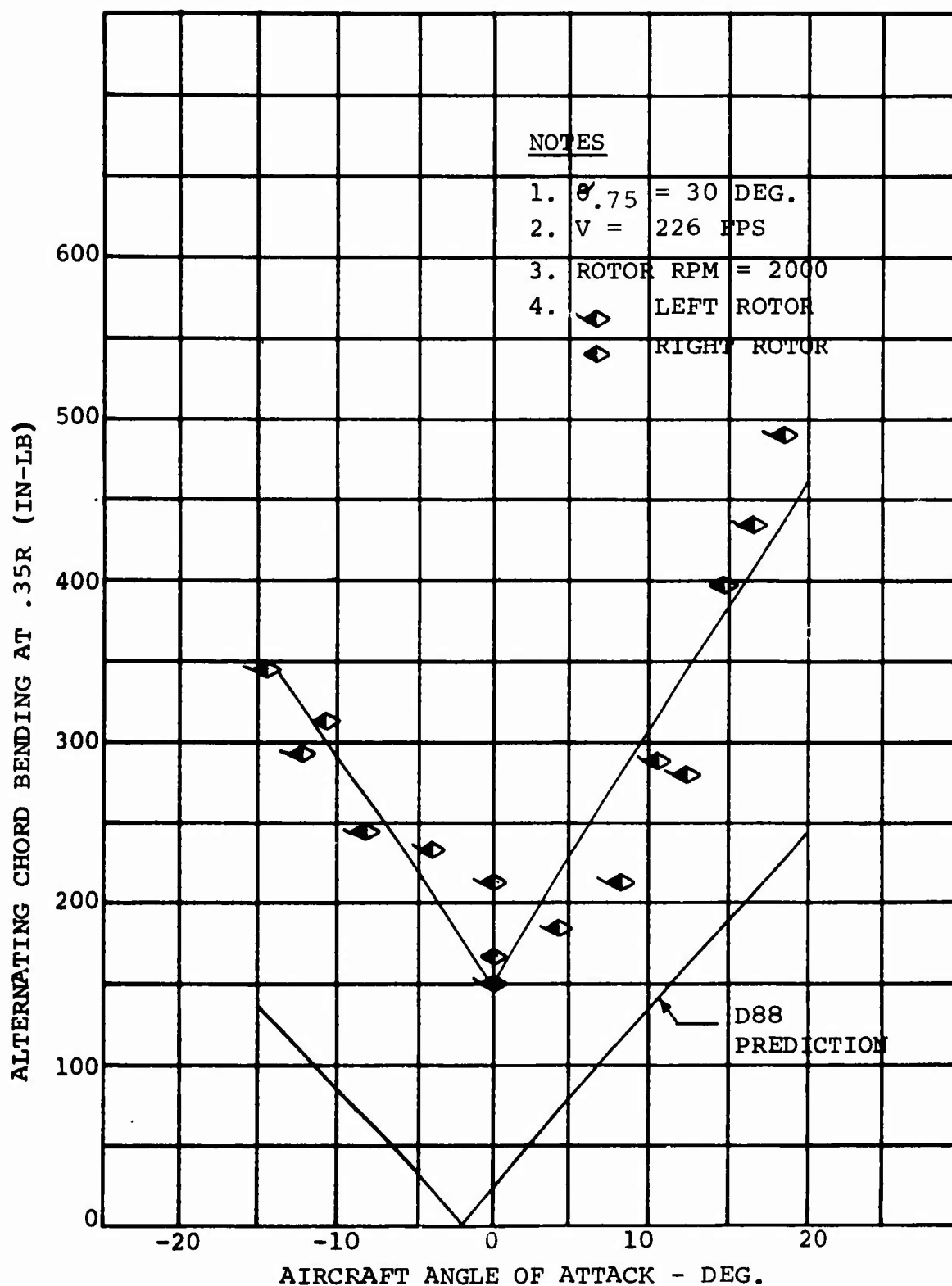
FIGURE 3.33 CORRELATION OF PREDICTED AND MEASURED ALTERNATING BLADE CHORD BENDING MOMENT WITH ANGLE OF ATTACK VARIATION FOR CRUISE FLIGHT, TILT ROTOR PERFORMANCE MODEL.
