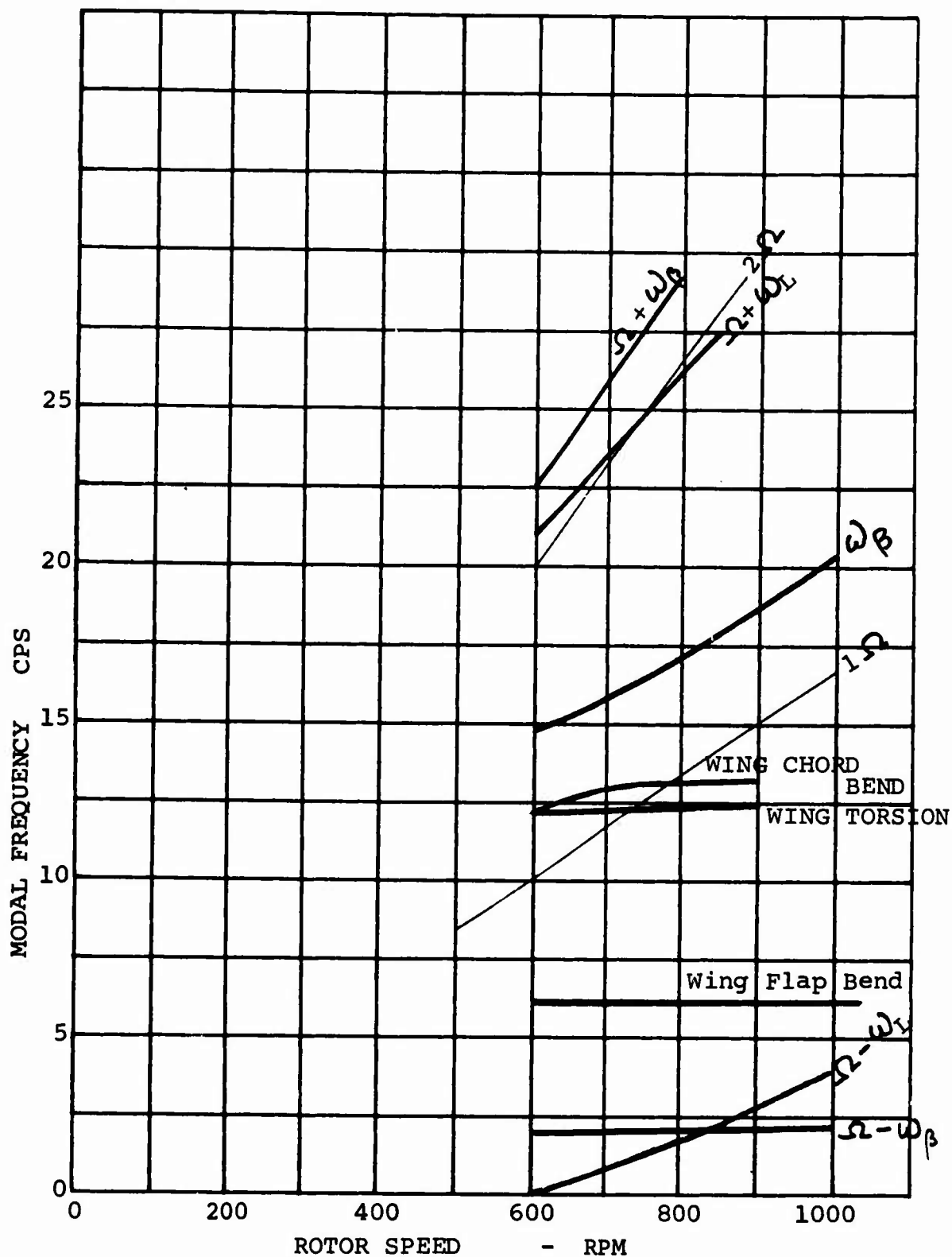
FIGURE 3.44. FREQUENCY SPECTRUM FOR NOMINAL STIFFNESS WING SPAR--WINDMILLING CONDITION-- V=104 FPS 1/9 SCALE CONVERSION MODEL
