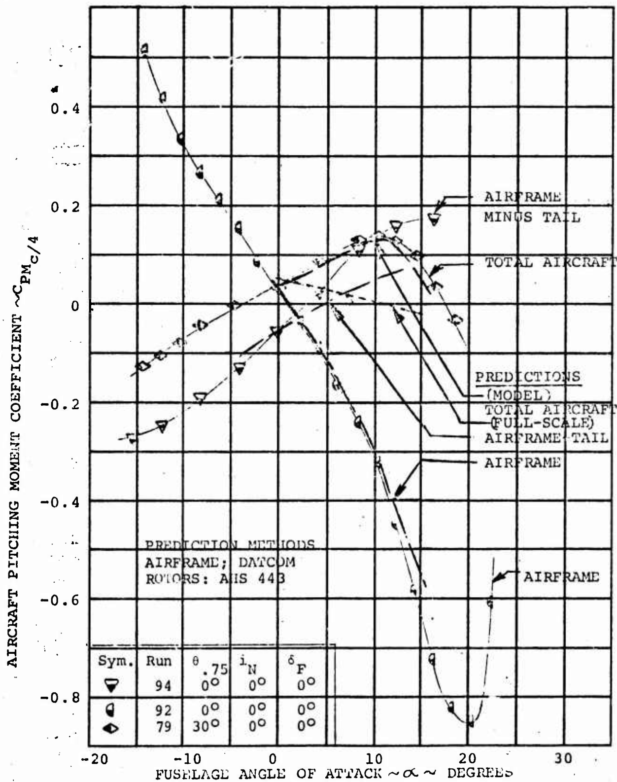
FIGURE 4.25 CONTRIBUTION OF PROP/ROTORS AND HORIZONTAL TAIL TO AIRCRAFT PITCHING MOMENT AT V/V_T = 0.386
