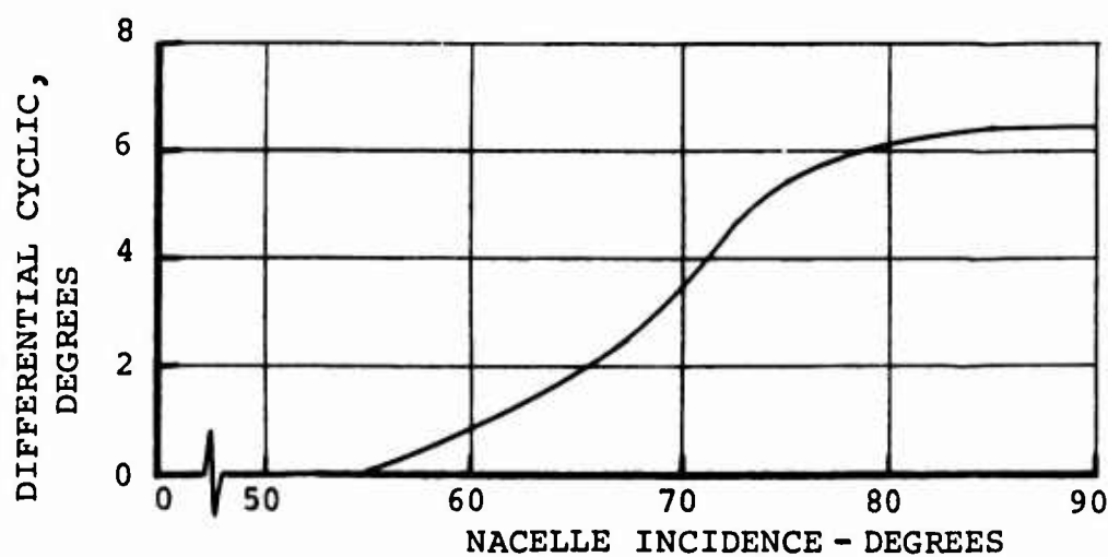
FIGURE 5.33: YAW CONTROL PHASING THROUGH TRANSITION
