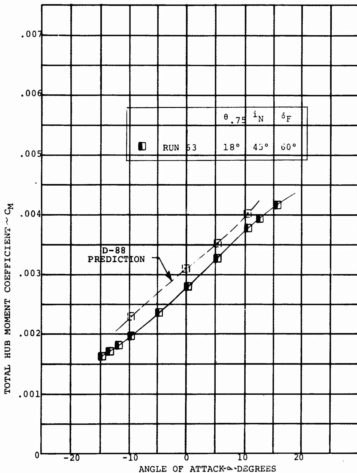
FIGURE 5.25: COMPARISON OF TEST AND PREDICTION FOR TOTAL HUB MOMENT IN TRANSITION
