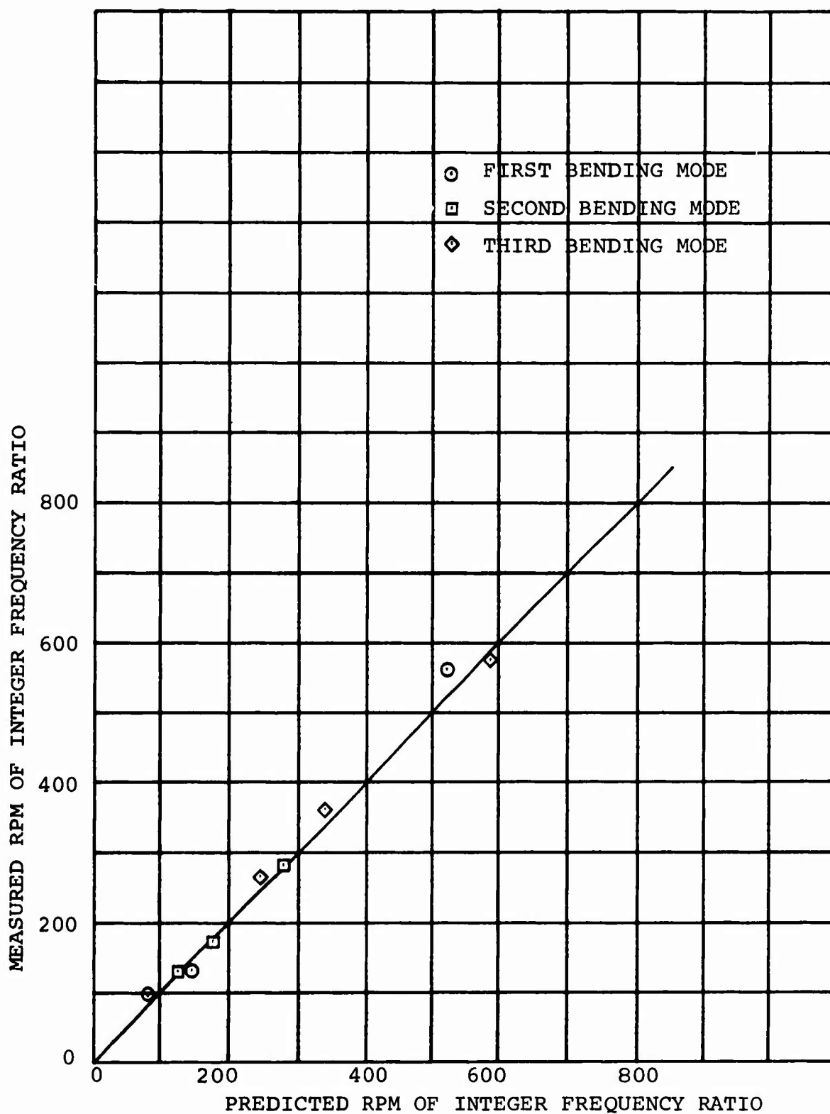
FIGURE 3.8 CORRELATION OF MEASURED AND PREDICTED BLADE FREQUENCIES TILT ROTOR DYNAMIC MODEL
