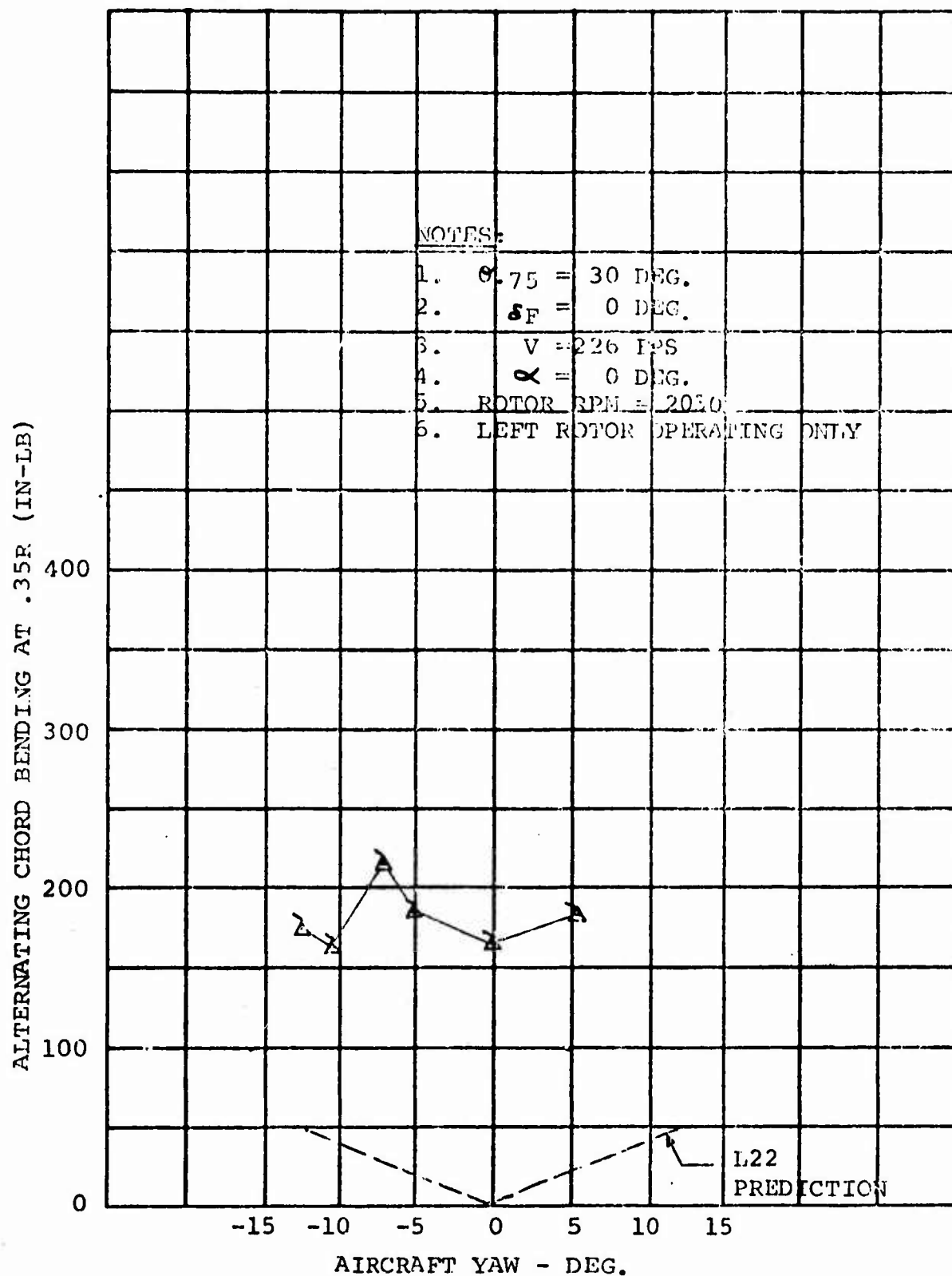
FIGURE 3.31 CORRELATION OF PREDICTED AND MEASURED ALTERNATING BLADE CHORD BENDING MOMENT WITH AIRCRAFT YAW ANGLE VARIATION FOR CRUISE FLIGHT, TILT ROTOR PERFORMANCE MODEL
