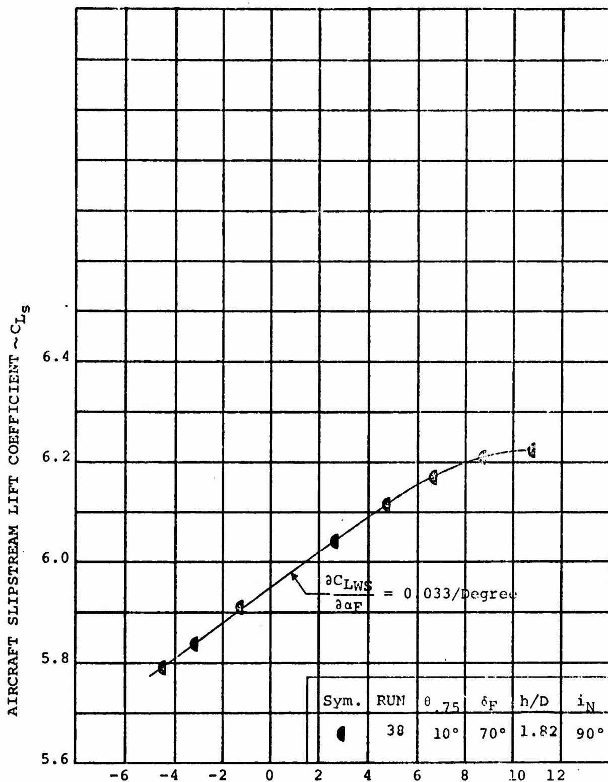
FIGURE 5.13 EFFECT OF ANGLE OF ATTACK ON AIRCRAFT LIFT IN THE NEAR HOVER MODE AT q=4 psf.
