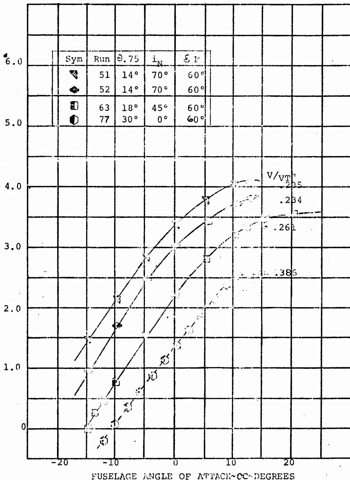
FIGURE 4.18 AIRCRAFT LIFT/ANGLE OF ATTACK VARIATION DURING TRANSITION
