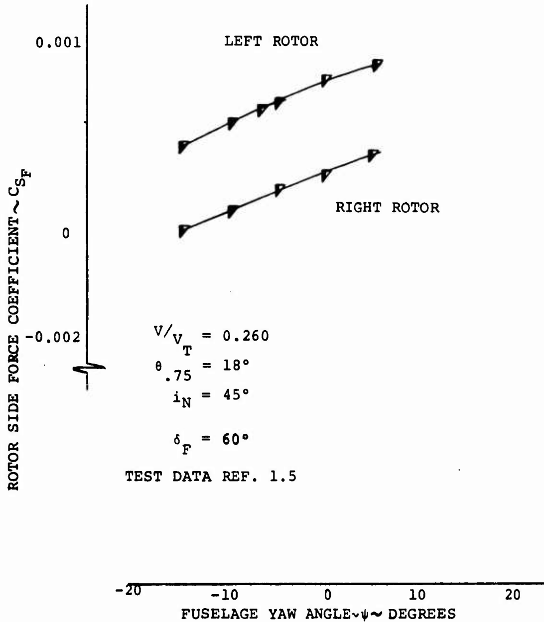
FIGURE 5.26: ROTOR SIDE FORCE IN MID-TRANSITION
