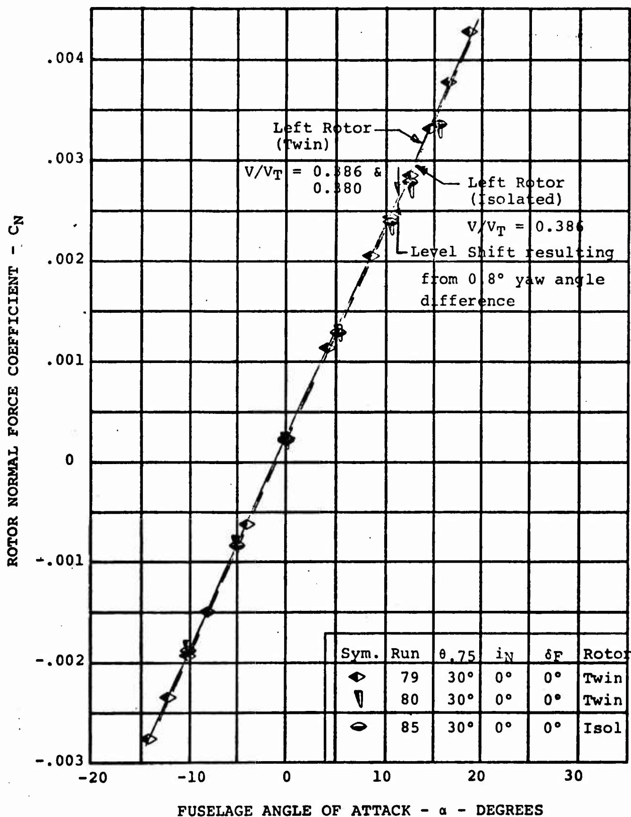
FIGURE 3.57. ROTOR/ROTOR INTERFERENCE EFFECTS ON CRUISE ROTOR CHARACTERISTICS, V/V_T = 0.386
