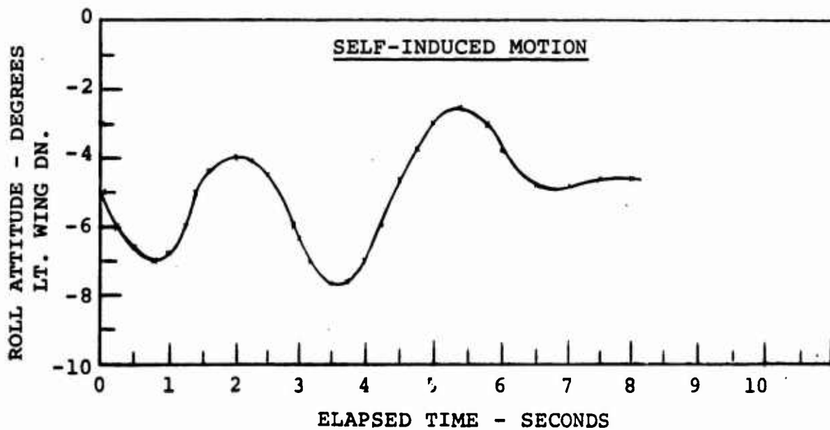
FIGURE 5.21.IGE ROLL STABILITY W/O ATTITUDE STIFFNESS
