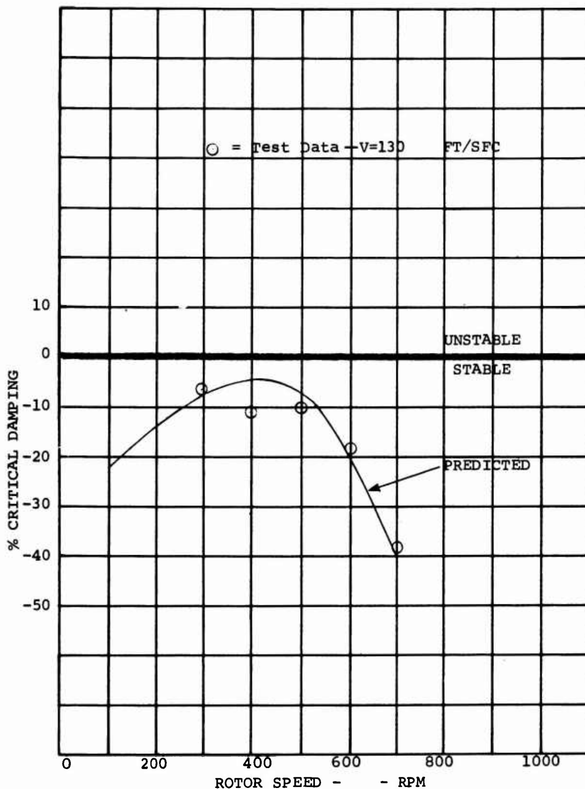
FIGURE. 3.47. DAMPING IN WHIRL MODE ( \Omega - \omega_\beta ) REDUCED TORSION STIFFNESS SPAR, V=130 FT/SEC 1/9 SCALE CONVERSION MODEL
