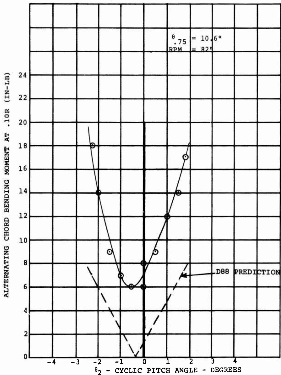
FIGURE 3.19 CORRELATION OF MEASURED AND PREDICTED ROTOR ALTERNATING CHORD BENDING MOMENT IN HOVER WITH CYCLIC PITCH VARIATION- TILT ROTOR DYNAMIC MODEL
