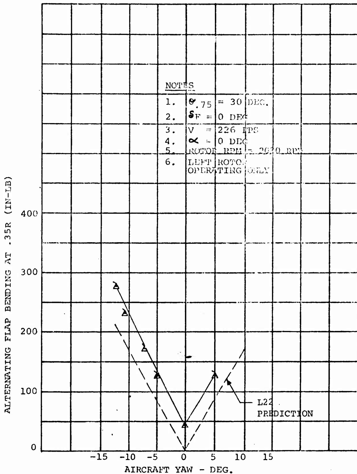
FIGURE 3.30 CORRELATION OF PREDICTED AND MEASURED ALTERNATING BLADE FLAP BENDING MOMENT WITH AIRCRAFT YAW ANGLE VARIATION FOR CRUISE FLIGHT, TILT ROTOR PERFORMANCE MODEL.
