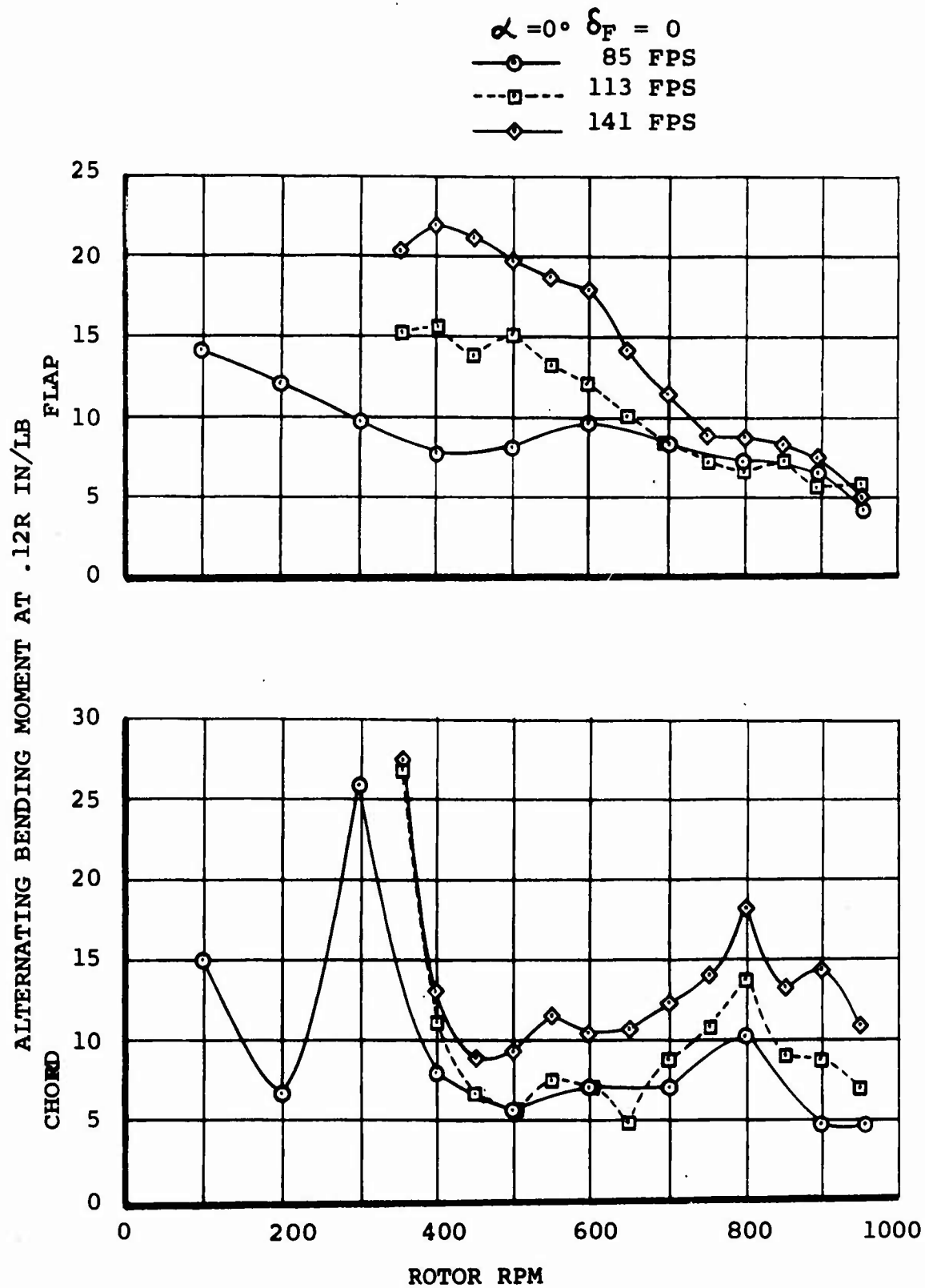
FIGURE 3.13 ALTERNATING BLADE BENDING MOMENTS FOR STEADY WINDMILLING 1/9 SCALE STOWED ROTOR MODEL
