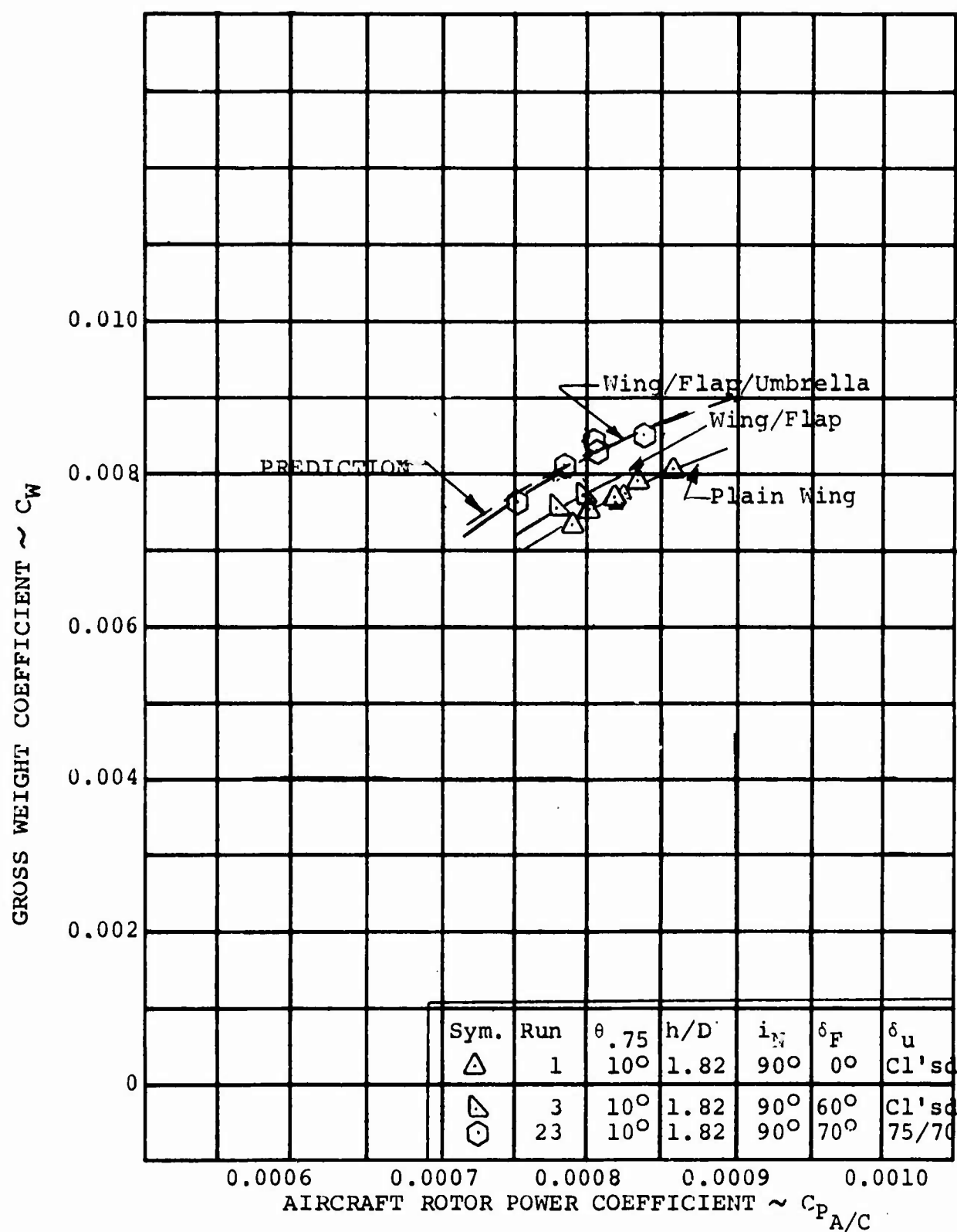
FIGURE 4.12: EFFECT OF UMBRELLA & FLAP ANGLE ON TOTAL AIRCRAFT HOVER PERFORMANCE
