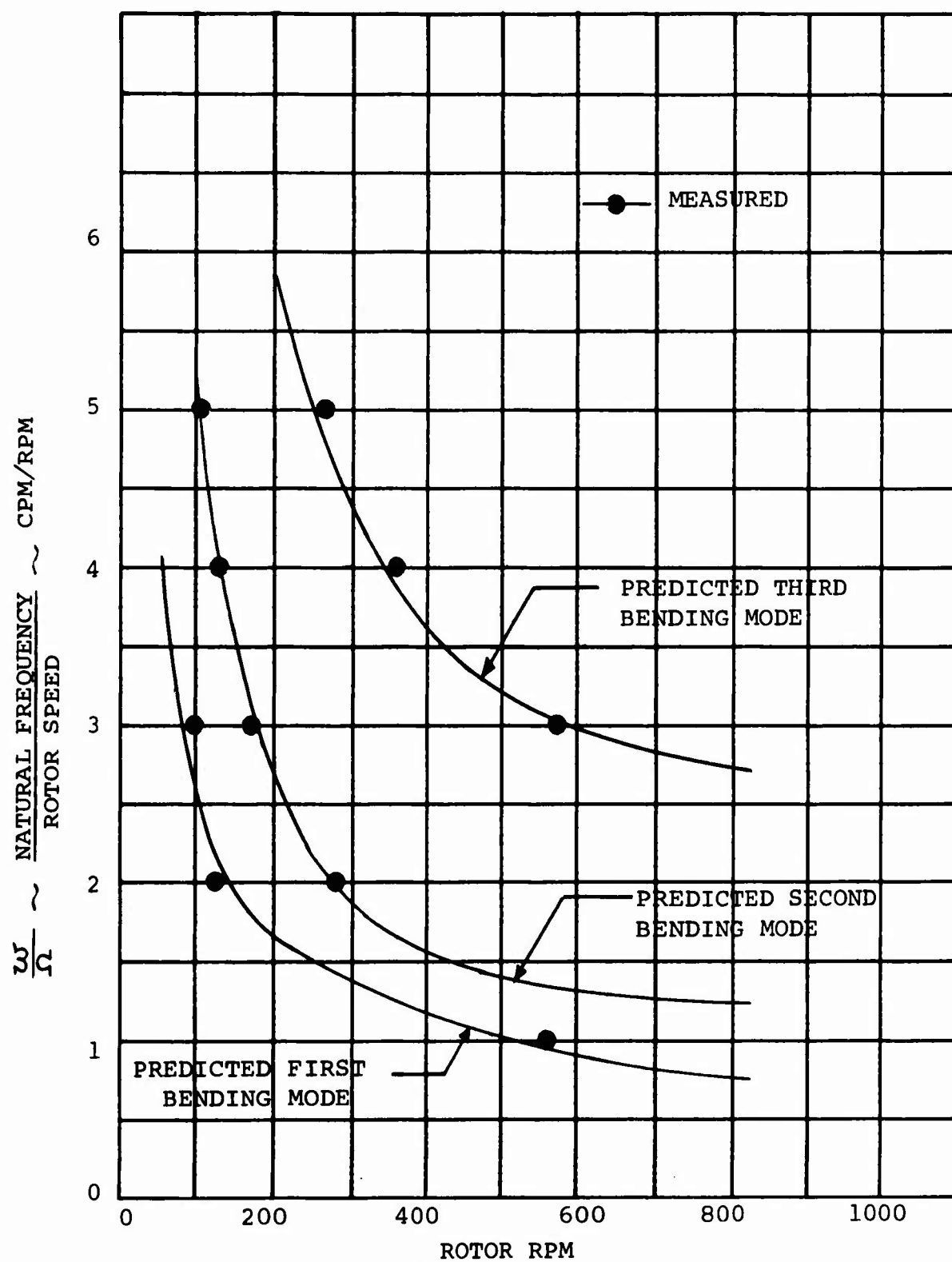
FIGURE 3.6 PREDICTED AND MEASURED ROTOR BLADE NATURAL FREQUENCIES FOR \theta_{.75} = 3 DEG. TILT ROTOR DYNAMIC MODEL
