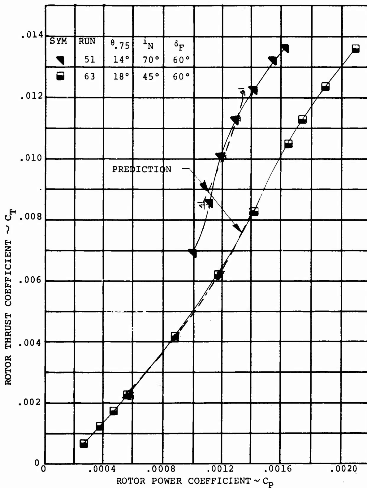
FIGURE 4.14: COMPARISON OF TEST AND PREDICTION FOR ROTOR THRUST/POWER COEFFICIENT VARIATION IN TRANSITION
