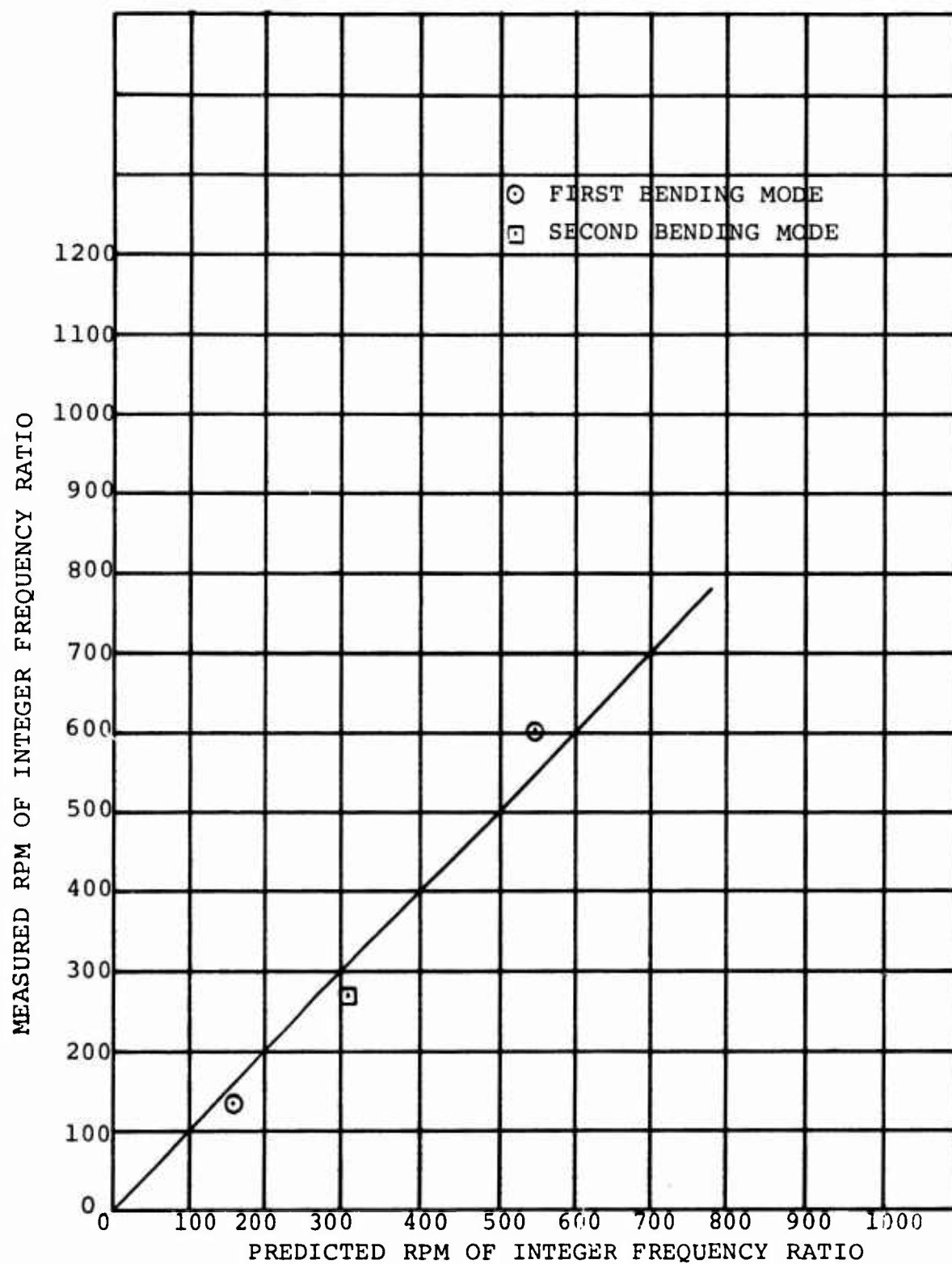
FIGURE 3.9 CORRELATION OF MEASURED AND PREDICTED BLADE FREQUENCIES 1/9 SCALE CONVERSION MODEL
