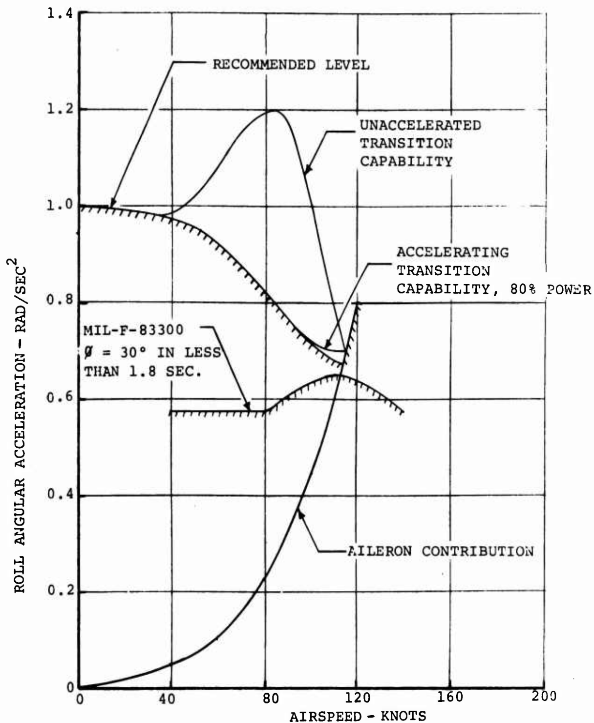
FIGURE 5.30: ROLL CONTROL POWER THROUGH TRANSITION
