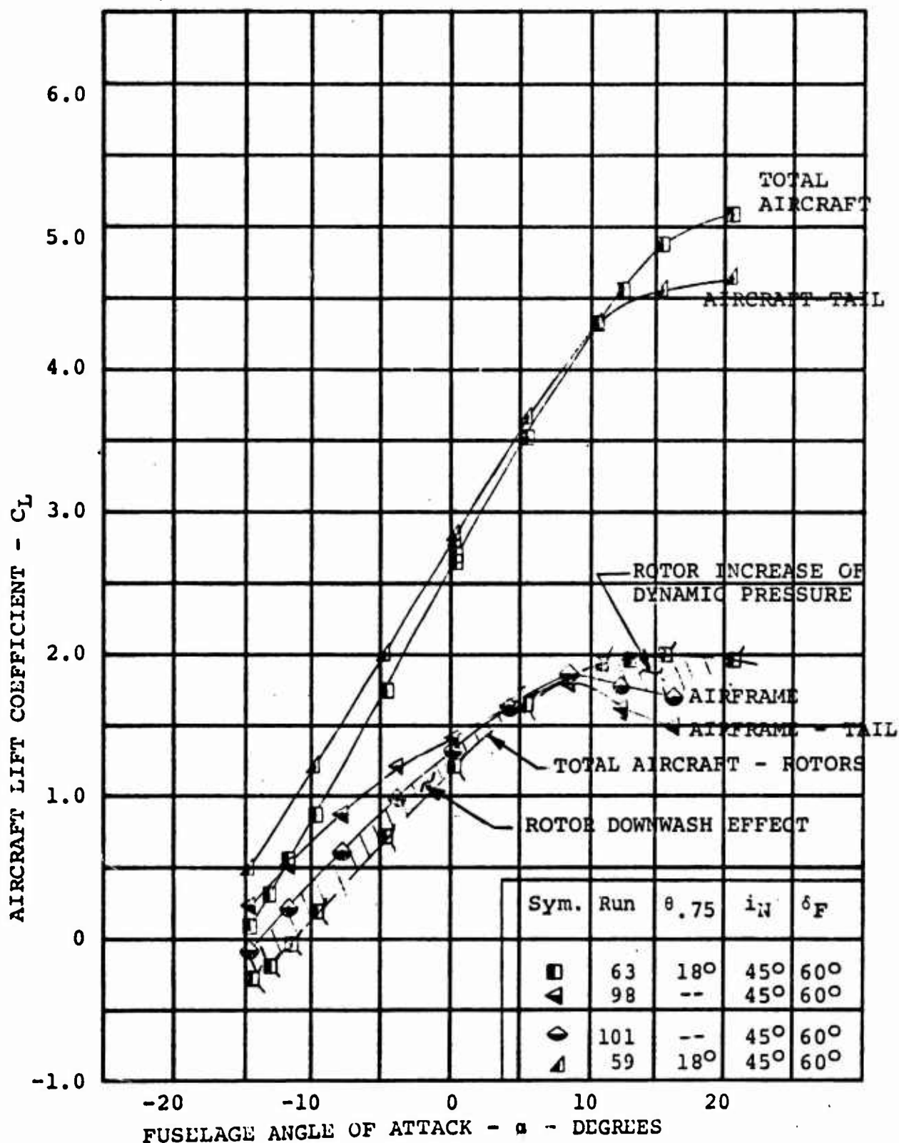
FIGURE 4.17 CONTRIBUTION OF PROP/ROTOR AND HORIZONTAL TAIL TO AIRCRAFT LIFT AT V/V_T = 0.260 WITH i_N = 45^\circ
