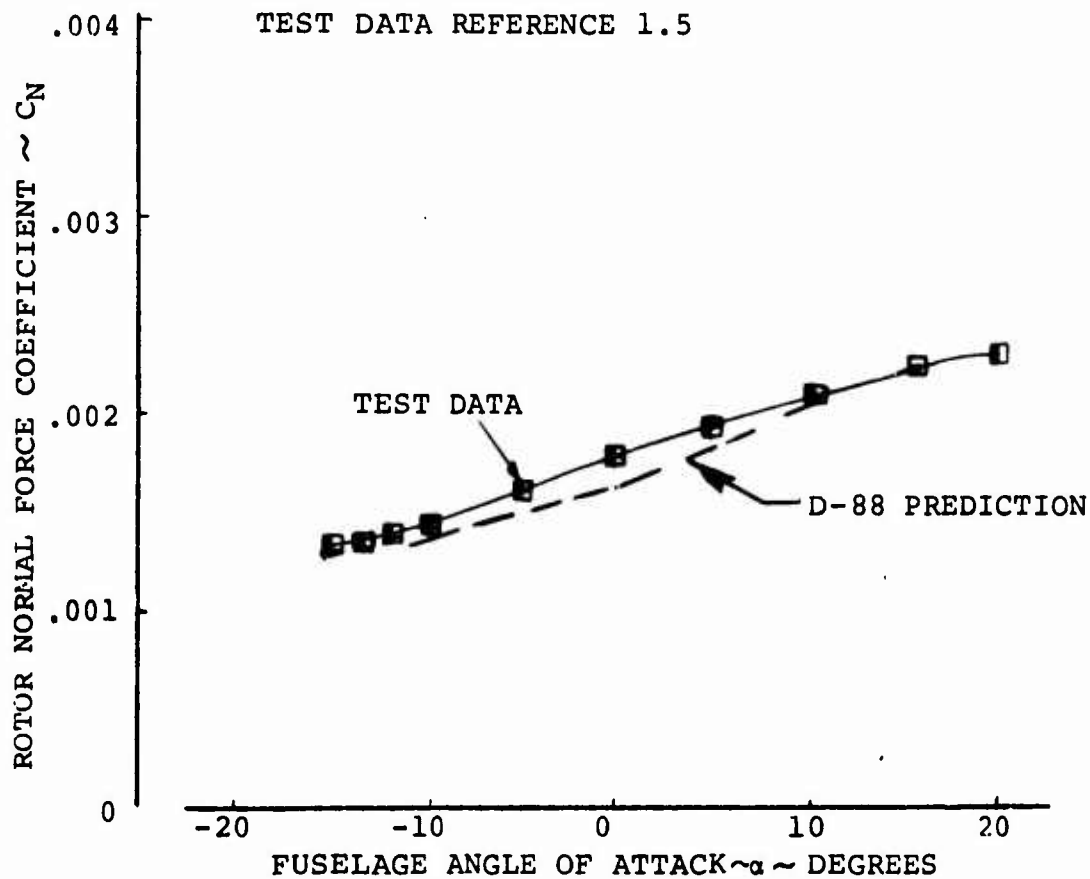
FIGURE 5.24: COMPARISON OF TEST DATA AND PREDICTION OF ROTOR NORMAL FORCE IN MID-TRANSITION
