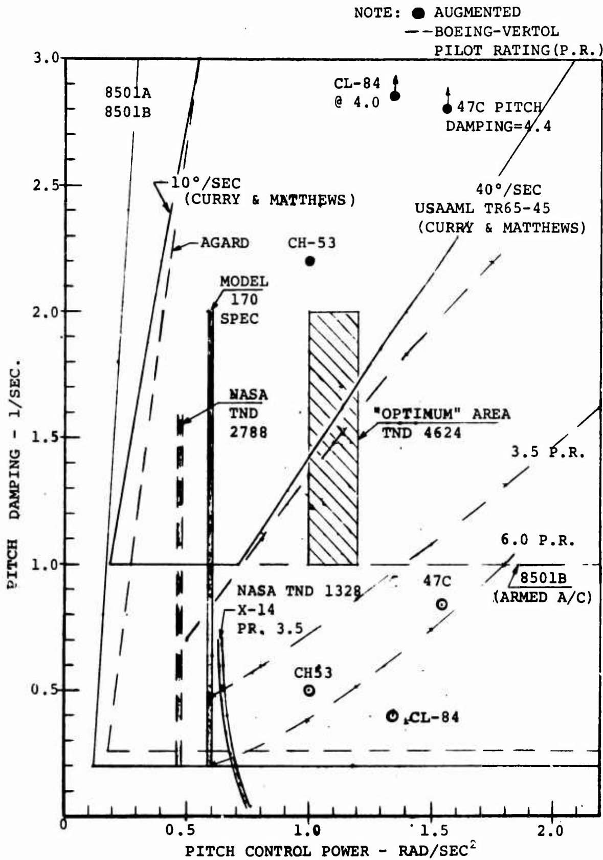
FIGURE 5.16. PITCH CONTROL POWER
