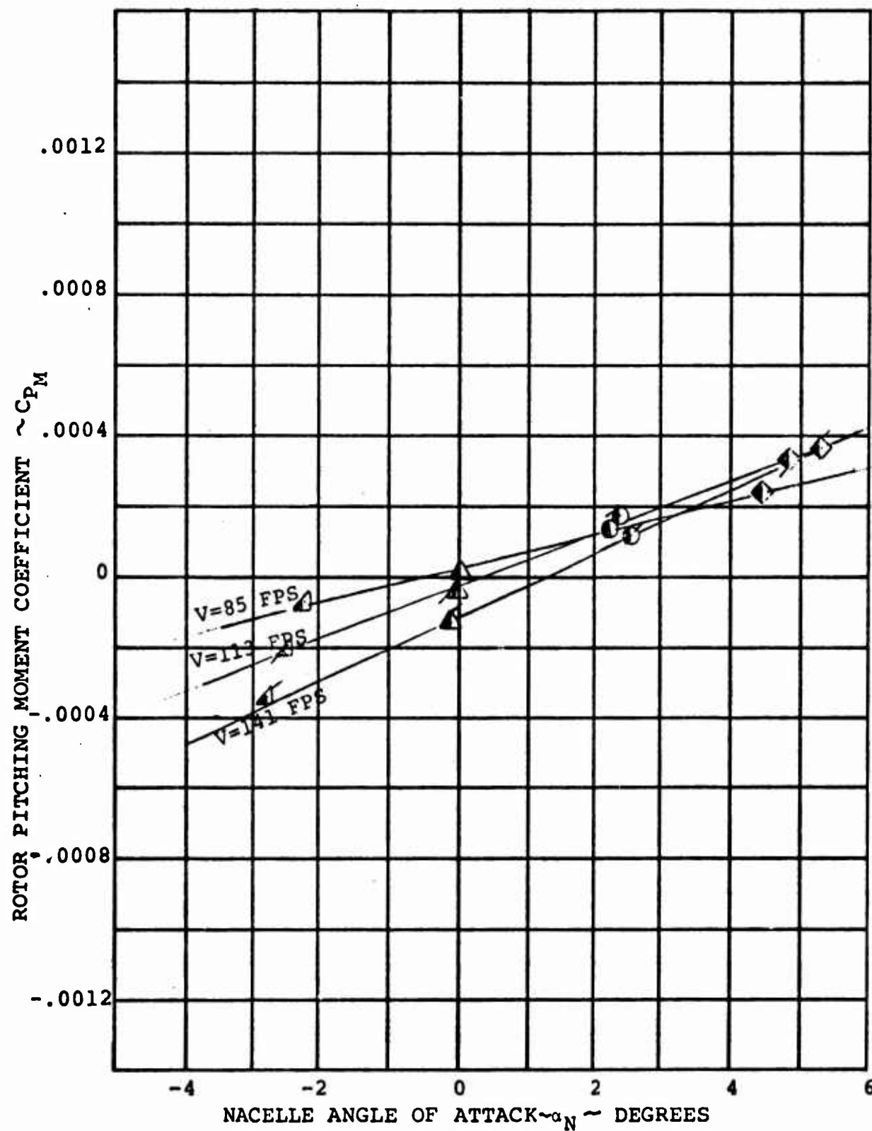
FIGURE 5.41. ROTOR PITCHING MOMENT/NACELLE ANGLE OF ATTACK FOR ROTOR RPM = 950 \delta_f = 0^\circ
