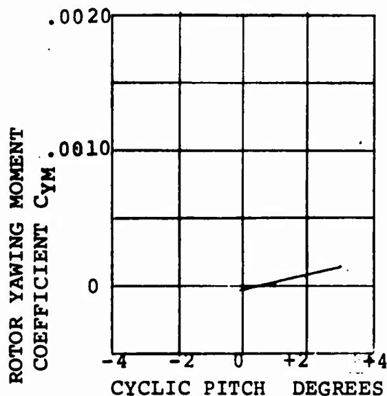
FIGURE 5.20: CYCLIC PITCH EFFECTIVENESS FOR HOVER YAW CONTROL
