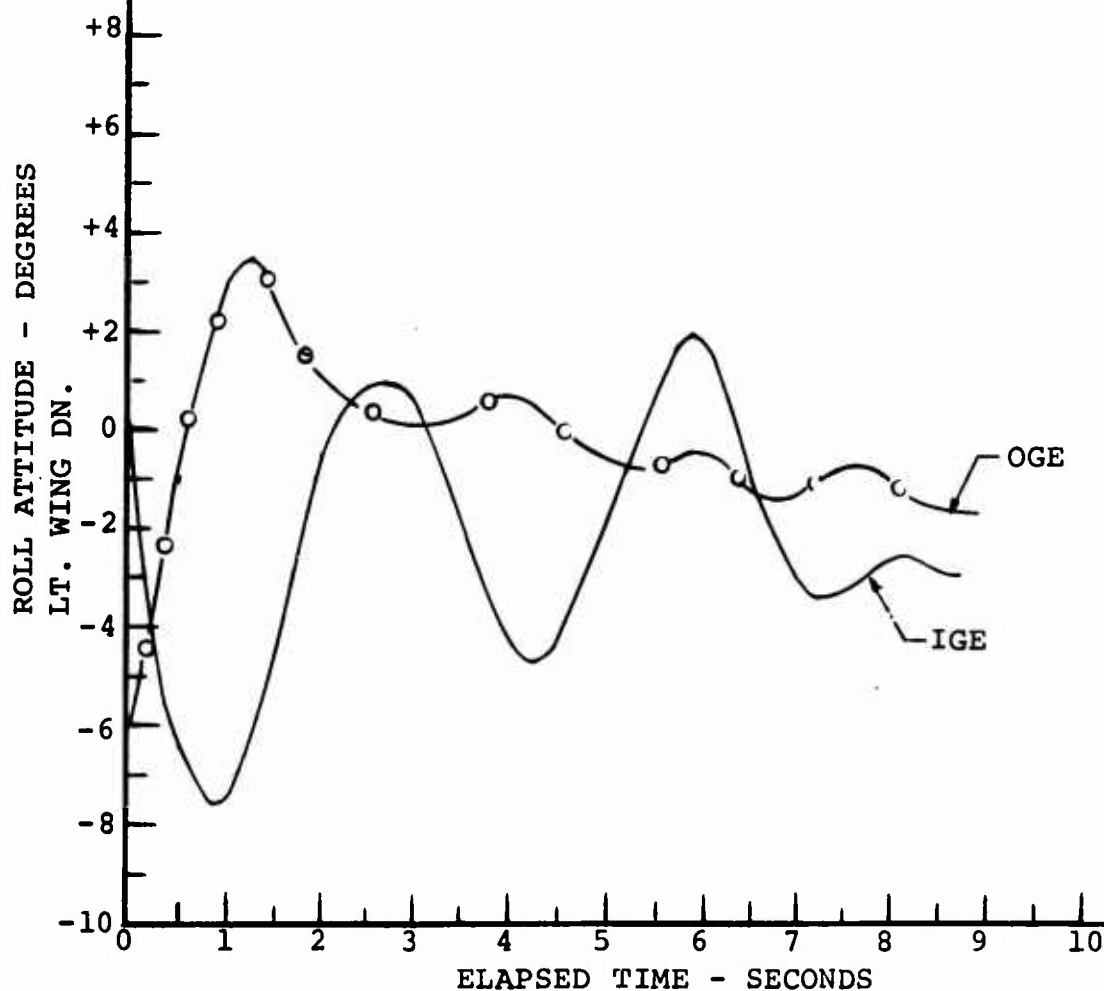
FIGURE 5.22. IGE/OGE ROLL STABILITY W/O ATTITUDE STIFFNESS
