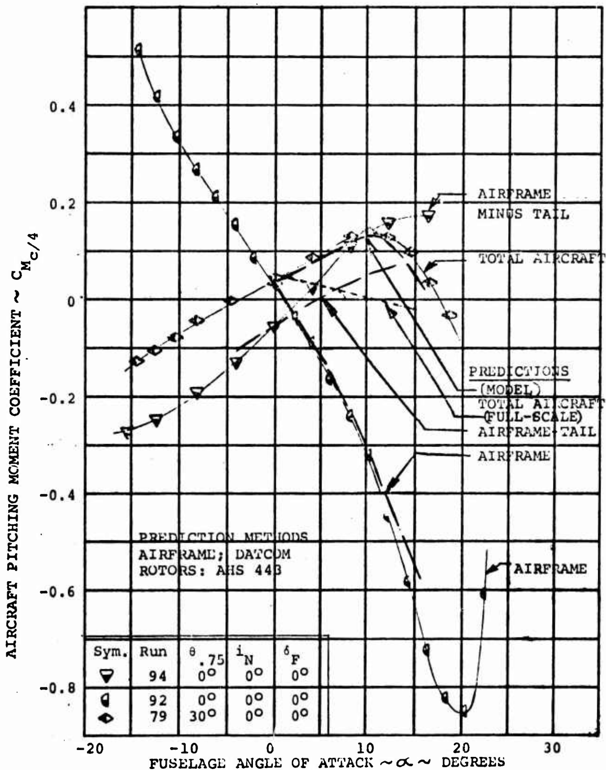
FIGURE 5.60. CONTRIBUTION OF PROP/ROTORS AND HORIZONTAL TAIL TO AIRCRAFT PITCHING MOMENT AT V/V_T = 0.386
