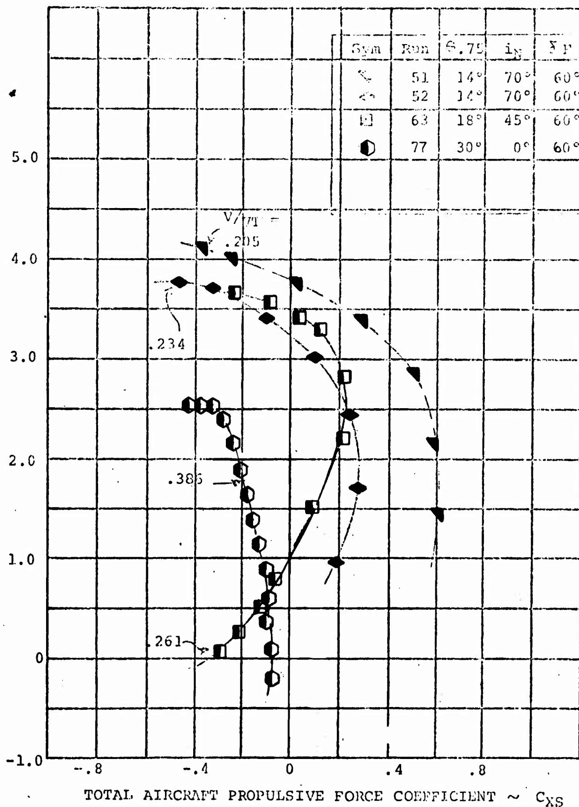
FIGURE 4.19 AIRCRAFT LIFT/PROPULSIVE FORCE VARIATION DURING TRANSITION
