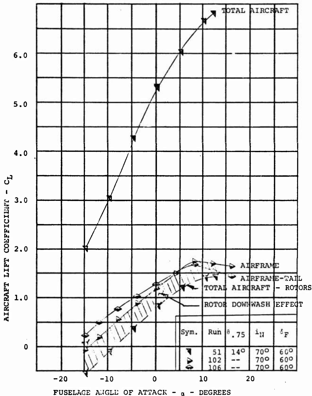
FIGURE 4.16 CONTRIBUTION OF PROP/ROTOR AND HORIZONTAL TAIL TO AIRCRAFT LIFT AT V/V_T = 0.206 WITH i_N = 70^\circ
