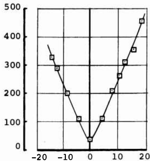
FIGURE 3.12 EFFECT OF AIRCRAFT PITCH ON BLADE ROOT BENDING MOMENTS IN CRUISE FLIGHT
