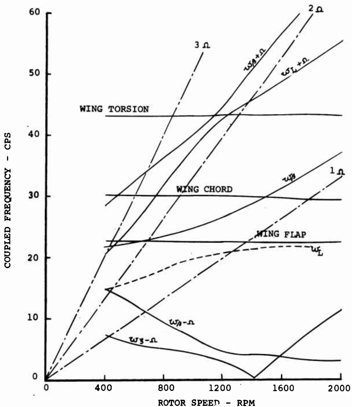
FIGURE 3.41 FREQUENCY SPECTRUM FOR 1/16 SCALE CONVERSION MODEL - CRUISE MODE V = 135 FPS
