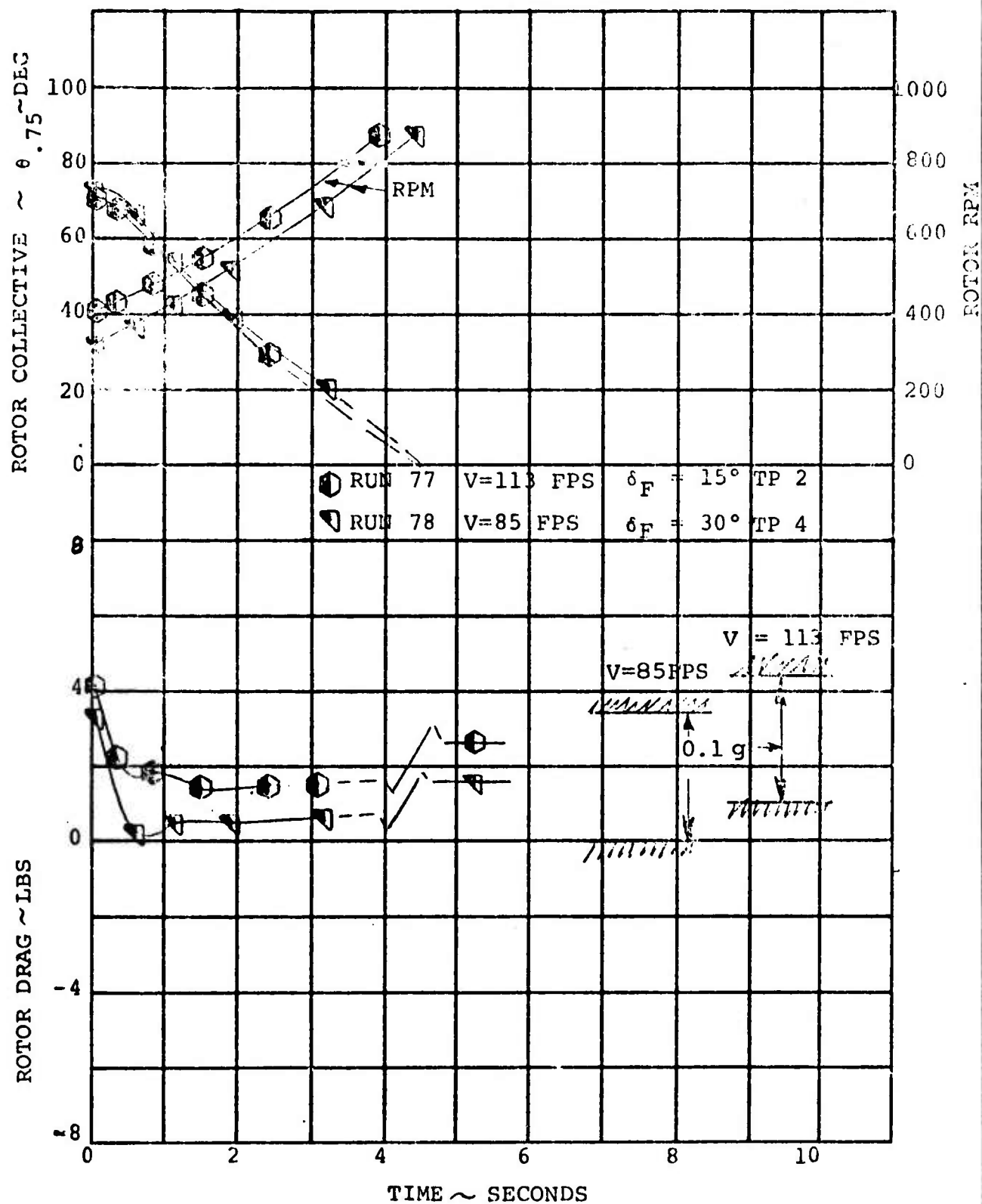
FIGURE 5.72. EFFECT OF FORWARD SPEED ON ROTOR DRAG DURING FEATHER FOR 4.5 LINEAR COLLECTIVE RATE, INITIAL RPM = 715
