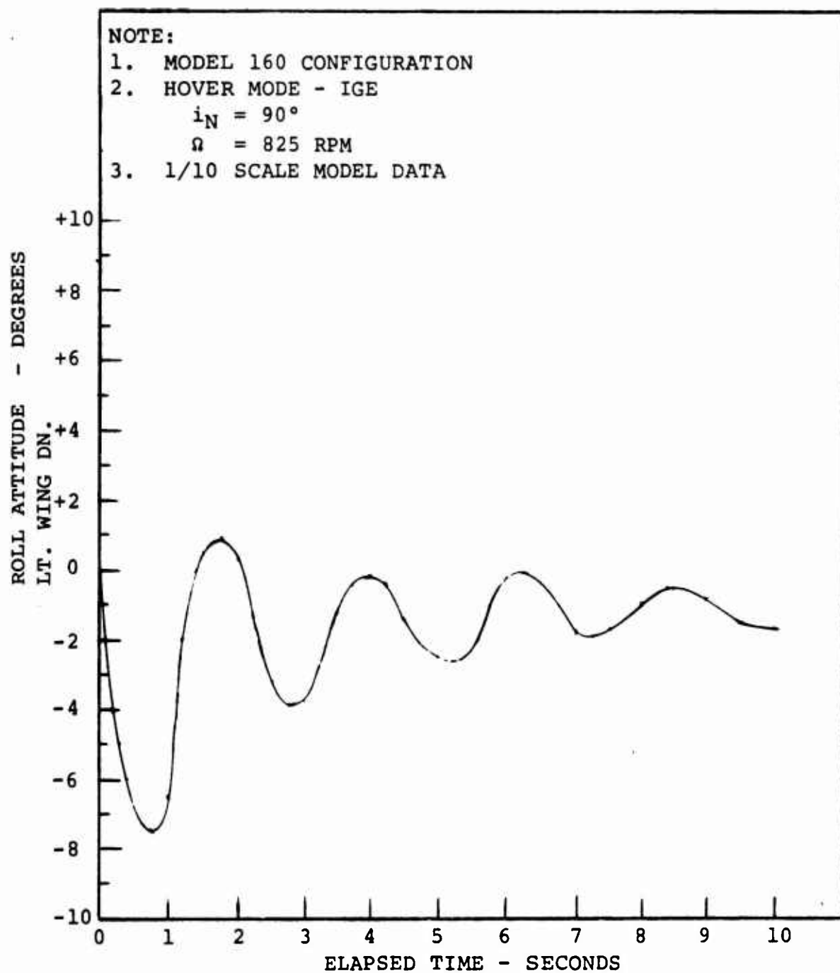
FIGURE 5.23. IGE ROLL STABILITY W/ ATTITUDE STIFFNESS
