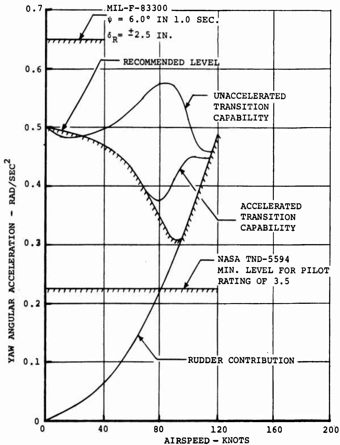
FIGURE 5.32: YAW CONTROL POWER THROUGH TRANSITION
