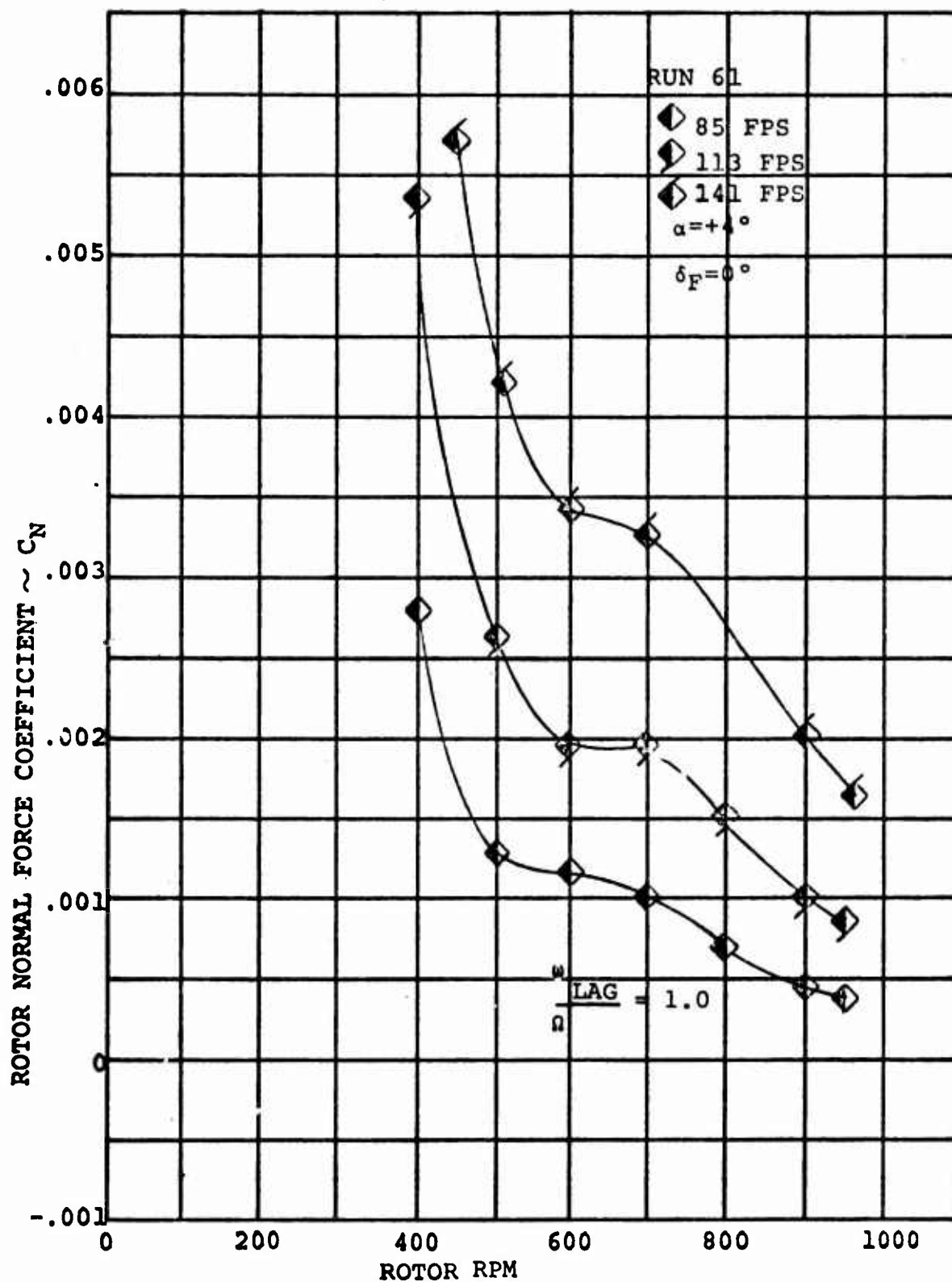
FIGURE 5.38. ROTOR NORMAL FORCE/RPM VARIATION FUSELAGE ATTITUDE = +4^\circ \delta_F = 0^\circ (STEADY WINDMILLING)
