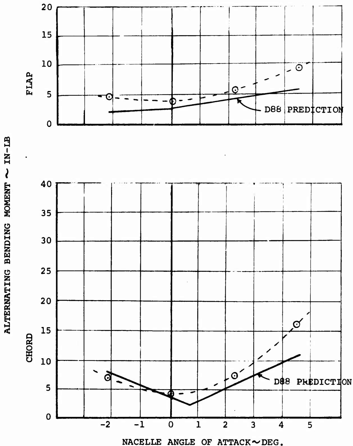
FIGURE 3.40 CORRELATION OF MEASURED AND PREDICTED BLADE BENDING MOMENT FOR STEADY WINDMILLING ROTOR 1/9 SCALE CONVERSION MODEL
