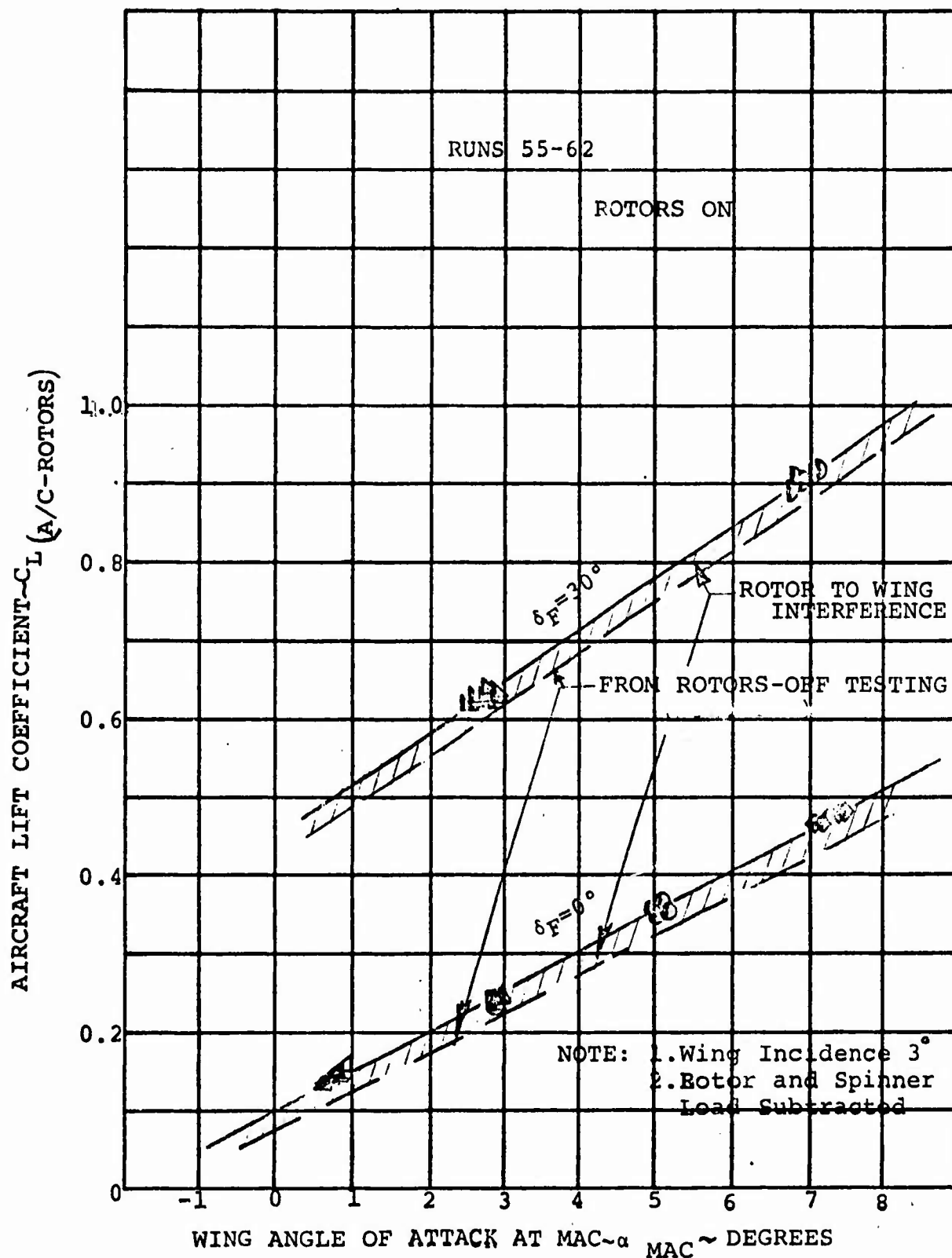
FIGURE 4.33 AIRFRAME LIFT/ANGLE OF ATTACK VARIATION FOR FLAP DEFLECTIONS OF 0^\circ AND 30^\circ
