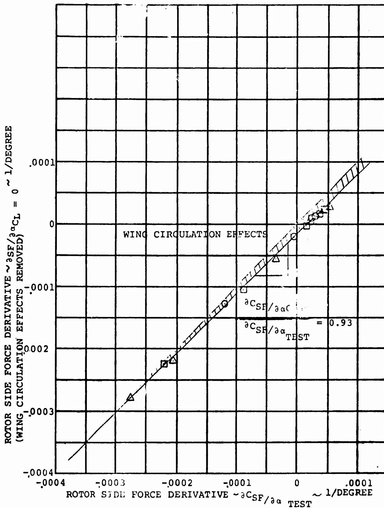
FIGURE 5.51. COMPARISON OF ROTOR SIDE FORCE DERIVATIVES WITH AND WITHOUT WING CIRCULATION EFFECTS
