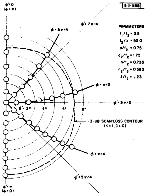
Fig. 11. Theoretical scan-coverage diagram with magnification of 3.5 and 1/2° beam.
