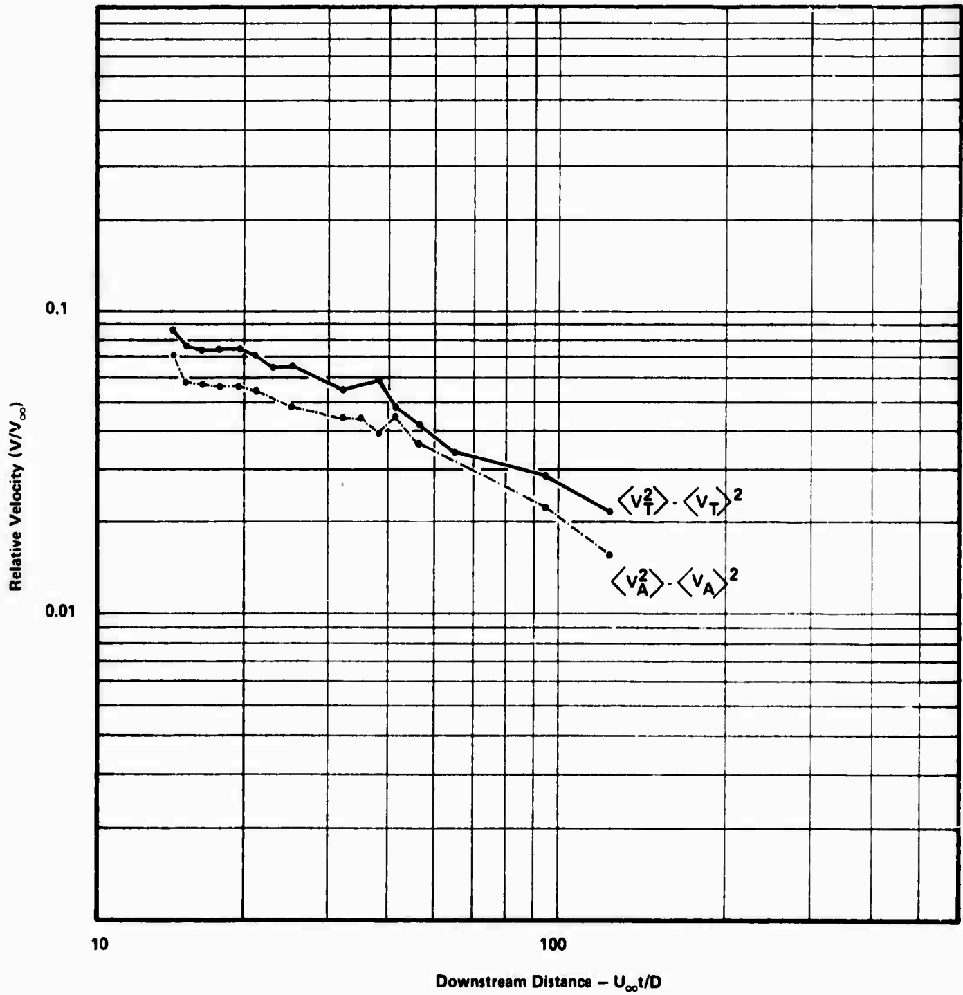
Figure 11. Axial and Transverse RMS Turbulent Relative Velocities.
