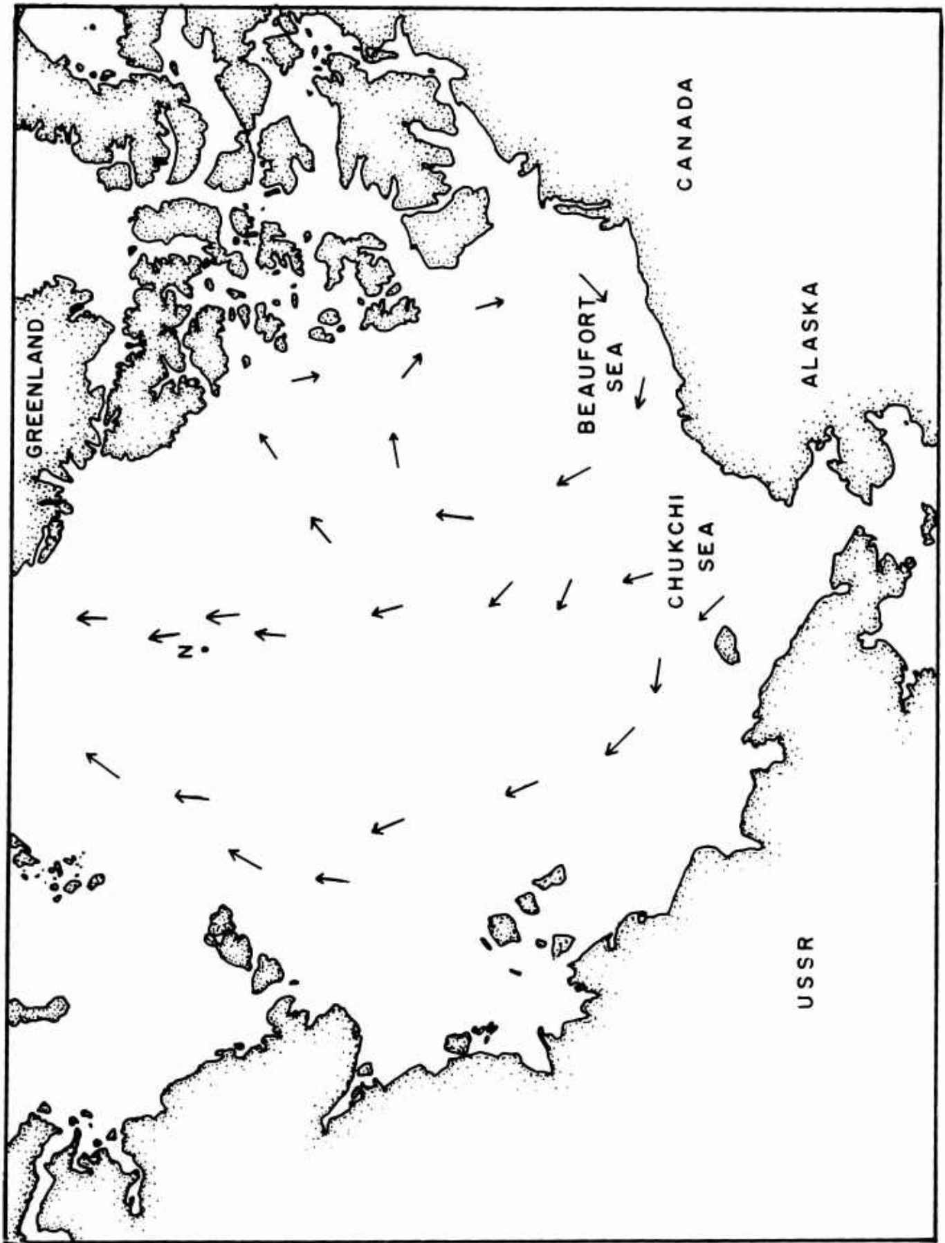
Figure A. Diagrammatic map showing the general surface circulation of the Arctic Ocean (after Harding, 1966).
