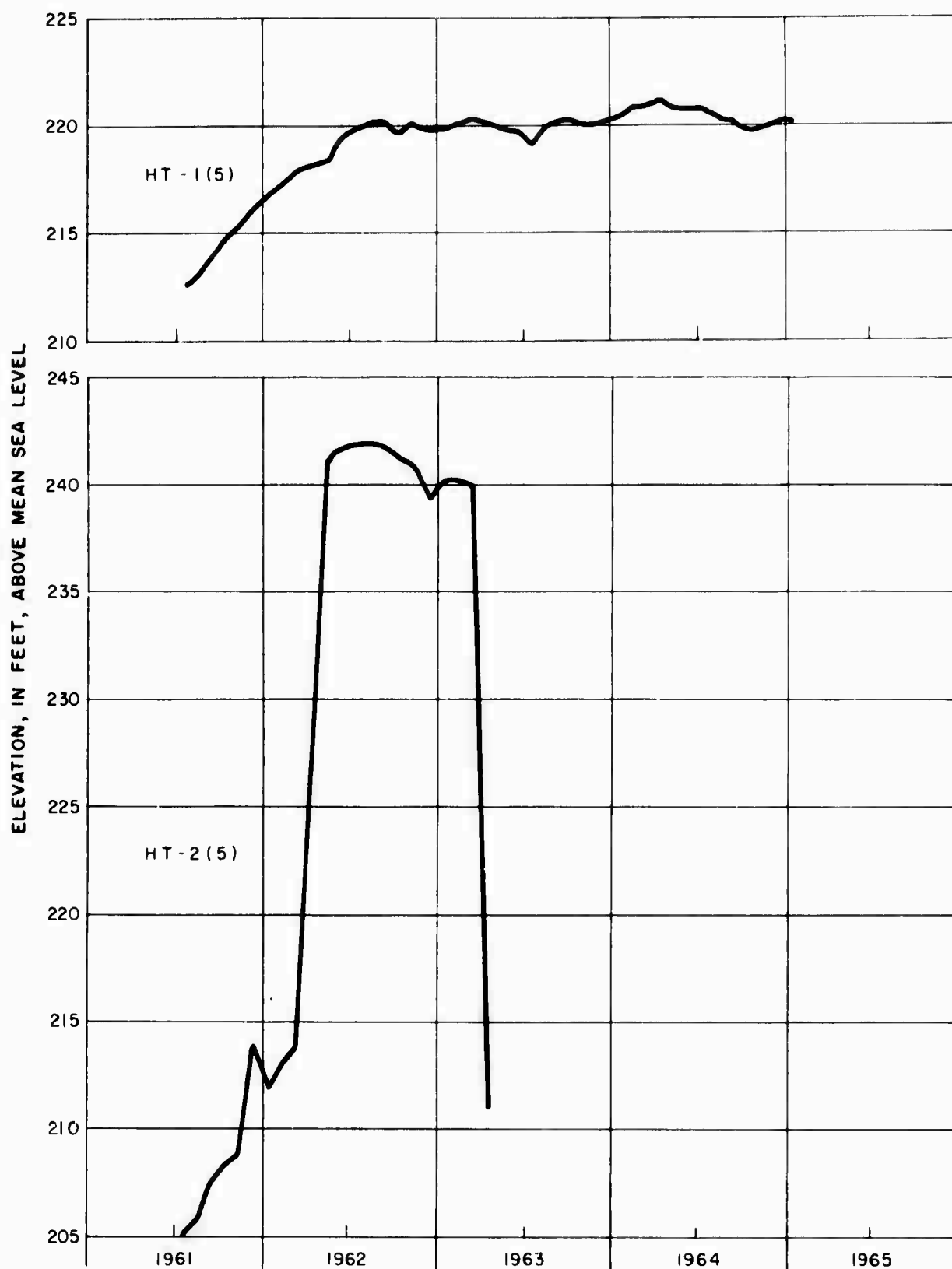
Figure 5.1 Hydrographs for wells HT-1(5) and HT-2(5) in the Cook Mountain Limestone (Aquifer 5).
