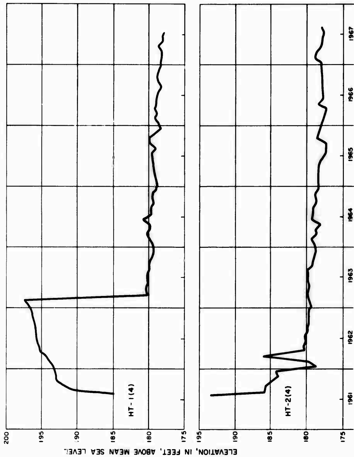
Figure 5.2 Hydrographs for wells HT-1(4) and HT-2(4) in the Vicksburg Group (Aquifer 4).
