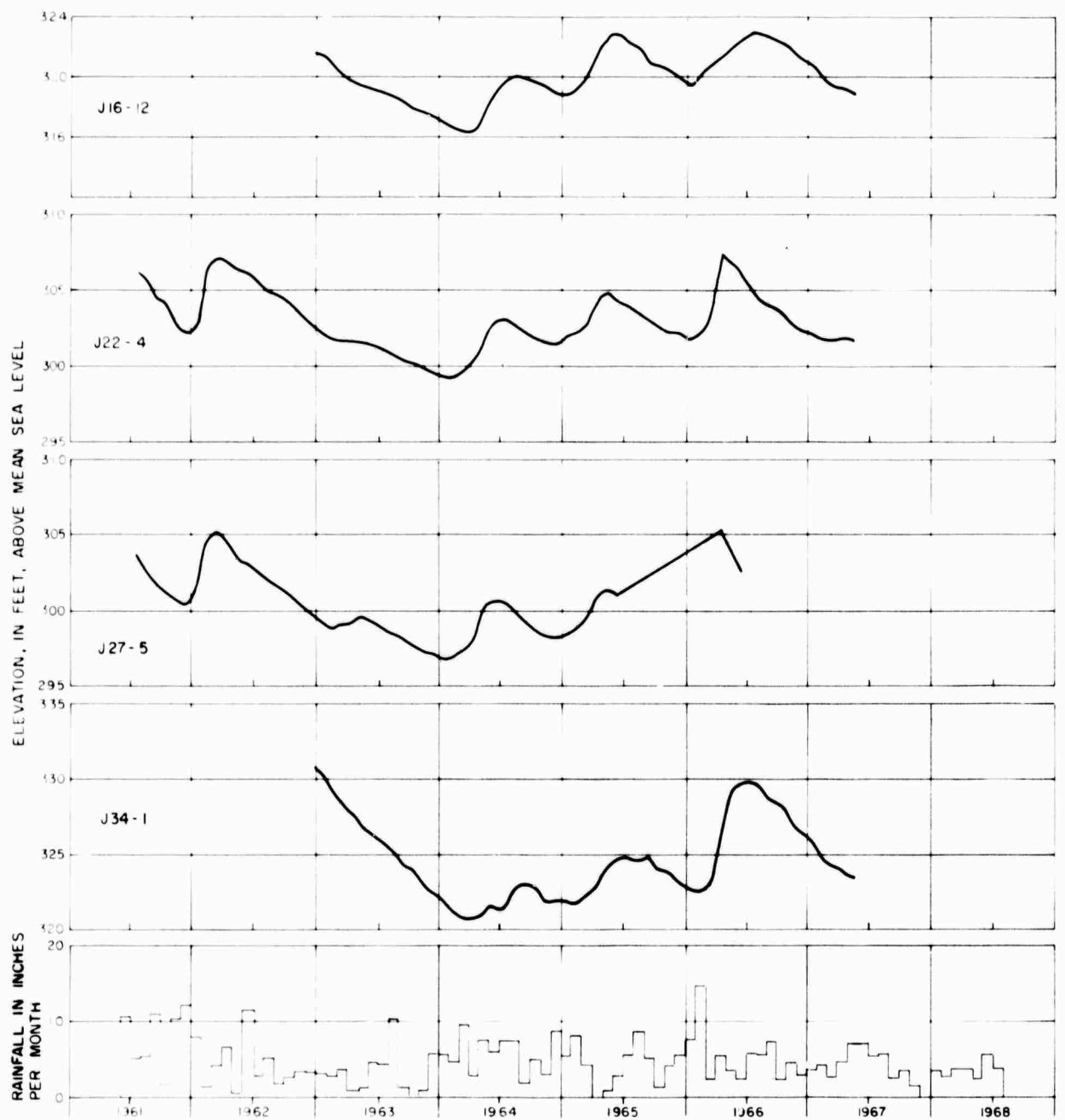
Figure 5.7 Area precipitation and hydrographs for wells
