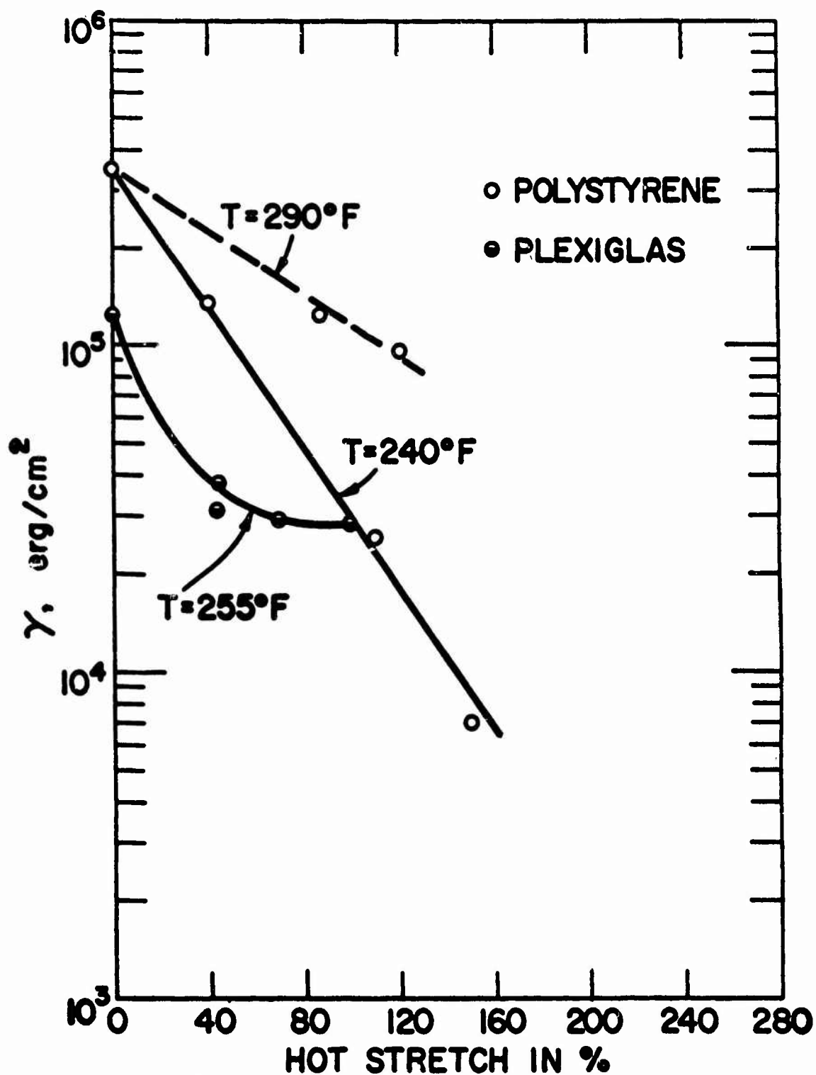
FIGURE 8. FRACTURE SURFACE WORK FOR ORIENTED POLYMERS (BROUTMAN, REF. 9).
