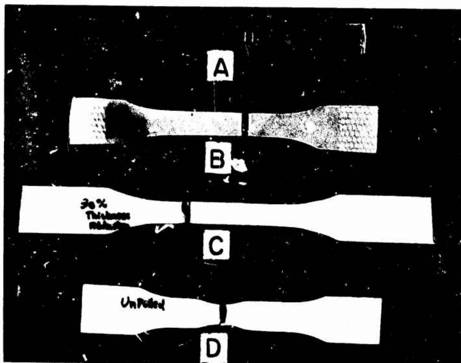
THICKNESS REDUCTION BY ROLLING A: 74 % , B: 60 % , C: 30 % , AND D: UNROLLED.
