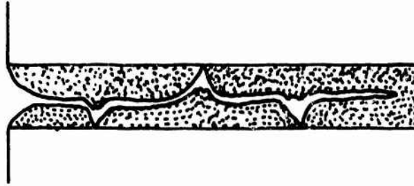
i) CAVITATION OF THE CRAZE AND FINAL SEPARATION BY TEARING OF THE MATERIAL IN THE CRAZE LAYER
