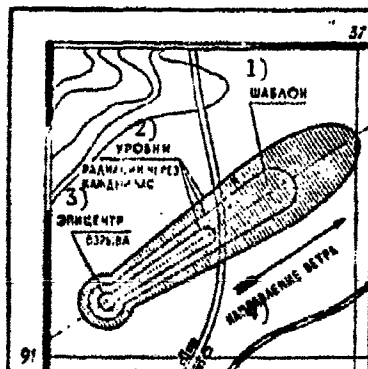
Figure 20. Forecasting boundaries of radioactive fallout zone. KEY: 1, Template; 2, Levels of radiation after each hour; 3, Explosion epicenter; 4, Wind direction.
