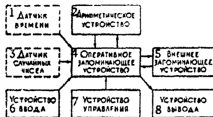
Figure 19. Block diagram of electronic computer. KEY: 1, Time pickup; 2, arithmetic unit; 3, random numbers pickup; 4, operational memory bank; 5, external memory bank; 6, input system; 7, control system; 8, readout system.
