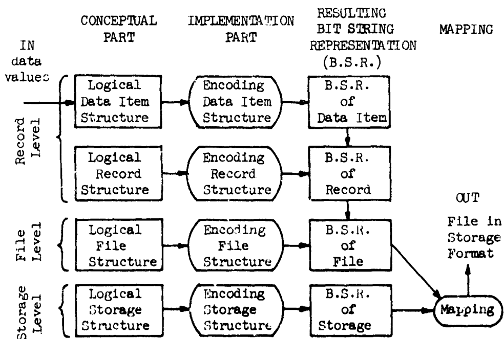
Figure 1-1. The Components of a Data Structure and their Interrelationships
