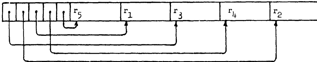
Figure 4-6. File Linked by a Pointer Table
