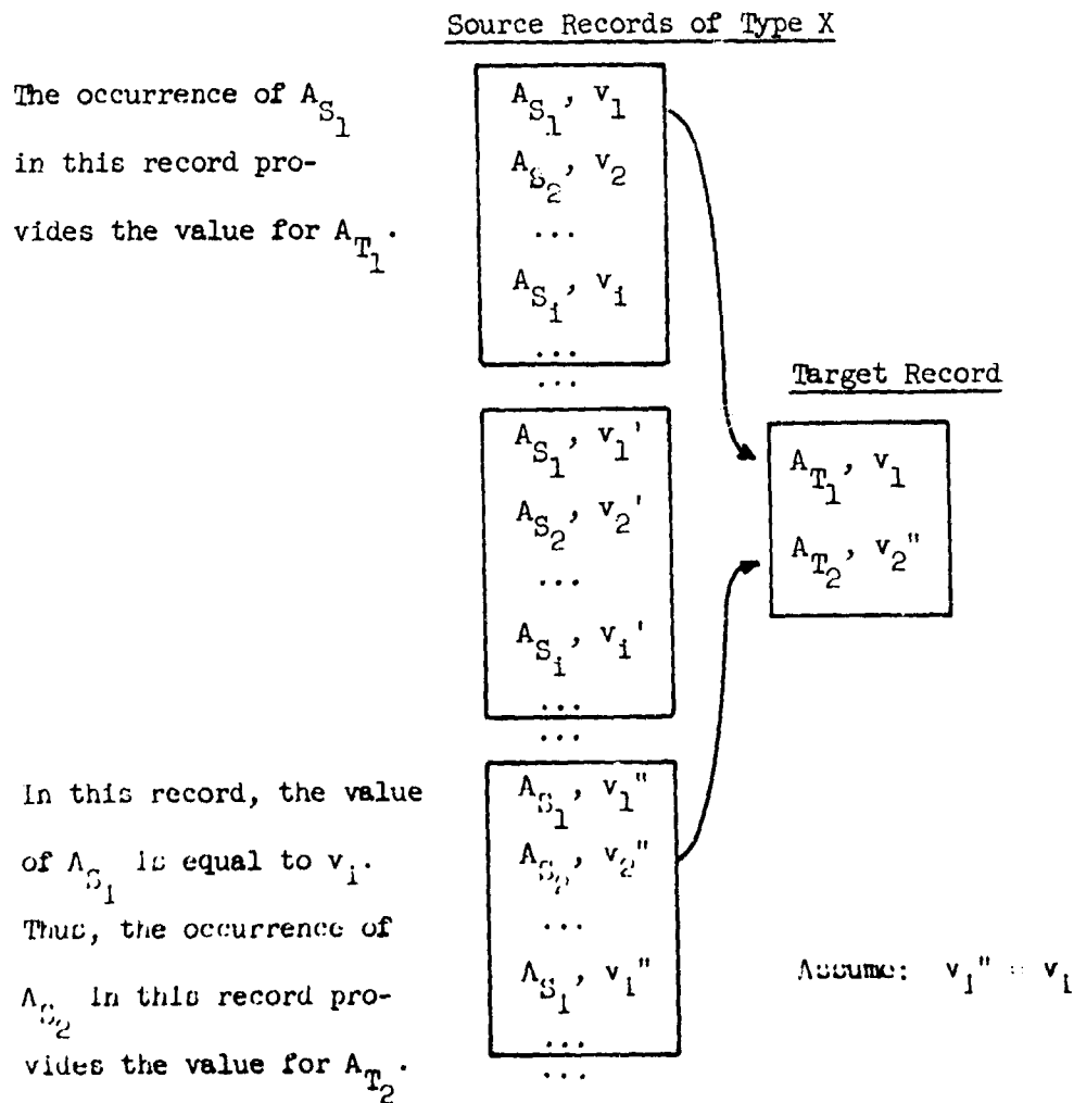
Figure 6-2. An Example of Source Record Selection for the Formation of Target Records
