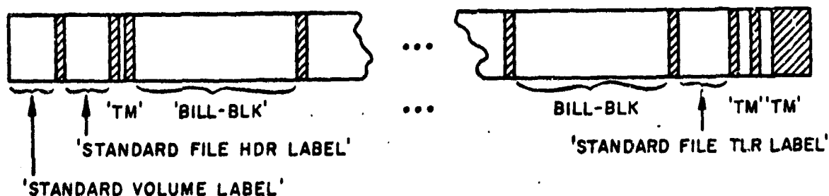
Figure 2-3 Storage Image of BILL-FILE
