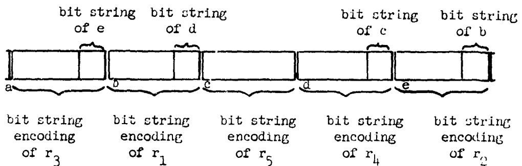
Figure 4-3. Bit String Representation of File Encoded by Embedded Pointers
