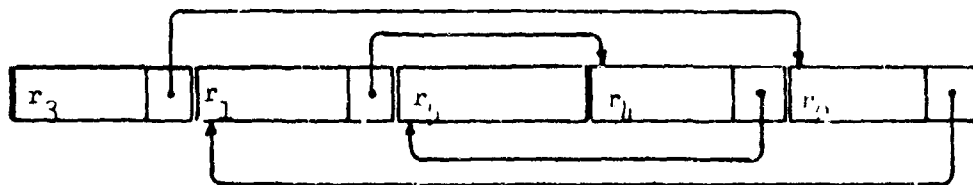
Figure 4-4. File Linked by Embedded Pointers
