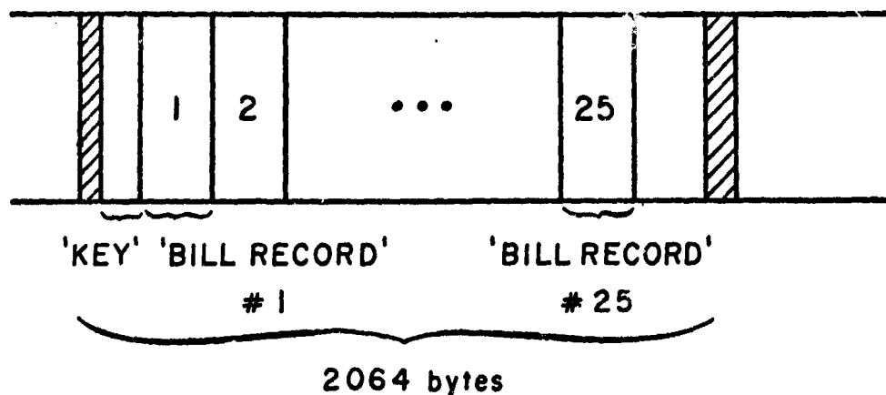
Figure 2-4 Storage Structure of 'BILL-BLK'
