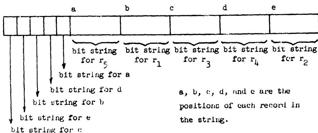
Figure 4-5. Bit String Representation of File Encoded by a Pointer Table
