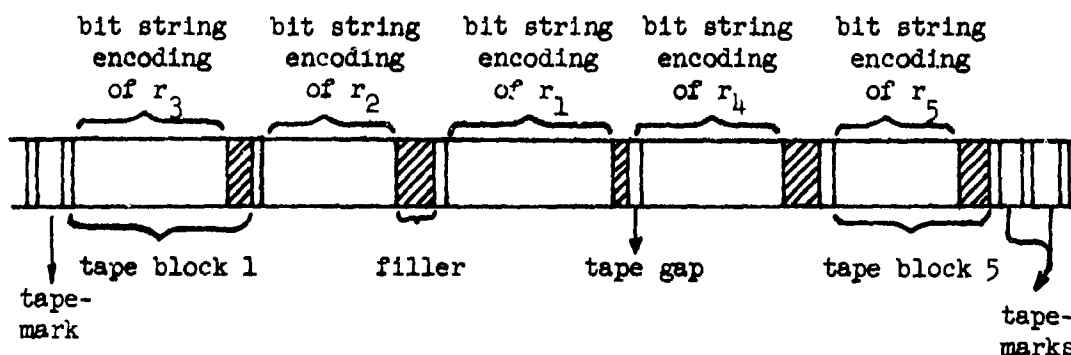
Figure 5-3. Bit String Representation of Tape File X
