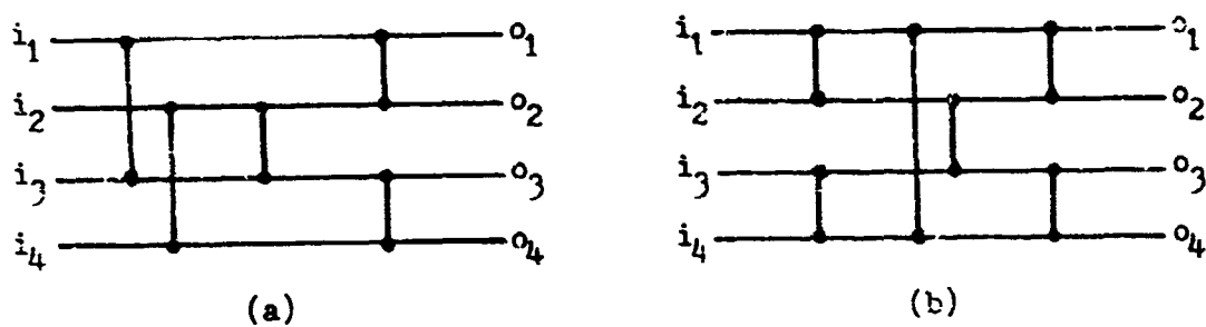
Fig. 2. Which of these is a 4-sorter network?
