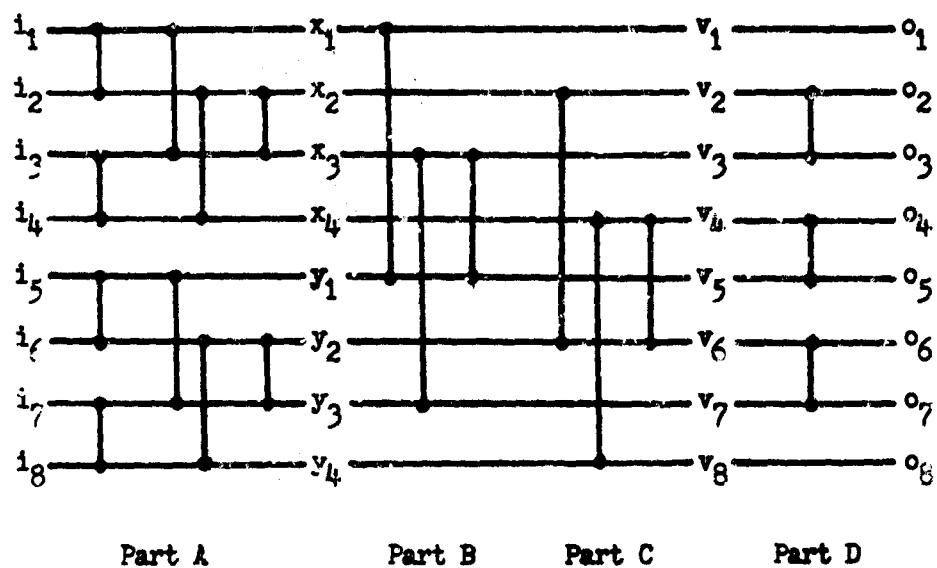
Fig. 7. Batcher's 8-sorter network.
