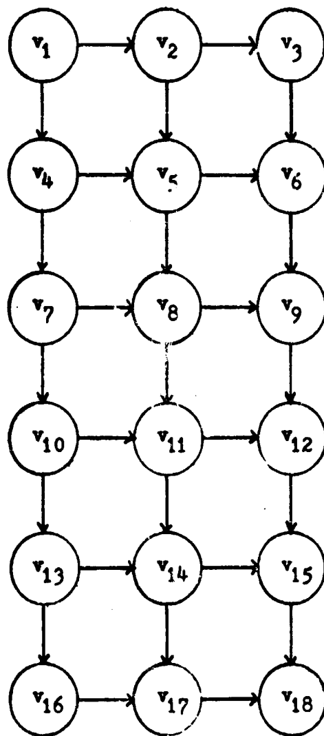
Fig. 14. V for the [6,3] 18-sorter.
