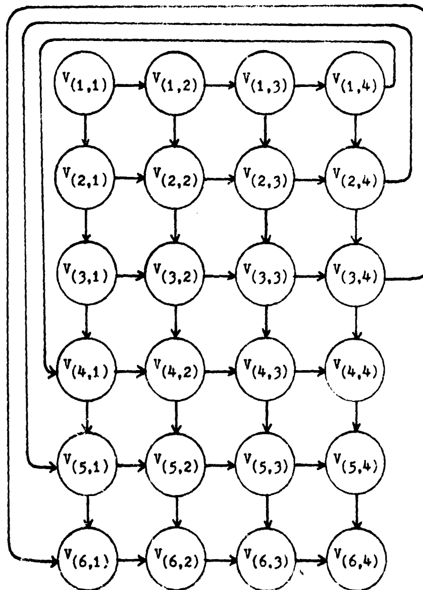
Fig. 11. Partial ordering in V
