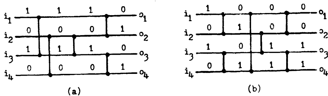
Fig. 3. Testing Comparator Networks.
