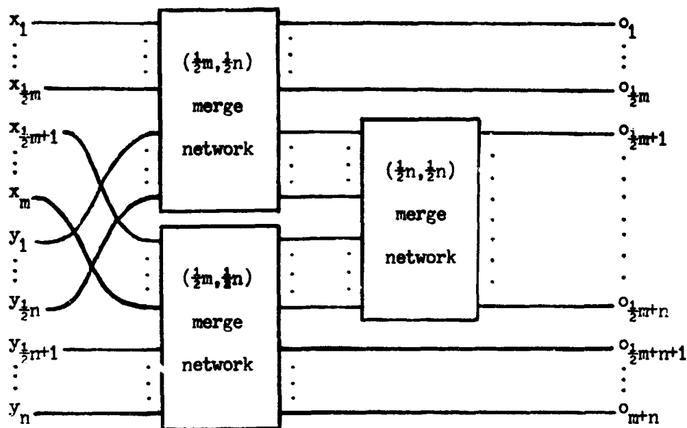
Fig. 5. Bose and Nelson's (m, n) merge network.
