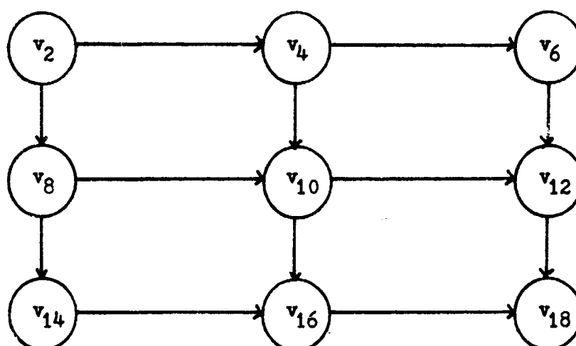
(b) Partial ordering in V_e .
