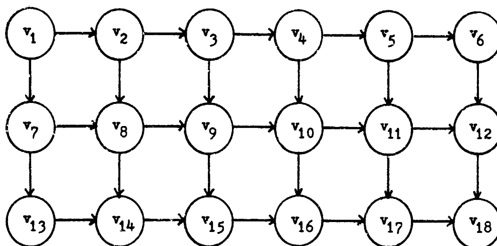
(a) V for [3,6] 18-sorter.
