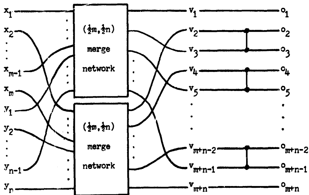
Fig. 6. Batcher's (m, n) merge network.
