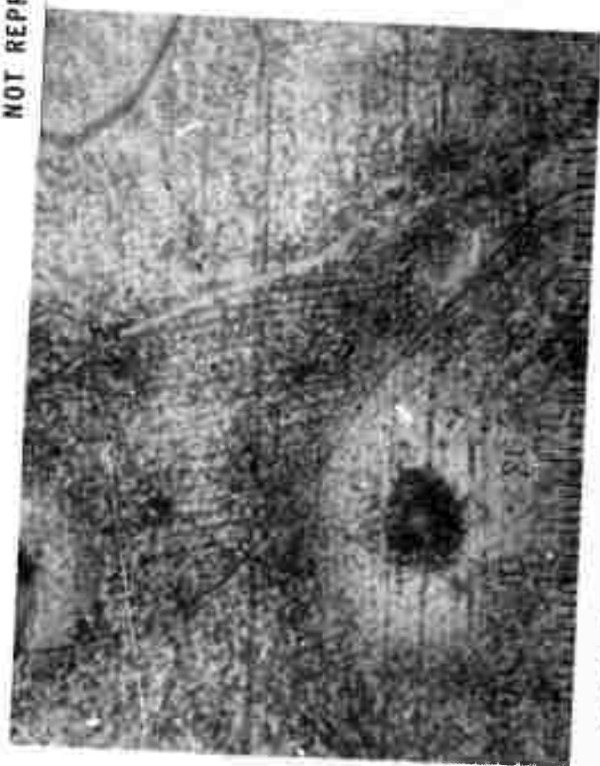
(a) Dislocation Distribution in Fe-3 Si Steel Stressed to 50 ksi, X1200
