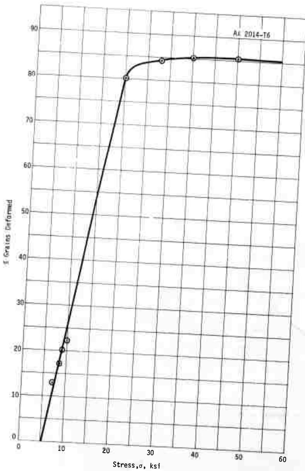
Figure 5 Deformation of Grains as a Function of Stress
