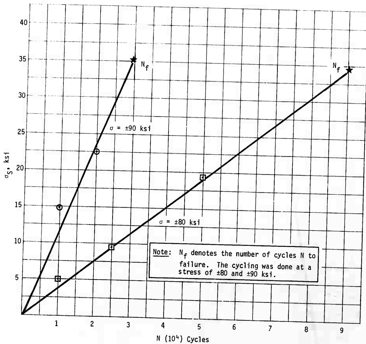
Figure 4 The Increase in Surface Layer Stress \sigma_S with Cycling for Titanium (6Al-4V)
