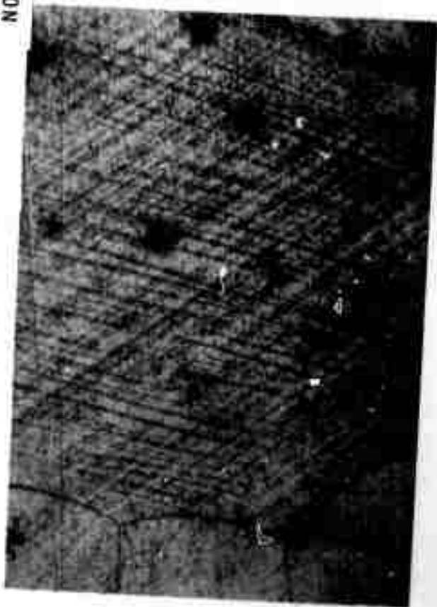
(a) Dislocation Distribution in Fe-3 Si Steel Stressed to 1.5% Strain, at Surface X1200
