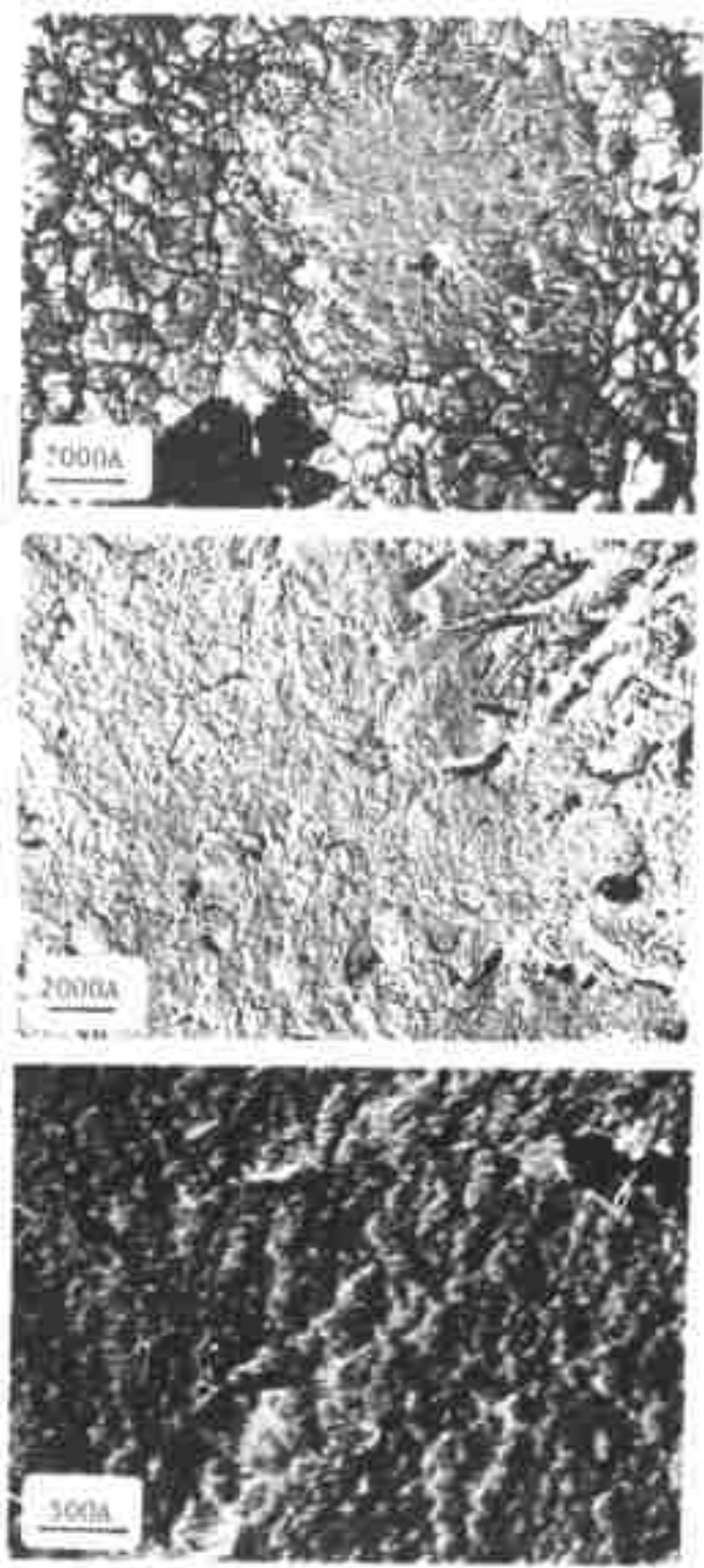
Figure 3. Bright field electron micrograph at various magnifications of two state Pt shadowed replica of a fractured surface in the 311-19, 2000°C sample.
