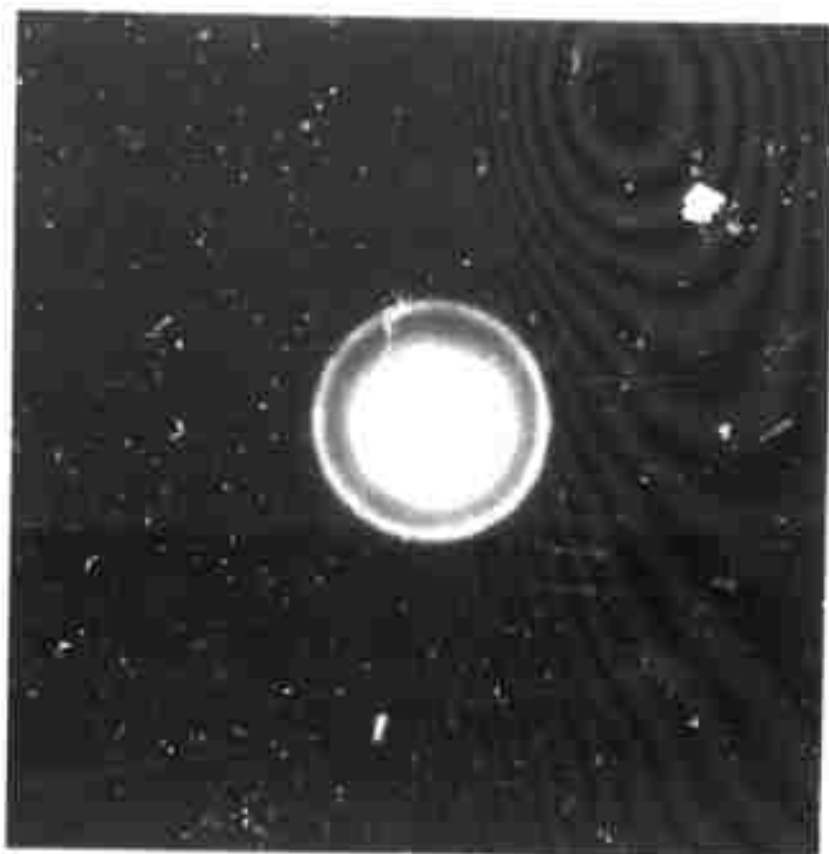
Figure 6. Electron diffraction pattern of sample 311-19, 750°C, showing spots in diffraction rings.
