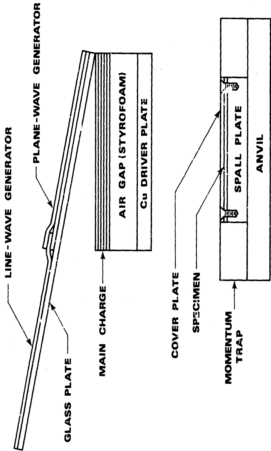
Figure 2. Shock-Loading Assembly
