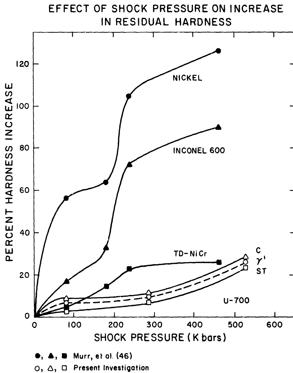
Figure 7. Shock-Hardening Curves for Several Nickel-Base Alloys
