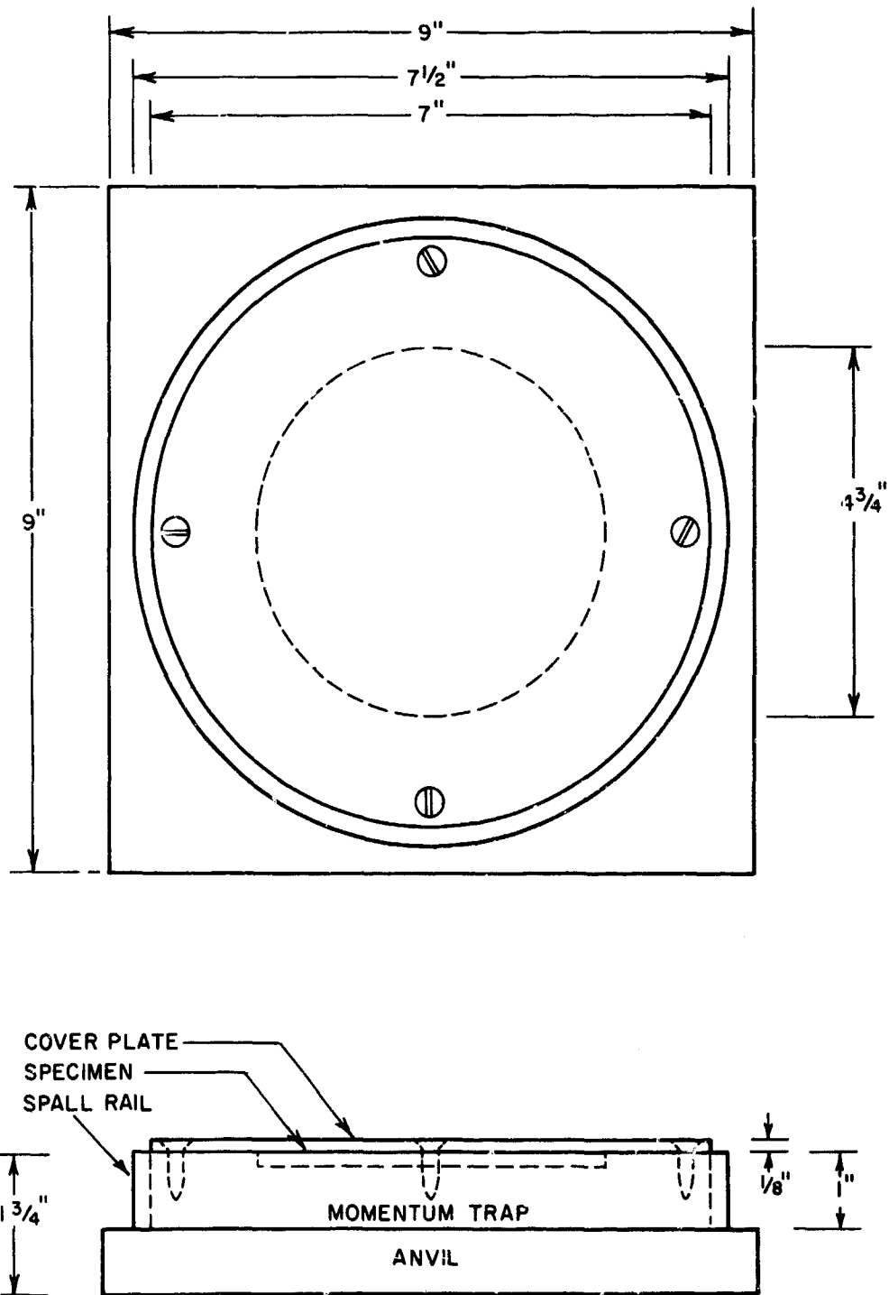
Figure 5. Specimen Assembly: Pancake Geometry
