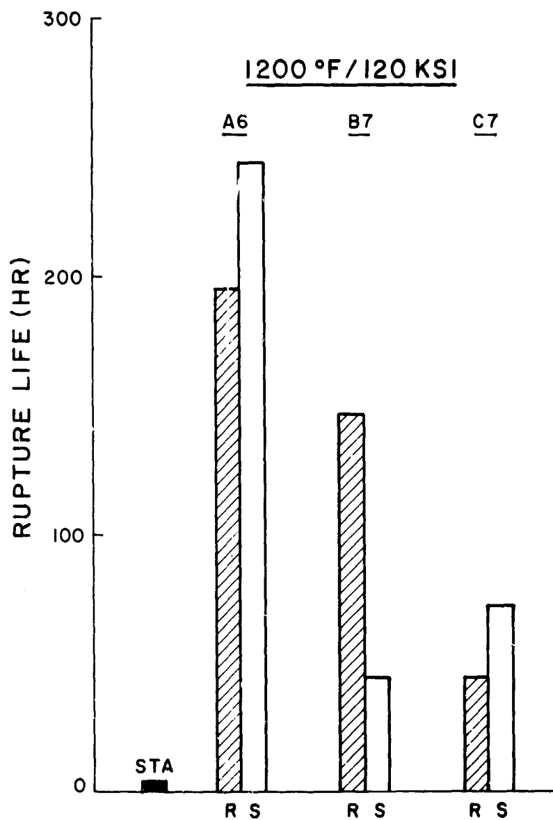
Figure 15. Stress-Rupture Life of Udimet 700 Following Thermal Processing (STA), Conventional TMP by Cold Rolling (R; 19.1% Reduction), and Shock TMP (S; 527 kbar)
