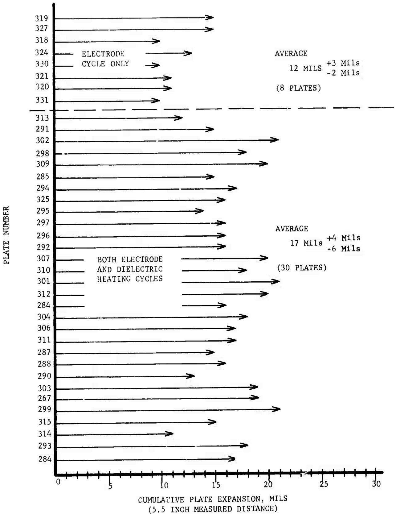
FIGURE 1. 128-60 PLATE STABILITY STUDY
