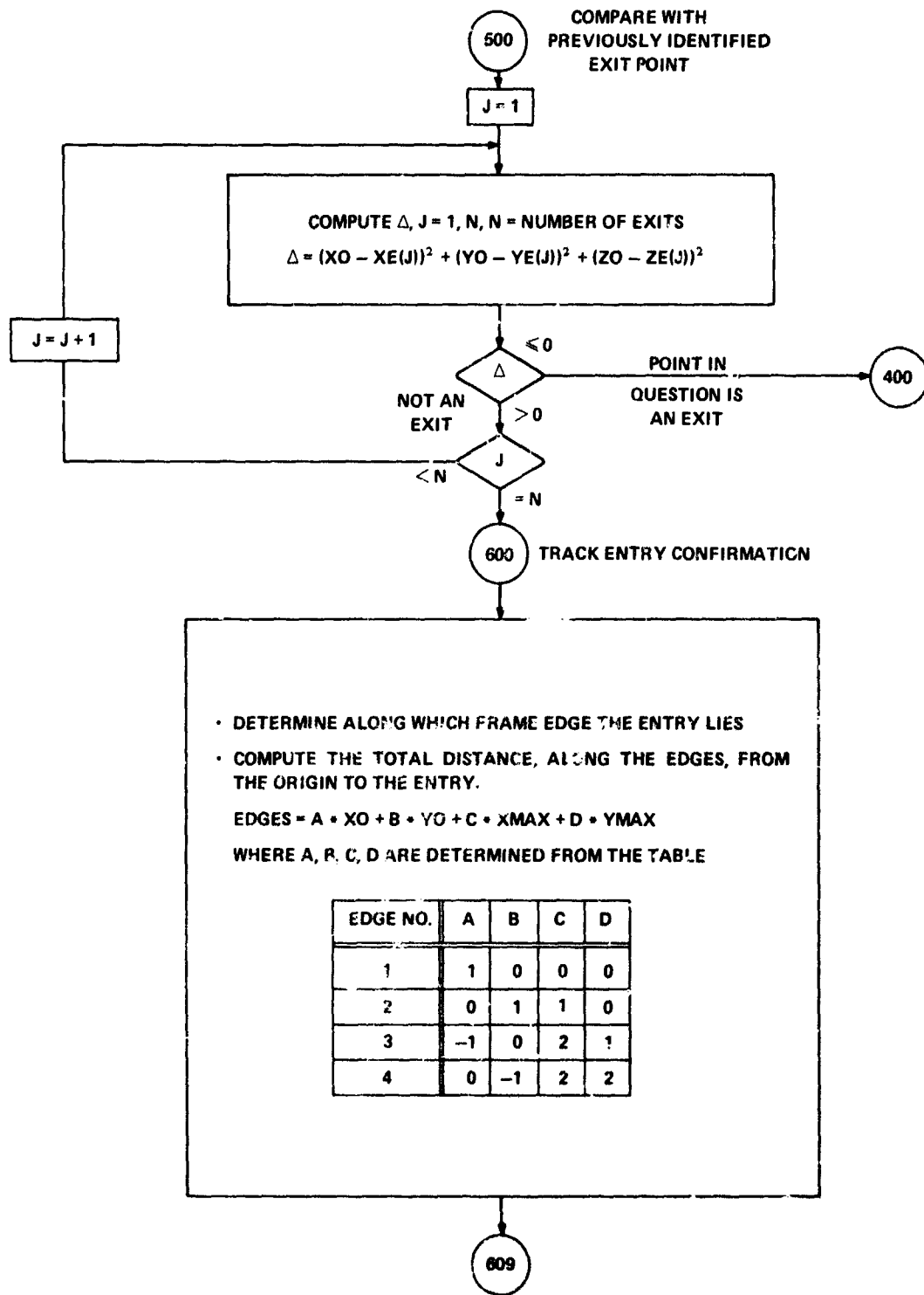
Figure (III-11) Exit Comparison and Confirmation
