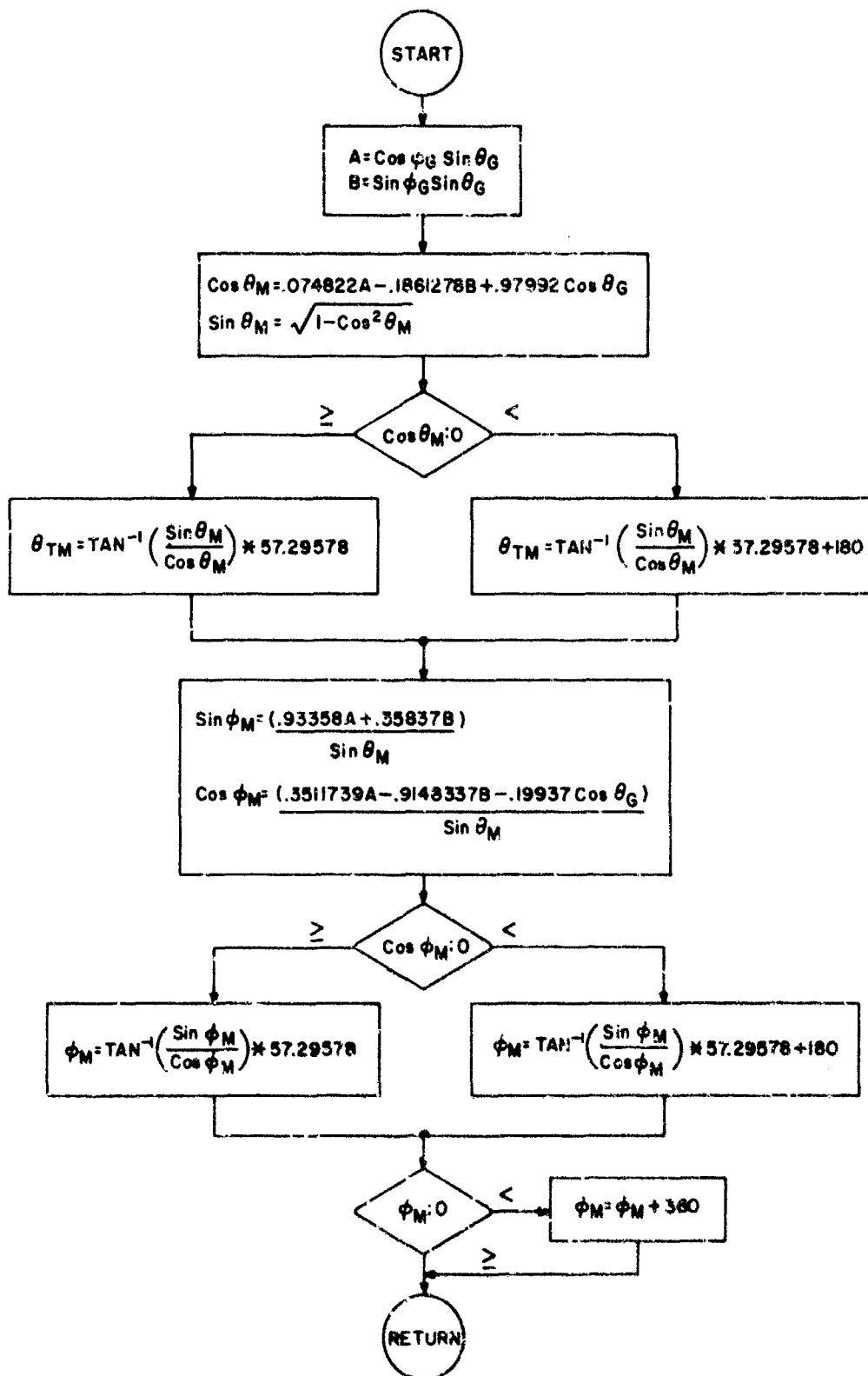
Figure (IIA11.) Subroutine GEOTOM REF: (P3-21, AFCL 69-0123)
