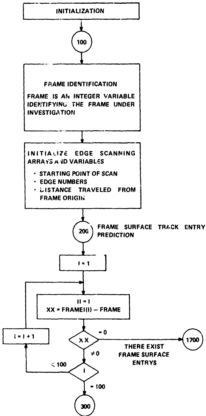
FIGURE (11-9) - INITIALIZATION PROCEDURES
