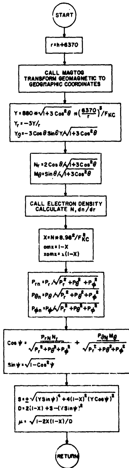
Figure (ILA6.) Subroutine Index of Refraction REF: (PP(3-12) to (3-14) APCR 69-0123)
