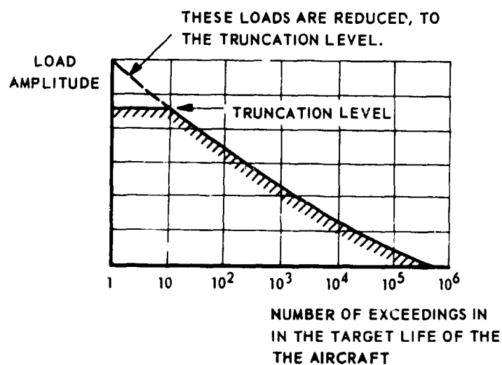
FIG. 7.4 EXAMPLE OF TRUNCATING THE INFREQUENTLY OCCURRING HIGH AMPLITUDES OF A LOAD SPECTRUM.
