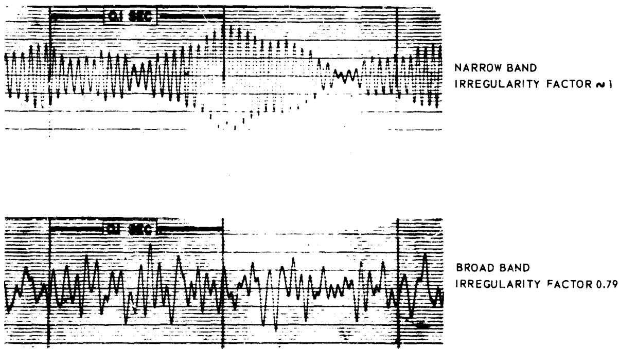
b. STRESS-TIME HISTORY FOR NARROW-BAND AND BROAD-BAND LOADING.
