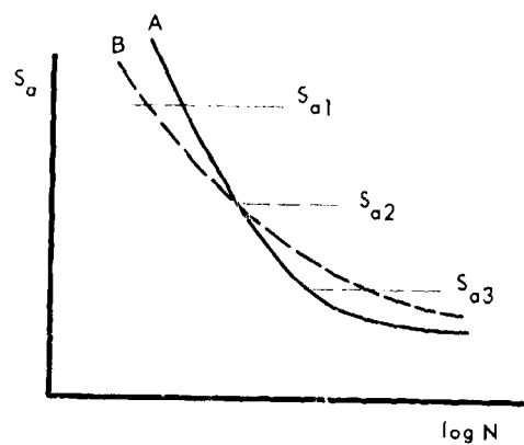
FIG. 7.2 TWO INTERSECTING S-N CURVES
