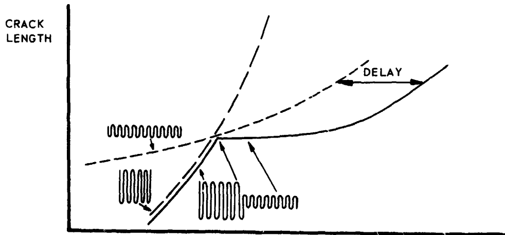
A CRACK GROWTH DELAY IN TWO-STEP TEST.
