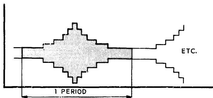
F PROGRAM LOADING WITH LO-HI-LO SEQUENCE. LO-HI AND HI-LO SEQUENCES WERE ALSO ADOPTED, SEE FIGURE 4.17
