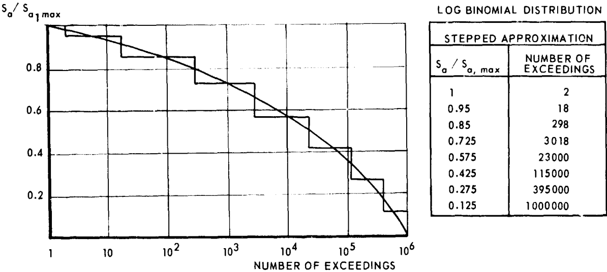
a. STANDARDIZED LOAD SPECTRUM
