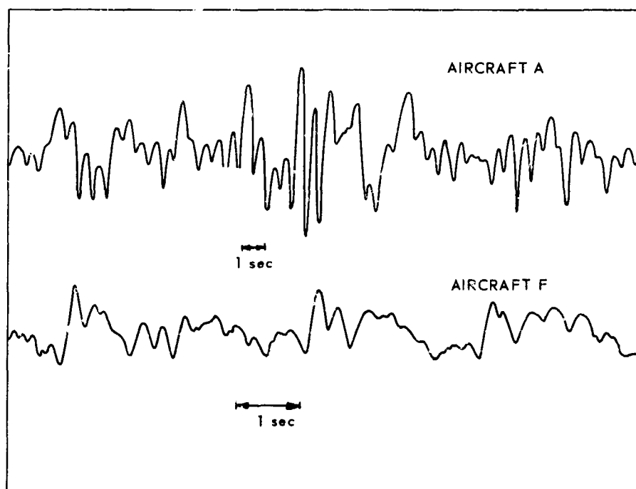
FIG. 6.2 STRAIN GAGE RECORDS OF THE WING BENDING MOMENT OF 2 AIRCRAFT FLYING IN TURBULENT AIR (REF. 174)
