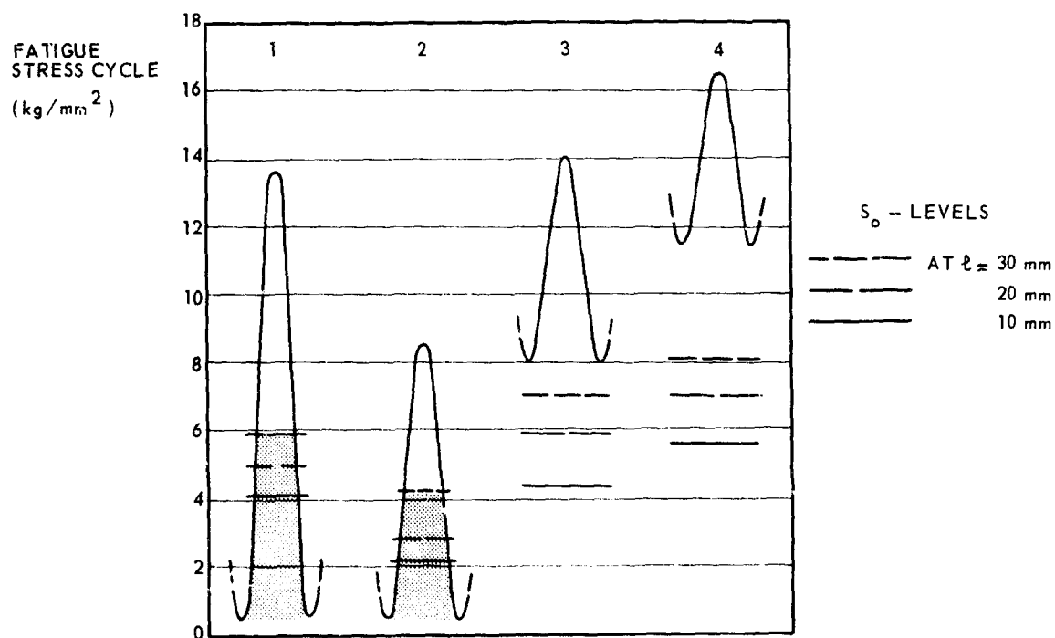
FIG. 3.1 CRACK CLOSURE ACCORDING TO ELBER (REF. 18). RESULTS FROM NLR TESTS (REF. 20).
