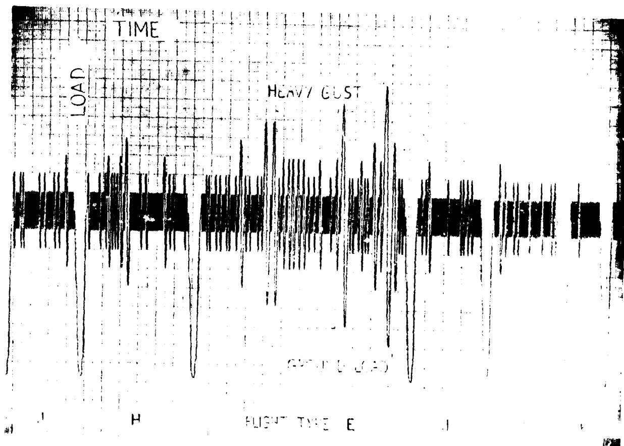
FIG. 7.3 SAMPLE OF A LOAD RECORD, ILLUSTRATING THE LOAD SEQUENCE APPLIED IN THE F-28 WING FATIGUE TEST. TEN DIFFERENT TYPES OF WEATHER CONDITION ARE SIMULATED, FLIGHT TYPE E CORRESPONDS TO FAIRLY SEVERE STORM WHILE FLIGHT TYPE K IS FLOWN IN GOOD WEATHER (REF. 96)
