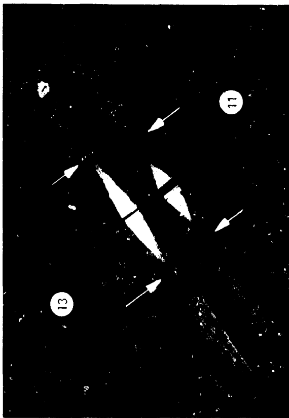
FIG. 3.5 INCOMPATIBILITY BETWEEN CRACK FRONT ORIENTATION AND STRESS AMPLITUDE (REF. 22).
