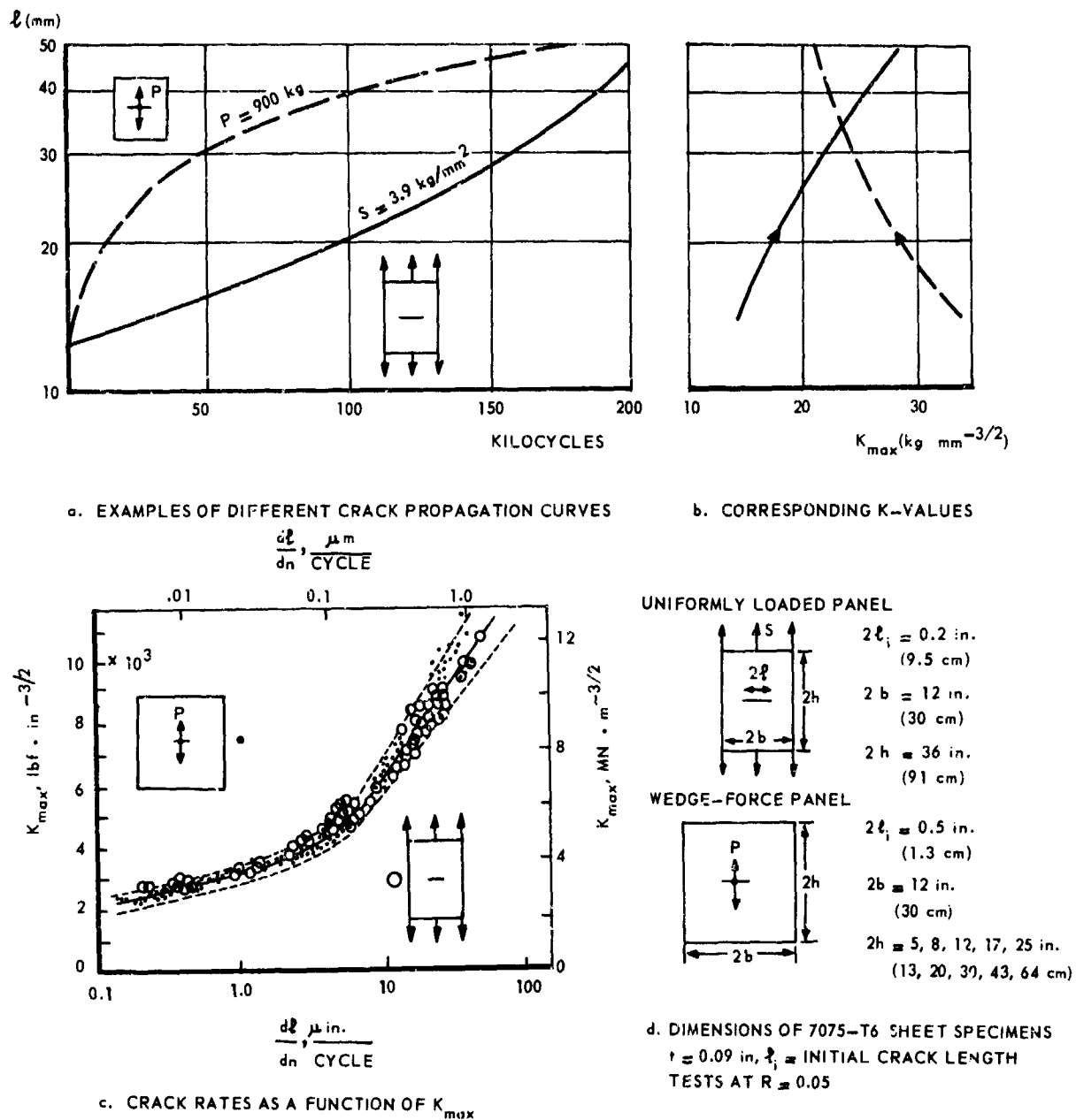
FIG. 5.4 A COMPARISON BETWEEN THE CRACK RATES IN UNIFORMLY LOADED AND WEDGE-FORCE LOADED SPECIMENS RESULTS FROM FIGGE AND NEWMAN (REF. 164).
