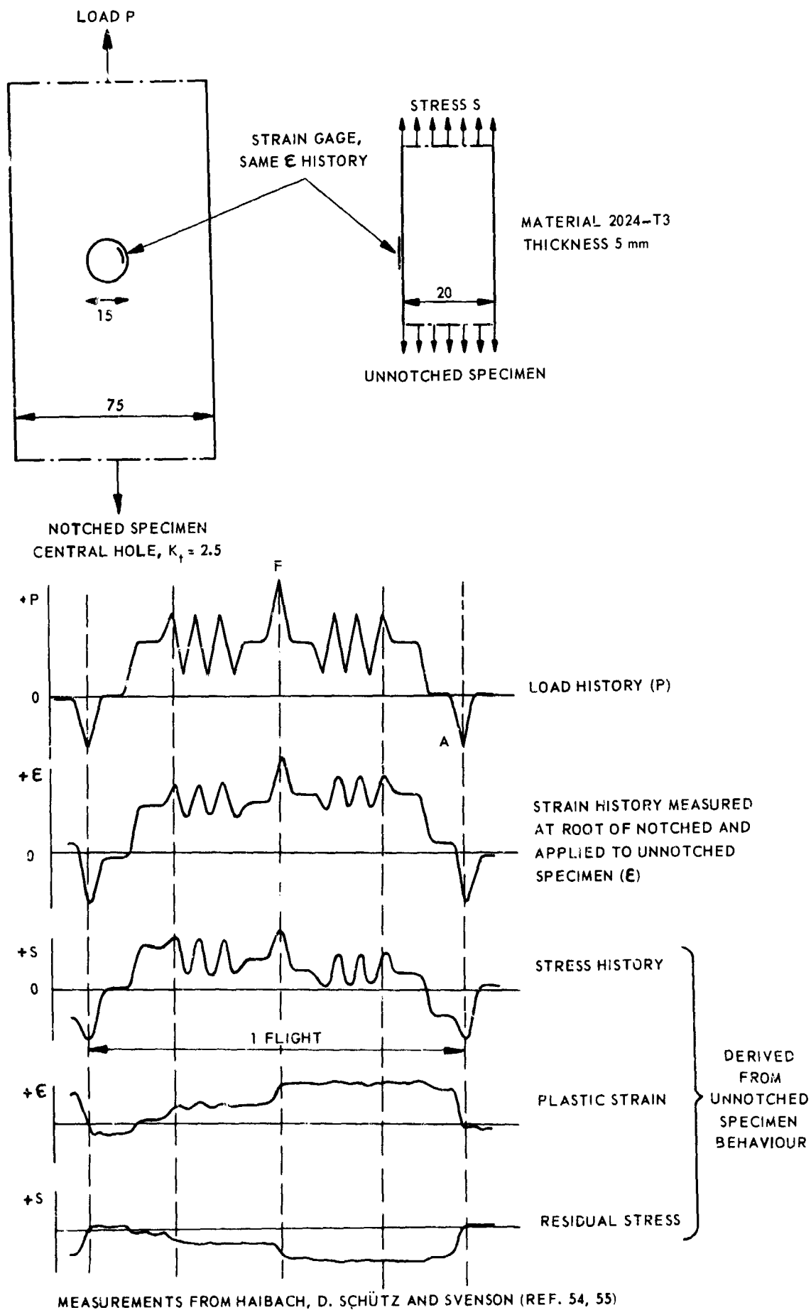
FIG. 4.8 DETERMINATION OF RESIDUAL STRESS AT THE ROOT OF A NOTCH DURING A SIMPLE FLIGHT-SIMULATION LOADING
