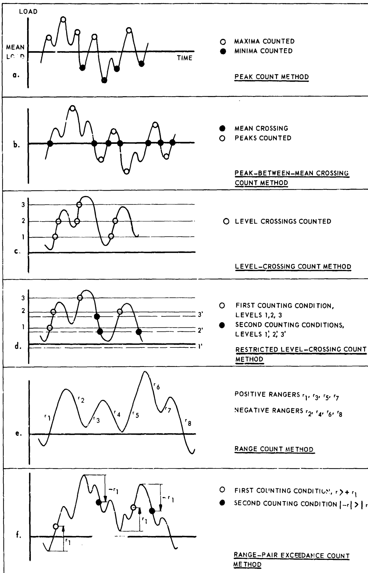
FIG. 6.3 SEVERAL COUNTING METHODS FOR A STATISTICAL DESCRIPTION OF A LOAD-TIME HISTORY. NAMES OF METHODS AFTER VAN DIJK (REF.176)
