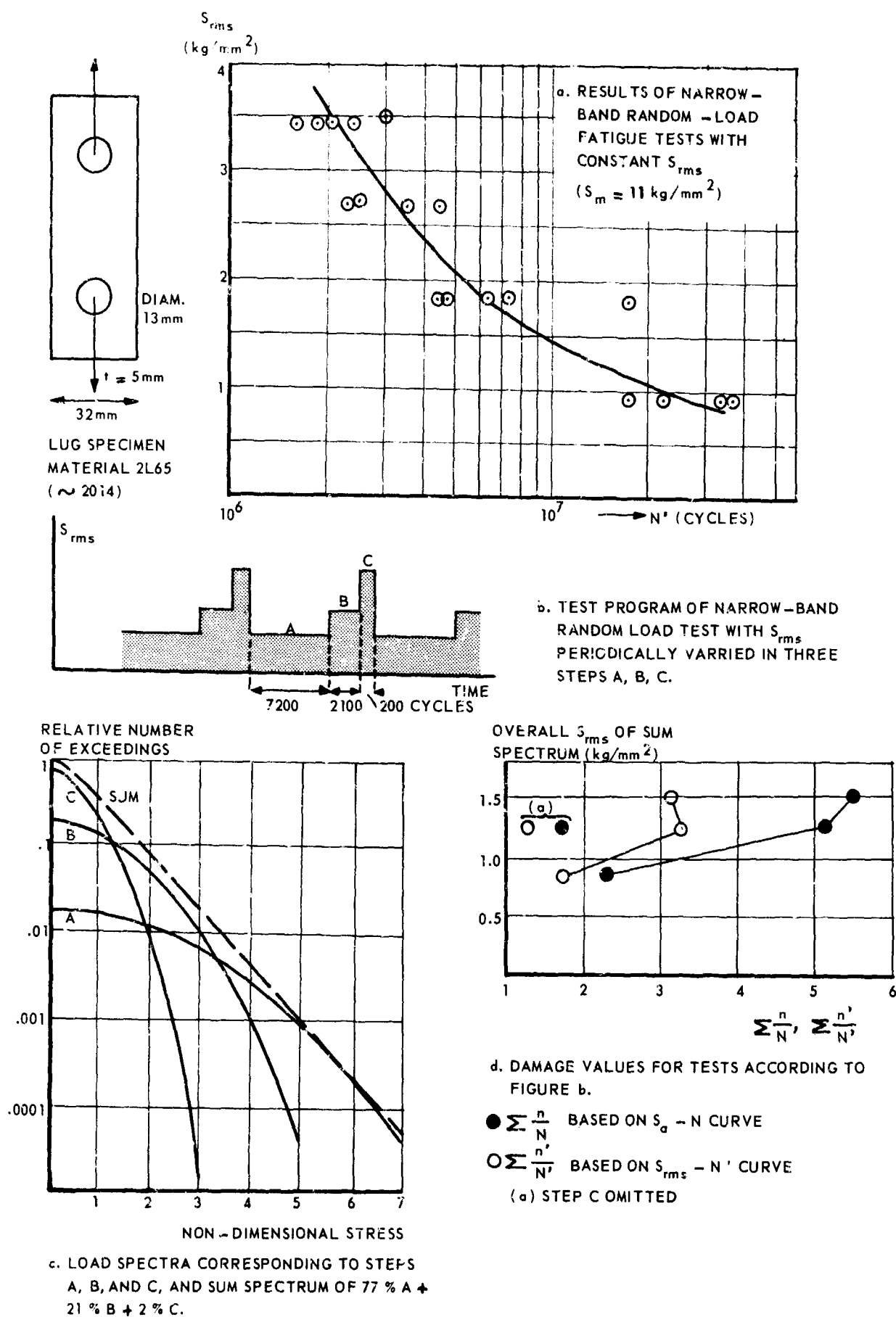
FIG. 5.2 NARROW-BAND RANDOM LOAD TESTS WITH CONSTANT S_{rms} AND PROGRAMMED S_{rms} . RESULTS FROM KIRKBY AND EDWARDS (REF. 99).
