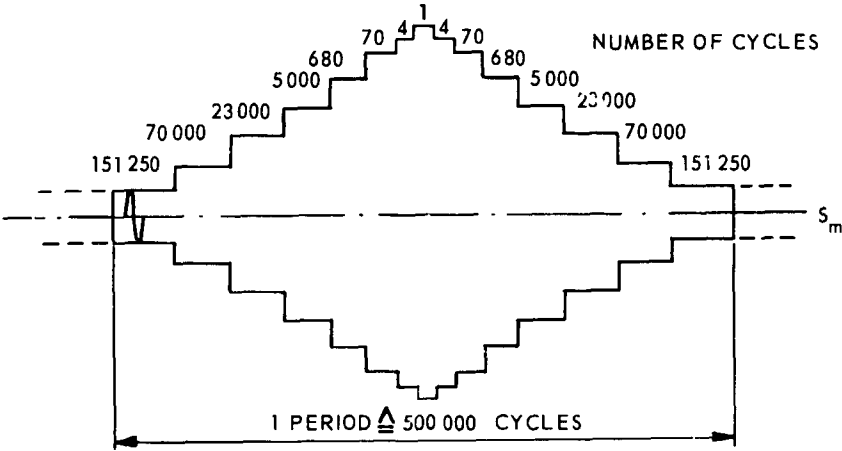
b. LOAD SEQUENCE IN PROGRAM TEST AND NUMBERS OF CYCLES IN ONE PERIOD
