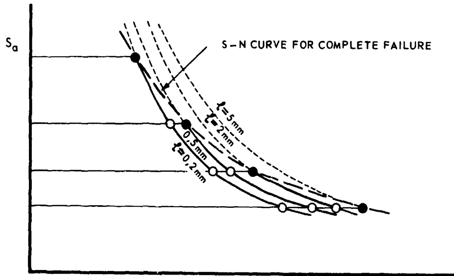
FIG. 3.6 S-N CURVES FOR CONSTANT AMOUNTS OF CRACKING ( l IN MILLIMETERS) AND S-N CURVE FOR COMPLETE FAILURE.
