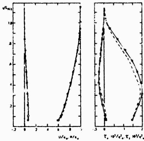
FIG. 6 INITIAL PROFILES FOR THE CALCULATION OF EXPERIMENT BY BRADSHAW AND TERRELL (REF. 5). —, x = 77, z = 2, \delta_{995} = .95 (in.); ---, x = 83, z = 0, \delta_{995} = .95 (in.); o, EXPERIMENTAL RESULTS AT x = 77, z = 2 .
