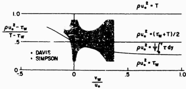
Figure 10. Test of best assumption for characteristic stress \rho u_o^2 . Data points show values of \rho u_o^2 which reproduce C_f obtained by mixing-length method (i.e., C_f(MIX) in figure 1).
