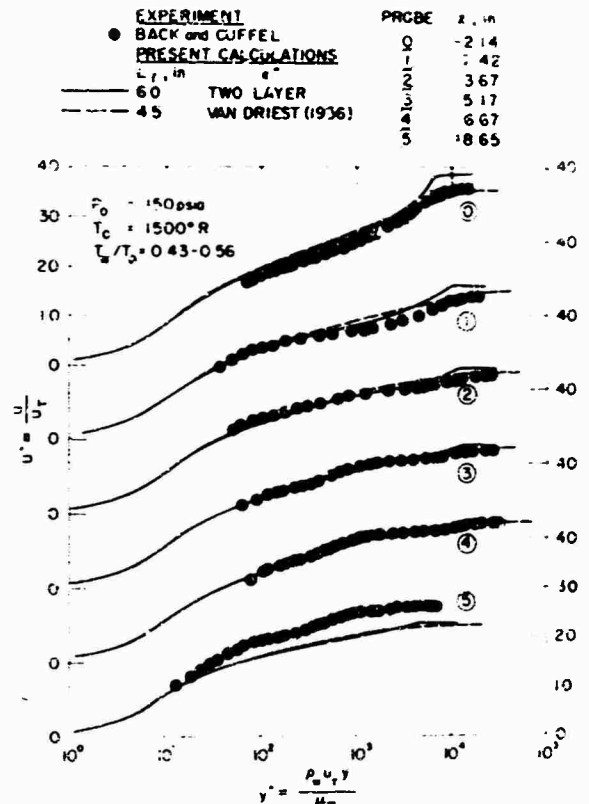
Fig. 12 - Velocity Profiles in Law-of-the-Wall Coordinates for the Back and Cuffel Cooled Wall Nozzle Flow
