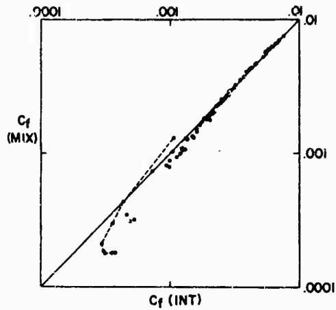
Figure 16. Data of Simpson (1967). Abscissa, C_f (INT), is obtained by fit of each profile to equations (4'), (50) and (44), with integral definition for \rho u_0^2 . Ordinate, C_f (MIX), is same as in figure 1. Dashed line is trace of data for flow 121266 ( v_w/u_\infty = 0.0094 ).
