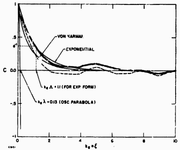
Fig. 9 Expanded plot of the autocovariance coefficients of Fig. 8 showing a comparison of the data with two analytic forms.
