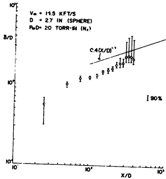
Fig 19. Mean position of turbulence interface or the intermittency radius
