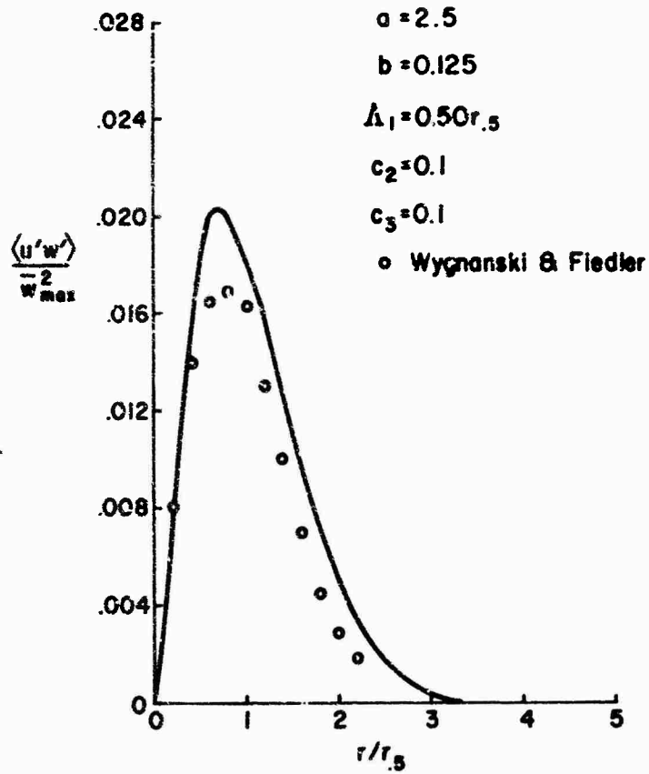
Figure 12. Comparison of experimental results and model predictions for the shear correlation in a free jet
