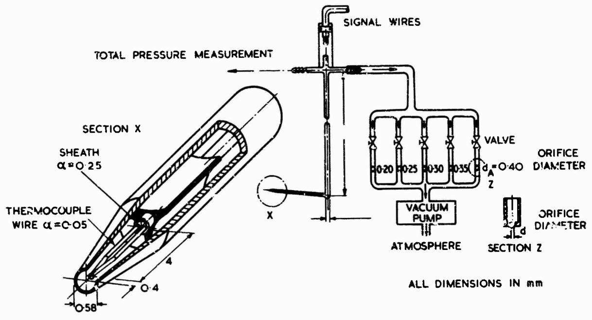
Fig.1 Combined total-temperature and pitot-pressure probe
