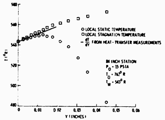
FIGURE 6 TYPICAL FINE-WIRE TEMPERATURE PROFILE NEAR WALL
