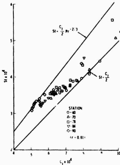
FIGURE 18 REYNOLDS ANALOGY CORRELATION
