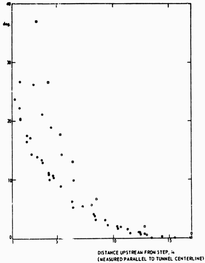
FIG. 13 ANGLE BETWEEN WALL STREAMLINE AND TUNNEL CENTERLINE, JOHNSTON'S EXPERIMENT (REF. 14). \bullet , PRESENT CALCULATION AT .074 in. FROM THE WALL; \circ , EXPERIMENT; \circ , CALCULATION, REF. 6.
