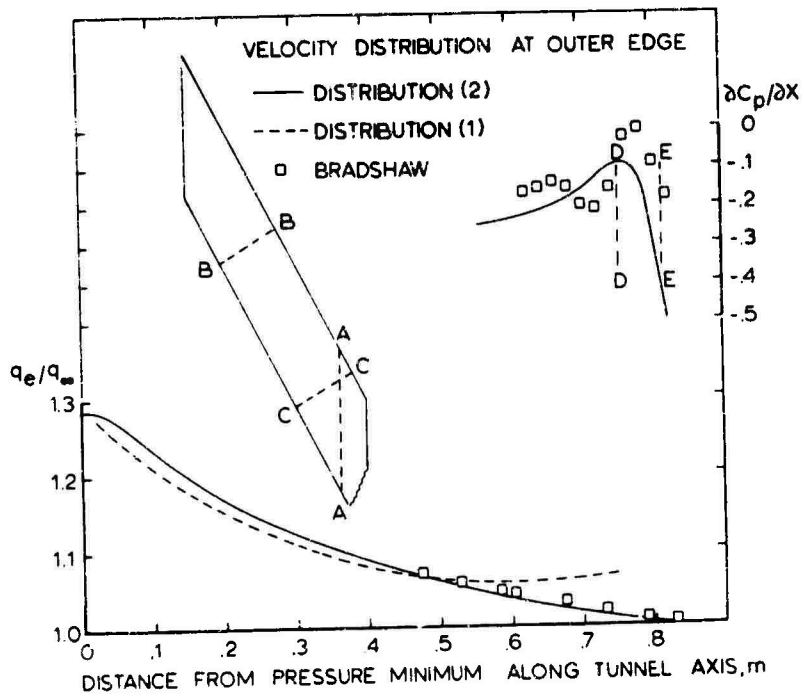
FIG. 16 THE TWO INVISCID VELOCITY DISTRIBUTIONS ALONG AA USED IN THE CALCULATIONS OF THE CUMSTY AND HEAD FLDW. AA, LINE ALDNG WHICH BOUNDARY LAYER MEASUREMENTS WERE MADE. BB AND CC, LINES ALDNG WHICH THE PRESSURE WAS MEASURED. DD AND EE, BRADSHAW'S AND PRESENT SEPARATION PREDICTION, RESPECTIVELY
