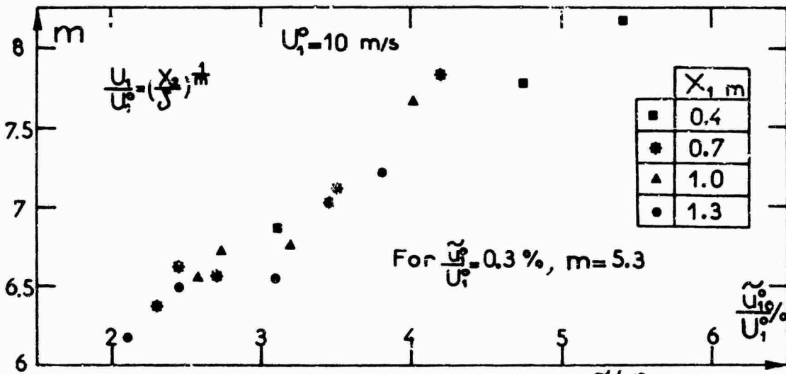
Fig. 7 Power law coefficient m versus \tilde{U}/U_1 .
