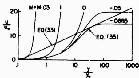
Figure 7. Intersections of the logarithmic curve, equation (33), with the laminar sublayer curve, equation (35).
