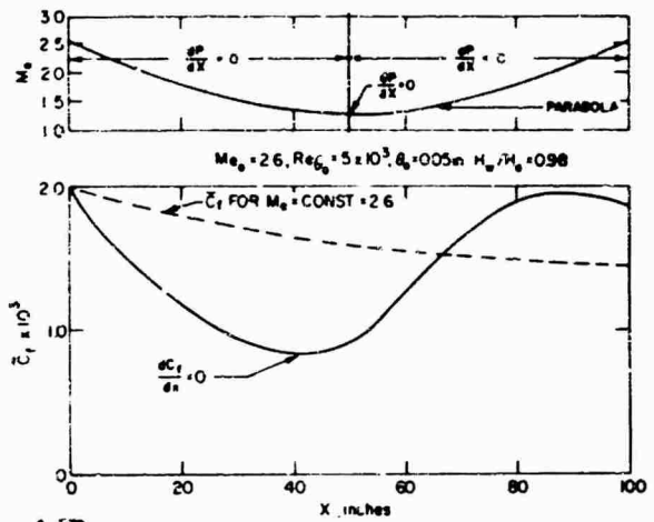
Figure 8a EFFECT OF dP/dx ON \bar{C}_f
