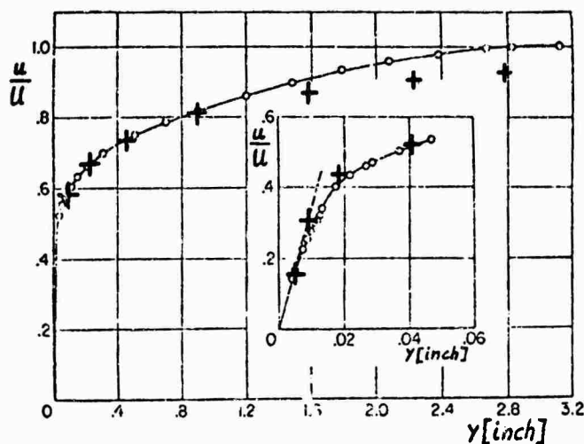
Fig. 5. Comparison of computed velocity profile (+) with measurements of KLEBANOFF [2], Re_{1cm} = 9.7 \cdot 10^3 .
