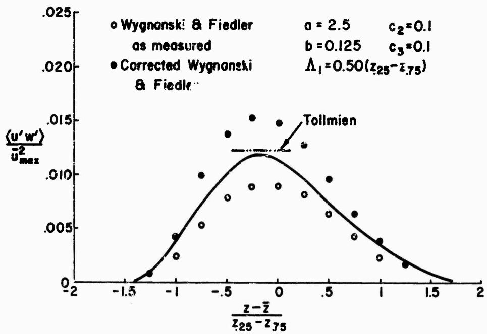
Figure 13. Comparison of experimental results and model computations for the shear correlation in a free shear layer
