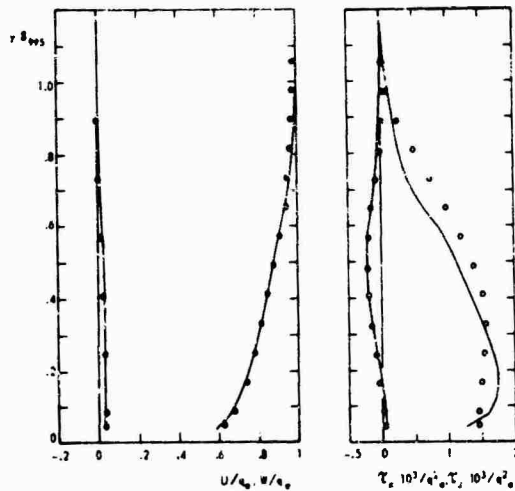
FIG. 8 MEASURED AND COMPUTED PROFILES, EXPERIMENT BY BRADSHAW AND TERRELL (REF. 5). x - z = 89 (in.), \delta_{995} = 1.23 (in.) o, EXPERIMENT; —, CALCULATION.
