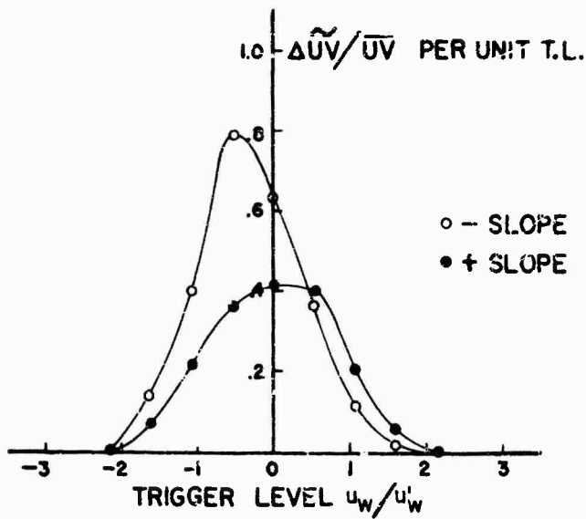
Fig. 8 Conditionally sampled contributions to uv as a function of T.L. A low pass filter was used for u_w frequency band 0.26 < f < 80 Hz. Signal uv sampled when u_w = T.L. u'_w , x^+ = 0, y^+ = 30 , U_\infty = 19.7 ft per sec.
