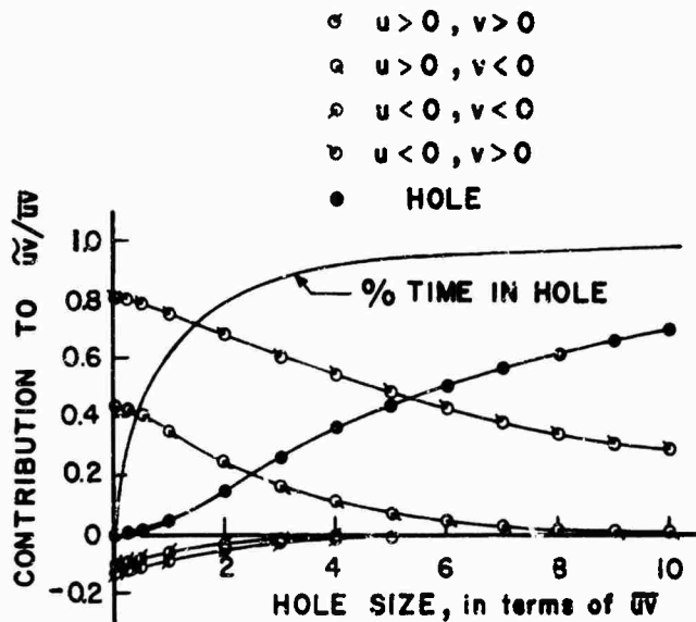
Fig.16 Contributions to Reynolds stress from truncated quadrants of u, v plane and percentage time spent in hole as a function of hole size. uv measured at y^+ = 30 in low speed boundary layer, U_\infty = 19.7 ft/sec.
