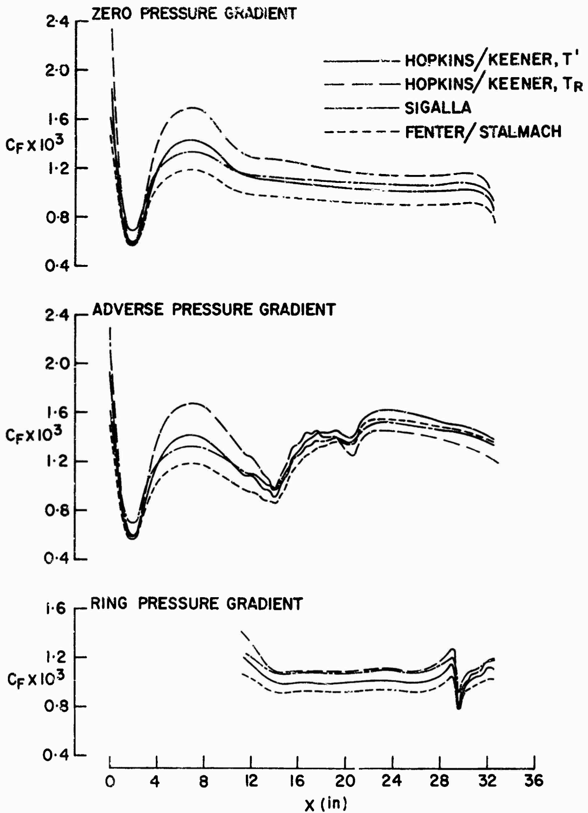
Fig. 9a Distributions of skin friction coefficient along the duct
