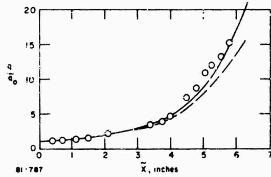
Figure 15 COMPARISON WITH DATA ON AN AXISYMMETRIC COMPRESSION SURFACE
