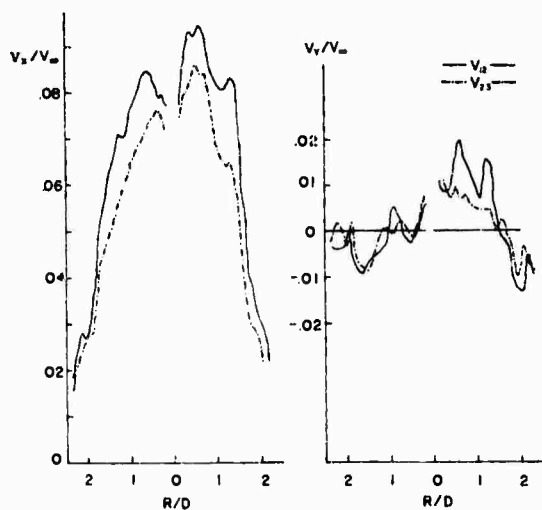
Fig 4. Typical velocity profile from sparks
