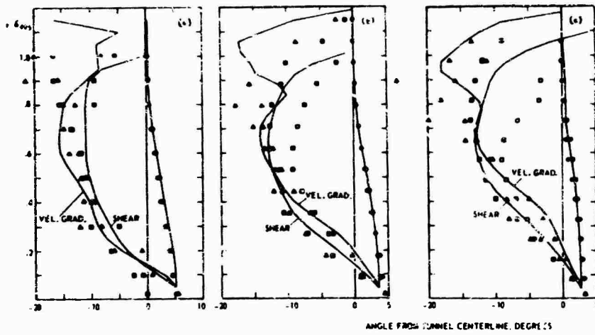
FIG. 7 CALCULATION OF VELOCITY, SHEAR STRESS AND VELOCITY GRADIENT ANGLES IN EXPERIMENT BY BRADSHAW AND TERRELL (REF. 5). —, CALCULATION. EXPERIMENTAL RESULTS: o, VELOCITY; square, SHEAR STRESS; triangle, VELOCITY GRADIENT. CALCULATION, REF. 6: o, VELOCITY; square, SHEAR STRESS; triangle, VELOCITY GRADIENT. (a), x - z = 77, \delta_{995} = 1.00 (in.); (b), x - z = 83, \delta_{995} = 1.14 (in.); (c), x - z = 89, \delta_{995} = 1.23 (in.)
