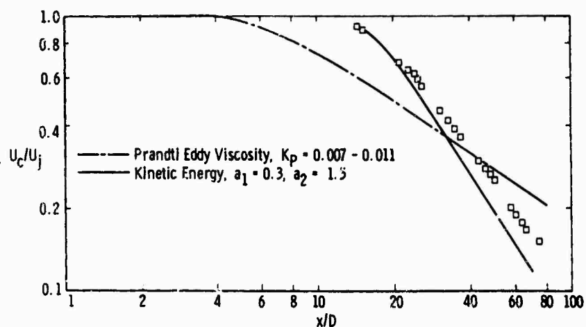
Fig. 3 Comparison of Best Predictions with Data for the Compressible Jet-into-Still-Air. Data from Eggers 6 , M_j = 2.22
