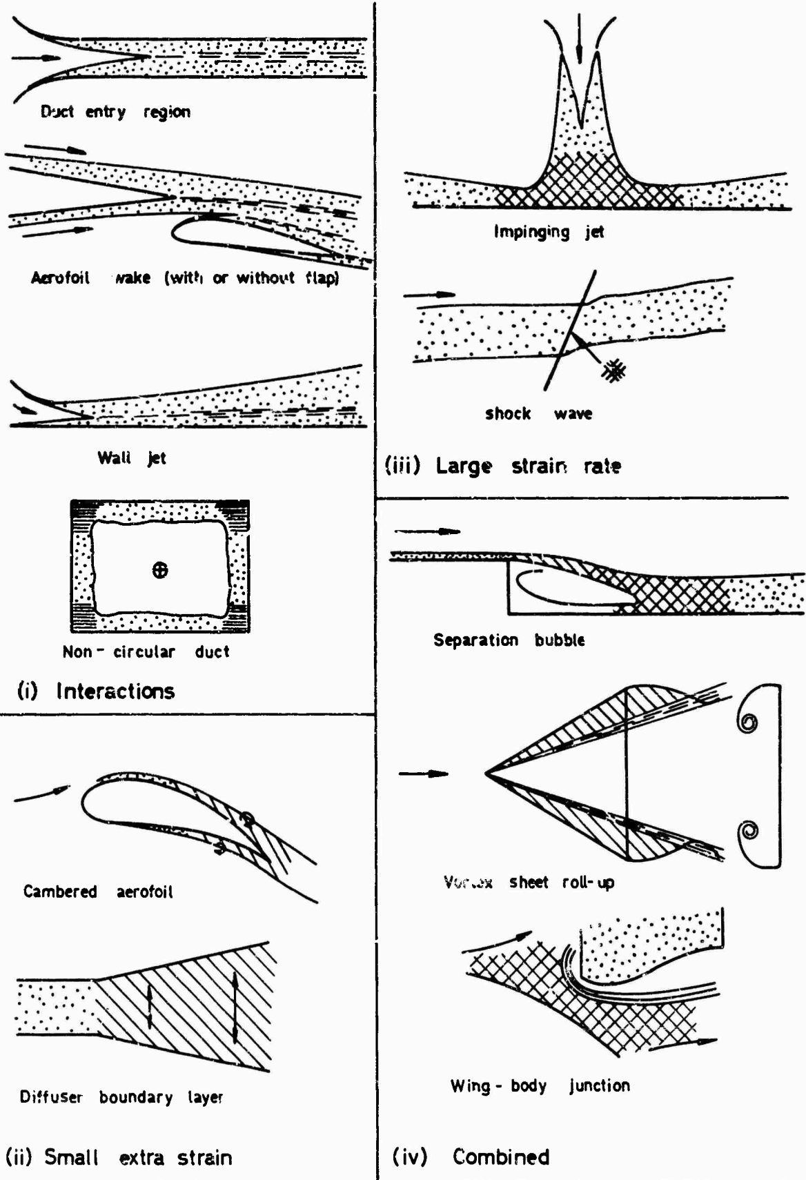
FIG. 1 EXAMPLES OF COMPLEX TURBULENT FLOWS.
