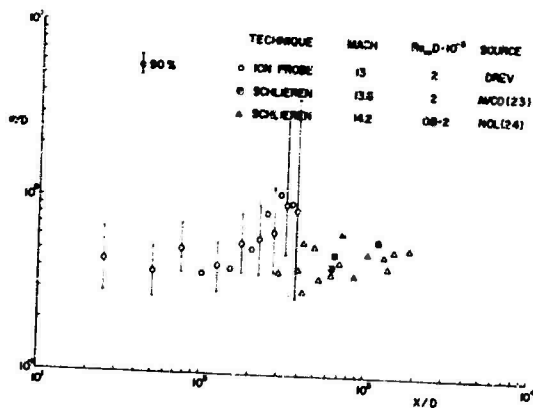
Fig 20. Standard deviation of the position of the turbulence interface
