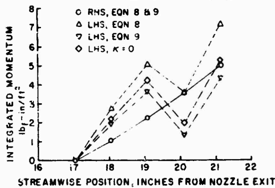
Figure 11. The Distribution of \partial(\rho u)/\partial x
