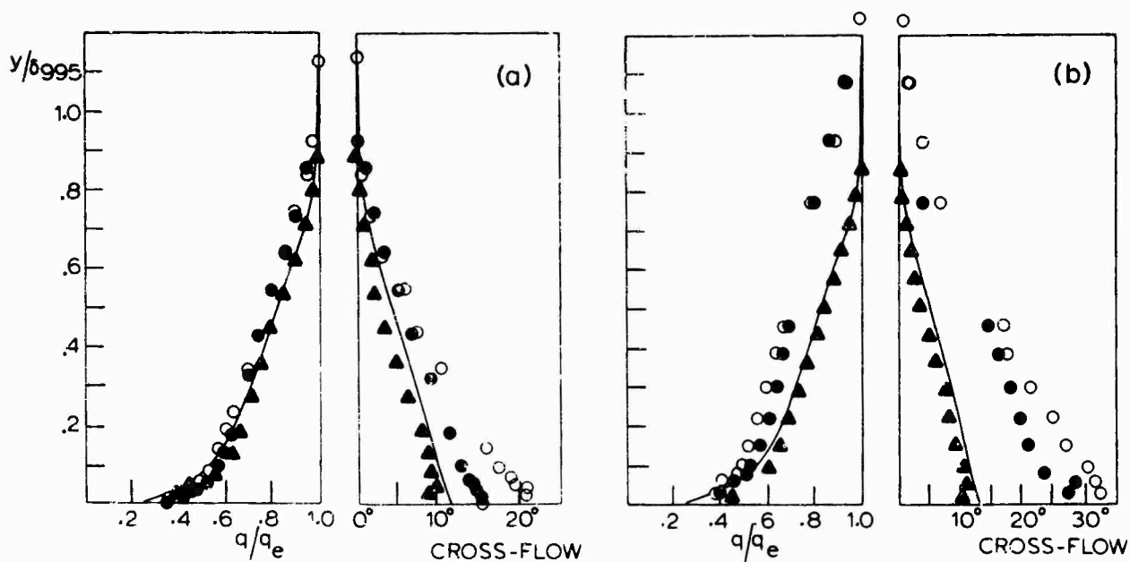
FIG. 19 CUMPSTY AND HEAD EXPERIMENT, MAGNITUDE AND DIRECTION OF VELOCITY VECTOR. —, PRESENT CALCULATION WITH PRESSURE DISTRIBUTION (1); O, EXPERIMENT; A, CALCULATION BY NASH (REF. 2); ●, CALCULATION BY NASH WITH ADDITIONAL SPANWISE PRESSURE GRADIENT. (a), d_{995} = 15.4 mm., CHORDWISE DISTANCE FROM PRESSURE MINIMUM 195 mm (b), d_{995} = 19.0 mm., CHORDWISE DISTANCE FROM PRESSURE MINIMUM 249 mm.
