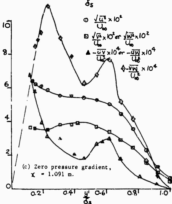
Fig. 5. Reynolds Stresses Along Centre Plane.
