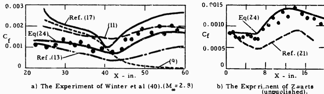
Figure 5. THEORY AND EXPERIMENT FOR RELAXING SUPERSONIC BOUNDARY LAYERS.
