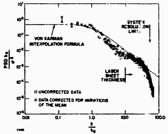
Fig. 7 Ensemble averaged estimate of the energy spectrum. The adjusted points have been corrected for deterministic components.
