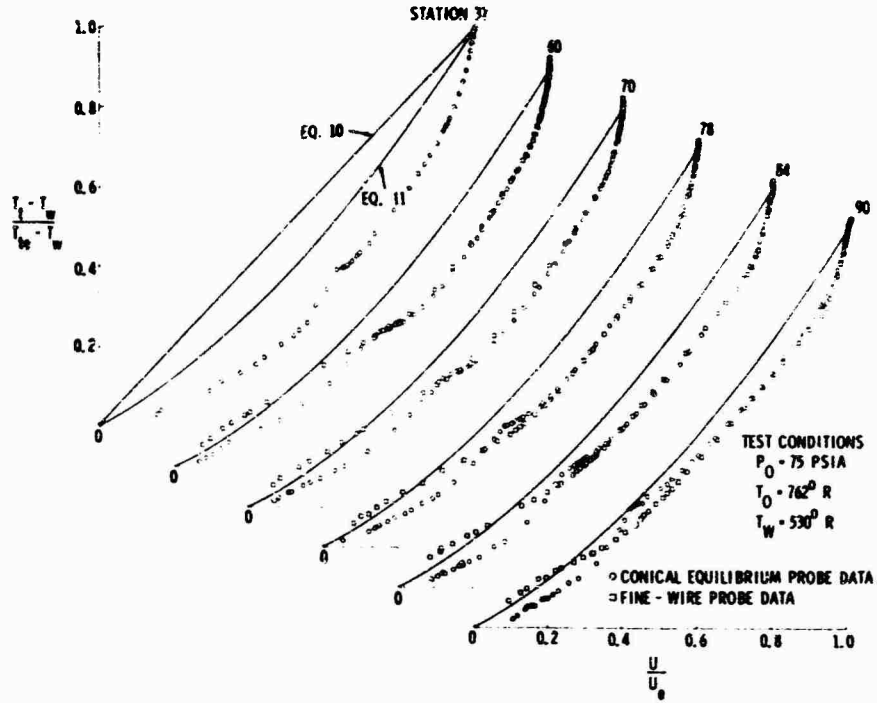
FIGURE 15 MODERATE-HEAT-TRANSFER TEMPERATURE-VELOCITY CORRELATION
