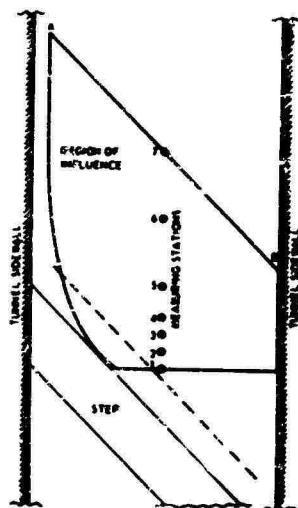
FIG. 10 REGION OF INFLUENCE OF SURFACE AB. ALSO COMPUTATIONAL REGION: JOHNSTON'S EXPERIMENT (REF. 14). ---, EXPERIMENTAL SEPARATION LINE.
