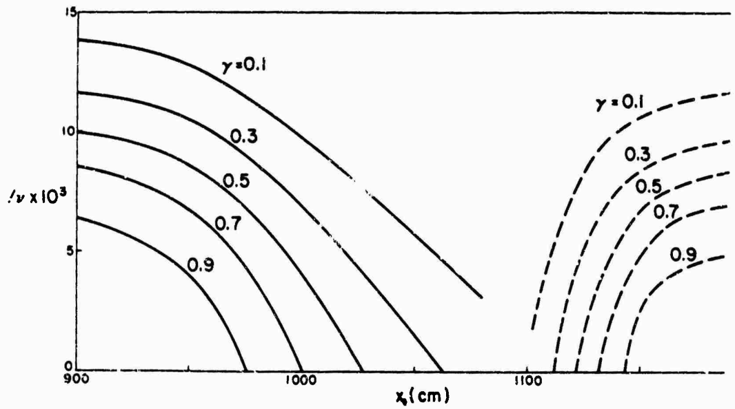
Figure 10. Variation of the intermittency factor in the accelerated boundary layer.
