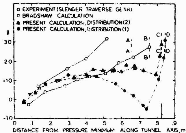
FIG. 18 CUMPSTY AND HEAD EXPERIMENT, SURFACE CROSS-FLOW ANGLE WITH RESPECT TO LOCAL FREE STREAM DIRECTION. EXTENDED LAW OF THE WALL USED IN THE CALCULATIONS. AA, BB, CC, DD, SEPARATION POSITIONS, EXPERIMENTAL, BRADSHAW CALCULATION AND PRESENT CALCULATIONS, RESPECTIVELY.
