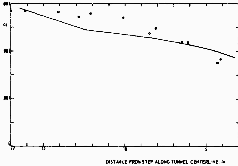
FIG. 12 JOHNSTON'S EXPERIMENT (REF. 14), c_f —, CALCULATION, \bullet , EXPERIMENT; \circ , CALCULATION, REF. 6.
