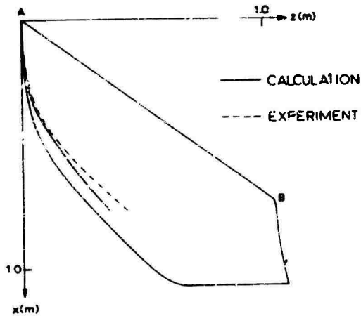
FIG. 15 REGION OF INFLUENCE, ALSO COMPUTATIONAL REGION, USING SIMPLE LAW OF THE WALL, NLR - EXPERIMENT. - - - - , EXPERIMENTAL WALL STREAMLINE. ———— , COMPUTED WALL STREAMLINE USING EXTENDED LAW OF THE WALL
