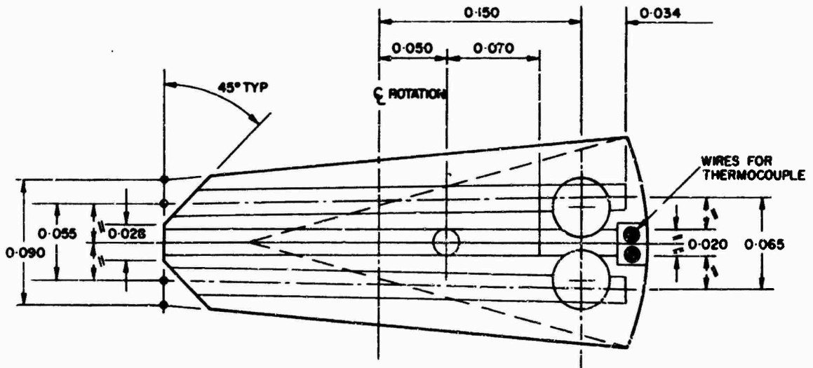
SECTION IN PLAN VIEW
