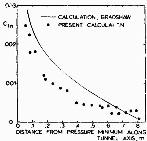
FIG. 17 CUMPSTY AND HEAD EXPERIMENT. COMPARISON OF CHORDWISE COMPONENT OF SKINFRICTION COEFFICIENT IN CALCULATION OF REF. 6 AND PRESENT CALCULATION, USING EXTENDED LAW OF THE WALL AND PRESSURE DISTRIBUTION (2).
