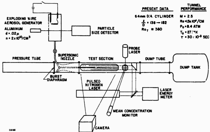
Fig. 2 Schematic of the experimental arrangement.
