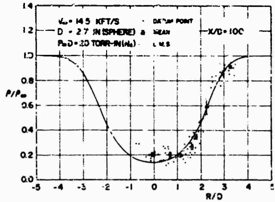
Fig 13. Radial profile of density in the wake
