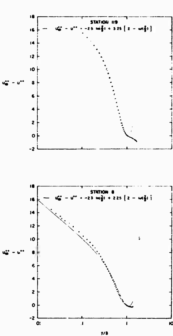
Figure 16. Velocity Defect Data Correlation
