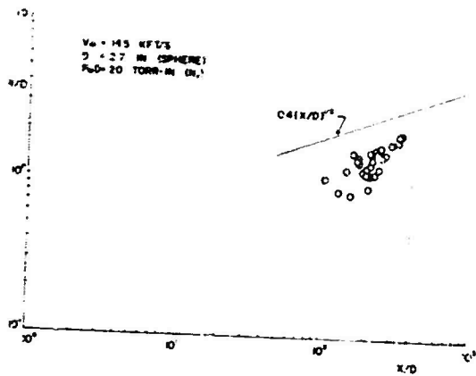
Fig 18. Position of wake transition
