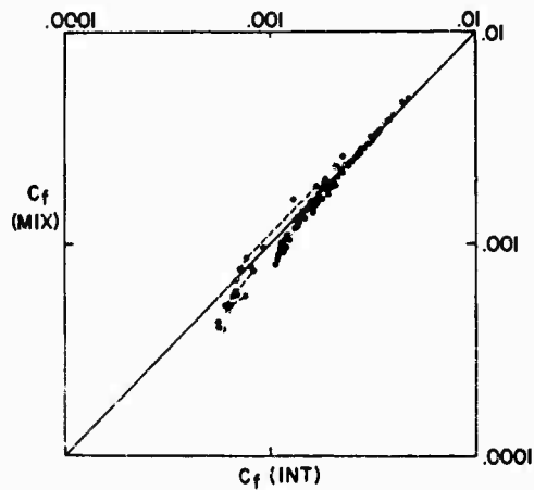
Figure 18. Data of Mickley and Davis (1957). Notation as in figure 16. Dashed line is trace of data for flow C-10-20 ( v_w/u_\infty = 0.0095 ).
