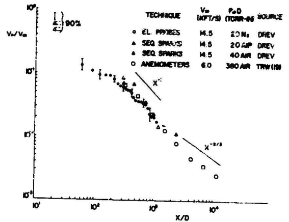
Fig 9. Axis velocity in sphere wakes
