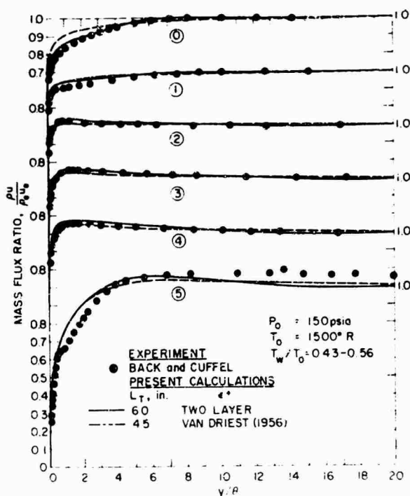
Fig. 16 - Mass Flux Ratio Profiles for the Back and Cuffel Cooled Wall Nozzle Flow
