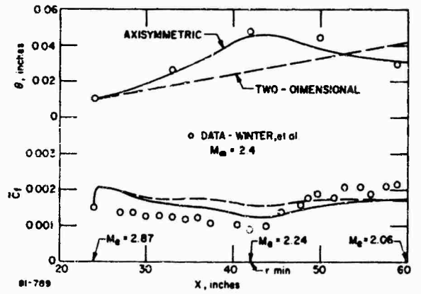
Figure 17 WAISTED BODY OF REVOLUTION
