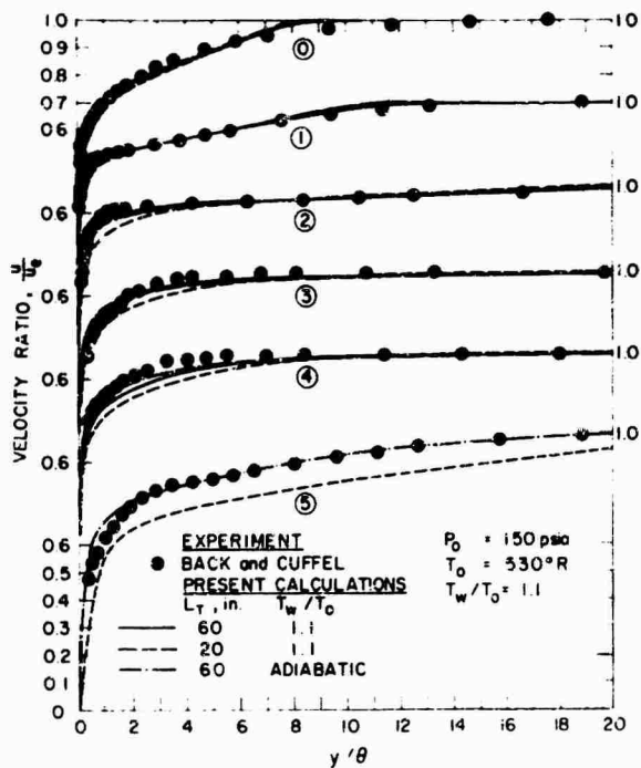
Fig. 18 - Velocity Profiles for the Back and Cuffel Heated Wall Nozzle Flow
