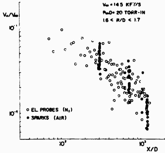
Fig 12. Comparison of velocities measured in sphere wakes with the probe array and the spark techniques at radial distances from 1.6 to 1.7 diameters
