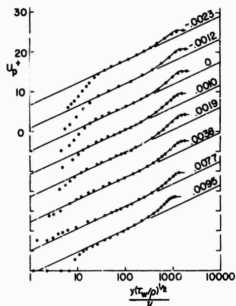
Figure 2. Data of Simpson (1967). Typical profiles fitted to equations (11) and (16). Ordinate, U_p^+ , is pseudo-velocity given by left side of equation (11). Numbers are values of v_w/u_\infty for each profile.
