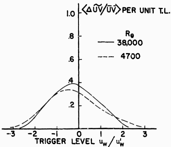
Fig. 10 Average of sampled contributions to uv for + and - slope as a function of T.L. at low and high Reynolds number. No filter was used for u_w . Hot wire locations were: high Re: u_w, y^+ = 7.5 u_v, x^+ = 1690, y^+ = 263 low Re: u_w, y^+ = 8.3 u_v, x^+ = 762, y^+ = 116
