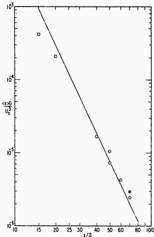
Figure 2. Dissipation Rate Correlation
