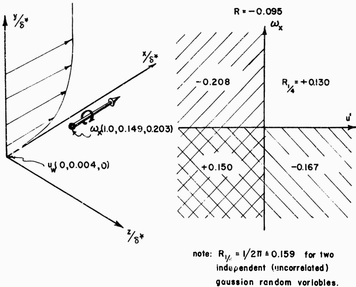
Fig.12 Contributions to correlation between streamwise vorticity and velocity in the sublayer from four quadrants in the u, \omega_x plane. U_\infty = 204 ft/sec.
