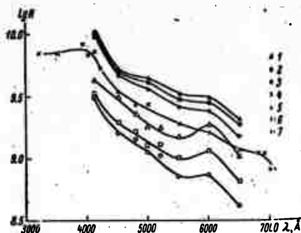
Fig. 1. Spectral energy distribution in a laser spark.
