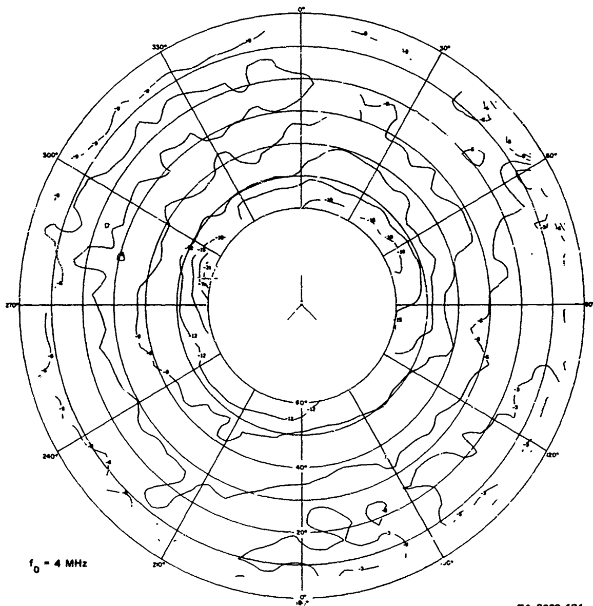
FIGURE A-40 MEASURED PATTERN OF 30° SLANT-WIRE ANTENNA AT LODI. E_\theta AT 4 MHz
