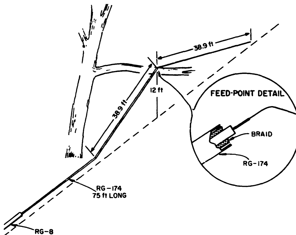
FIGURE 18 LONG-WIRE ANTENNAS
