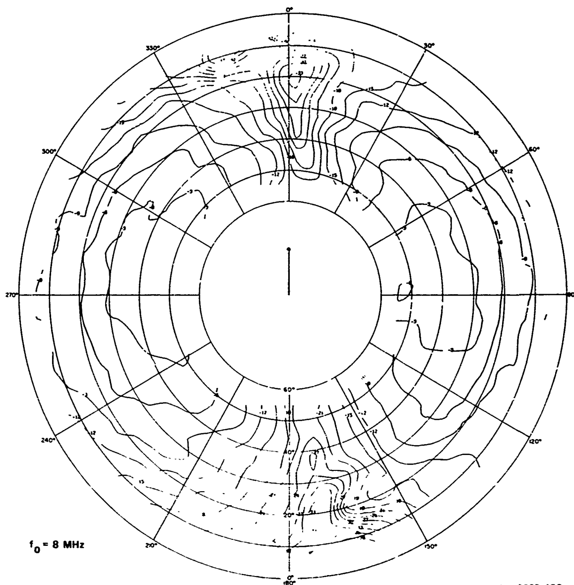
FIGURE A-29 MEASURED PATTERN OF 2:1 INVERTED-L ANTENNA IN FOREST AT ALMANOR, E_\phi AT 8 MHz
