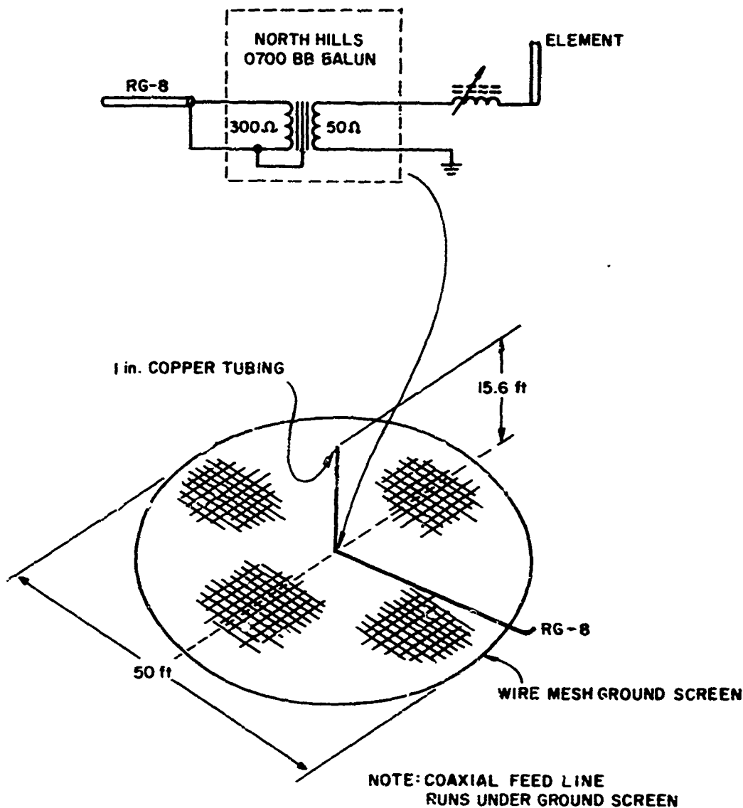
FIGURE 13 MONOPOLE ANTENNAS
