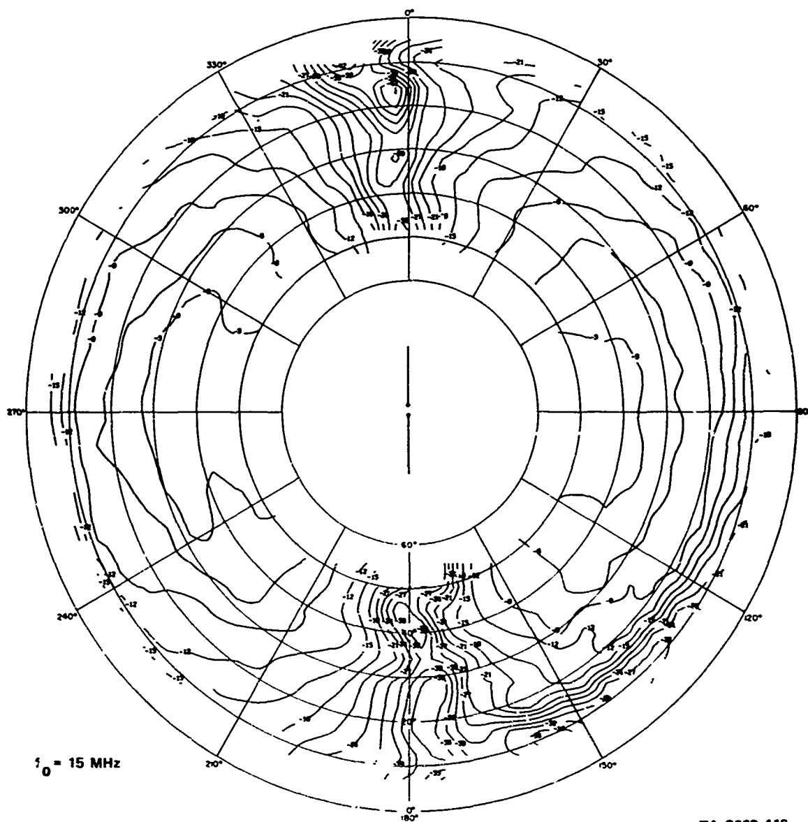
FIGURE A-18 MEASURED PATTERN OF 15-MHz BALANCED DIPOLE IN CLEARING AT ALMANOR, E_\phi AT 15 MHz
