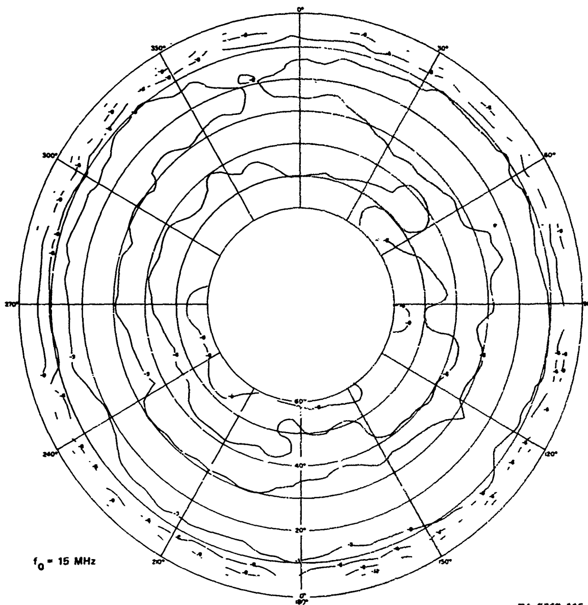
FIGURE A-22 MEASURED PATTERN OF MONOPOLE ANTENNA AT LODI, E_\theta AT 15 MHz
