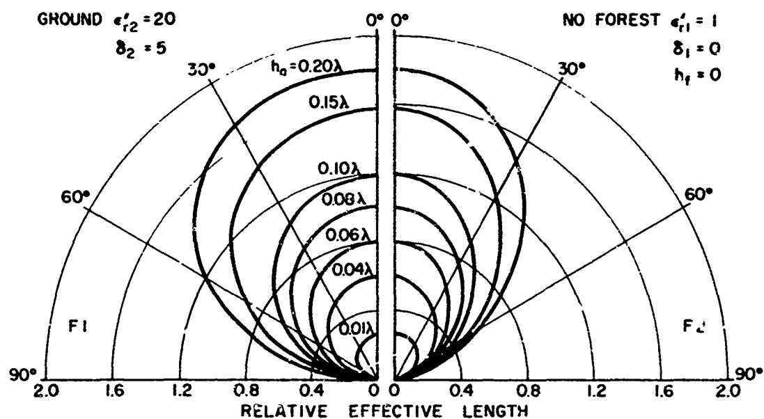
(a) EFFECTIVE ANTENNA LENGTH FOR VARIOUS HEIGHTS, h_0 — NO FOREST
