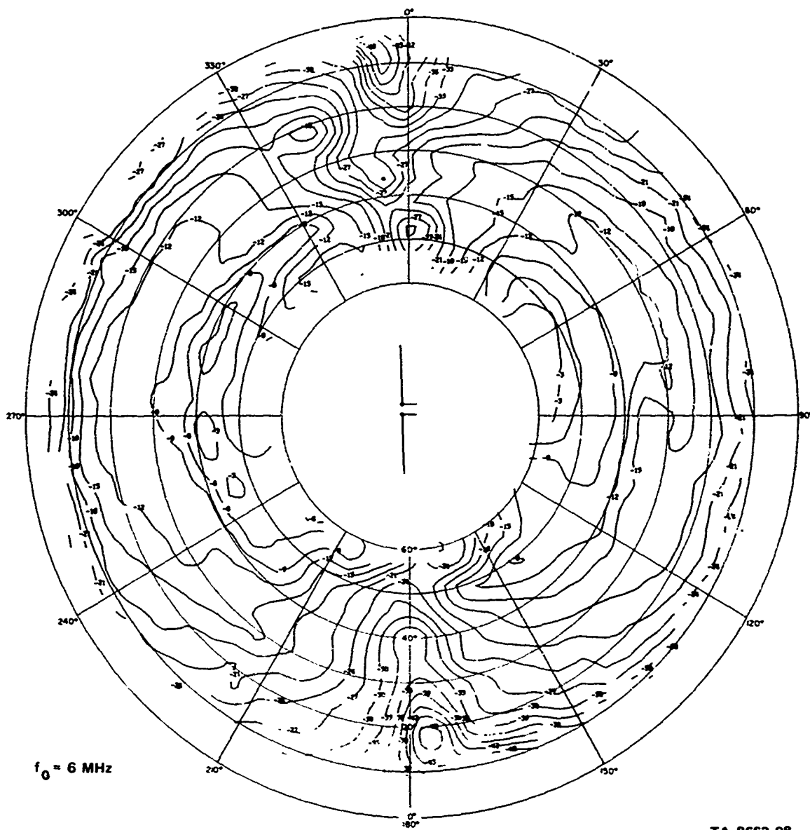
FIGURE A-4 MEASURED PATTERN OF 2-FOOT-HIGH UNBALANCED DIPOLE IN FOREST AT ALMANOR, E_\phi AT 6 MHz
