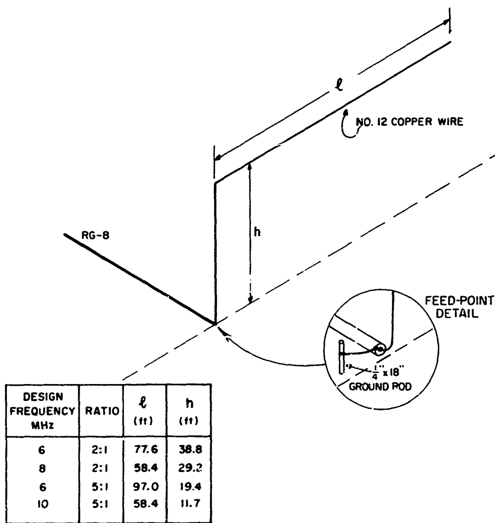
FIGURE 15 INVERTED-L ANTENNAS
