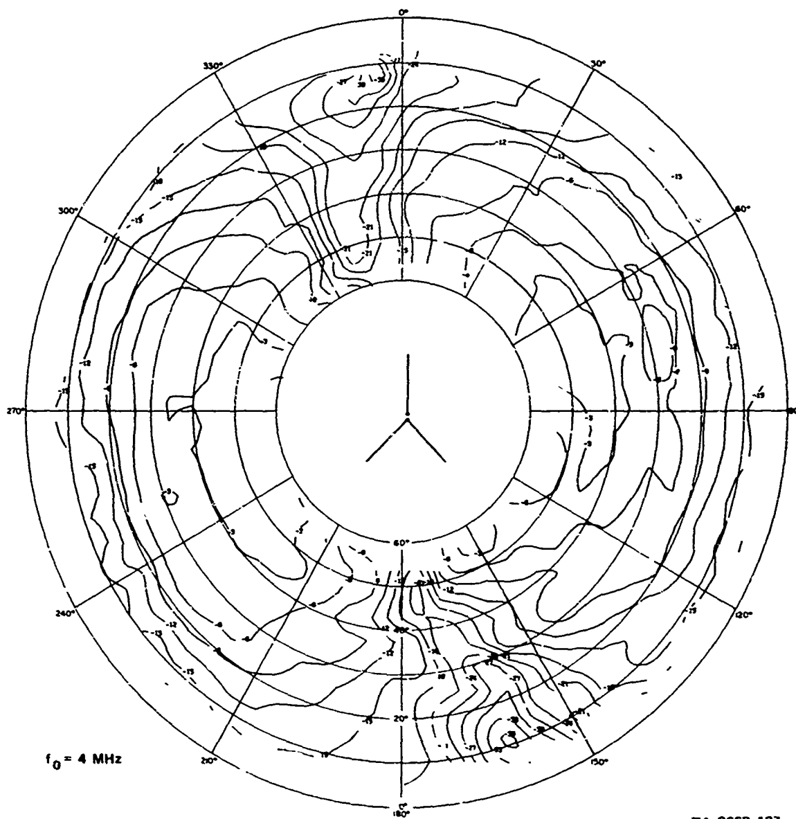
FIGURE A-43 MEASURED PATTERN OF 30° SLANT-WIRE ANTENNA IN FOREST AT ALMANOR, E_\phi AT 4 MHz
