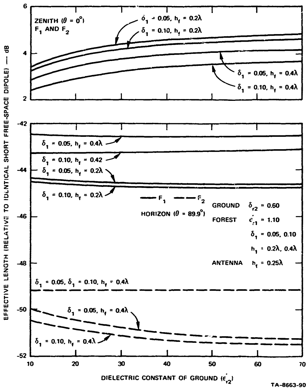
FIGURE 37 EFFECTIVE ANTENNA LENGTH AS A FUNCTION OF GROUND PERMITTIVITY— h_a = 0.25\lambda
