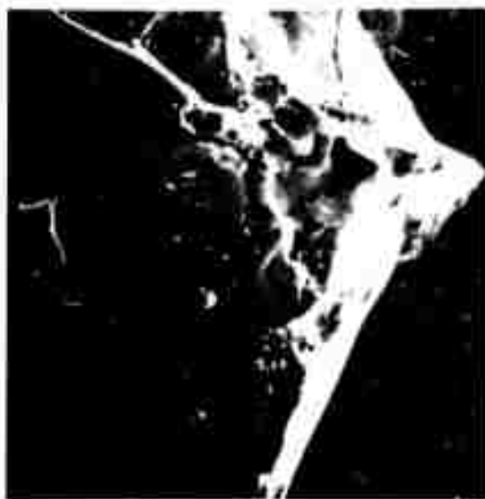
Fig. 16a Entrance Face Damage to \text{LiNbO}_3 when \text{TEM}_{00} Mode 1.06 \mu\text{m} Laser is Focused on the Entrance Face.
