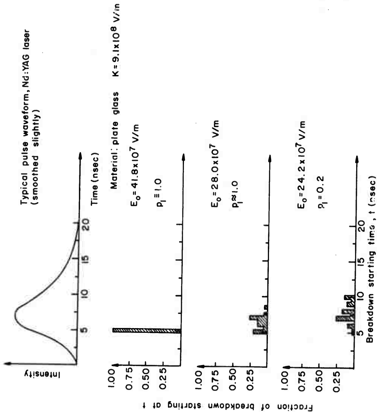
Fig. 30 Distribution of Surface Breakdown Starting Times for Plate Glass for Three Different Damage Probabilities.
