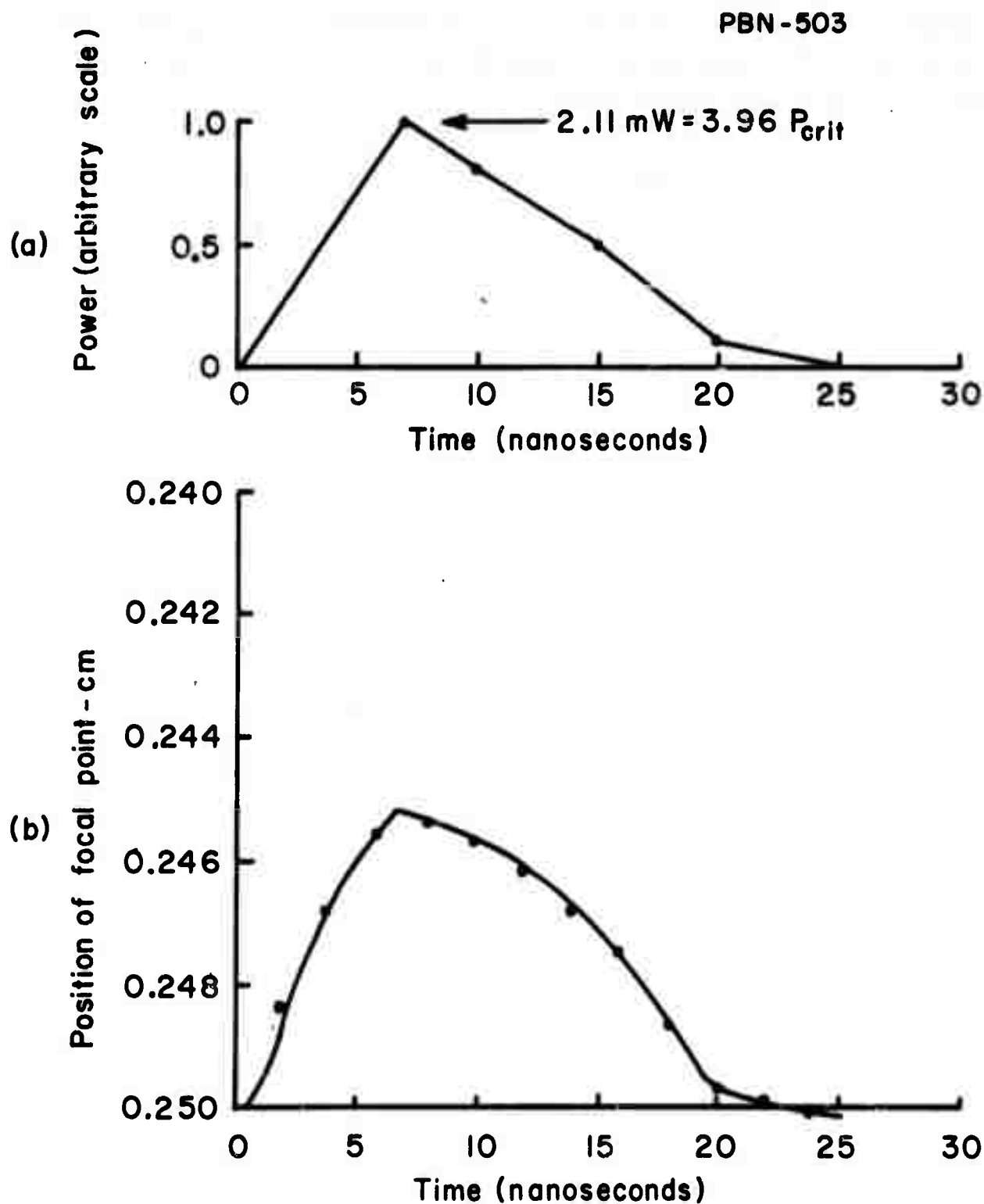
Fig. 36 Calculated Distance of the Focal Point From Entrance Face as a Function of Time for an Initial Beam Radius of 0.184 mm and a Convergence Angle of 73.6 Milliradians.
