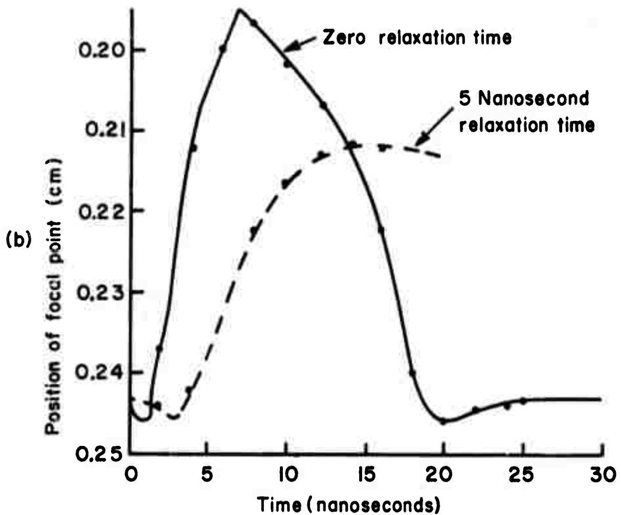
Fig. 37 Calculated Distance of the Focal Point from Entrance Face as a Function of Time for an Initial Beam Radius of 50 \mu\text{m} and a Convergence Angle of 20 Milliradians.
