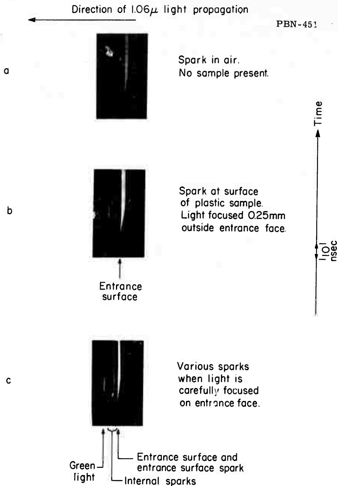
Fig. 20 Breakdown on the Entrance Face of a Acrylic Plastic Sample. a. Breakdown in air with no sample present. b. Breakdown near the surface of the sample. The focus was 0.25 mm outside the entrance face. c. Breakdown when focused on the sample's entrance face. Note internal sparks are also produced.
