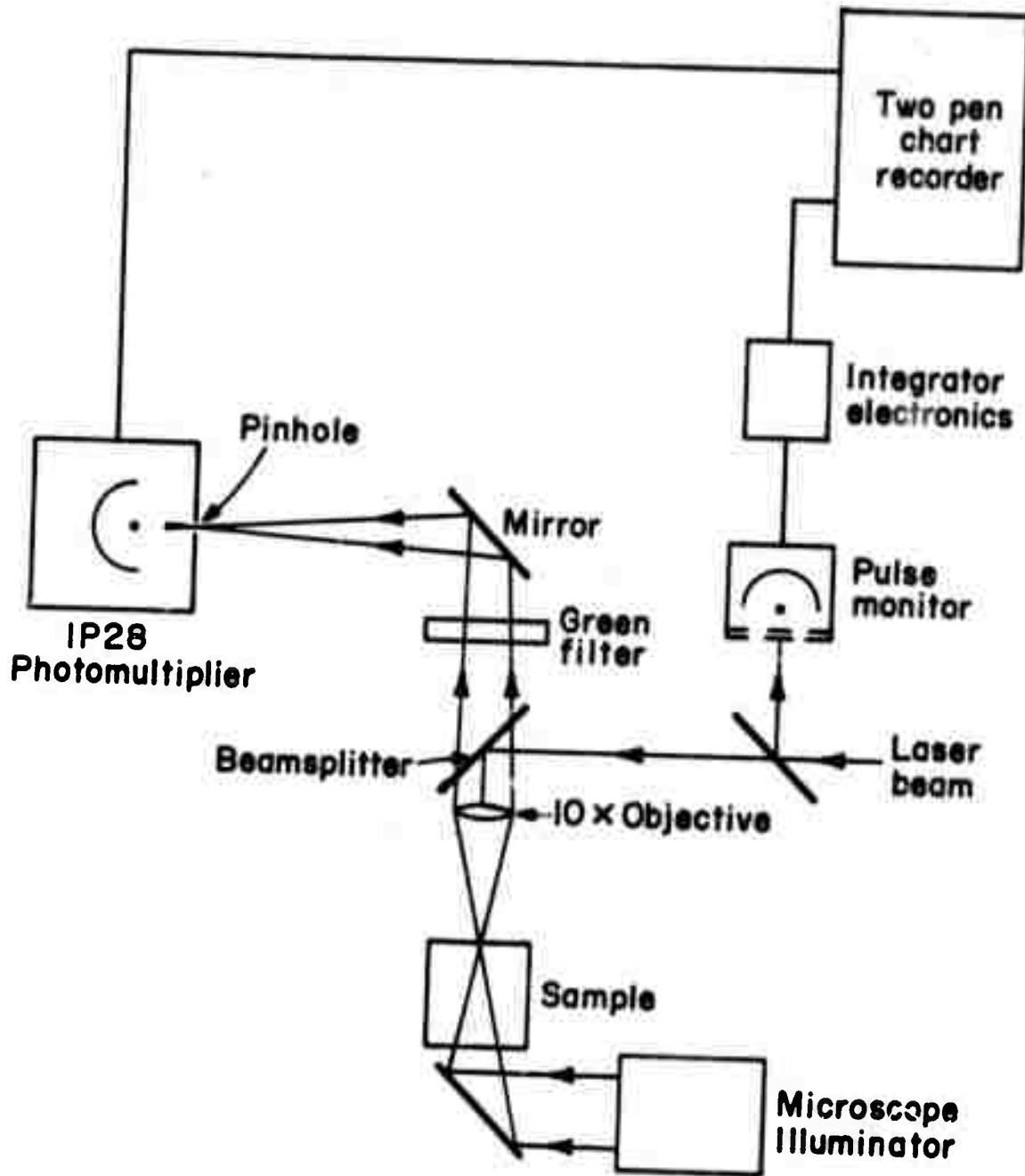
Fig. 27 Schematic Diagram of Automatic Pulse and Damage Monitoring Apparatus.
