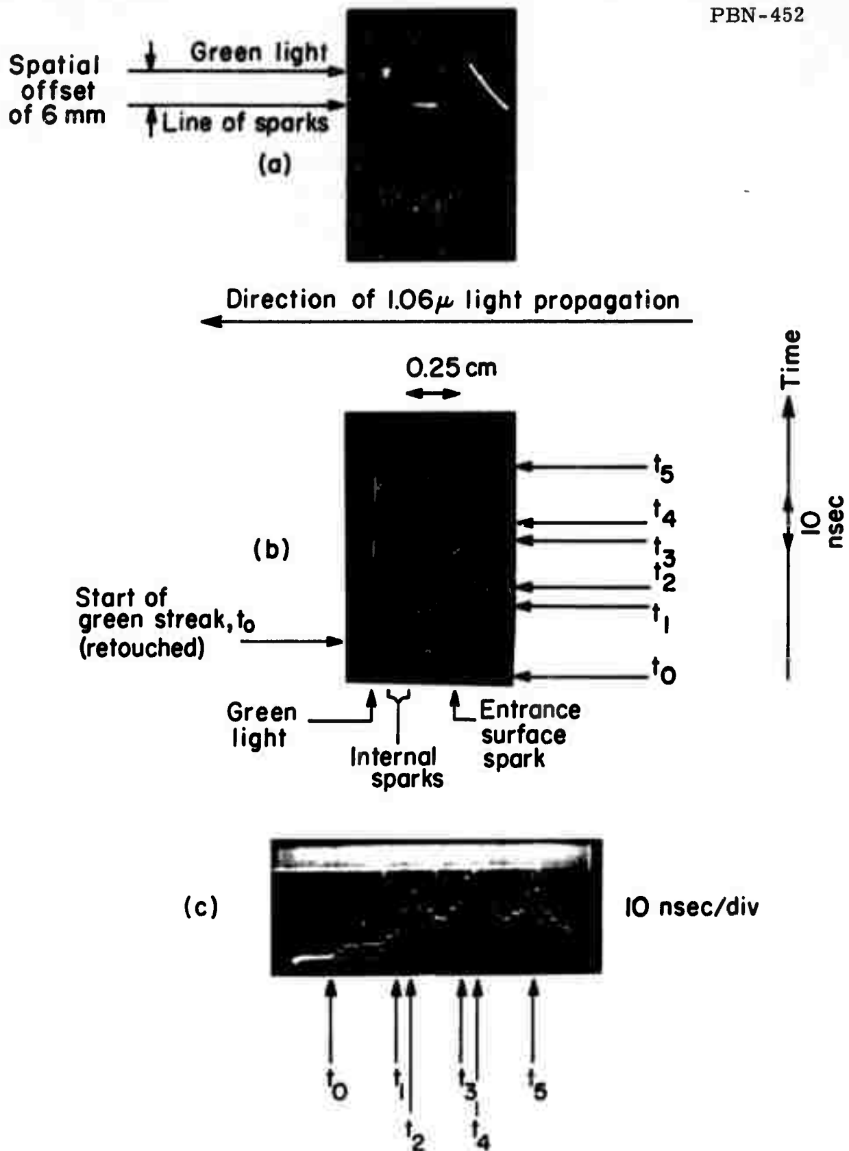
Fig. 21 Streak Photographs of Laser-Induced Sparks in Plate Glass. a. Unstreaked sparks and green light b. Streaked sparks and green light c. Waveform of the pulse which produced the sparks in (b). Arbitrary vertical scale.
