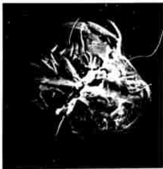
Fig. 16b Exit Face Damage to \text{LiNbO}_3 when Same Lens as Used Above is Set to Focus the Same Pulse as Used Above on the Exit Face.
