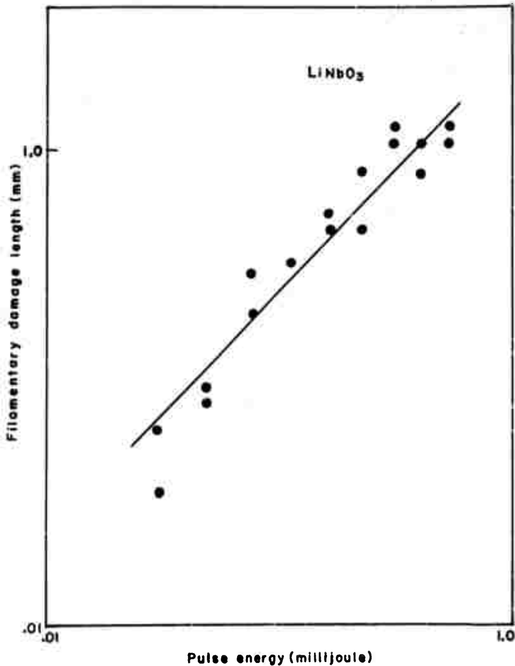
Fig. 11 Filamentary Damage Length Versus Pulse Energy Where the 1.06\text{ }\mu\text{m} TEM 00 Mode Laser is Focused Inside the Crystal. Pulse duration = 7 nsec. If there were no self-focusing, the focal diameter would have been 0.006 cm.
