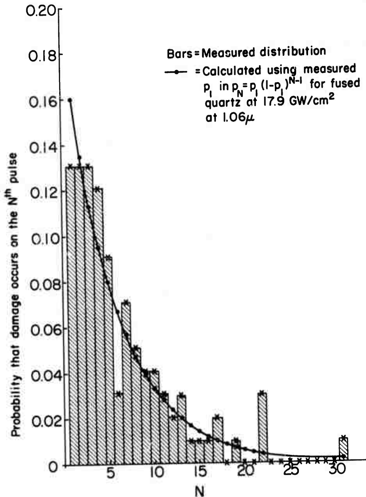
Fig. 26 Probability that Damage Occurs on the Nth pulse Versus N for the Fused Quartz. A 17.9 GW/cm 2 TEM 00 mode 1.064 \mu m beam was used.
