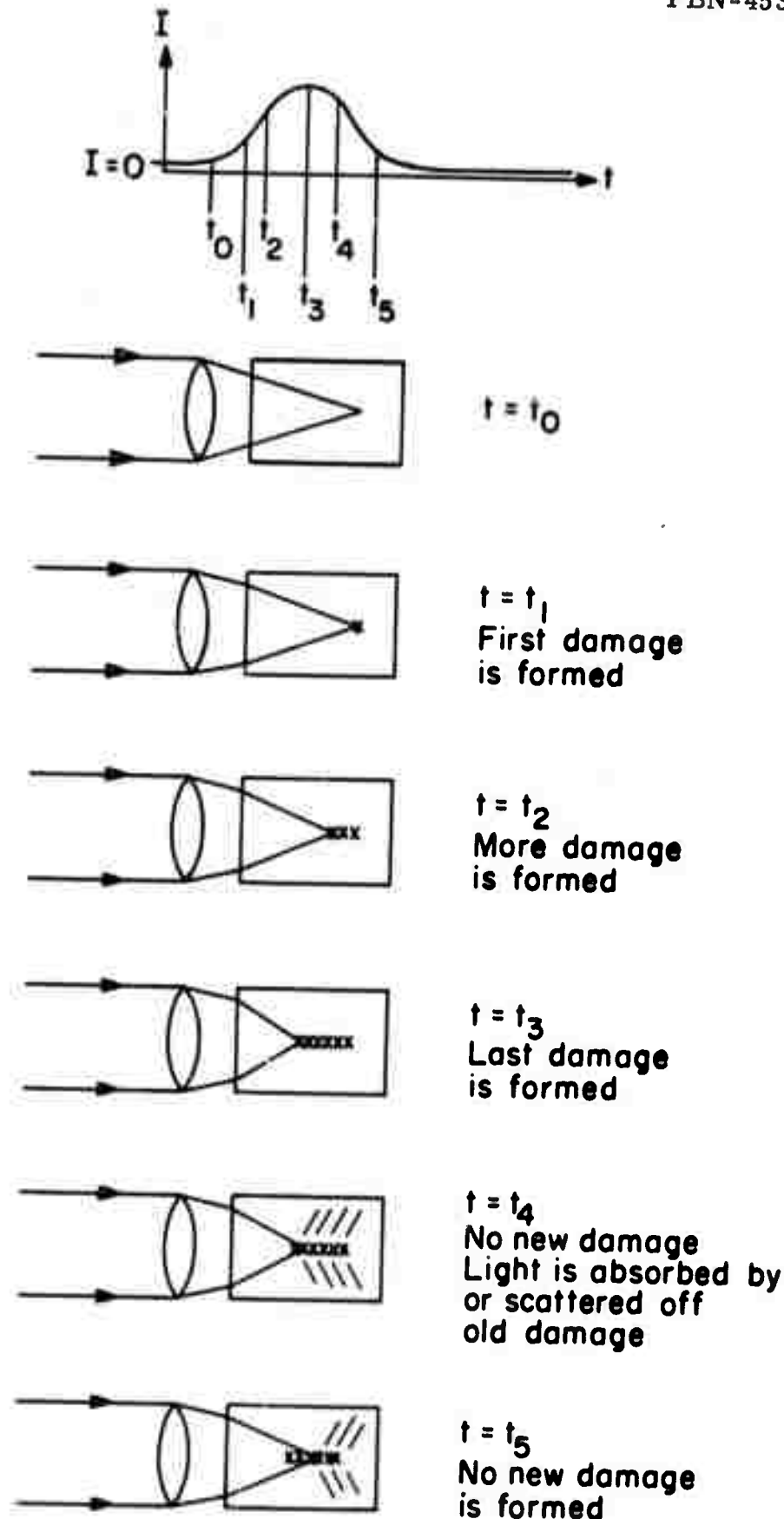
Fig. 22 Sketch of the Sequence of Breakdown Formation Assuming a Fast Response Self-Focusing Process and a Smooth Pulse Waveform.
