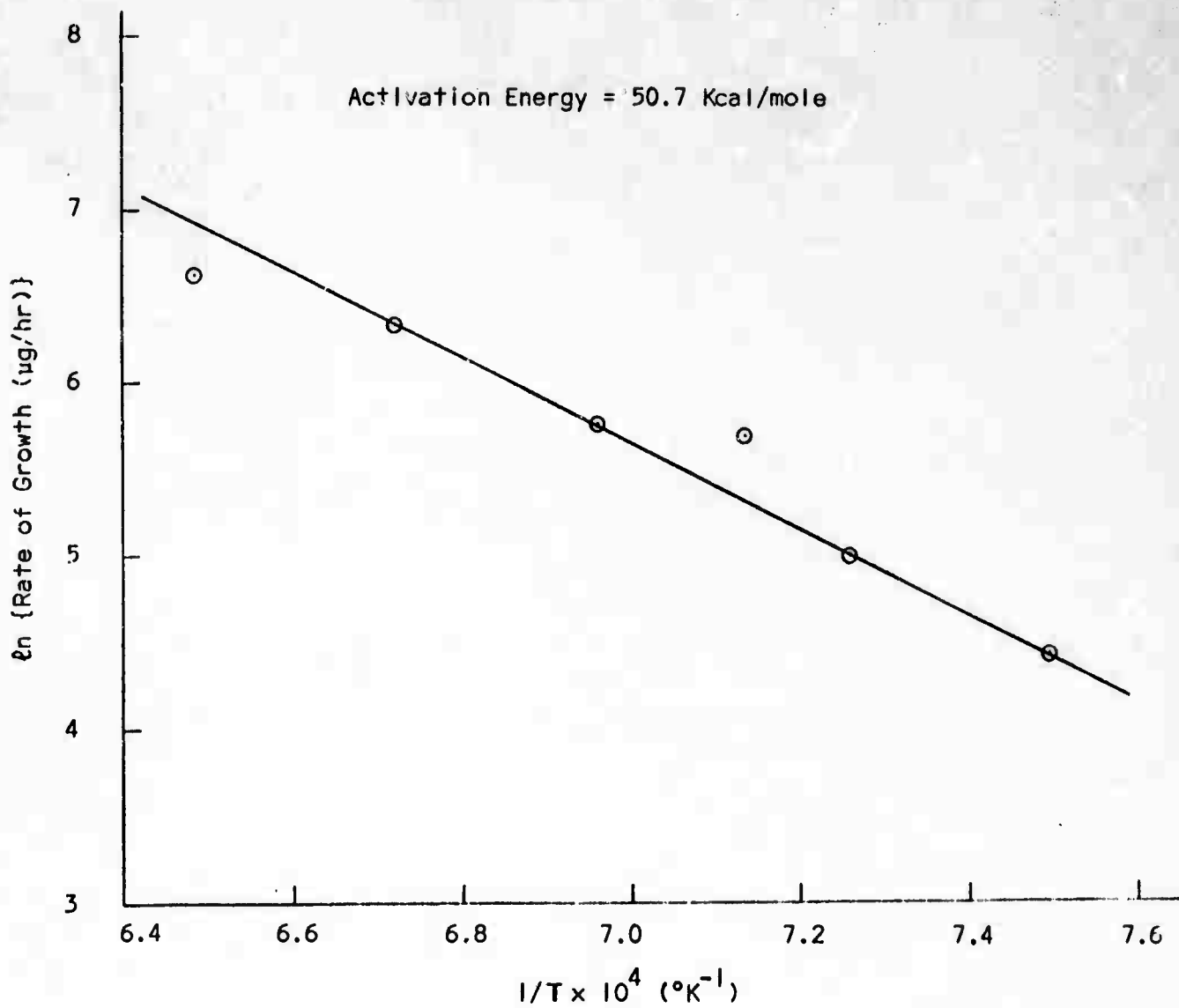
DIAMOND (0-1 \mu ) GROWTH RATE DEPENDENCE ON TEMPERATURE AT A METHANE PRESSURE OF 3.0 \times 10^{-3} TORR. WEIGHT OF SAMPLE = 60 mg.
