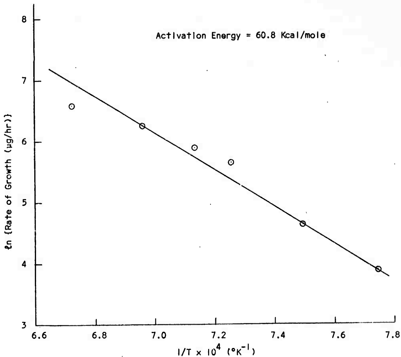
DIAMOND (0-1 \mu ) GROWTH RATE DEPENDENCE ON TEMPERATURE AT A METHANE PRESSURE OF 5.0 \times 10^{-3} TORR. WEIGHT OF SAMPLE = 60 mg.
