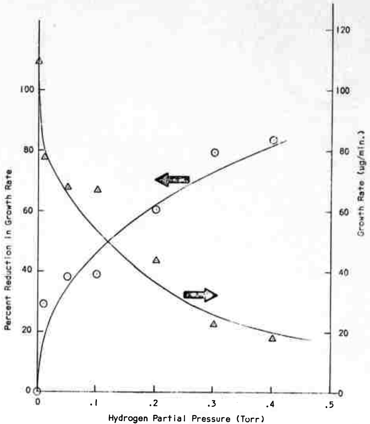
PERCENT REDUCTION OF GROWTH RATE (AS COMPARED TO PURE METHANE GROWTH RATE) OF DIAMOND (0-1 \mu ) AND ABSOLUTE GROWTH RATE (WEIGHT OF SAMPLE = 60 mg.) AS A FUNCTION OF HYDROGEN PARTIAL PRESSURE AT A METHANE PRESSURE OF 0.1 TORR AND 1170.0°C.
