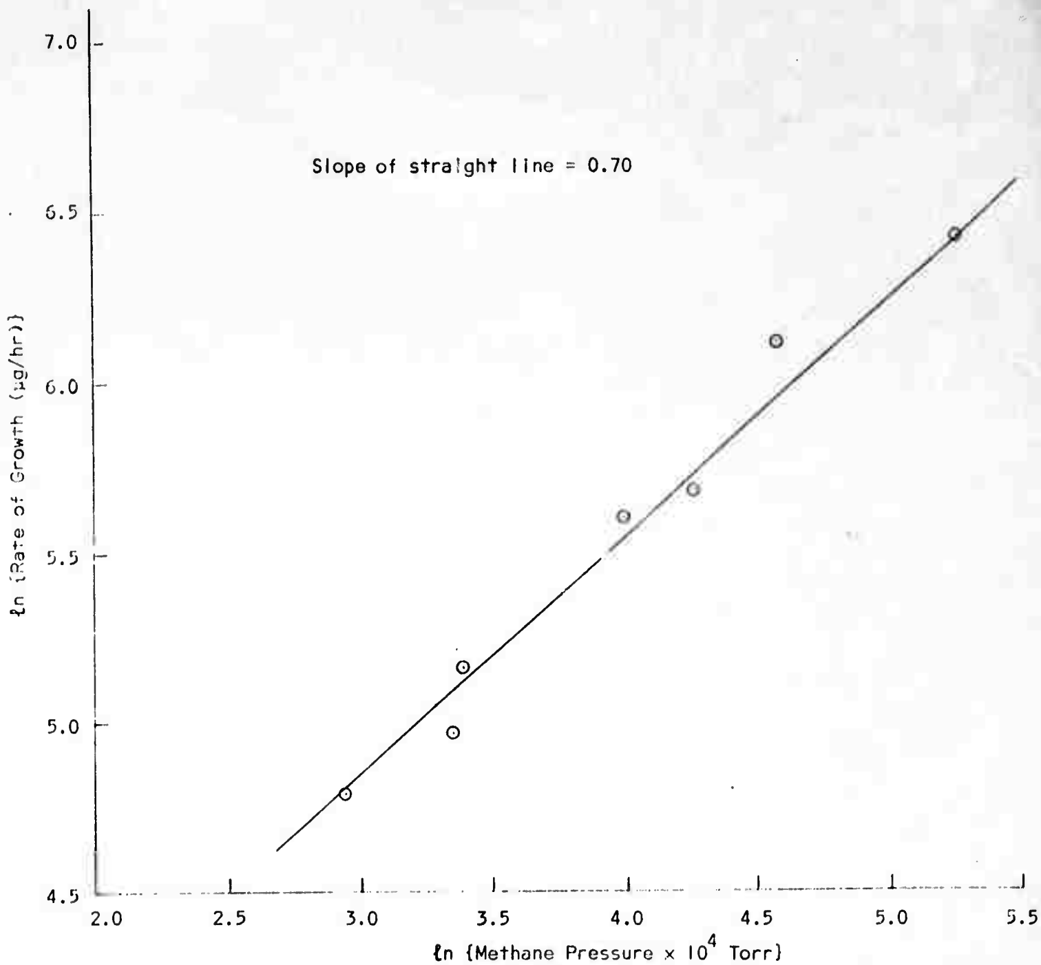
DIAMOND (0-1%) GROWTH RATE AS A FUNCTION OF METHANE PRESSURE AT 1128.7°C. WEIGHT OF SAMPLE = 60 mg.
