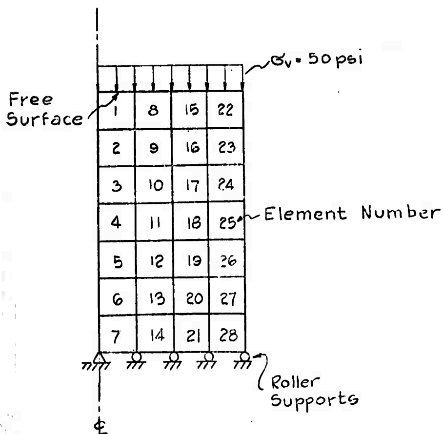
(b) Axisymmetric Finite Element Model
