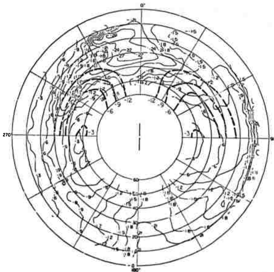
FIGURE B-16 CONTOUR PLOT OF THE MEDIAN RESPONSE OF THE HORIZONTAL BALANCED DIPOLE IN THE FOREST— E_0 AT 100 MHz
