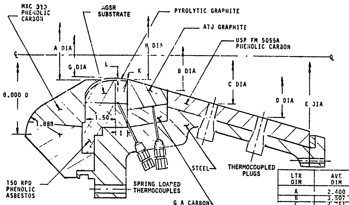
FIGURE 2-1 SCHEMATIC OF RESTART NOZZLE
