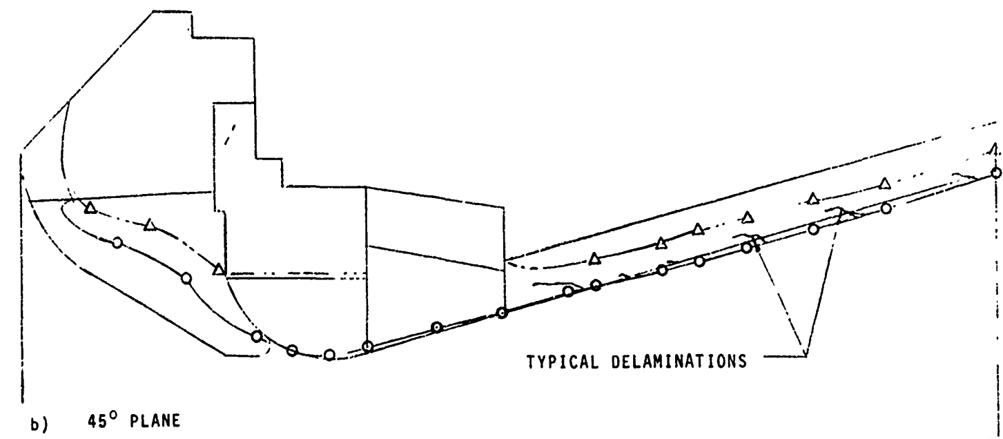
FIGURE 3-5 PRE, POST, AND CHAR LINE CONTOURS FOR NOZZLE NO. 8
