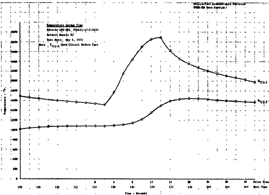
2) Pulse No. 3, Thermocoupled Plug at A/A* = 4.29 Figure B-5. (Continued)
