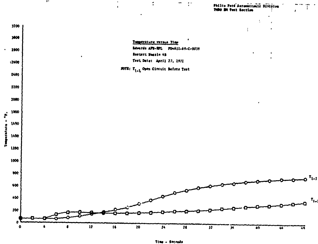
h) Pulse No. 2, Thermocoupled Plug at A/A^* = 6.66 Figure B-1. (Continued)
