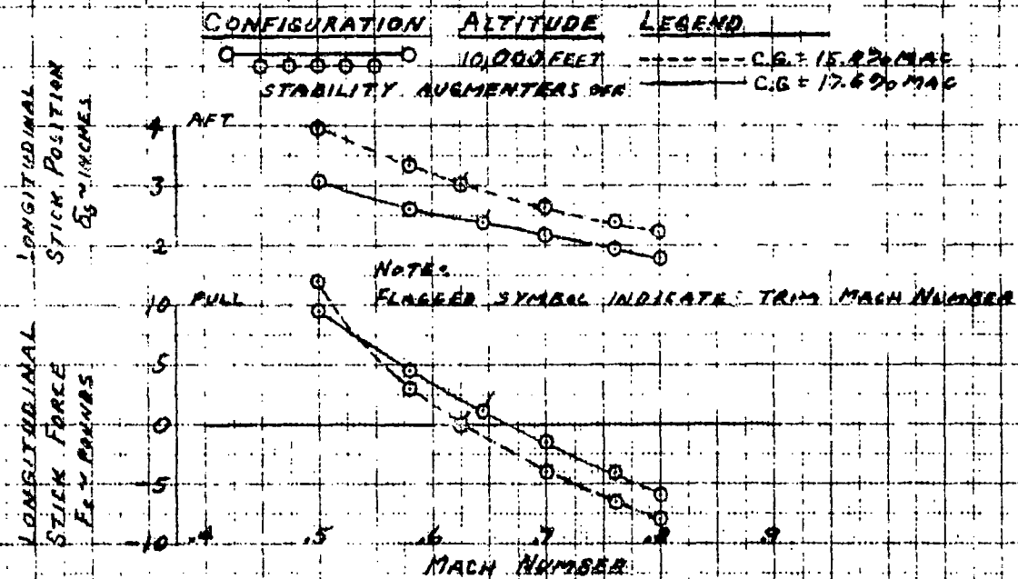
LONGITUDINAL STATIC STABILITY FIGURE 5 (3.2.1.1)
