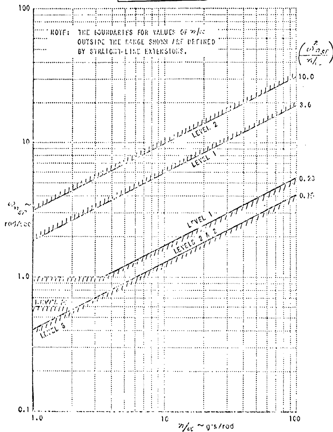
FIGURE 1. Short-Period Frequency Requirements - Category A Flight Phases
