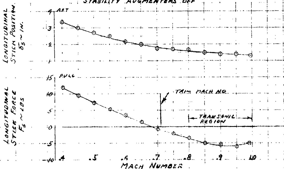
LONGITUDINAL STATIC STABILITY FIGURE 1(3.2.1.1)
