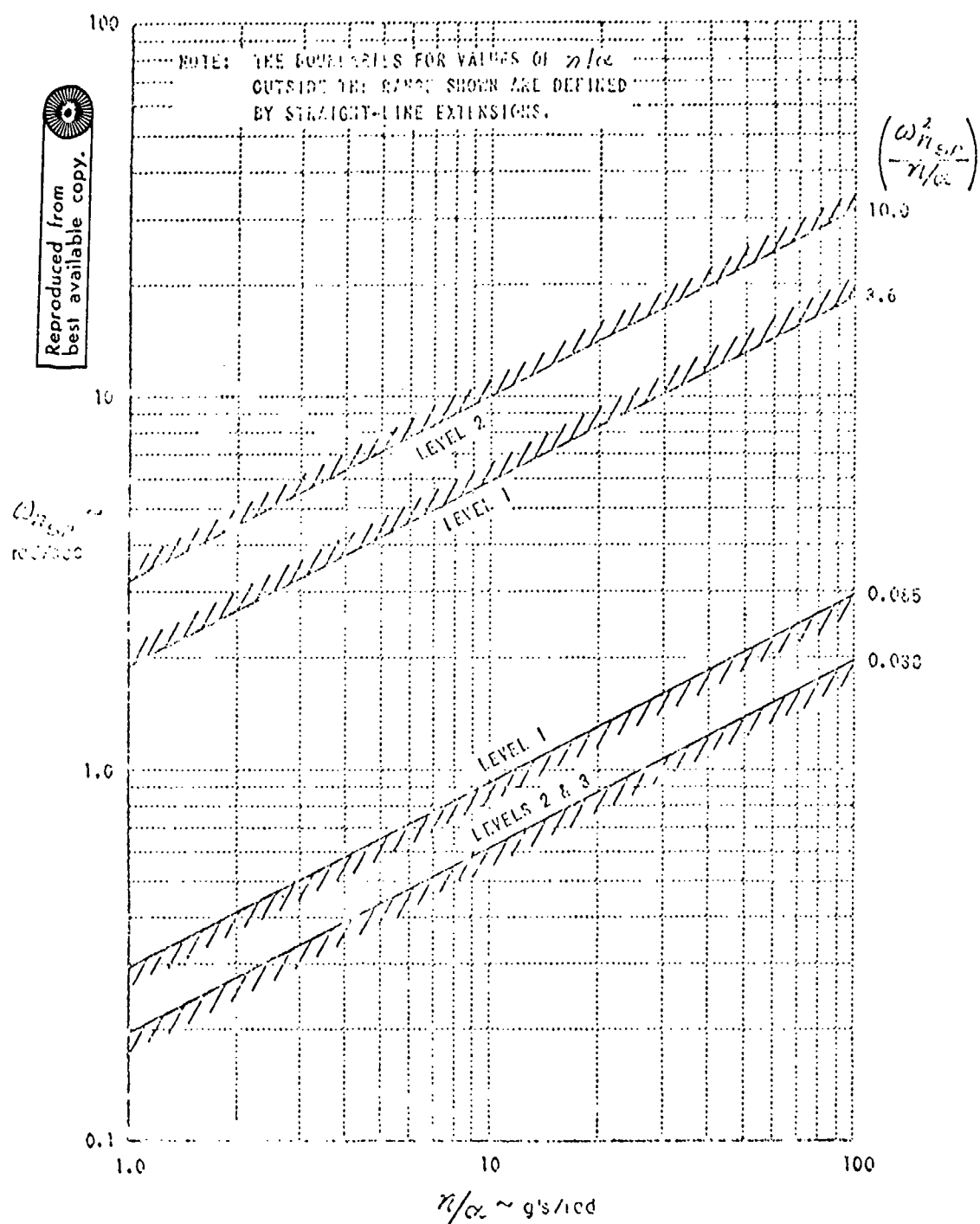
FIGURE 2. Short-Period Frequency Requirements - Category B Flight Phases
