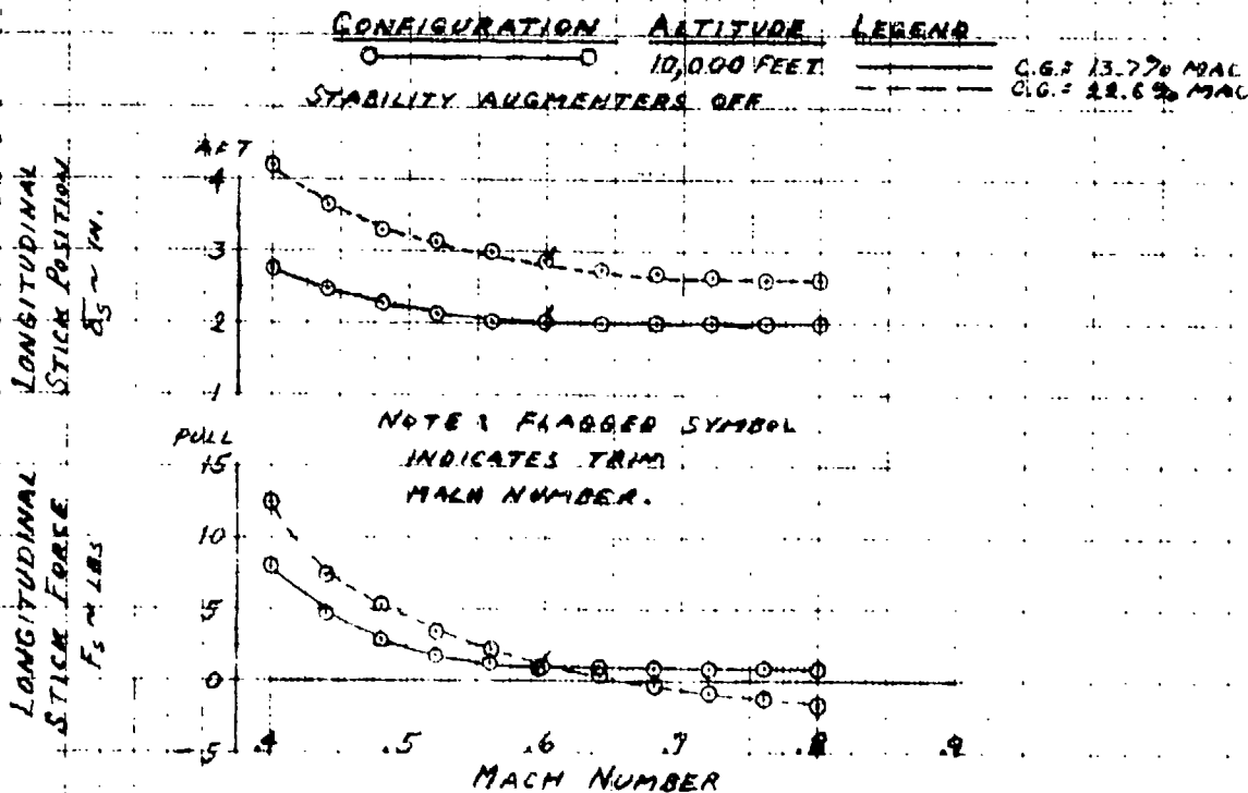
LONGITUDINAL STATIC STABILITY FIGURE 2 (3.2.1.1)
