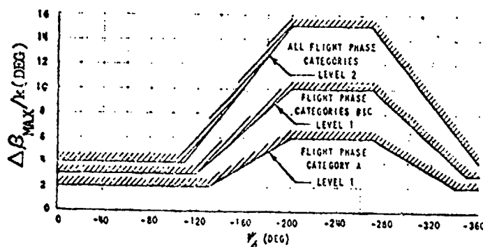
FIGURE 6. Sideslip Excursion Limitations
