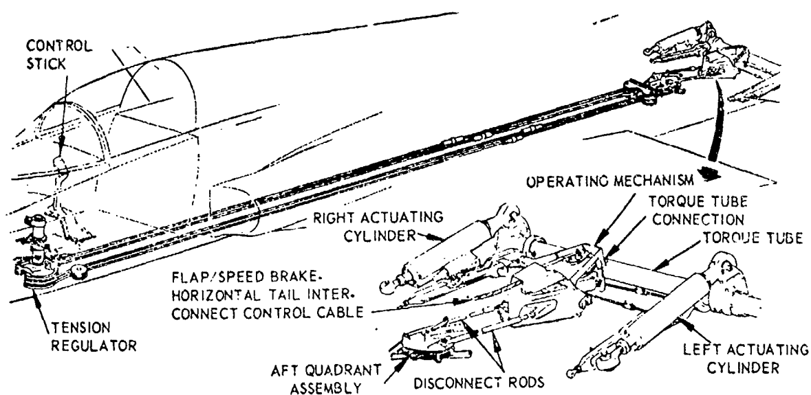
HORIZONTAL STABILIZER CONTROL SYSTEM
