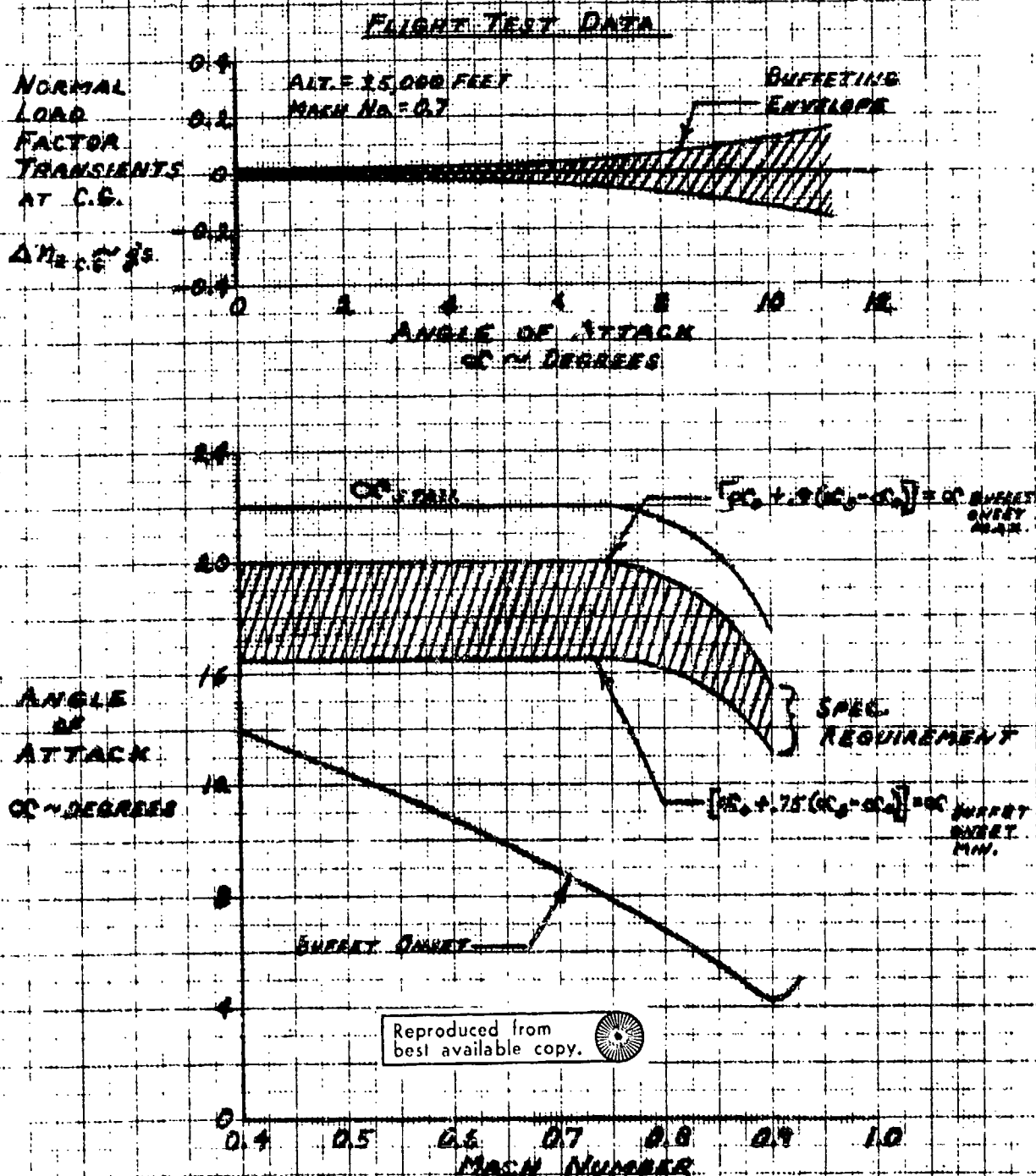
WARNING RANGE FOR ACCELERATED STALLS FIGURE 1 (3.4.2.2.2)
