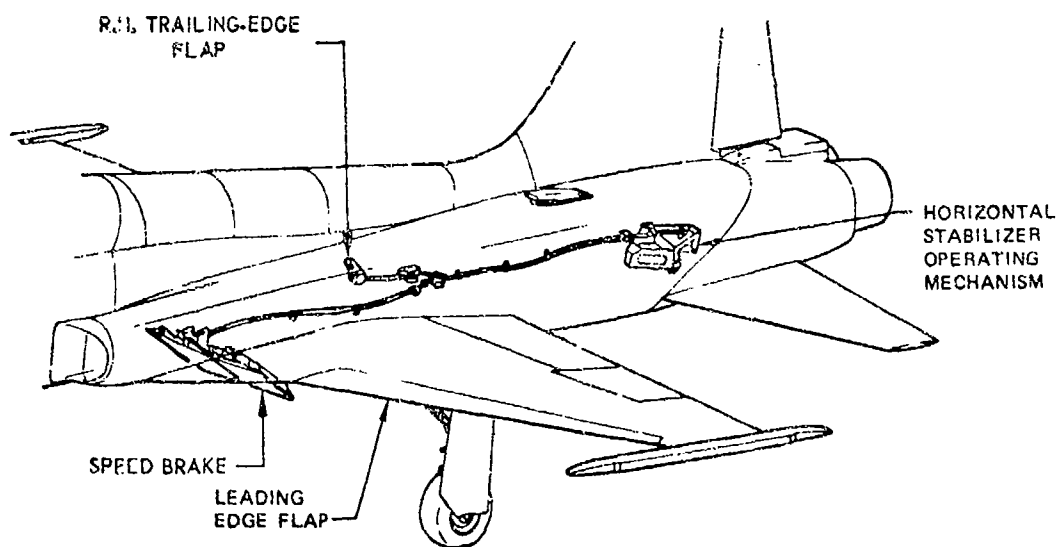
FLAP/SPEED BRAKE -- HORIZONTAL STABILIZER INTERCONNECT
