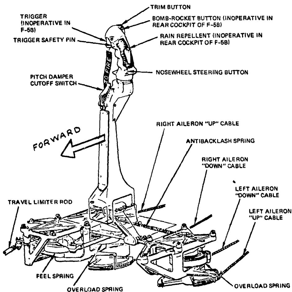
CONTROL STICK FIGURE 2.1
