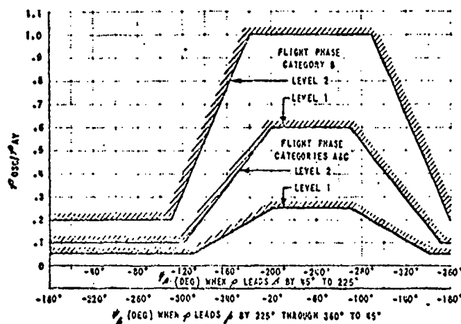
FIGURE 4. Roll Rate Oscillation Limitations
