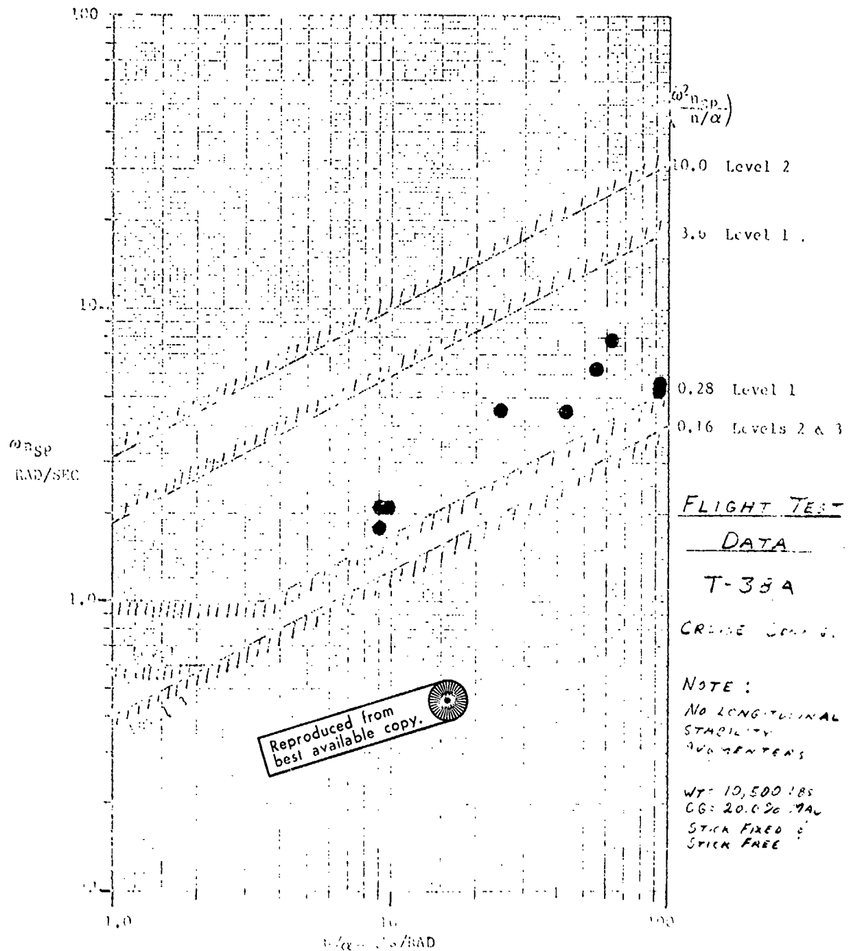
SHORT PERIOD FREQUENCY AND ACCELERATION SENSITIVITY FIGURE 4 (3.2.2.1.1)
