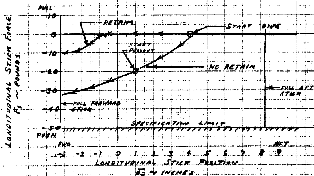
LONGITUDINAL CONTROL FORCES IN DIVES PERMISSIBLE FLIGHT ENVELOPE
