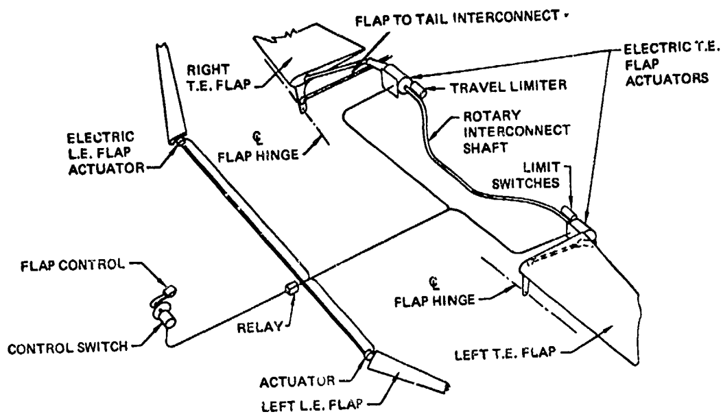
FLAP CONTROL SYSTEM
