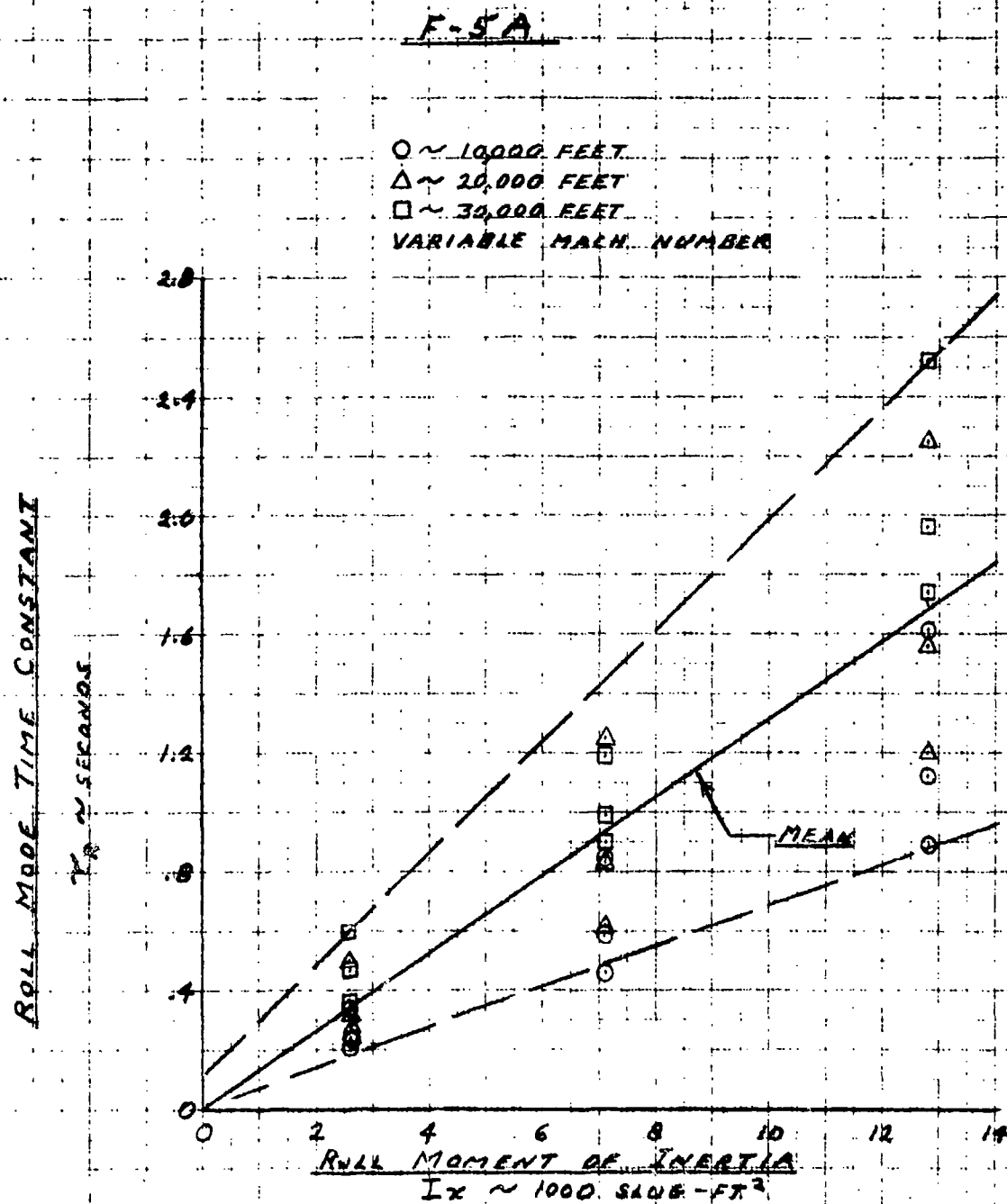
ROLL MODE FIGURE 3 (3.3.1.2)
