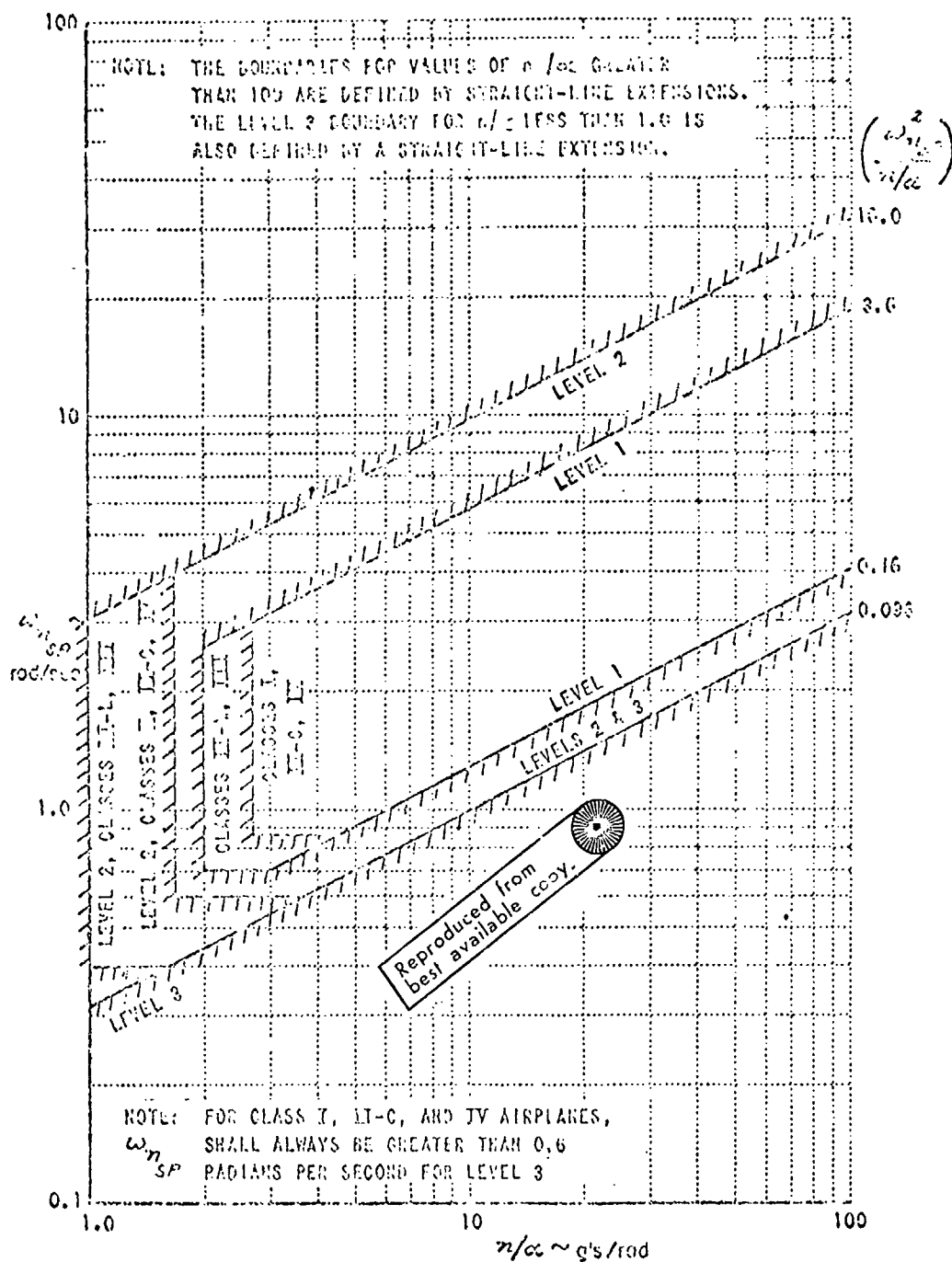
FIGURE 3. Short-Period Frequency Requirements - Category C Flight Phases
