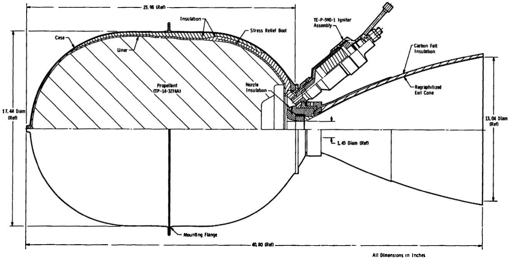
a. Schematic Fig. 1 Thiokol Chemical Corporation TE-T-607-1 Solid-Propellant Rocket Motor
