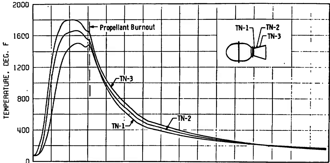
a. Nozzle Temperatures TN-1, TN-2, and TN-3
