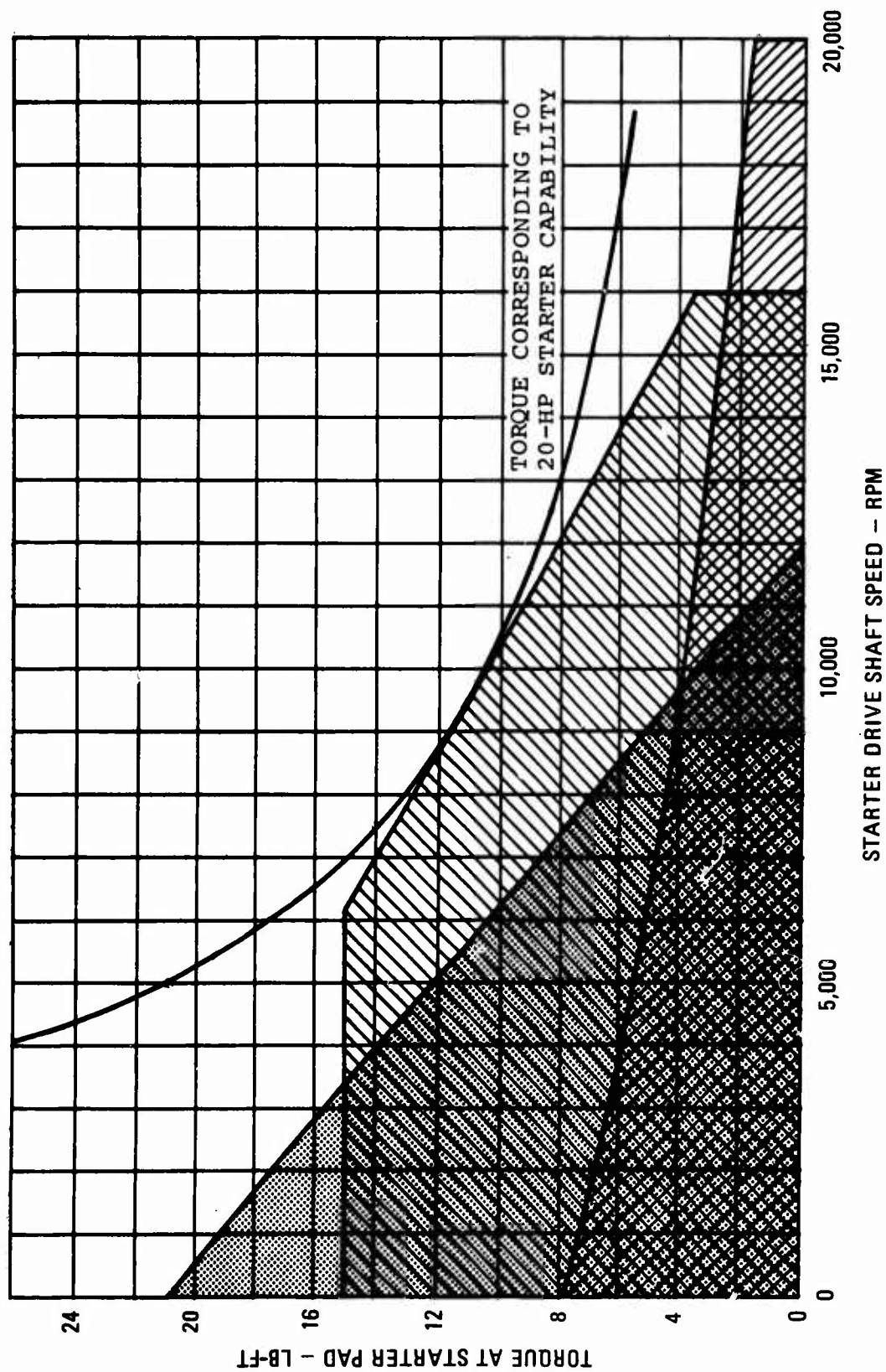
Figure 4. Main-Engine Starting Torque Requirements.
