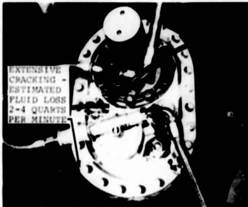
Figure 21. Damage to Right-Hand Boost Pump Plate (Test 1).
