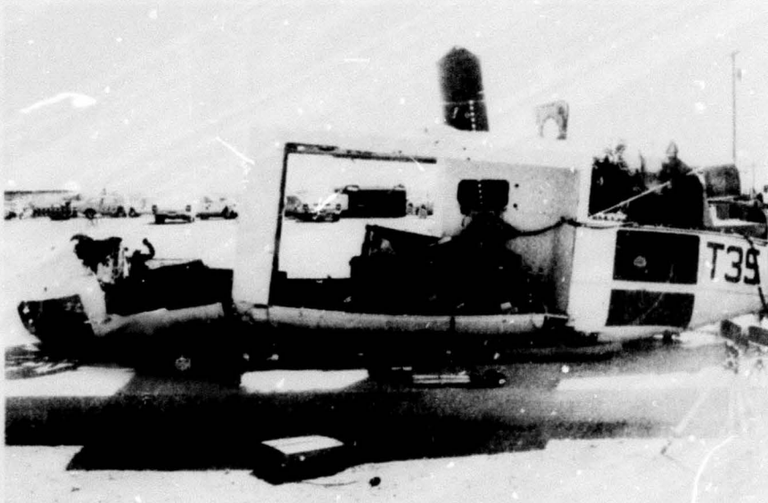
Figure 12. Fuselage Deflection - Left Side (Test 1).
