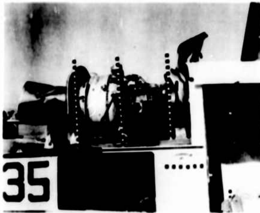
Figure 15. Posttest Position of Engine (Test 1).
