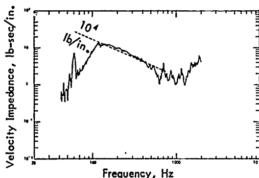
Figure 17. Summed Impedance at Location S
