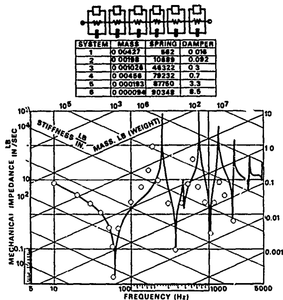
Fig. 11 - Computer Simulation - Cantilever Beam Impedance
