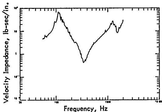
Figure 15. Impedance of Component Package
