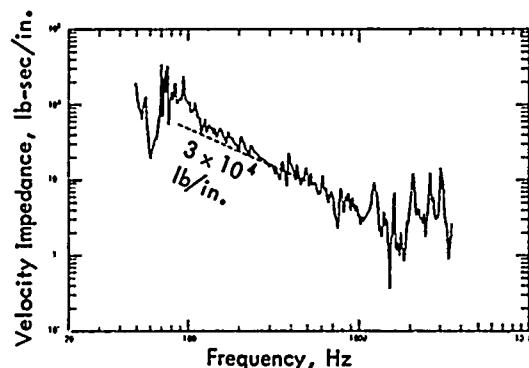
Figure 16. Summed Impedance at Location R
