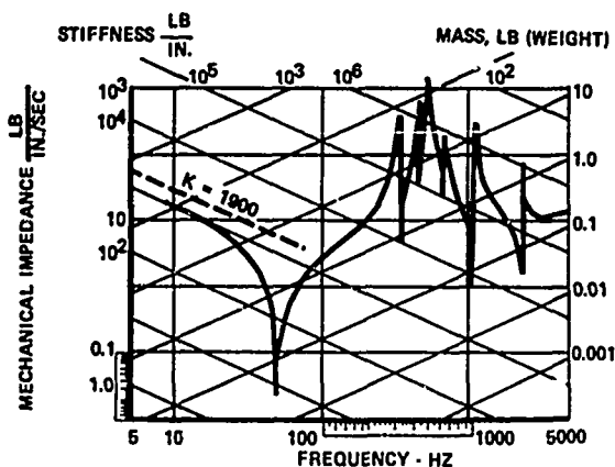
Fig. 8 - Impedance of the Cantilever Beam Drive Pt. 4 in from Tip
