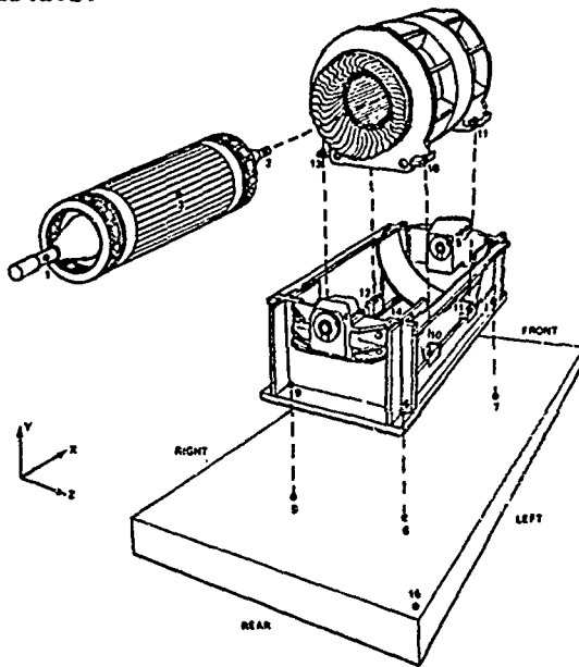
Fig. 3 - Components Selected for the Dynamic Design Analysis.
