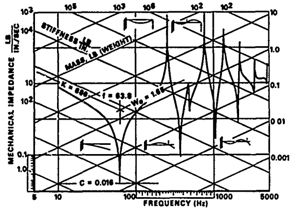
Fig. 7 - Impedance of the Cantilever Beam Drive Pt. - Tip
