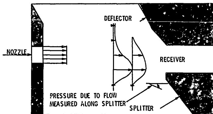
Fig. 13 - Pressure Profiles, First Stage Nozzle, Control Input = 0.034 lbm/sec, Nozzle Supply = 10 psig Original Configuration
