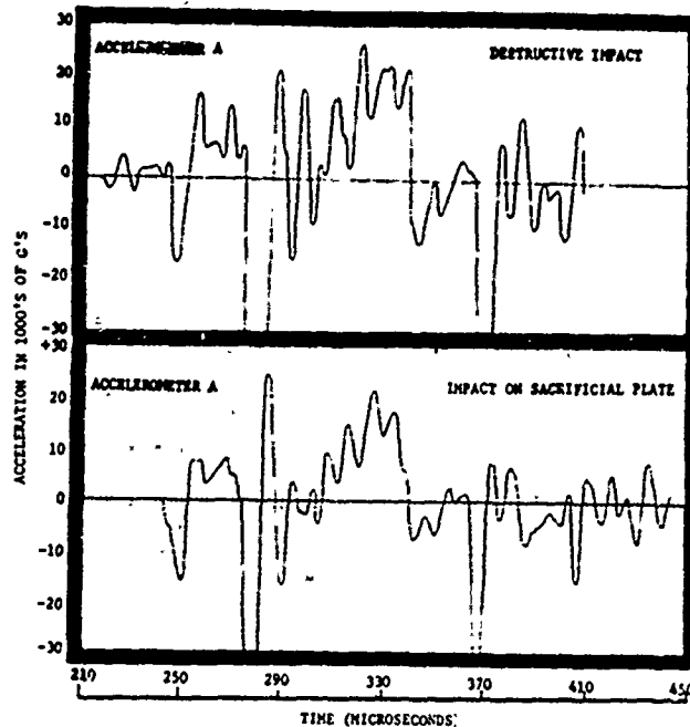
Fig. 6 - Ballistic Impact Experiment Accelerometer Traces
