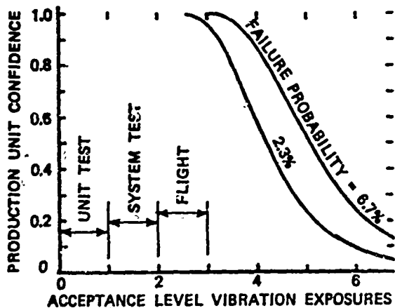
FIGURE 13. EFFECT OF MULTIPLE EXPOSURES ON PRODUCTION UNIT CONFIDENCE (SEE TEXT FOR ASSUMPTIONS)
