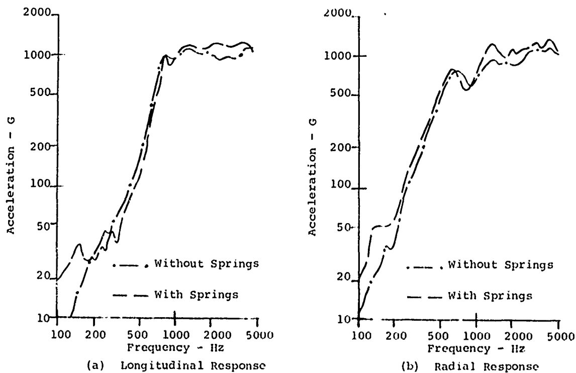
Figure 12 Effect at separation of separation springs
