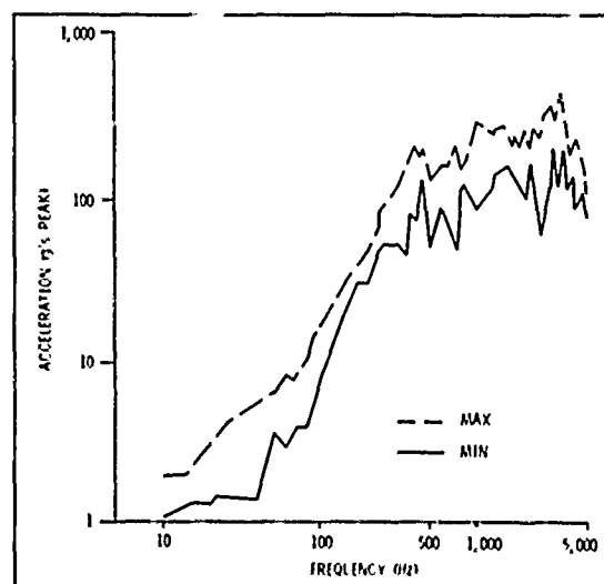
FIG. 7. Typical Range of Maximum and Minimum Undamped Shock Spectra (Tail Vertical)
