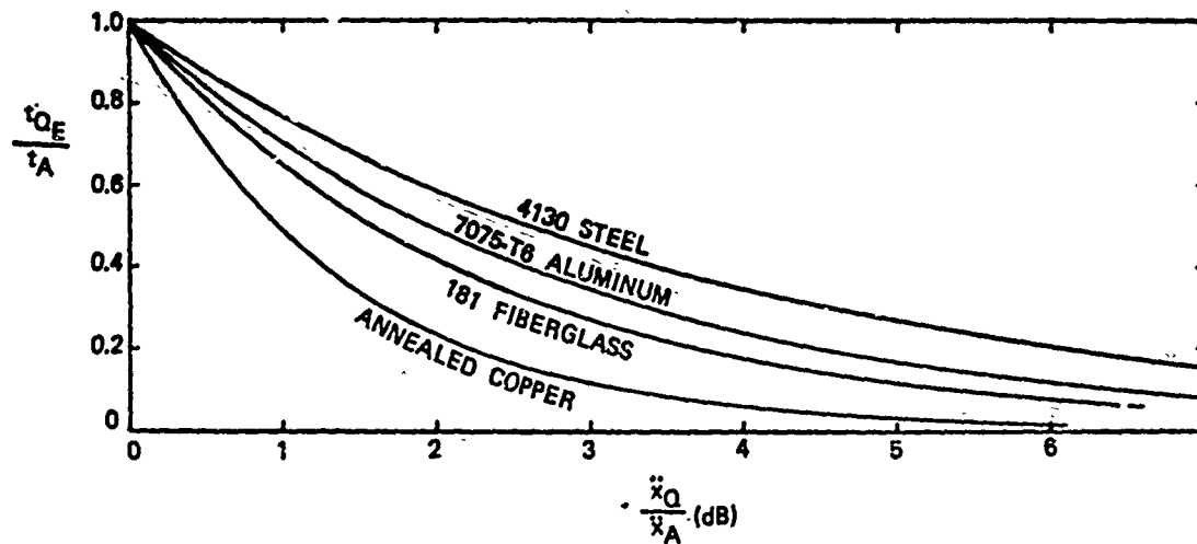
FIGURE 9. EFFECT OF MATERIAL PROPERTIES ON "EQUIVALENT-TIME-AT-QUALIFICATION-LEVEL"
