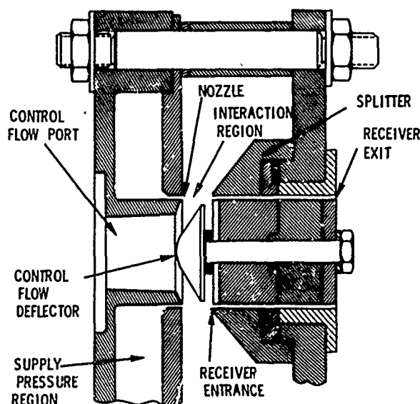
Fig. 8 - Drawing of Annular Slot model
