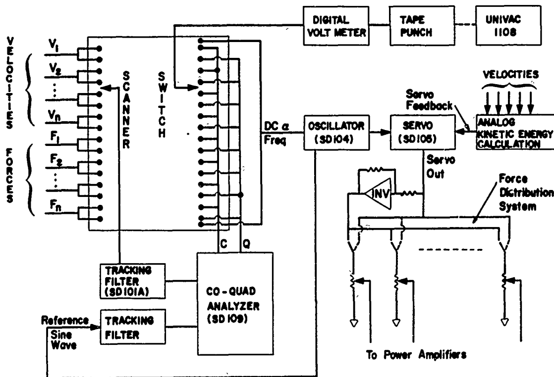
Fig. 3 - Instrumentation system
