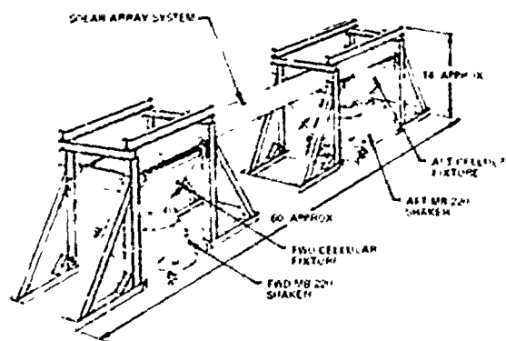
Fig. 5 - Solar array radial axis vibration setup using cellular fixtures
