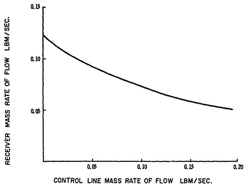
Fig. 14 - Mass Rate of Flow Characteristics, First Stage, 10 psig Supply, Original Configuration
