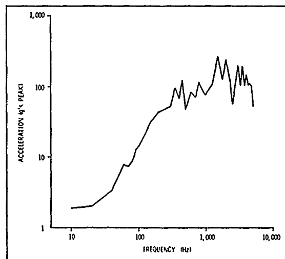
Fig. 5. Typical Undamped Shock Spectrum, (Run 1, Tail Vertical)
