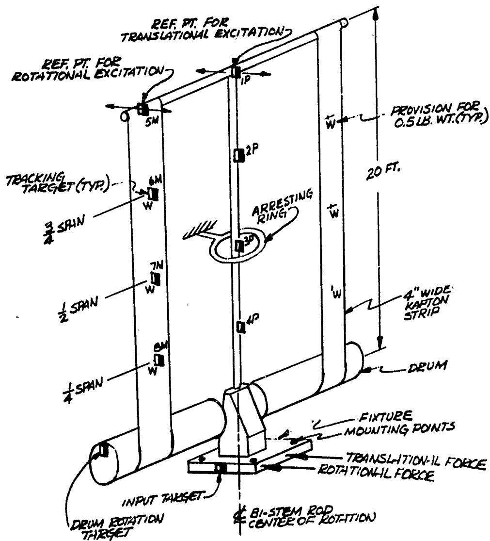
Figure 2. Phase I Test Arrangement
