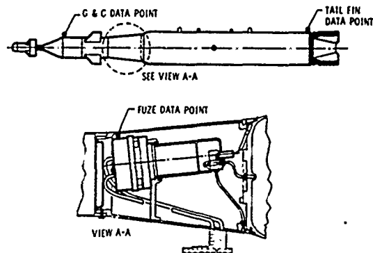
FIG. 3. Accelerometer Locations
