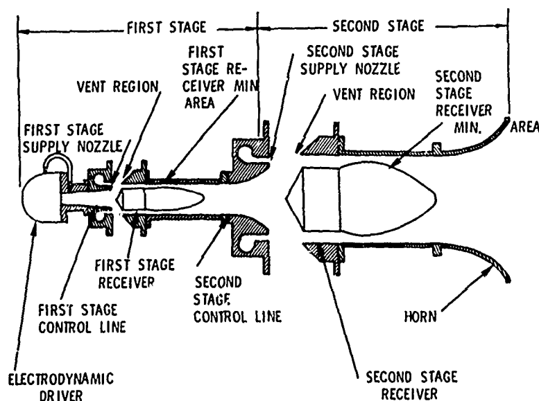
Fig. 7 - Original Configuration of Two Stage Annular Slot Amplifier
