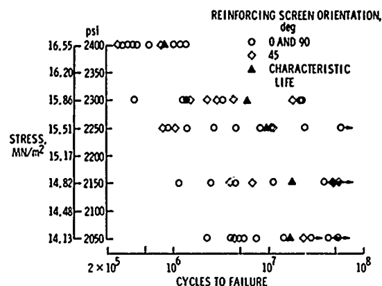
Fig. 9 - Stress-cyclic life data for AISI 347 stainless-steel fiber metal.
