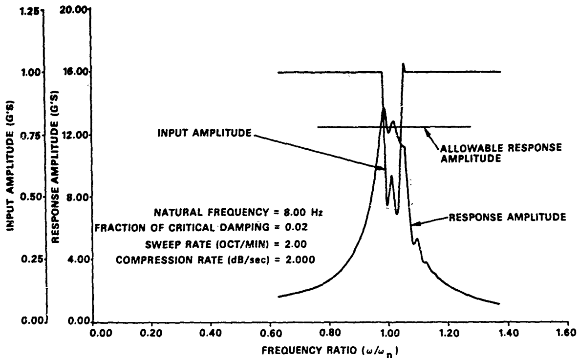
Fig. 3 - Response for swept notched excitation
