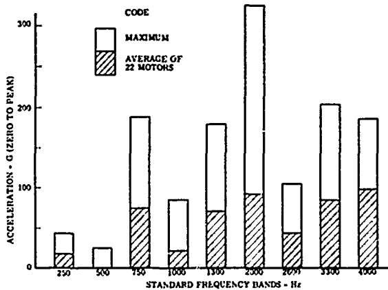
Figure 4 Amplitude of Second Stage Motor Vibration Measured at the Thrust Termination Ports
