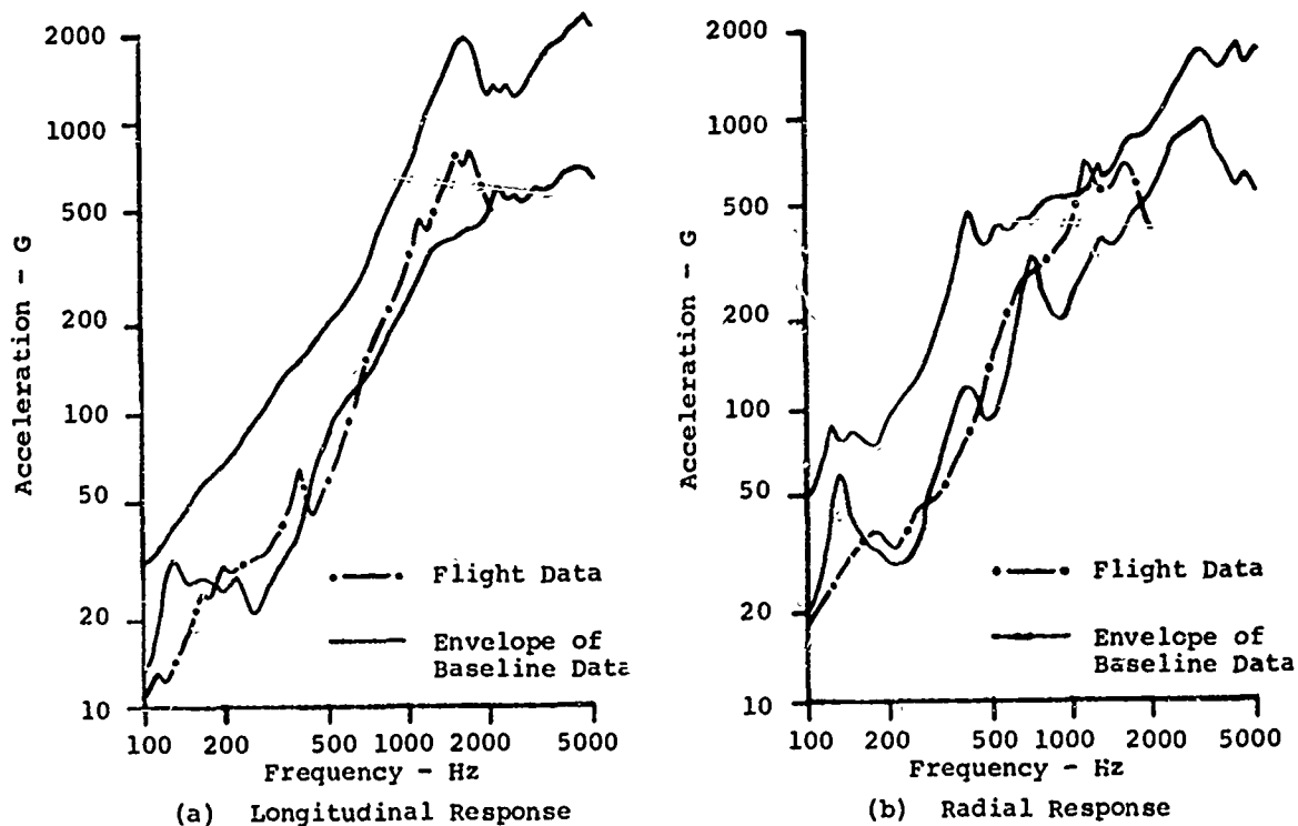
Figure 2 - Comparison of Flight and Test Data at Phase of Attach Fitting
