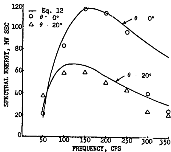
FIG. 9. COMPARISON OF THEORETICAL ENERGY DISTRIBUTION TO EXPERIMENTAL RESULTS
