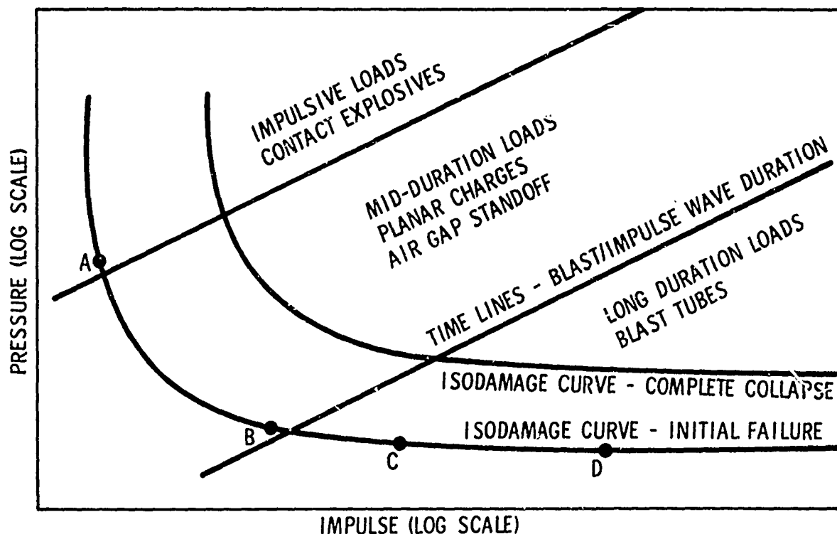
Fig. 1 Isodamage curve
