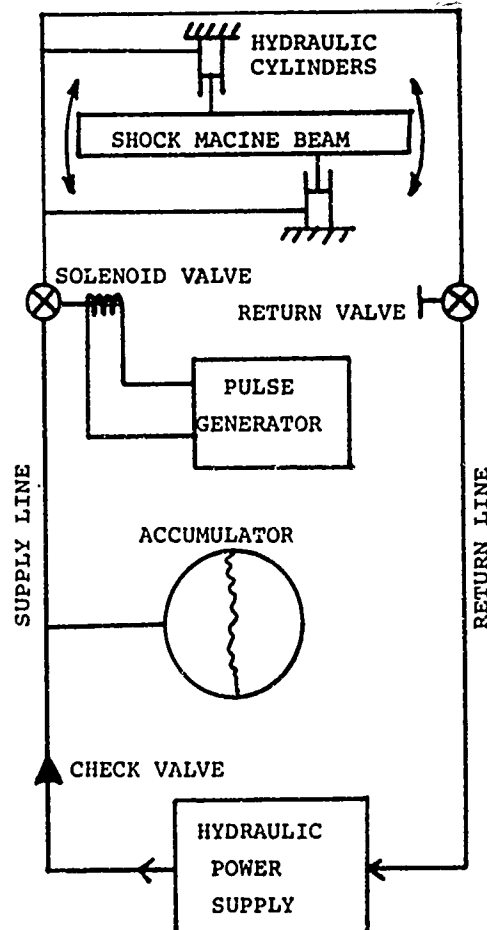
FIGURE 5 HYDRAULIC CIRCUIT
