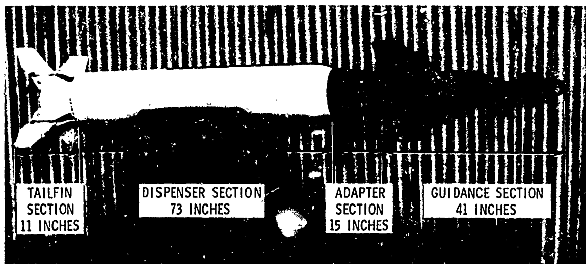
FIG. 1. Guided Rockeye Modular Dispenser Weapon (GRM)
