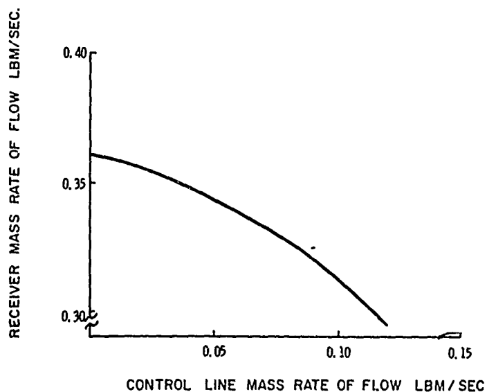
Fig. 16 - Mass Rate of Flow Characteristics, First Stage, 10 psig Supply Minimum Load Configuration
