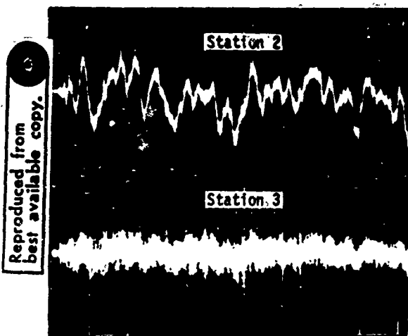
Fig. 7 - Strain gage signals from Stations 2 and 3 for Test No. 1 (sacrificial plate impact). Both sweeps were at 200 microseconds per division and were delayed 240 microseconds from the breakwire trigger. The vertical scales were 240 microstrain per division for Station 2 and 1500 microstrain per division for Station 3.
