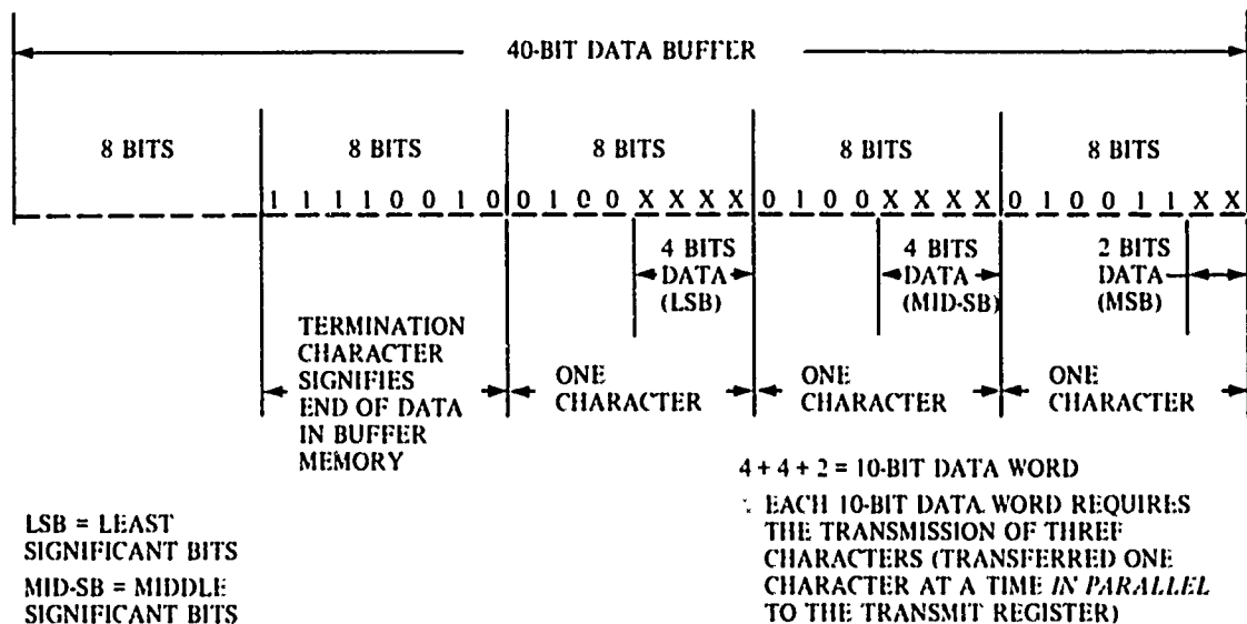
Figure 7a. Forty-Bit Data Buffer.
