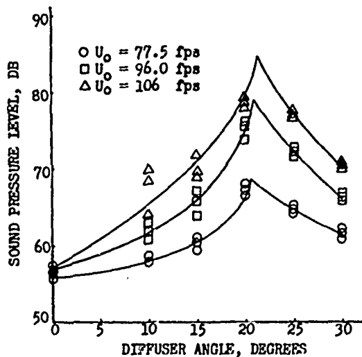
FIG. 3. SOUND PRESSURE LEVEL VERSUS DIFFUSER ANGLE
