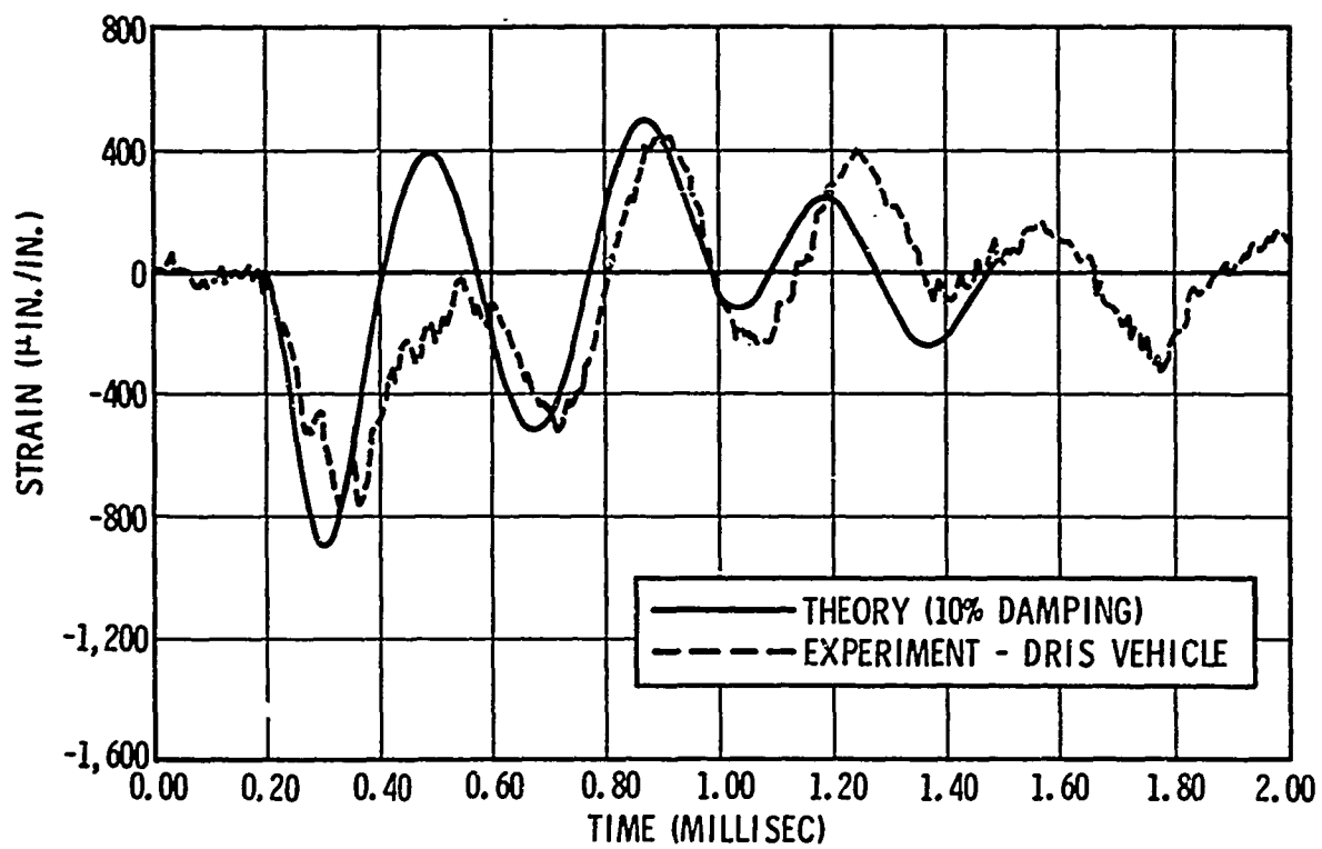
Fig. 14 - Correlation of SABOR3A/DRASTICII with DRIS vehicle test data substructure circumferential strain
