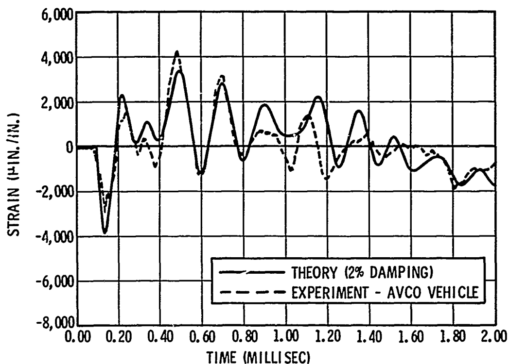
Fig. 16 - Correlation of SABOR3A/DRASTICII with Avco vehicle test data - inner fiber circumferential strain
