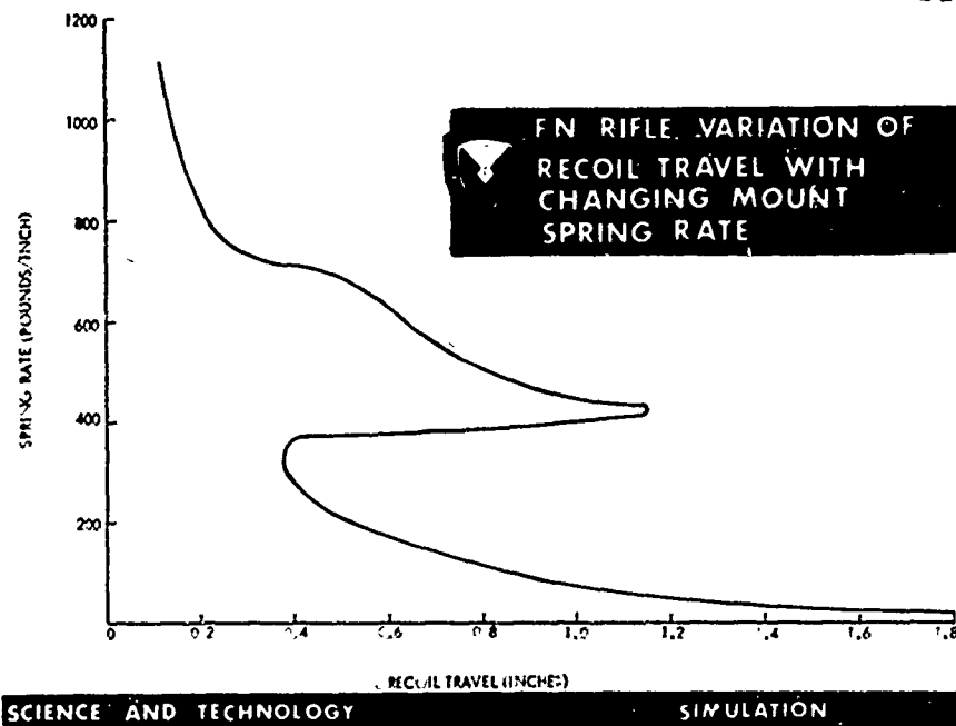
FN Rifle. Variation of Recoil Travel with Changing Mount Spring Rate
