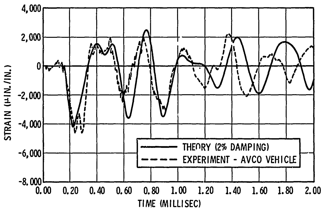
Fig. 15 - Correlation of SABOR3A/DRASTICII with Avco vehicle test data - outer fiber circumferential strain
