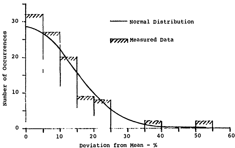
Figure 3 - Comparative Distribution of Measured Data and Normal Distribution
