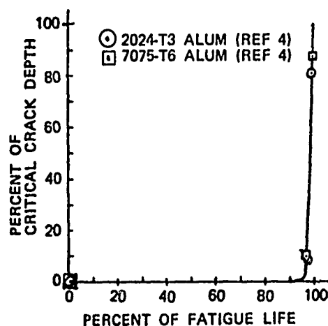
FIGURE 4. FATIGUE CRACK DEPTH GROWTH
