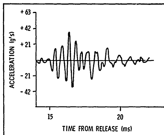
FIG. 4. Typical Acceleration Time History, (Run 1, Tail Vertical)
