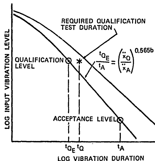
FIGURE 6. ILLUSTRATION OF QUALIFICATION TEST DERIVATION
