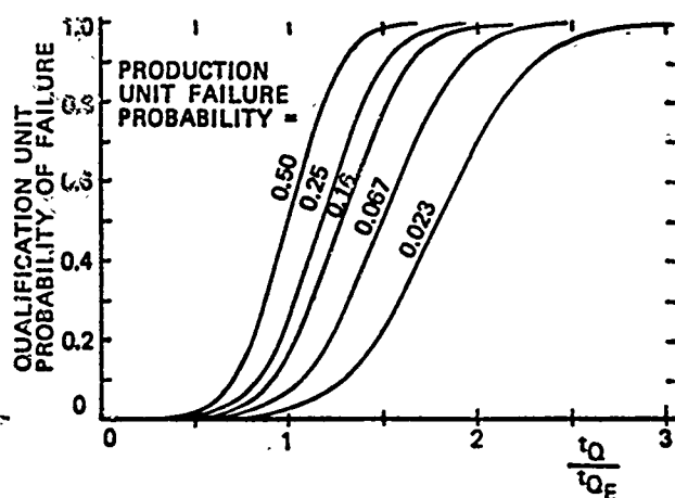
FIGURE 11b. EFFECT OF QUALIFICATION VIBRATION TIME (SCATTER BAND WIDTH = 5)
