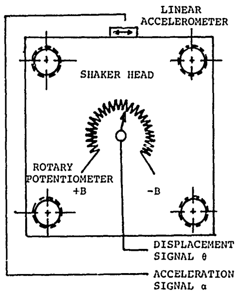
FIGURE 6 FEEDBACK SIGNALS
