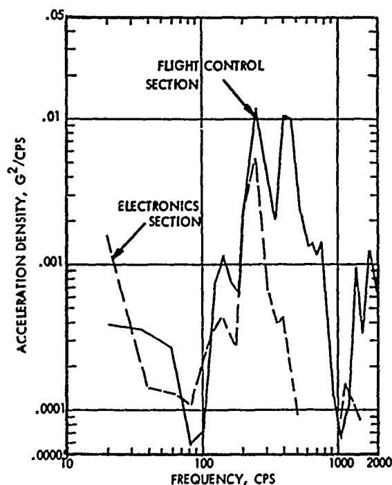
FIGURE 7 MISSILE VIBRATION MEASUREMENTS CAPTIVE FLIGHT B-52 PYLON
