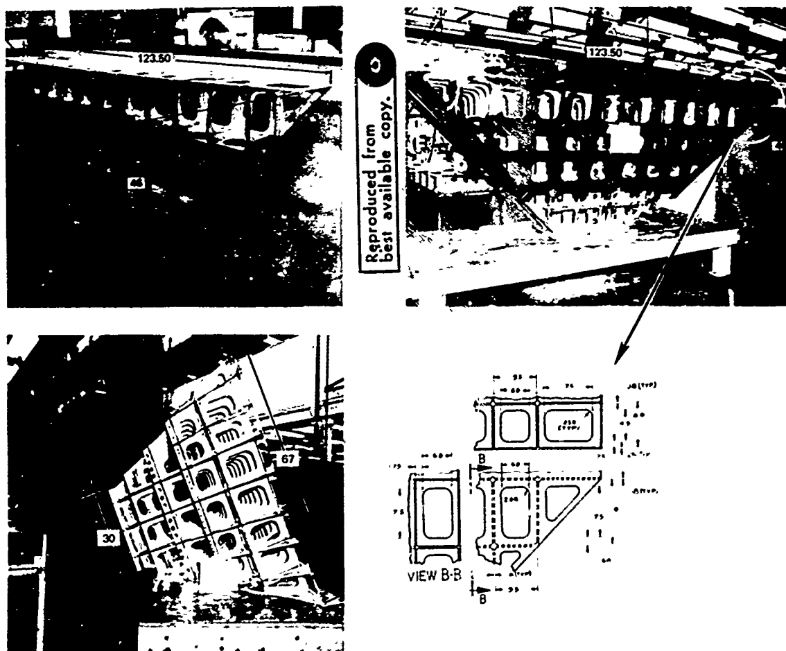
Fig. 3 Cellular fixture in various stages of fabrication
