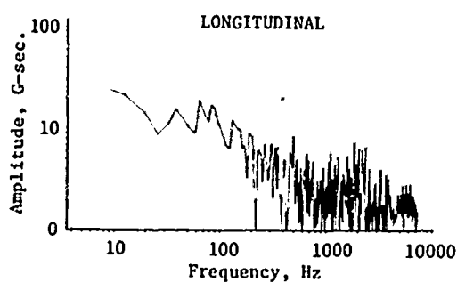
Fig. 14 - Fourier spectra from six accelerometer traces
