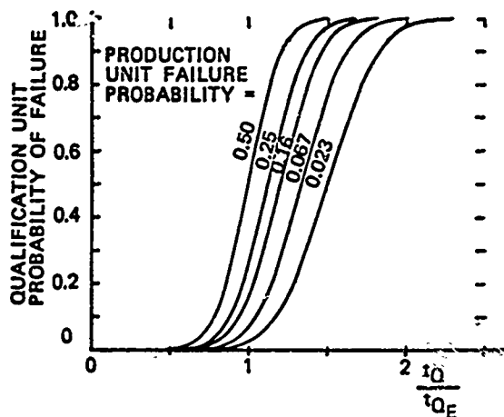
FIGURE 11a. EFFECT OF QUALIFICATION VIBRATION TIME (SCATTER BAND WIDTH = 3)
