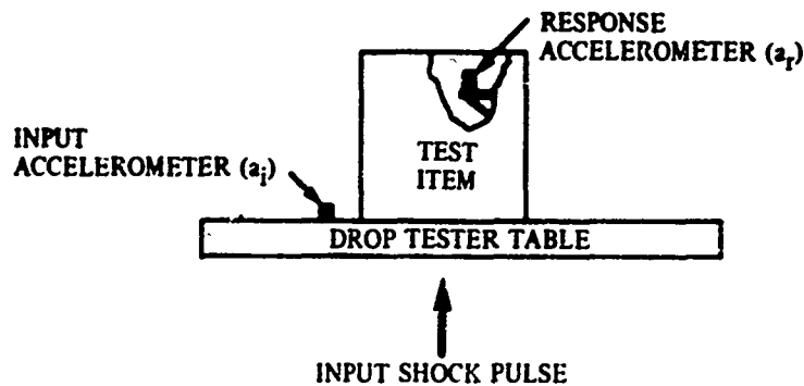
Figure 9a. Accelerometer Placement.
