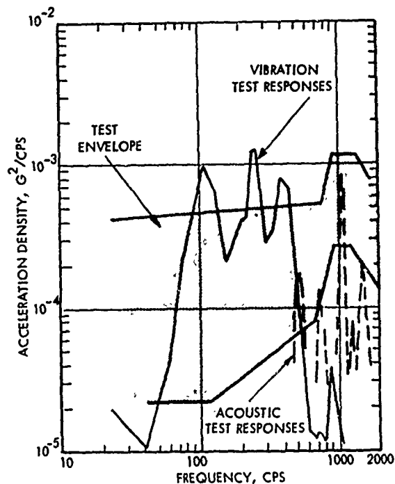
FIGURE 16 COMBINED TEST RESULTS CAPTIVE FLIGHT, WARHEAD AFT MOUNT (VERTICAL)
