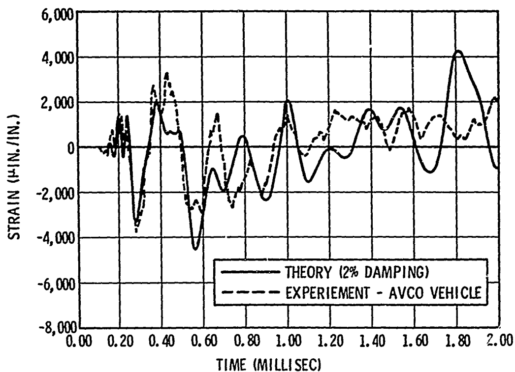
Fig. 18 - Correlation of SABOR3A/DRASTICII with Avco vehicle test data - outer fiber meridional strain
