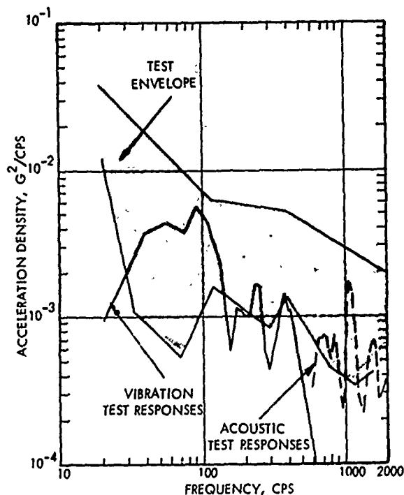
FIGURE 15 COMBINED TEST RESULTS FREE FLIGHT WARHEAD AFT MOUNT (VERTICAL)
