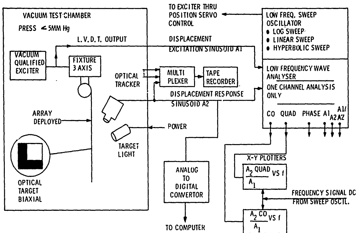
Figure 5. Block Diagram of Equipment Interrelation
