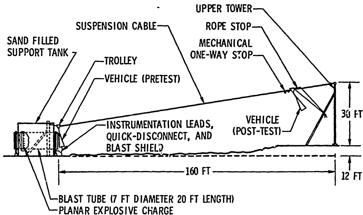
Fig. 7 - Seven foot diameter shock tube and vehicle support and retrieval system
