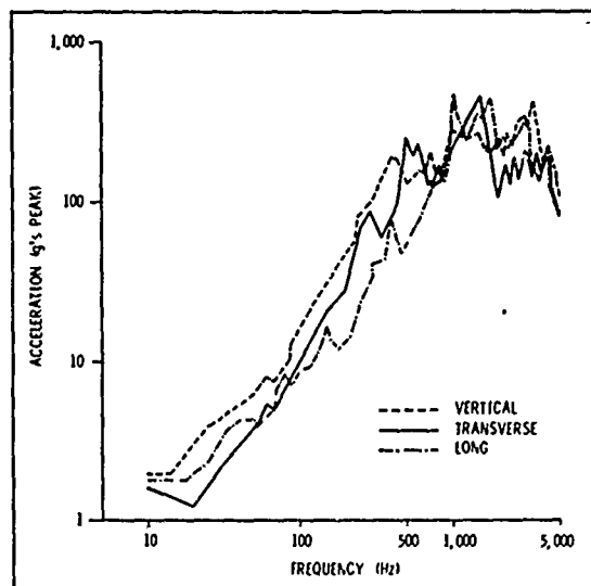
FIG. 8. Maximum Envelope of Tail Shock Spectrum
