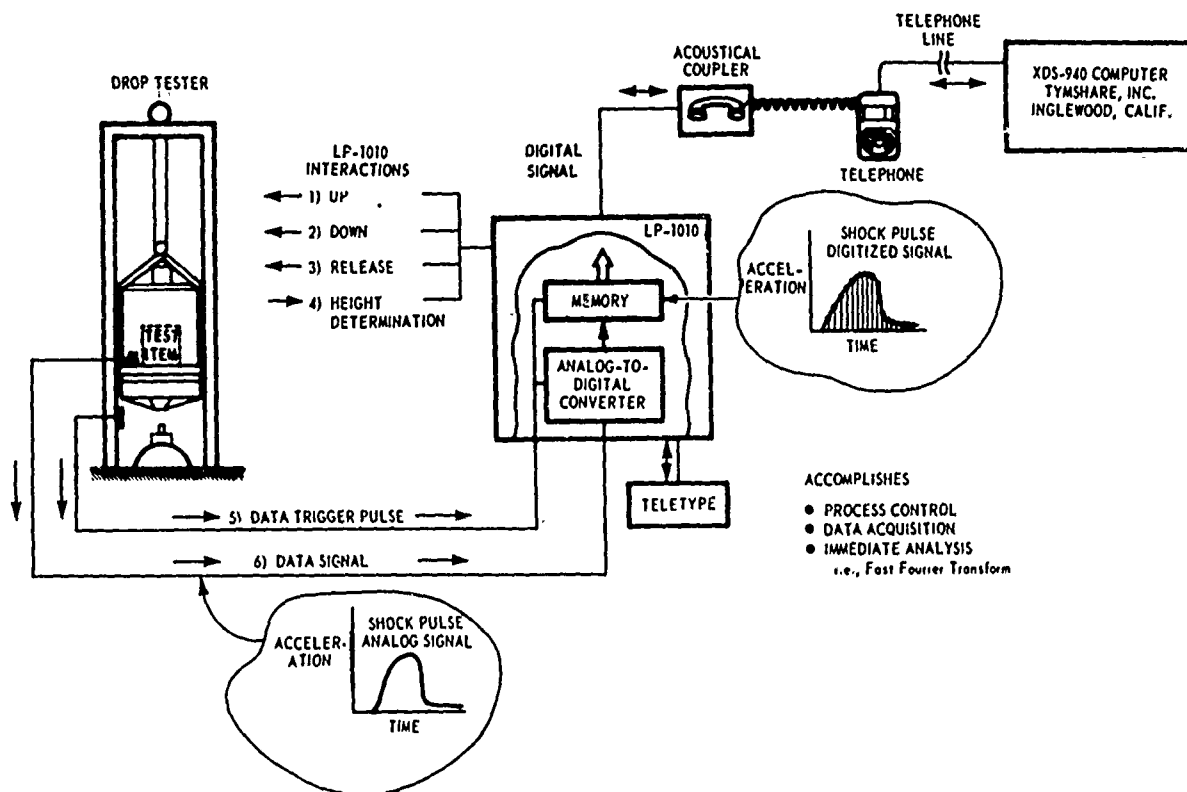
Figure 3. Drop Tester-LP-1010 Setup With Timesharing Digital Computer.
