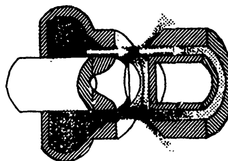
Fig. 6 - Negative Peak of an Input Cycle - Annular Slot Nozzle
