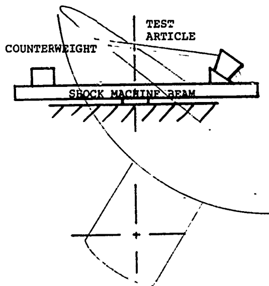
FIGURE 4 ARRANGEMENT OF TEST ARTICLE
