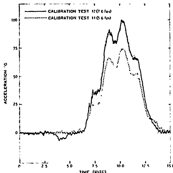
FIGURE 5 6- k_{3B} METALLIC PLATE CONFIGURATION; EFFECT OF CHANGING IMPACT VELOCITY
