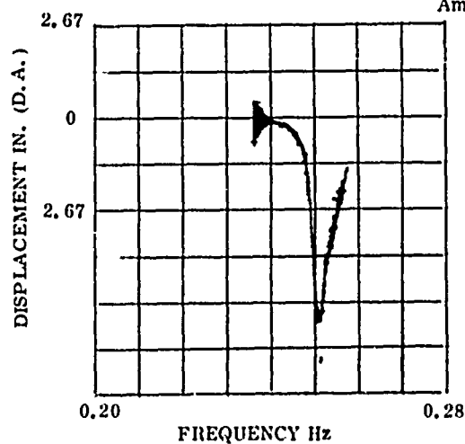
Figure 11. Quadrature Response
