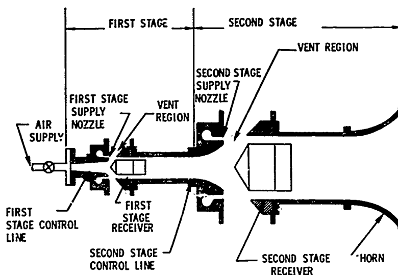
Fig. 10 - Minimum Load Configuration of Two Stage Annular Slot Amplifier
