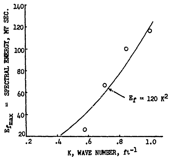
FIG. 11 MAXIMUM VALUE OF THE SPECTRAL ENERGY
