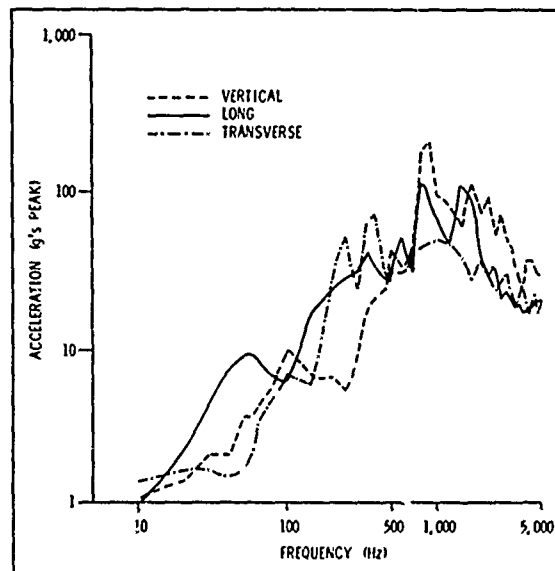
FIG. 10. Maximum Envelope of Guidance Shock Spectrum
