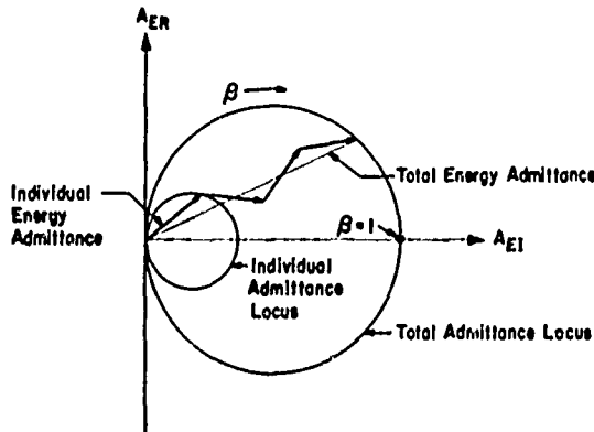
Fig. 1 - Energy admittance in the complex plane
