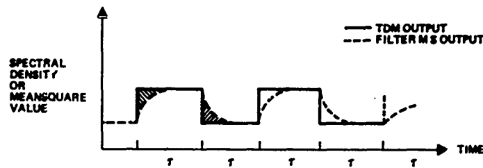
Fig. 14 - Input and response of filter to TDM output
