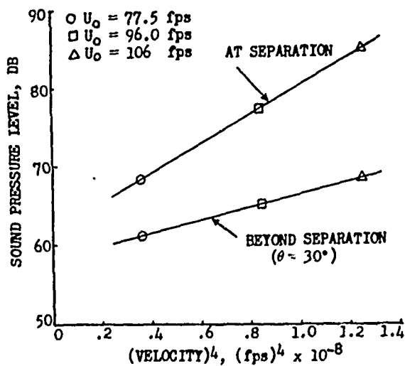
FIG. 4. SOUND PRESSURE LEVEL VERSUS THE FOURTH POWER OF VELOCITY.
