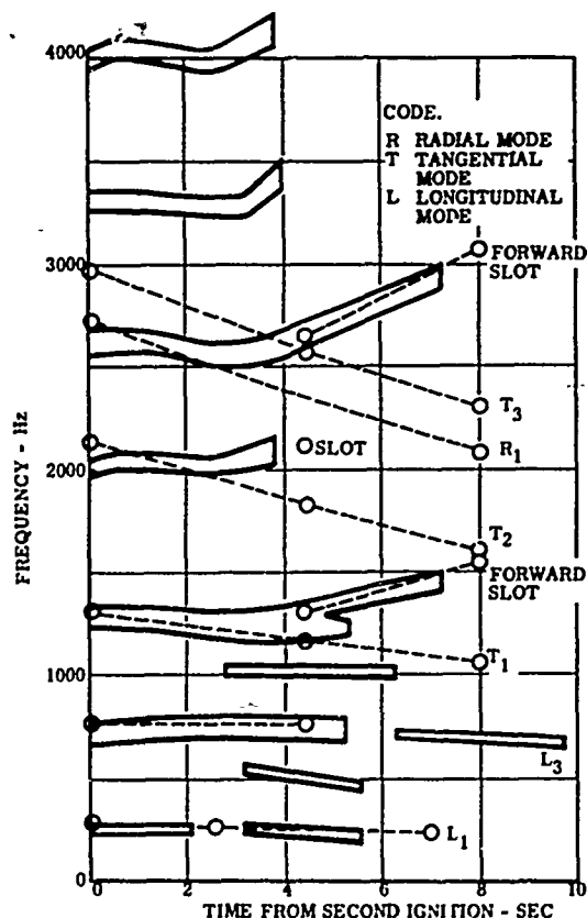
Figure 7 Modal Frequencies Measured During Acoustic Tests Compared with Vibration Data Envelope
