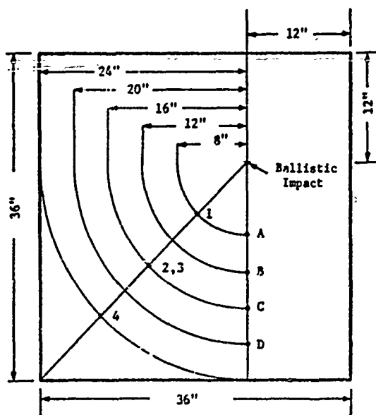
Fig. 2 - Diagram of instrumented test plate showing the point of impact of the bullet and the positions of the accelerometer stations (letters) and the strain gage stations (numbers)
