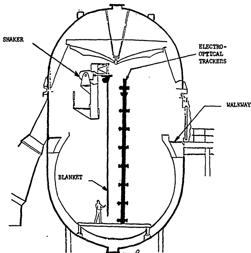
Figure 6. Deployed Modal Test Set Up
