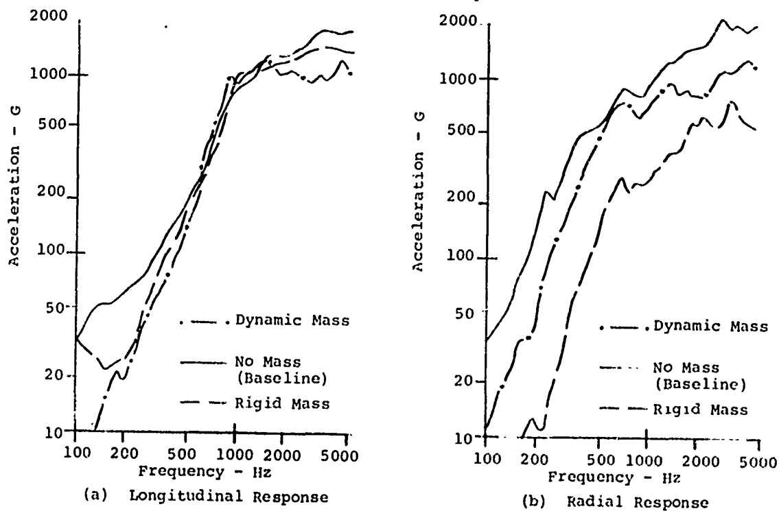
Figure 8 - Effect at Separation Plane of Mass loading
