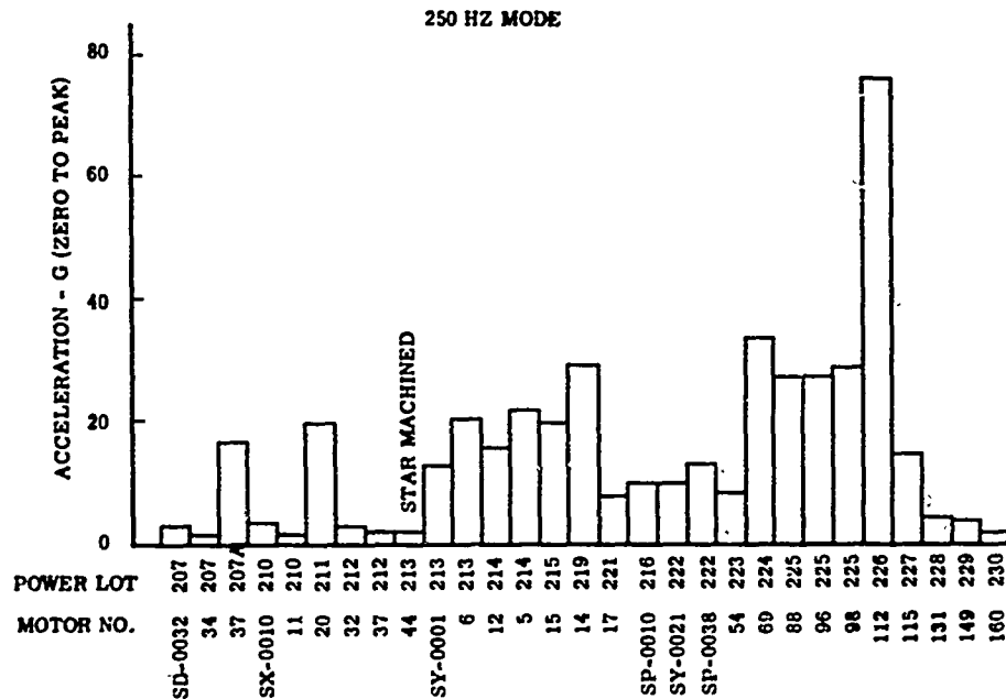
Figure 14 Amplitude of 250 Hertz Mode Measured at the Forward Adapter
