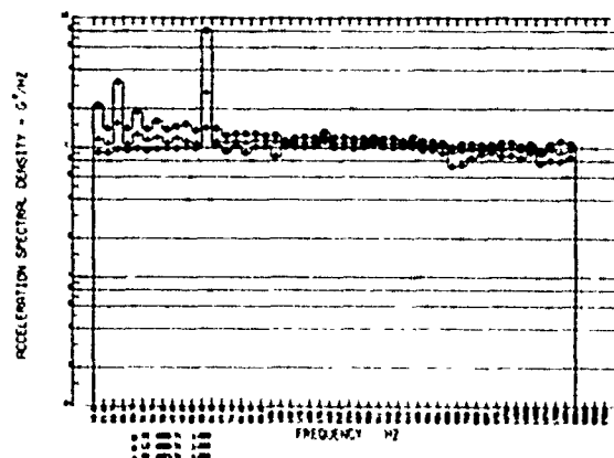
Fig. 18 - Three hardmounted racks - maximum, mean and minimum of TDM/pwr. ave.
