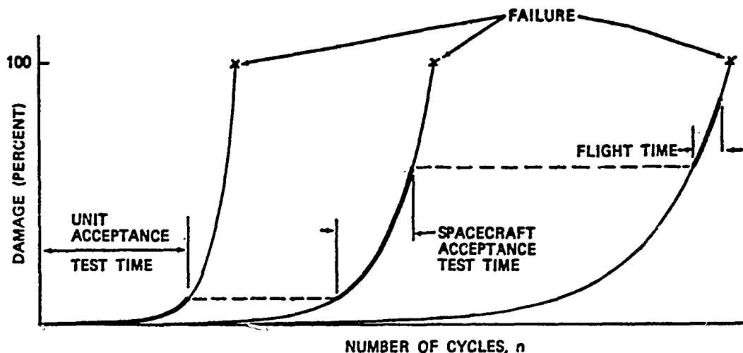
FIGURE 1. FATIGUE DAMAGE ACCUMULATION
