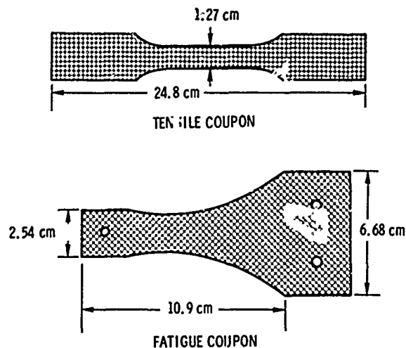
Fig. 3 - Drawings of tensile test and fatigue test models.
