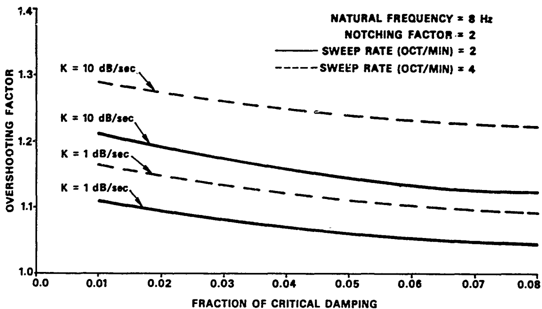
Fig. 5 - Overshooting factor for automatic notch control system
