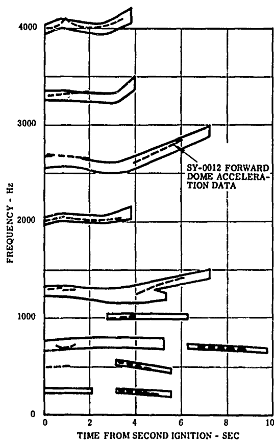
Figure 3 Envelope of Frequencies Measured During Second Stage Motor Vibration and Data From a Typical Static Motor Firing
