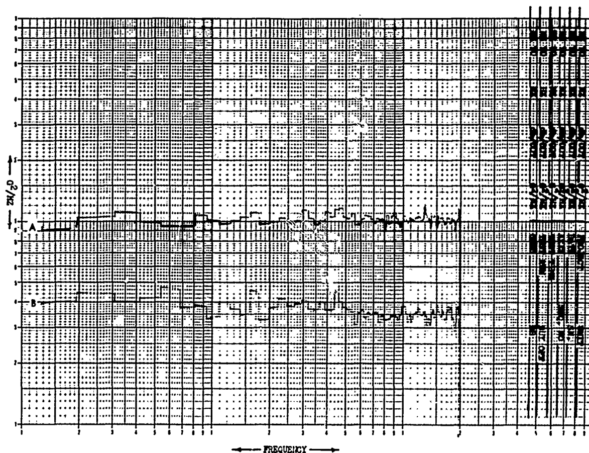
Fig. 11 - Spectral densities from equalization system; A. Equal inputs to two TDM channels B. Zero input to second TDM channel
