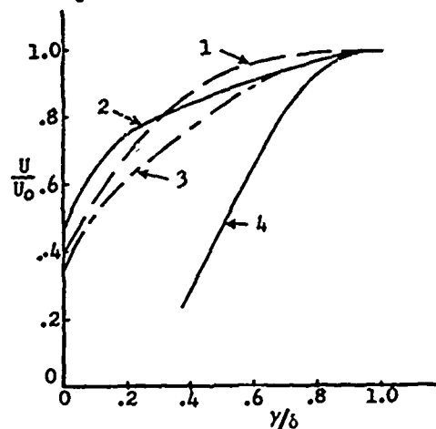
FIG. 2. TYPICAL NONDIMENSIONAL VELOCITY PROFILES
