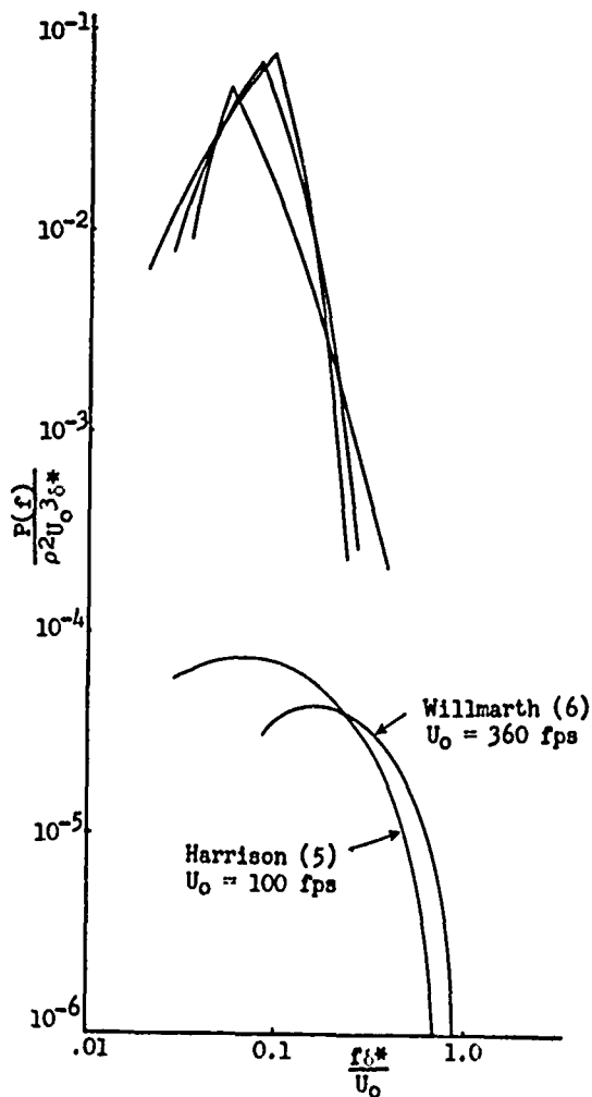
FIG. 6. NONDIMENSIONAL SPECTRAL DENSITY FOR ZERO PRESSURE GRADIENT
