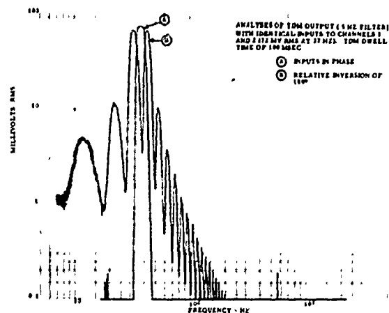
Fig. 2 - Spectral spreading of 37 Hz sinusoid with 100 msec gating time
