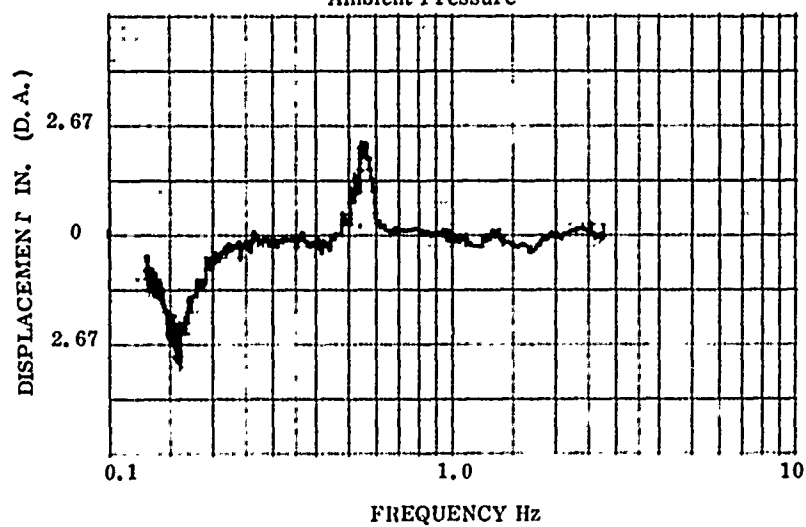
Figure 10. Quadrature Response - Translational Excitation Ambient Pressure
