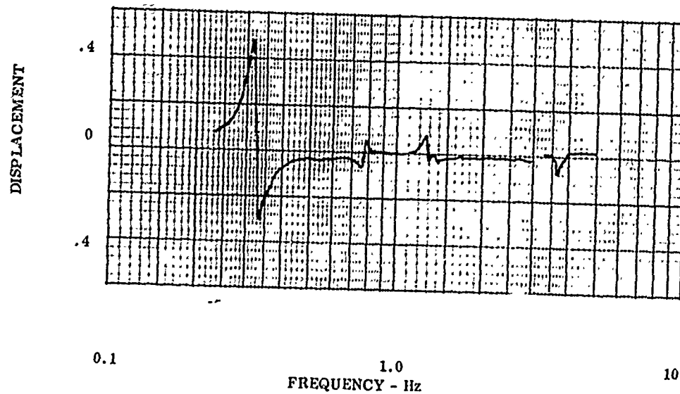
Figure 3. In-Phase Response - Translational Excitation
