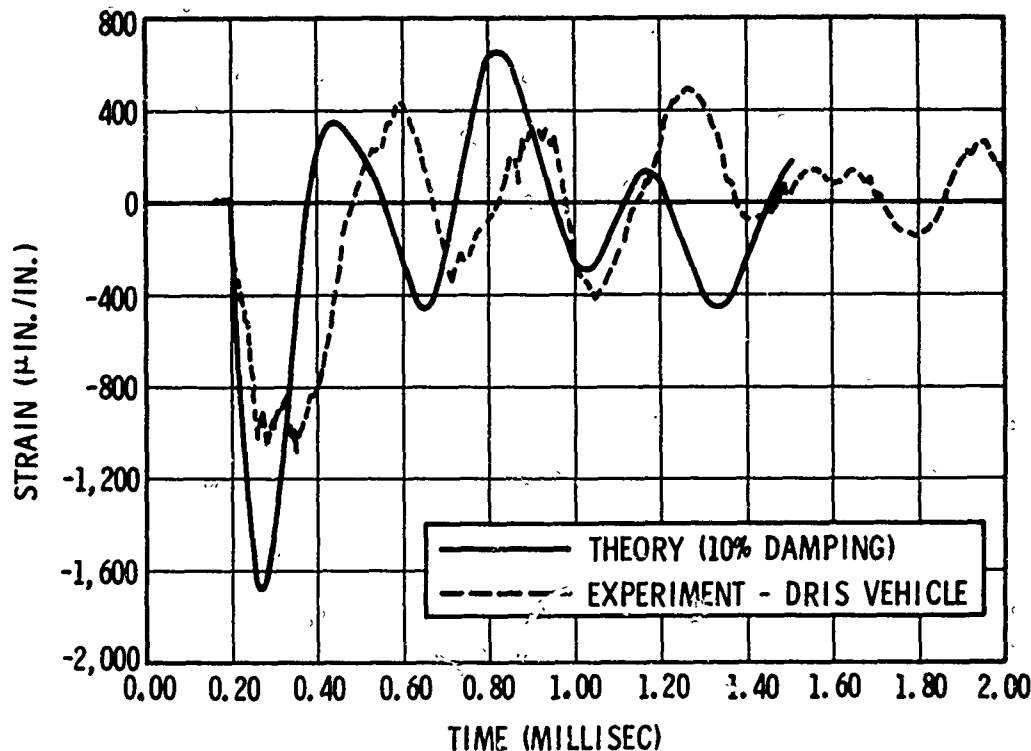
Fig. 20 - Correlation of SABOR3A/DRASTICII with DRIS vehicle test data - substructure circumferential strain
