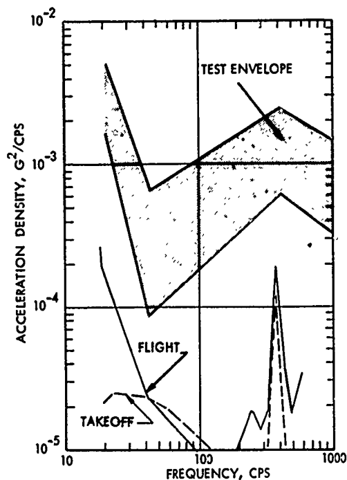
FIGURE 11 DERIVED TEST ENVELOPES ELECTRONICS SECTION CASTING(FORE/AFT)
