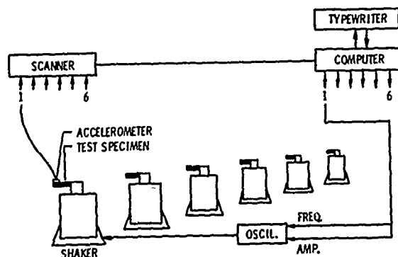
Fig. 6 - Schematic diagram of the computer control for fatigue testing of acoustic materials.
