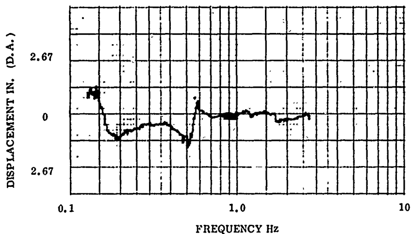
Figure 9. In-Phase Response - Translational Excitation Ambient Pressure
