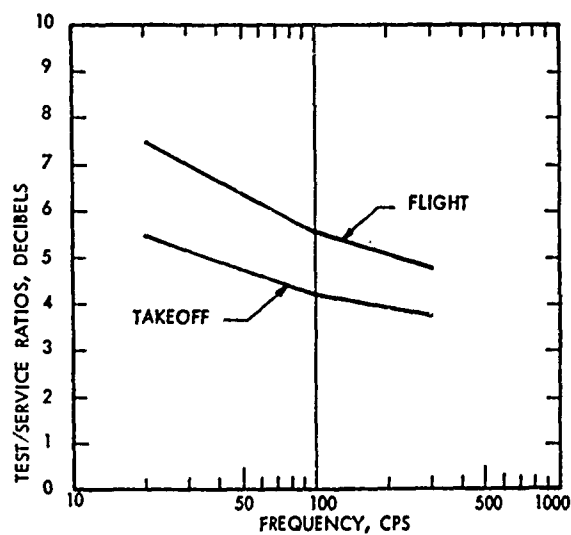
FIGURE 9 CORRECTION FACTORS FOR CAPTIVE FLIGHT MEASUREMENTS
