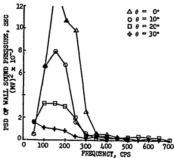
FIG. 5. POWER SPECTRAL DENSITY VERSUS FREQUENCY
