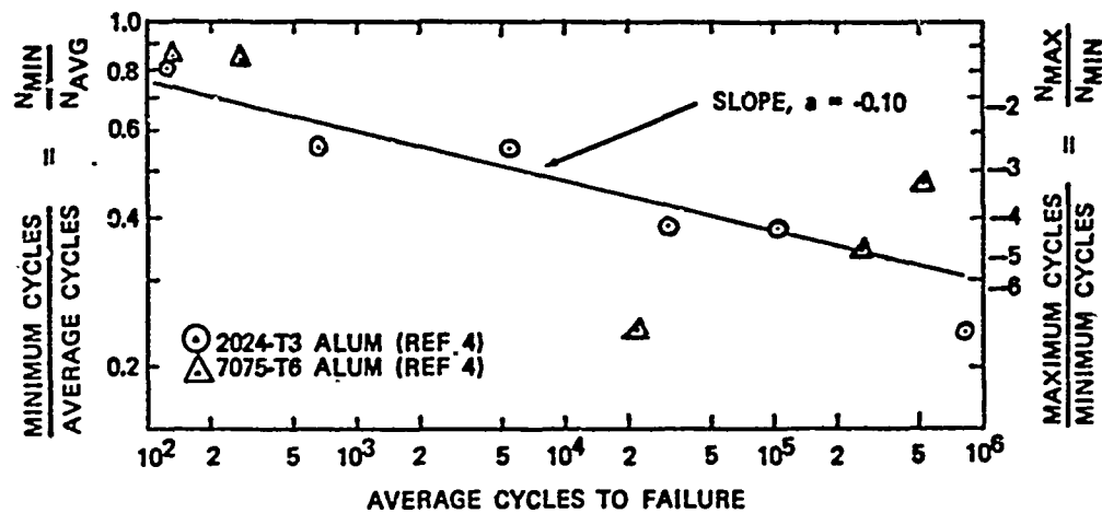
FIGURE 2b. VARIATION IN SCATTER BAND WIDTH
