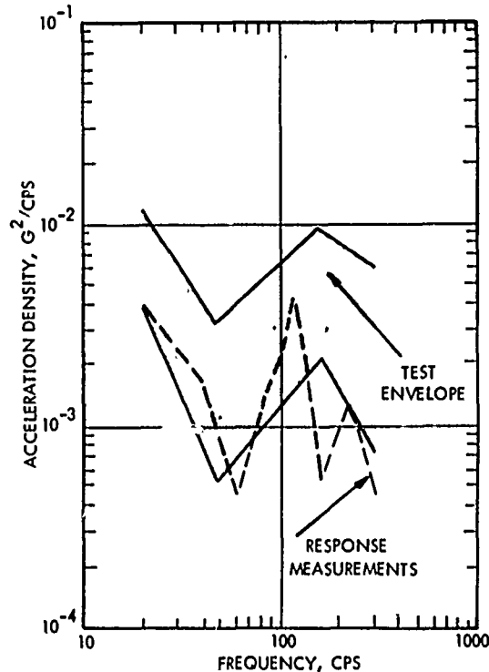
FIGURE 14 TEST RESULTS WARHEAD AFT MOUNT (LATERAL)
