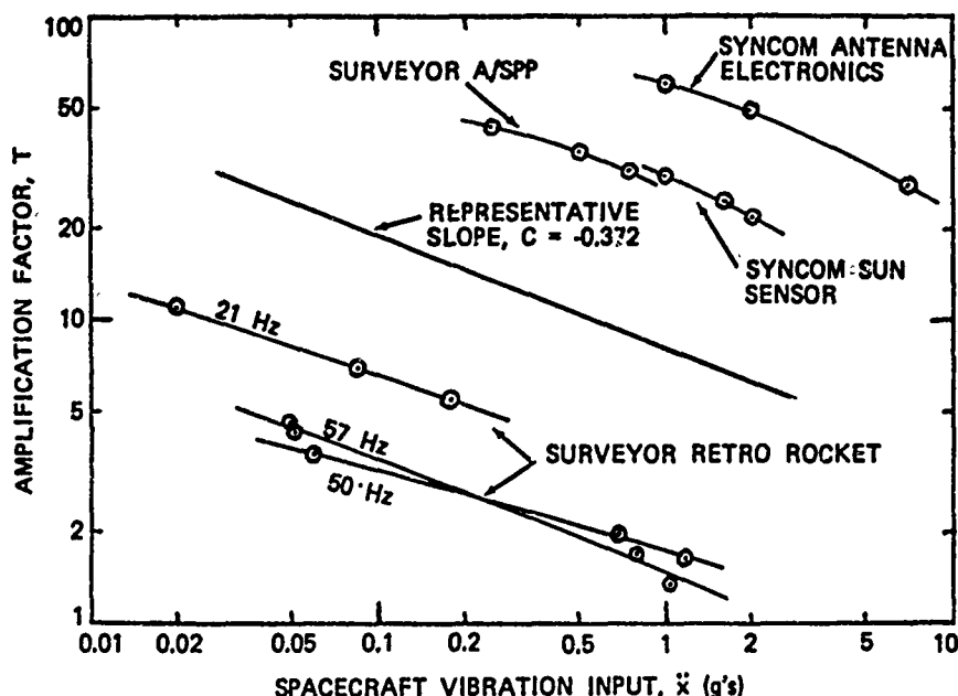
FIGURE 5. EFFECT OF STRUCTURAL DAMPING VARIATION
