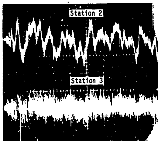
Fig. 8 - Strain gage signals from Stations 2 and 3 for Test No. 2 (direct impact). Sweep rates, delays and vertical scales remained the same as for Figure 7.
