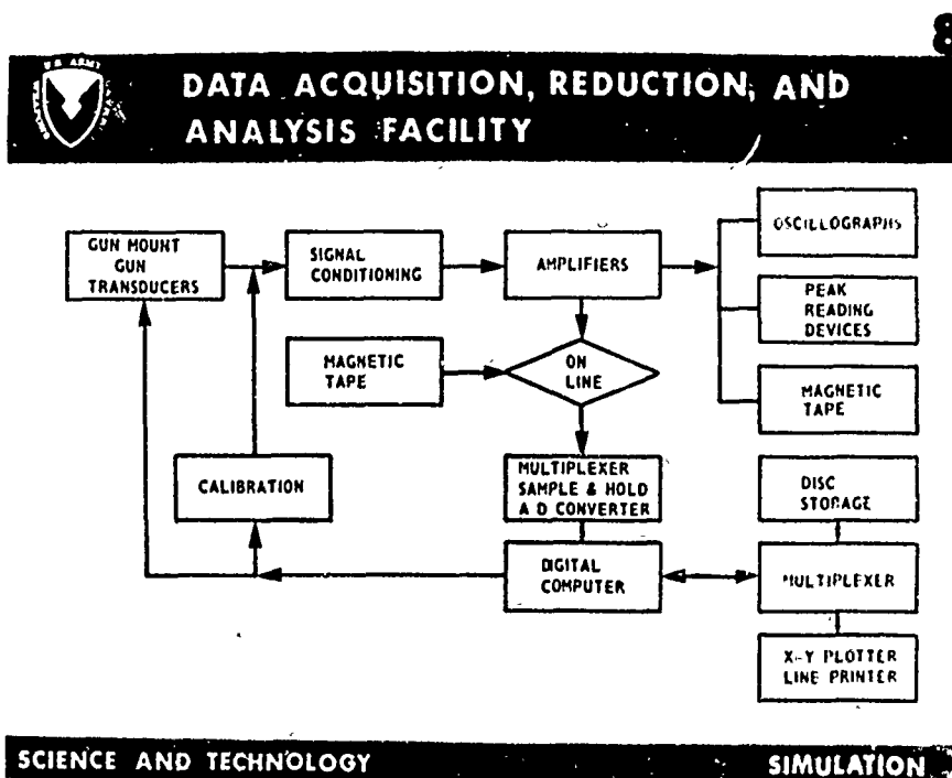
Data Acquisition, Reduction and Analysis Facility
