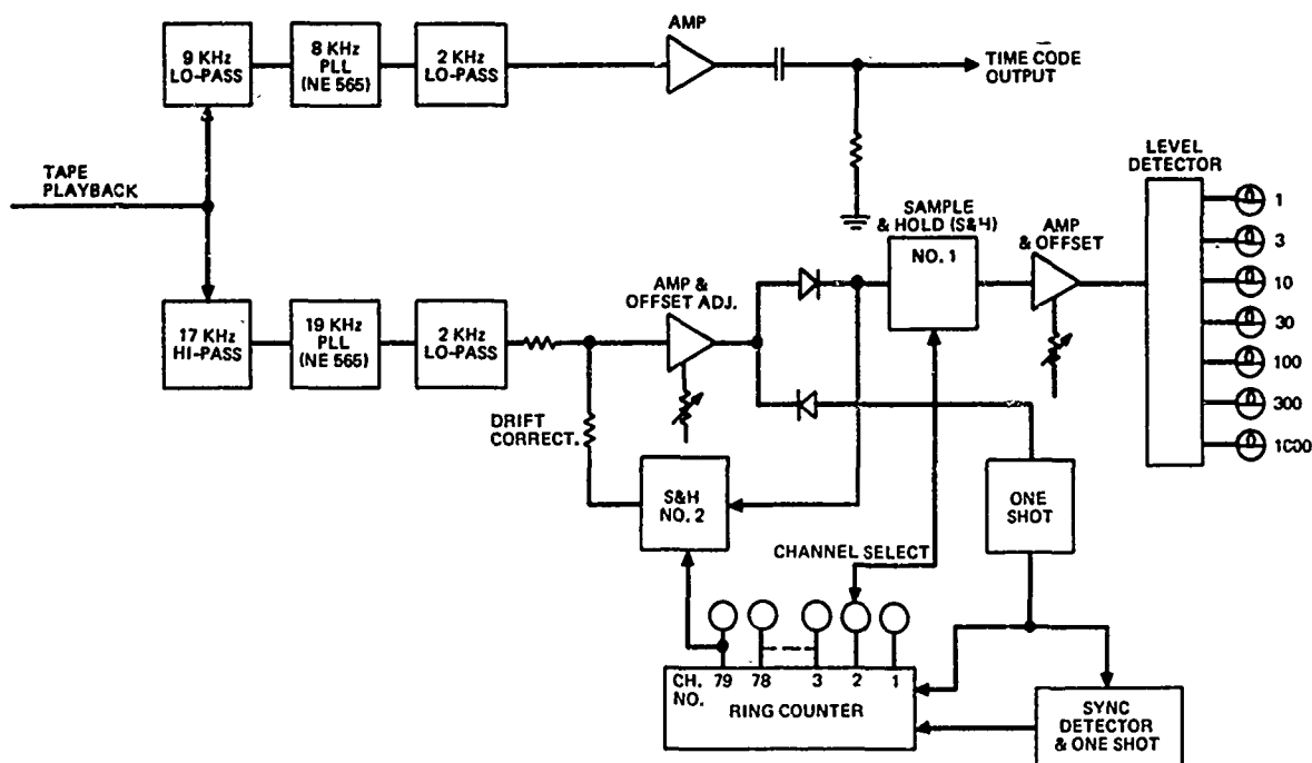
Figure 2 - Decoder Block Diagram
