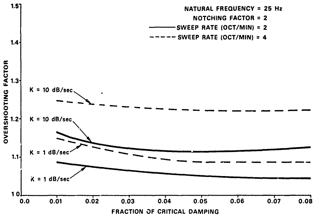
Fig. 6 - Overshooting factor for automatic notch control system
