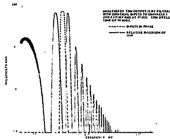
Fig. 1 - Spectral spreading of 37 Hz sinusoid with 50 msec gating time
