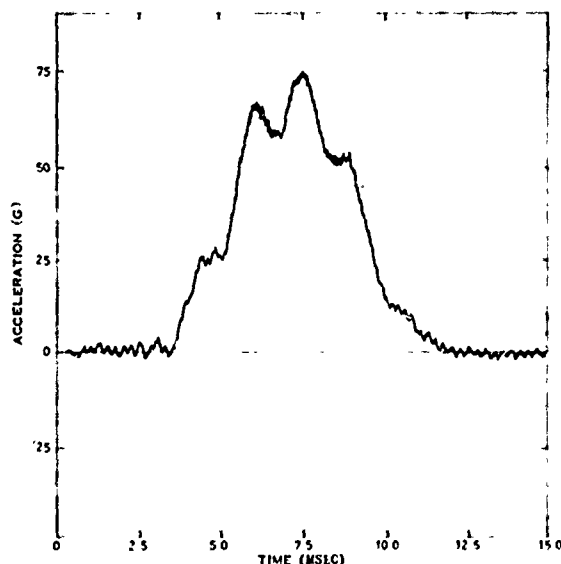
FIGURE 4 6- k_{3B} METALLIC PLATES CALIBRATION TEST 11
