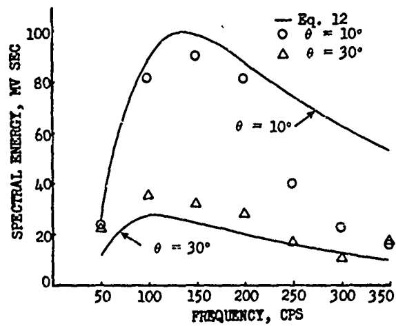
FIG. 10 COMPARISON OF THEORETICAL ENERGY DISTRIBUTION TO EXPERIMENTAL RESULTS
