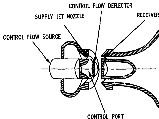
Fig. 4 - Annular Slot Jet Amplifier
