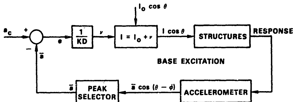
Fig. 1 - Notch control system block diagram
