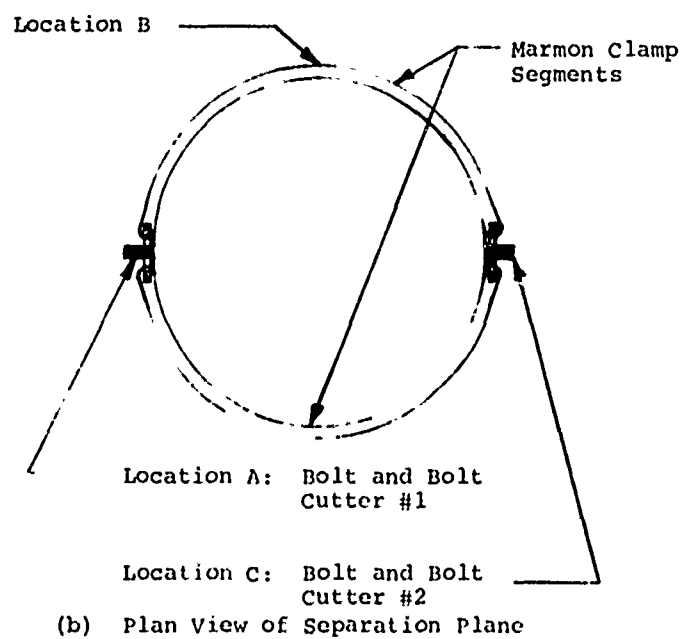
Figure - Structural Schematic of Test Hardware
