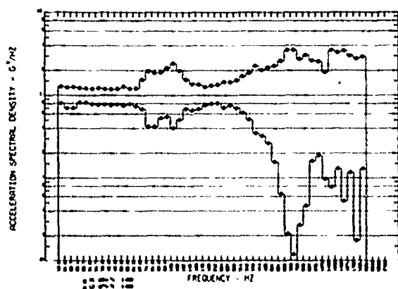
Fig. 17 - Three hardmounted racks - maximum and minimum C_1 /pwr. ave.
