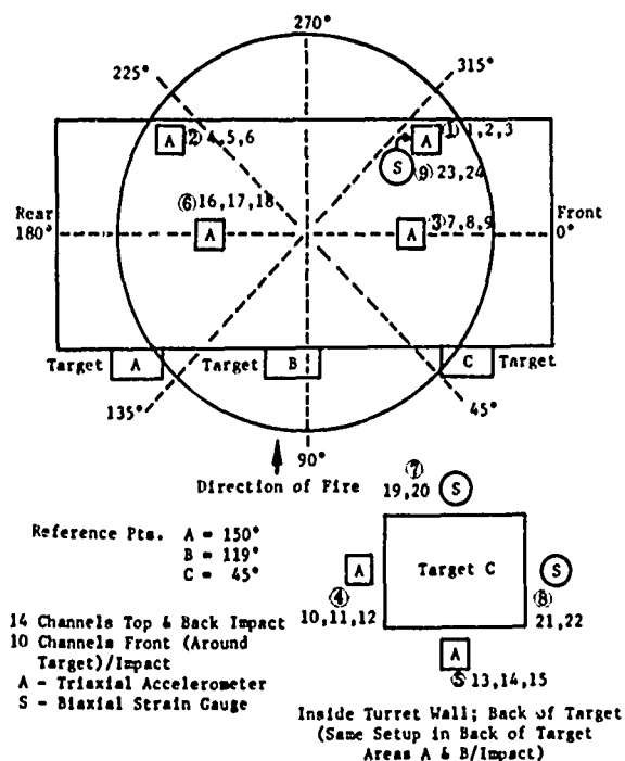
Fig. 10 - M60A1E1 turret schematic showing position of instrumentation relative to the sacrificial plates
