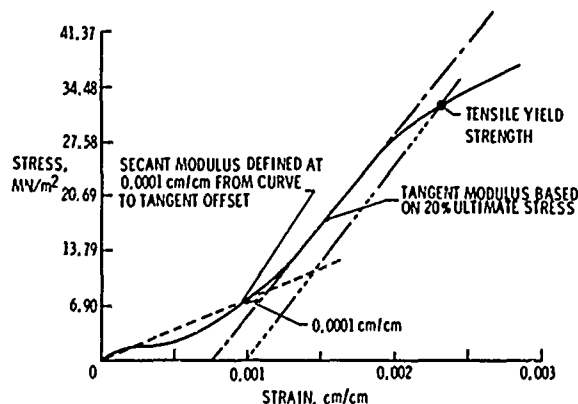
Fig. 4 - Typical stress-strain curve for AISI 347 stainless-steel fiber metal.
