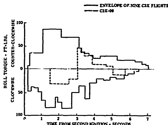
Figure 13 Roll Torque Measured During Poseidon Missile Flights
