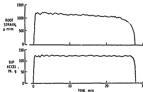
Fig. 5 - Samples of time averaged values of the peak acceleration and strain response time histories for a fiber-metal beam fatigue test.
