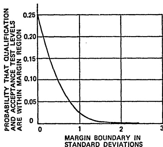
FIGURE 8. PROBABILITY OF VIOLATING QUALIFICATION TO ACCEPTANCE TEST MARGIN
