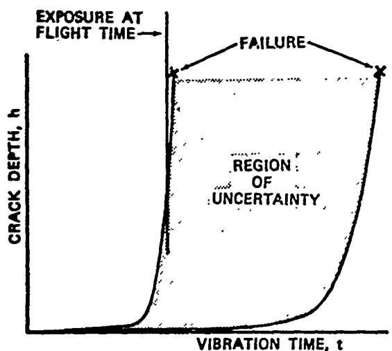
FIGURE 15. RISK OF FLYING PROTOTYPE UNITS
