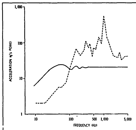
FIG. 6. Undamped Shock Spectrum Comparisons, MIL-STD-810, Operational Shock Response (—) and Maximum Envelope of Fuze Response From Fin Opening (-----)
