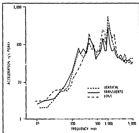
FIG. 9. Maximum Envelope of Fuze Shock Spectrum
