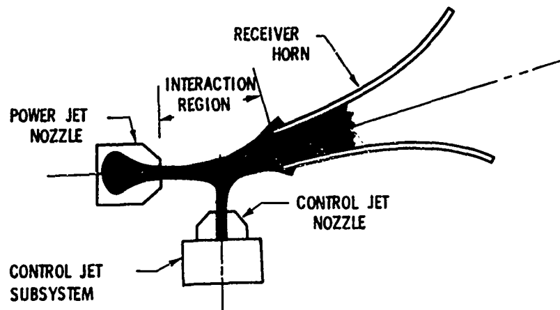
Fig. 3 - Negative Peak of an Input Cycle - Rectangular Nozzle
