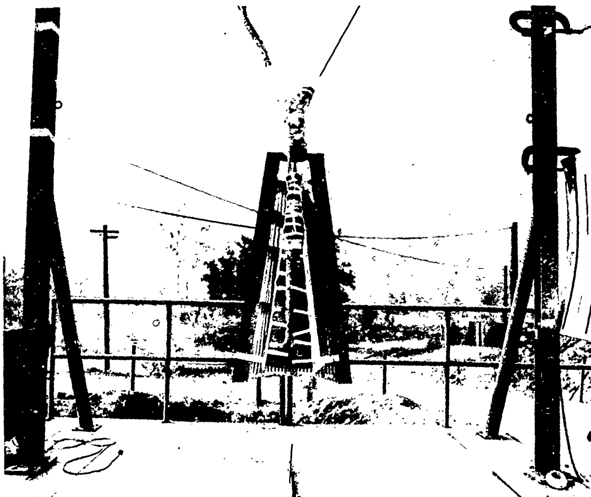
Fig. 3 - Air gap standoff loading technique
