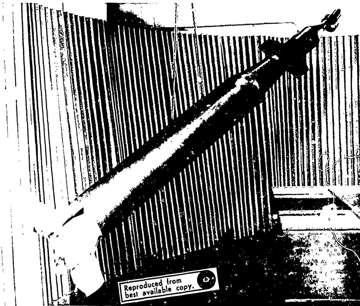
FIG. 2. GRM Suspended for Laboratory Test
