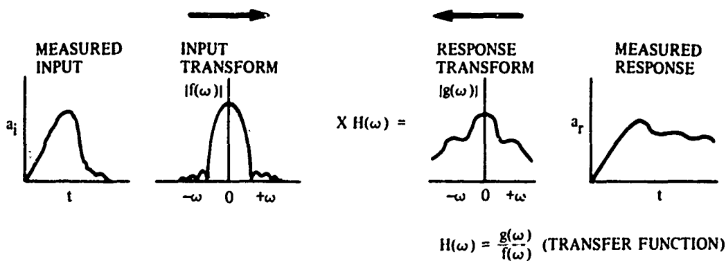
Figure 9b. Determination of the Transfer Function From Two Simultaneous Measurements.
