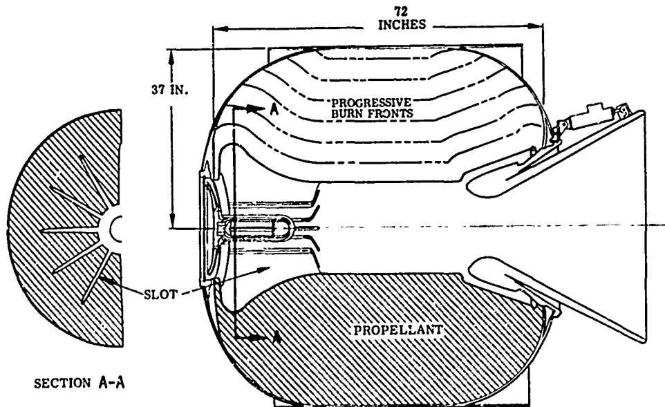
Figure 6 Cross Section of Poseidon Second Stage Motor
