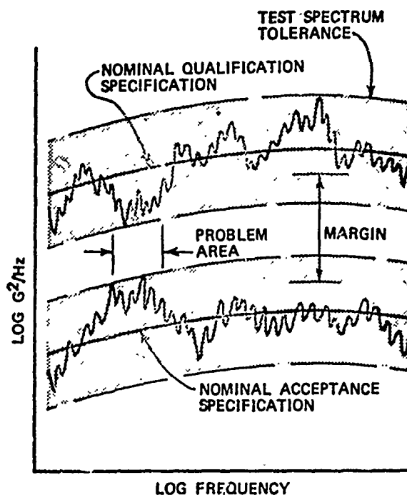
FIGURE 7. DEFINITION OF QUALIFICATION TO ACCEPTANCE TEST LEVEL MARGIN
