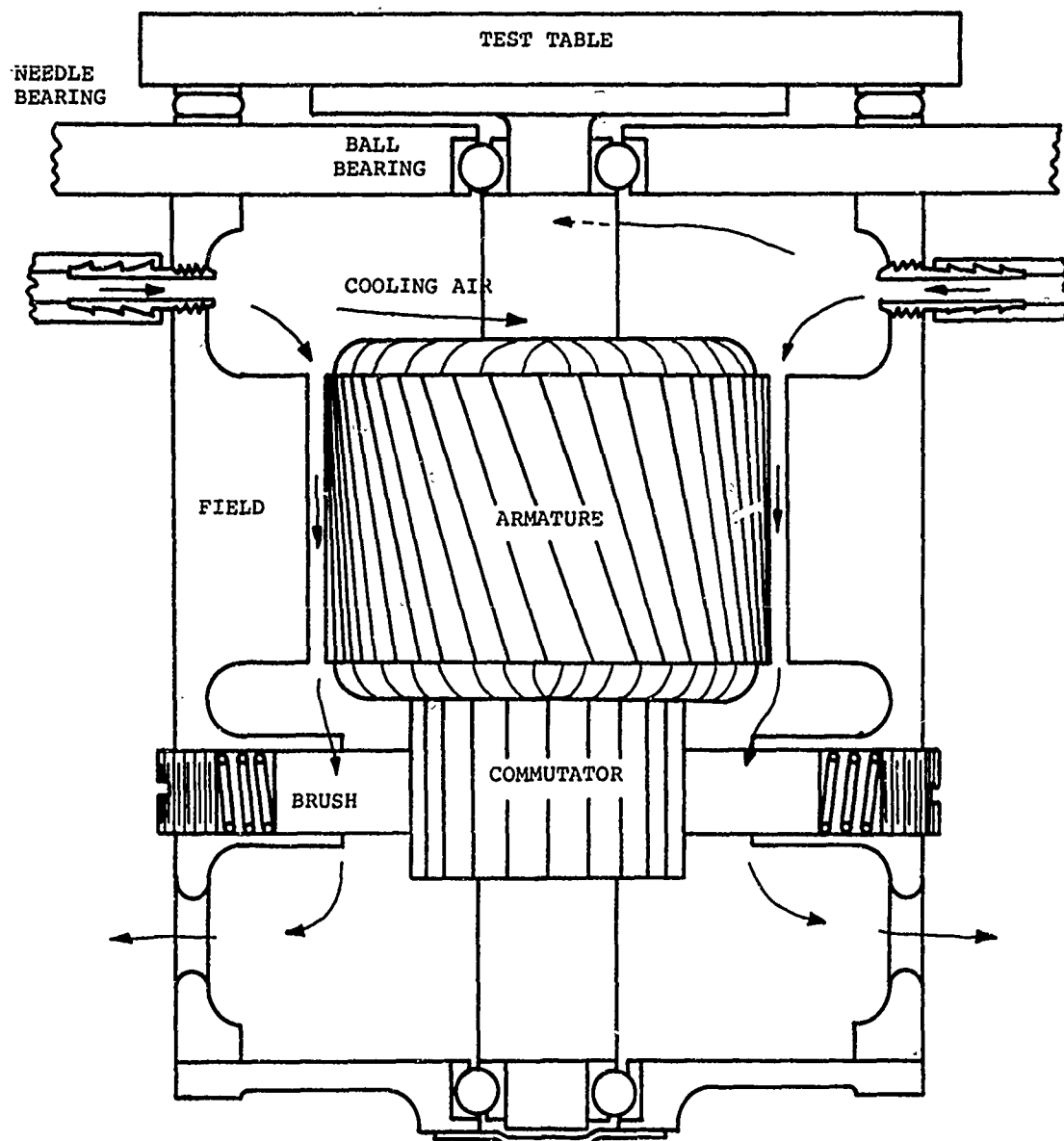
FIGURE 8 ROTATIONAL SHAKER CONSTRUCTION
