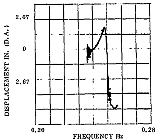
Figure 12. Quadrature Response
