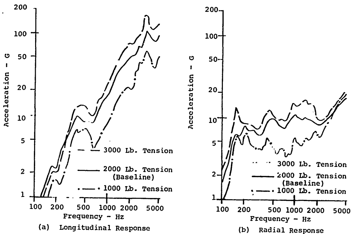
Figure 7 - Effect in spacecraft of Marmion Clamp Tension
