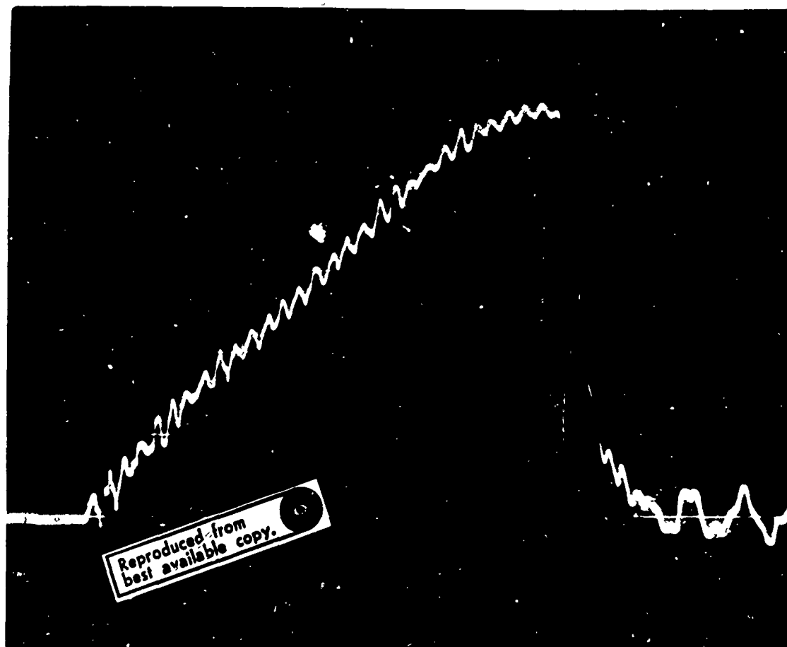
Figure 2. Acceleration Versus Time History of a Shock Input to a Test Item. Photograph is of memory oscilloscope trace.
