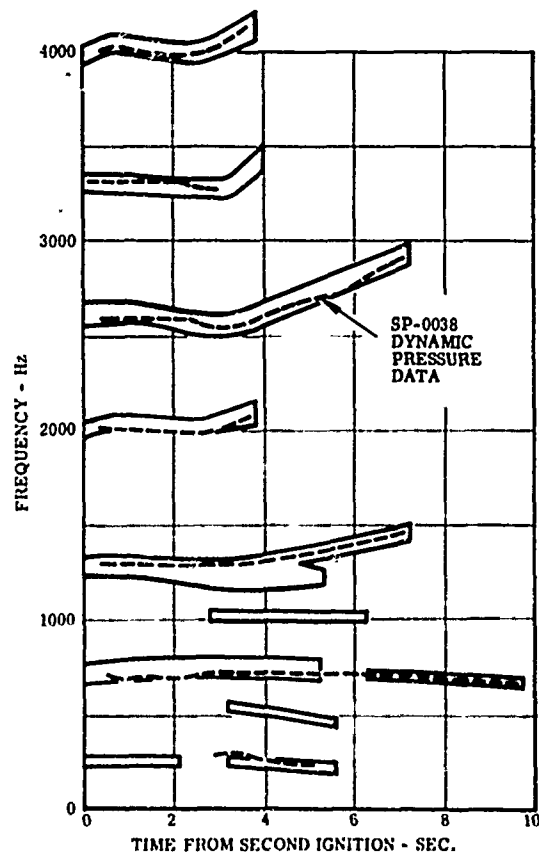
Figure 8 Frequency Profile of Dynamic Pressure Data Compared with Vibration Data Envelope
