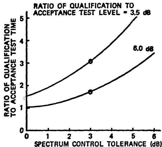
FIGURE 14. EFFECT OF TEST TOLERANCE ON REQUIRED QUALIFICATION TIME
