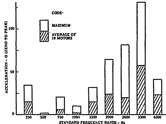
Figure 5 Amplitude of Second Stage Motor Vibration Measured at the Forward Adapter
