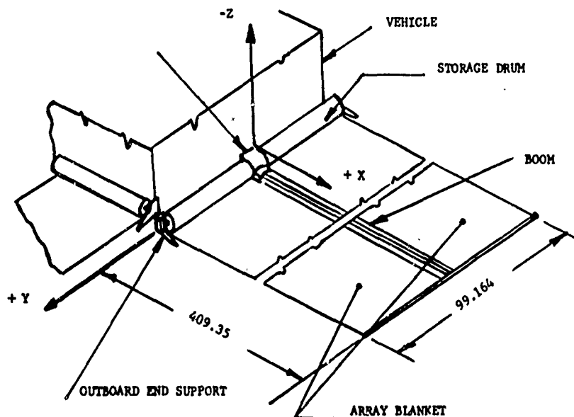
Figure 1. Roll-Up Solar Array Configuration (Coordinate System Shown)
