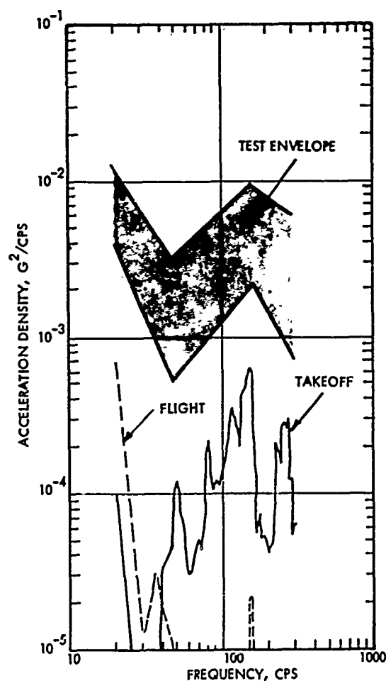
FIGURE 10 DERIVED TEST ENVELOPES WARHEAD AFT MOUNT (LATERAL)
