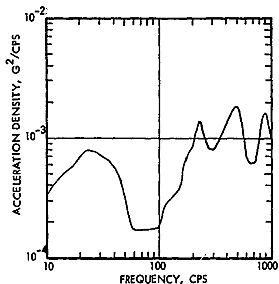
FIGURE 6 ROCKET MOTOR VIBRATION MEASUREMENTS CAPTIVE FLIGHT FB-111 BAY
