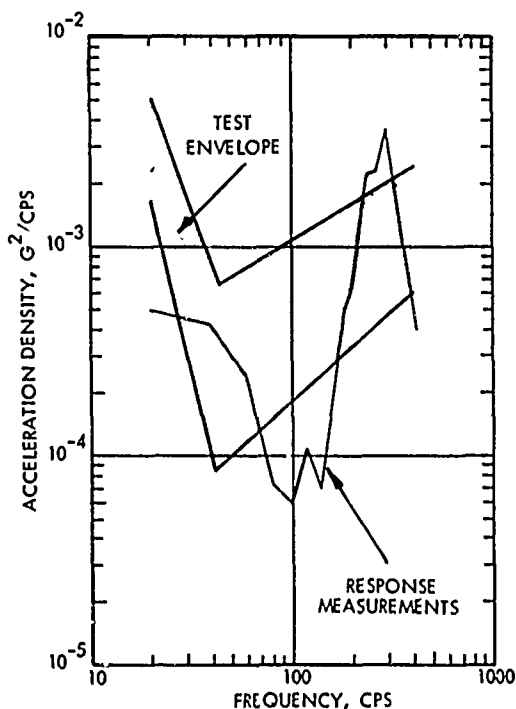
FIGURE 13 TEST RESULTS ELECTRONICS SECTION CASTING (FORE/AFT)
