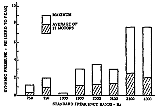
Figure 9 Amplitude of Chamber Pressure Oscillations Measured During Static Tests
