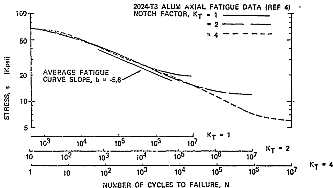
FIGURE 3. FATIGUE CURVE CHARACTERISTICS
