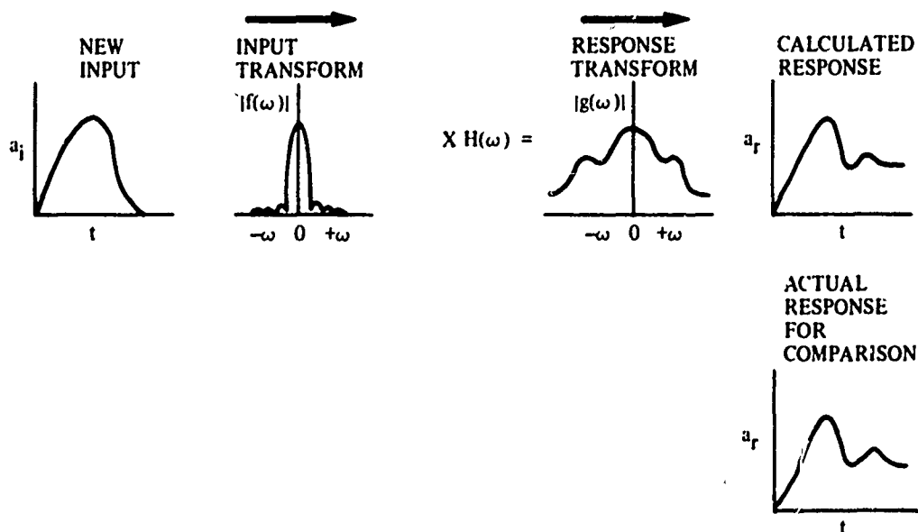
Figure 9c. Use of the Derived Transfer Function to Determine the Response to a New Input.
