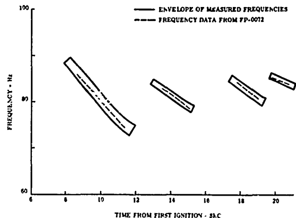
Figure 1 Envelope of Frequencies Measured During First Stage Motor Vibration and Data From a Typical Static Motor Firing
