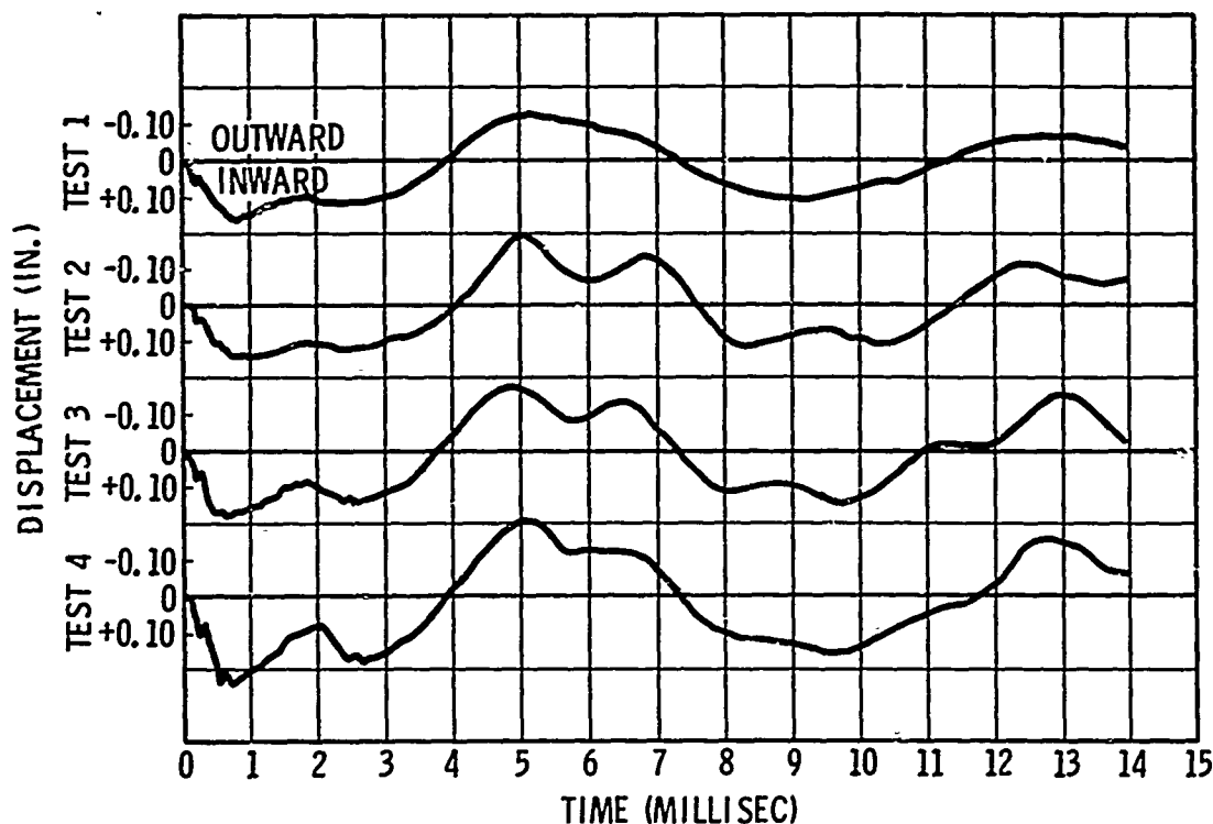
Fig. 12 - Displacement time curves
