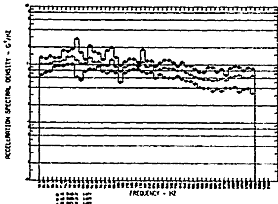
Fig. 24 - Missile - lateral - maximum, mean and minimum of TDM/pwr. ave.
