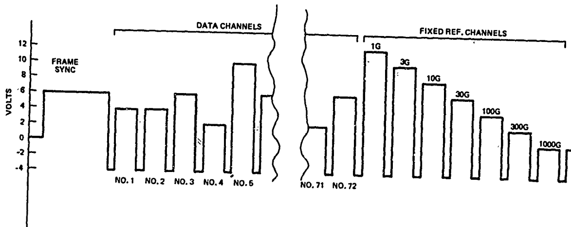
Figure 3 - Typical Scanner Output Frame
