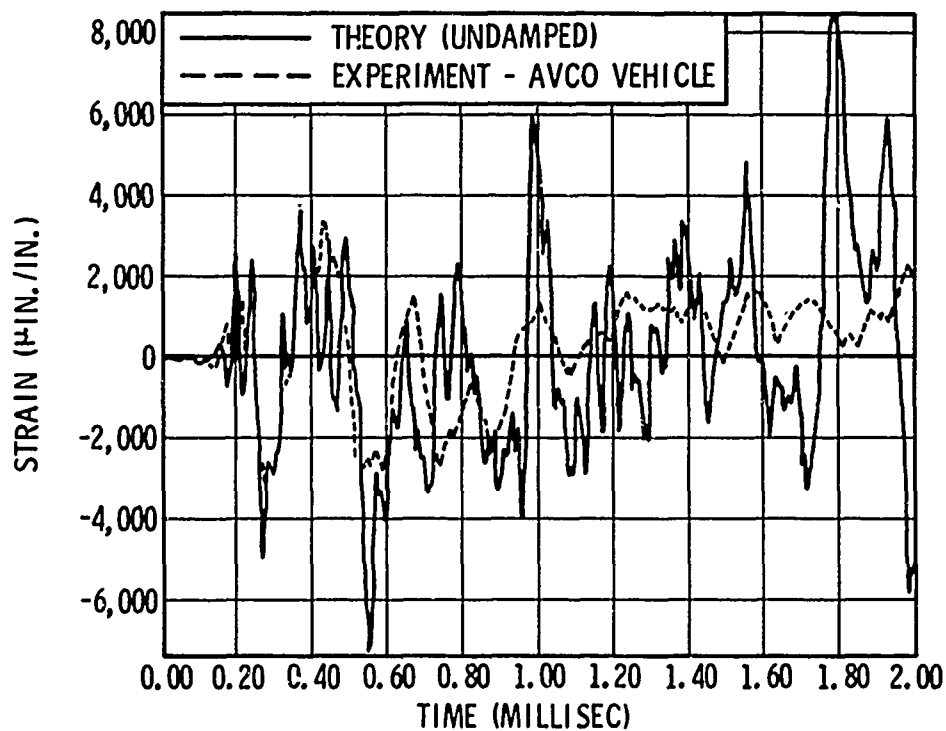
Fig. 17 - Correlation of SABOR3A/DRASTICII undamped analysis with Avco vehicle test data - outer fiber meridional strain
