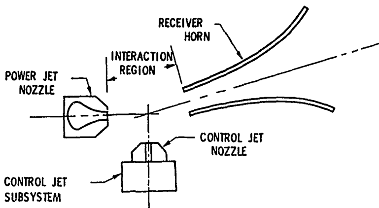
Fig. 1 - Basic Configuration of Fluidic Amplifier - Rectangular Nozzle
