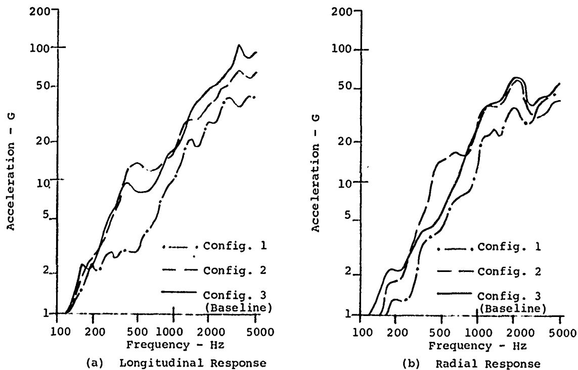
Figure 11 - Effect in spacecraft of End Condition
