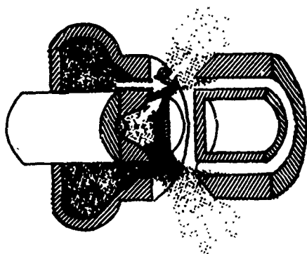
Fig. 5 - Positive Peak of an Input Cycle - Annular Slot Nozzle
