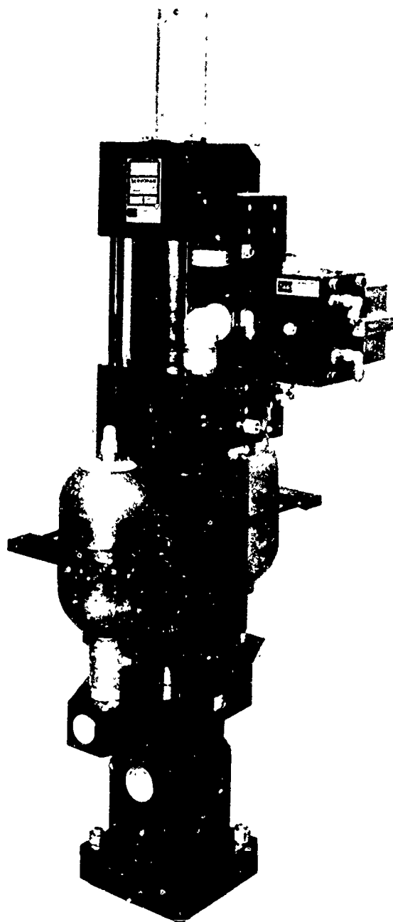
Hydraulic Tandem Actuator Providing Static 1g Support of Specimen in Vertical Direction.
