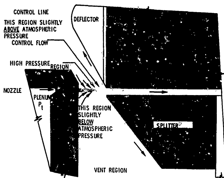
Fig. 12 - Nozzle-Vent Region Pressure Distribution, Original Configuration, No Input
