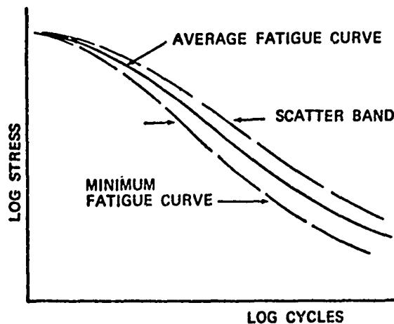
FIGURE 2a. FATIGUE SCATTER BAND ILLUSTRATION
