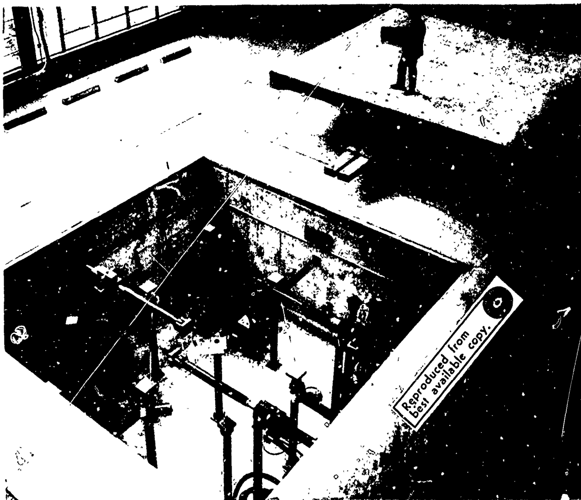
Seismic Shock Test Facility Having a 20 Foot By 20 Foot Table and 100,000 Pound Force Capacity For X-Z Motion.
