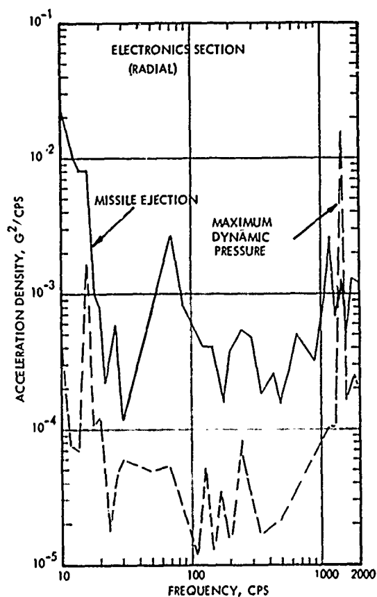
FIGURE 8 MISSILE VIBRATION MEASUREMENTS FREE FLIGHT
