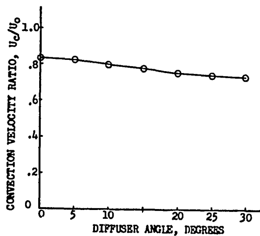
FIG. 8. CONVECTION VELOCITY OF NOISE ALONG THE DIFFUSER WALL
