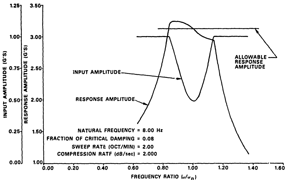
Fig. 4 - Response for swept notched excitation
