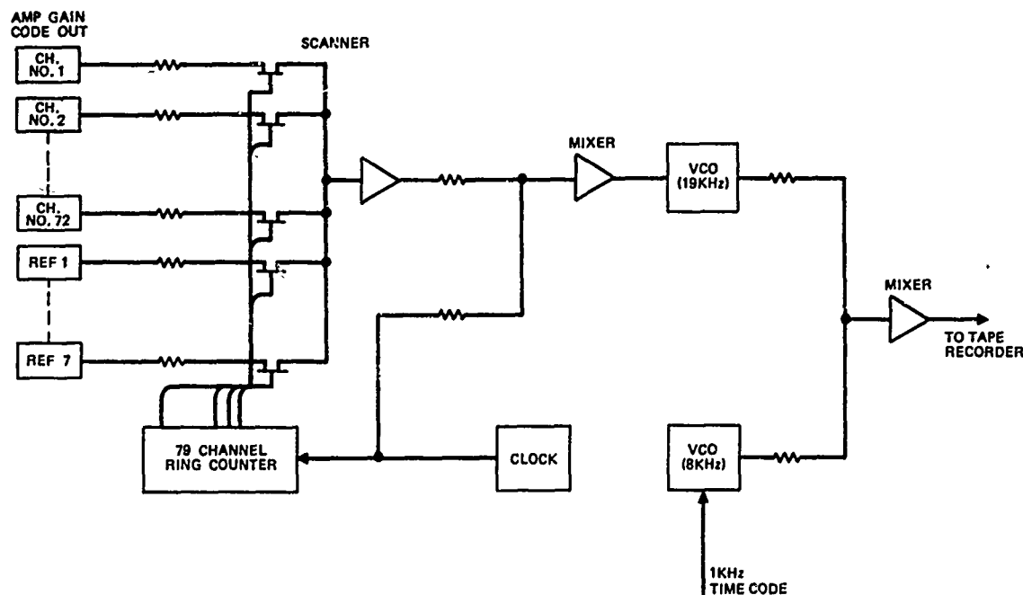
Figure 1 - Encoder Block Diagram
