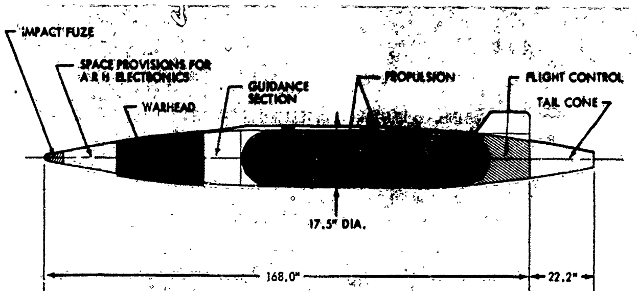
FIGURE 1 SRAM INBOARD PROFILE
