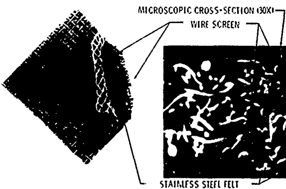
Fig. 2 - Illustration of random wire felt fiber-metal construction showing screen reinforcement and typical cross section.
