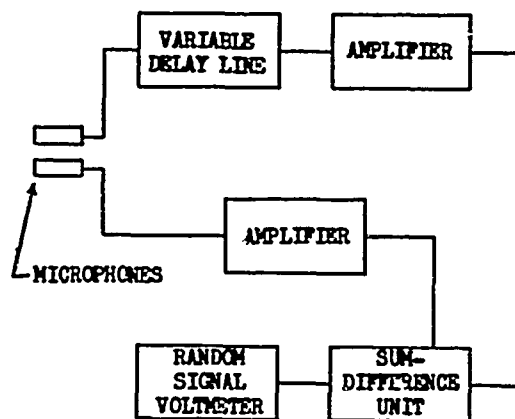
FIG. 7. BLOCK DIAGRAM OF CROSS-CORRELATION FUNCTION MEASUREMENT SYSTEM
