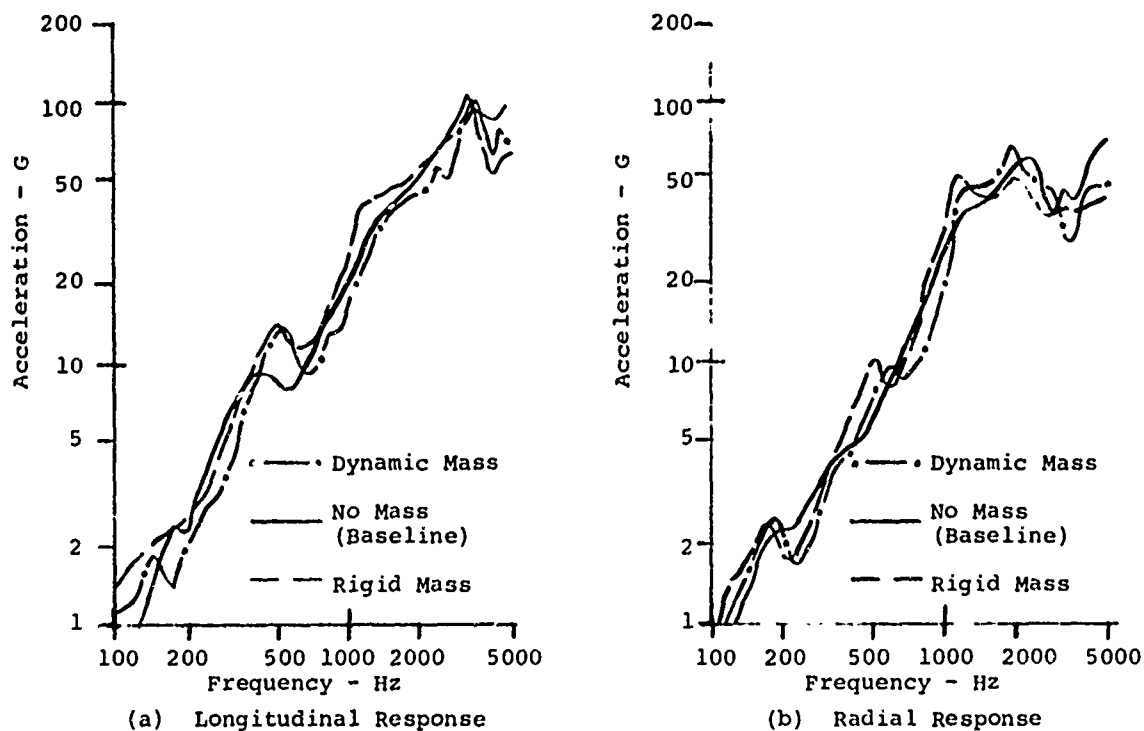
Figure 9 - Effect in Spacecraft of Mass Loading
