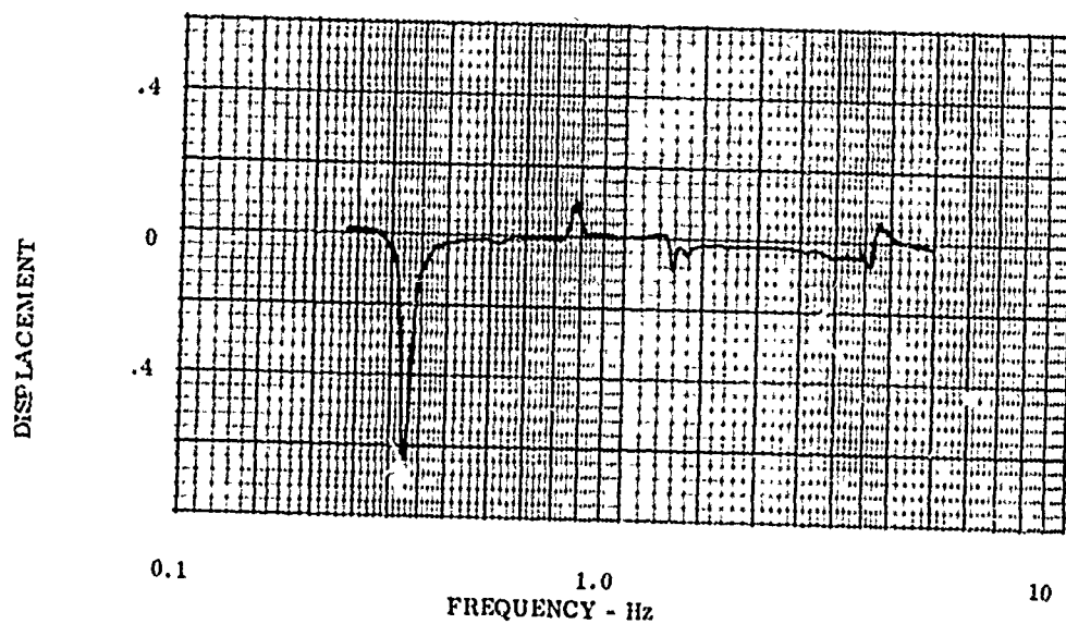
Figure 4. Quadrature Response - Translational Excitation
