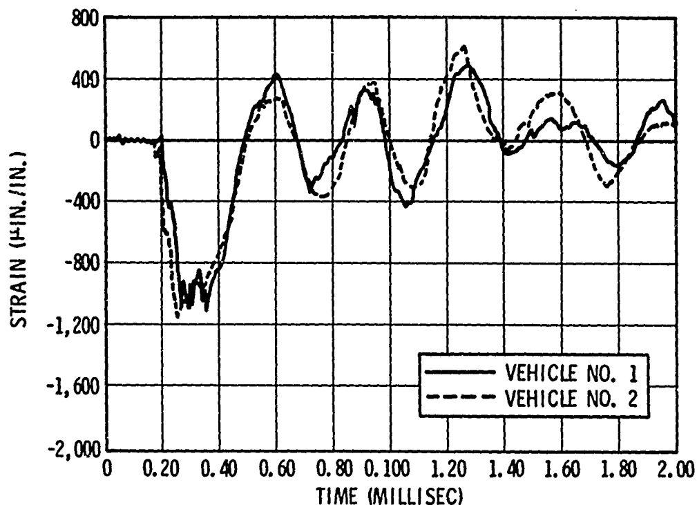
Fig. 21 - Comparison of experimental strain for two vehicles - substructure circumferential strain
