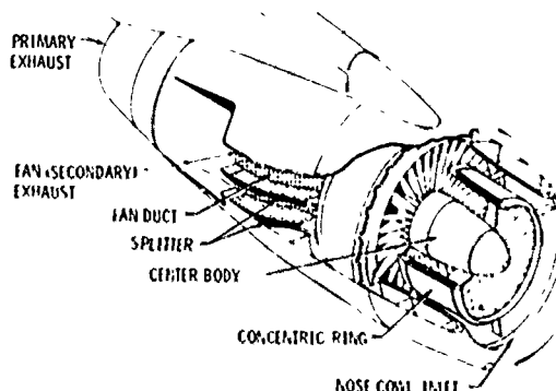
Fig. 1 - Cutaway view of modified turbofan engine nacelle showing treatment of inlet and fan ducts with acoustic material.
