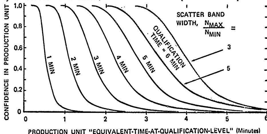
FIGURE 12. EFFECT OF QUALIFICATION TIME ON PRODUCTION UNIT CONFIDENCE (PRODUCTION UNIT FAILURE PROBABILITY = 2.3%)
