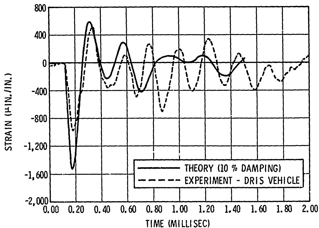
Fig. 19 - Correlation of SABOR3A/DRASTICII with DRIS vehicle test data substructure circumferential strain
