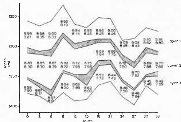
Depth variations of the layer system for Series A. Shading denotes interfaces and mean values of T and S within each layer also shown ( S to three decimals after 35‰).
