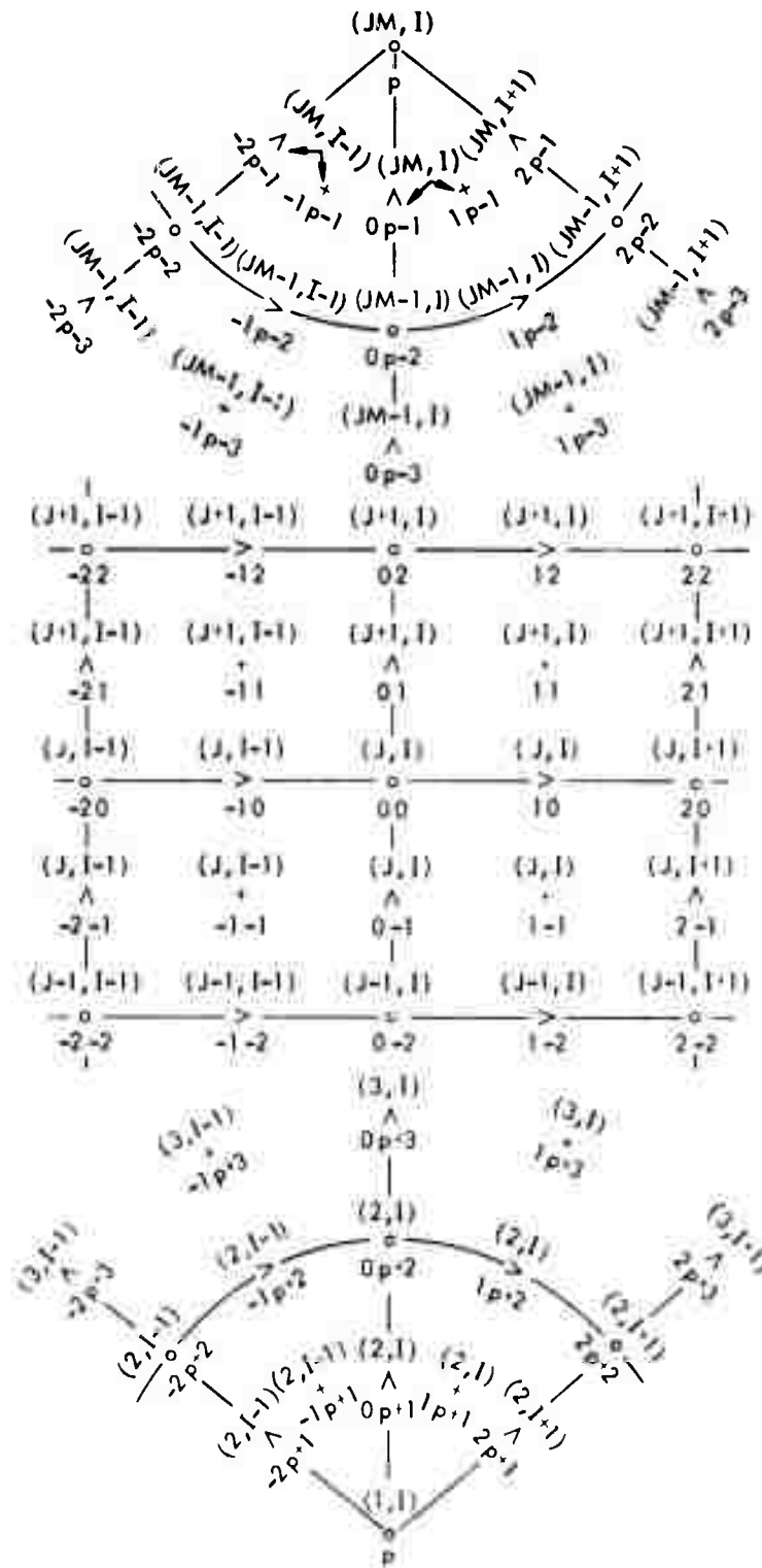
Fig. 3.6 -- The schematic finite-difference grid in \pi -centered notation. The symbols above each point are the FORTRAN J, I index, and those below each point are the finite-difference subscript notation relative to the origin 00 or relative to the poles ( p ). The open circles ( o ) are points of the \pi grid, the plus signs ( + ) are points of the u, v grid, and the carets ( \wedge and > ) are points of the v^* and u^* grids, respectively.
